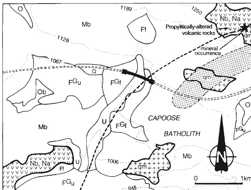
Figure 5. Bedrock and surficial geology of the region around EM survey site 1. The location of the EM survey (thick bar) along the Kluskus-Malaput forestry road (double dashed line), the inferred contact of the Capoose batholith with volcanic country rocks (thick dashed line) and an area of anomalous (10-80 ppb) gold in tills (shaded) are shown. qm – quartz monzonite; Nb, Na – basalt and andesite; FGf – glaciofluvial fan-delta; FGU – glaciofluvial outwash; Ff – alluvial fan; Mb – morained blanket; O, Ob – organics; U – undifferentiated (steep gullies).
