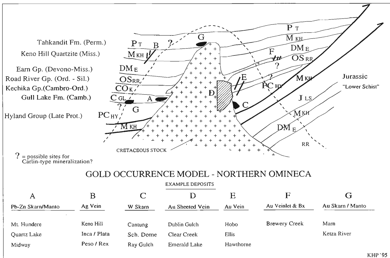
Figure 5. Schematic diagram illustrating an occurrence model for gold and related deposits in the Selwyn Basin and Cassiar Platform.
