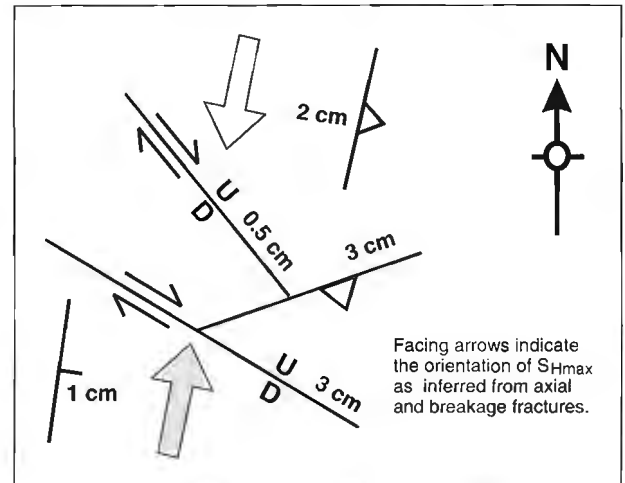
Figure 8. Orientation of, and offsets along, postglacial faults at Cheam View. Note that the movements observed are compatible with a stress regime where S_{Hmax} is oriented north to north-northeastward as could be inferred from the axial and breakage fractures at the site.
