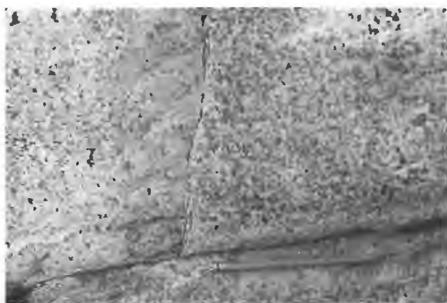
Figure 14. A hairline fracture (strike 155°, dip 76°NE) abuts against, but does not cut, a mineralized fracture striking at 45° in granodiorite of the Cochina Glacier forefield at Location 5. The fracture with a 155° azimuth is inferred to be the younger of the two structures.
