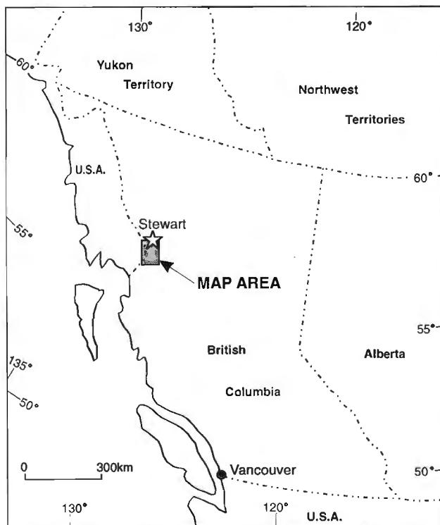
Figure 1. Location map of the study area in northwestern British Columbia. Shaded box outlines area of Figure 2.
