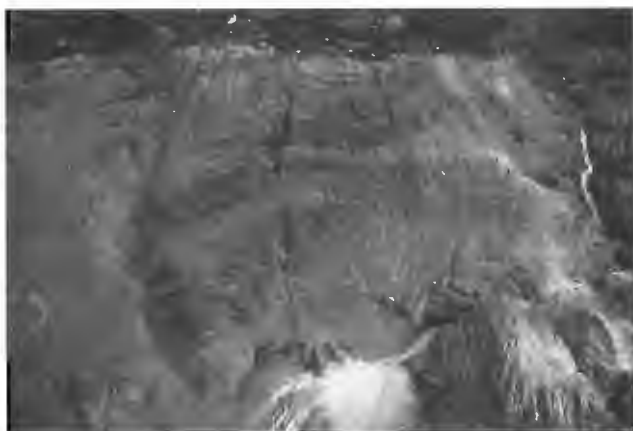
Figure 12. View northeast of southeast verging structures in Alice Arm area; width is 1 km.
