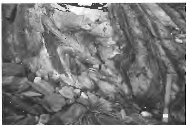
Figure 13. Ductile, rootless structures 1 km from the Hyder pluton.
