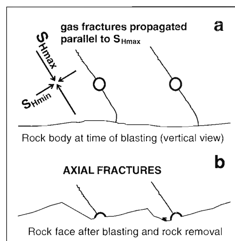
Figure 4. Schematic diagram showing the proposed origin of axial fractures in the wall of vertical boreholes during blasting. They are thought to originate as gas pressure-induced fractures.
