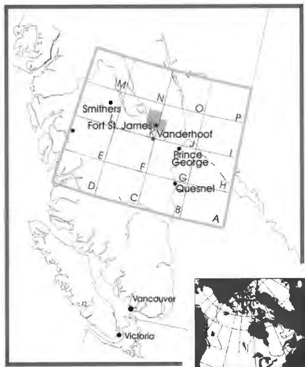
Figure 1. Regional geographic setting of the Fort St. James area. The grid represents 1:1 000 000 map of Parnip River (NTS 93). The shaded area is shown enlarged in Figure 2.
