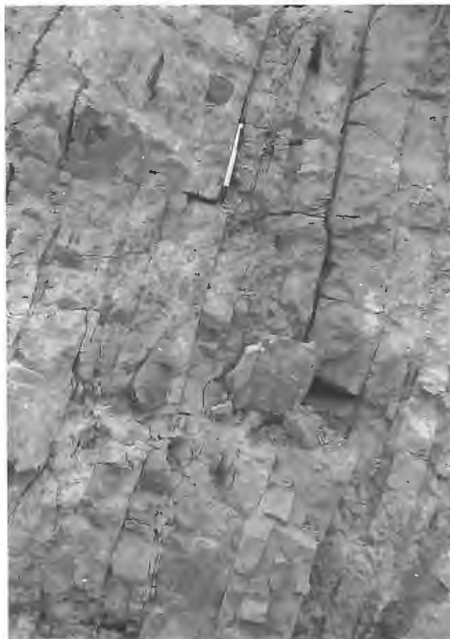
Figure 4. Silification layering in the Mount Pope sequence limestone to the east of Fort St. James.
