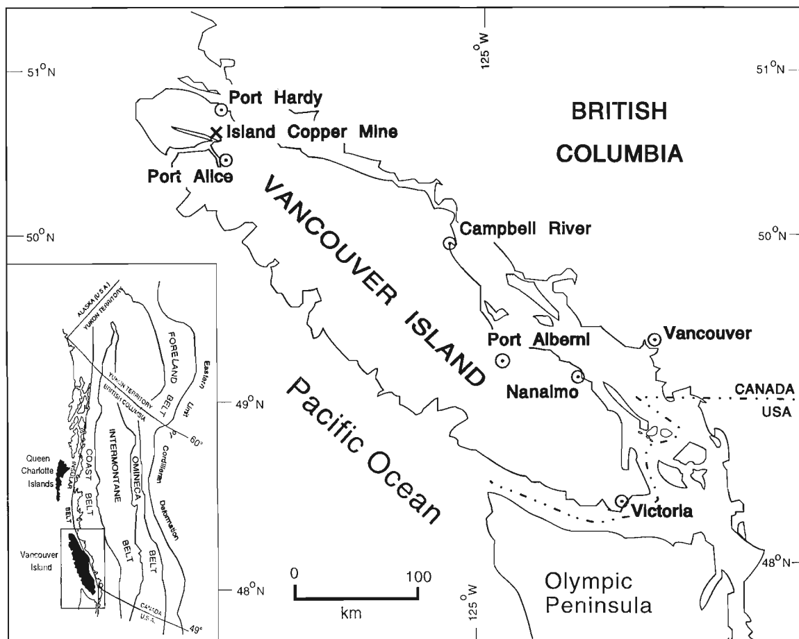
Figure 1. Location of the Island Copper mine, Port Hardy, British Columbia.
