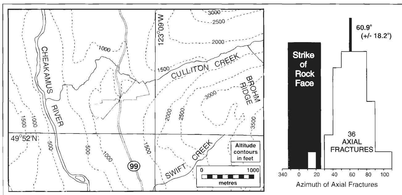
Figure 1. Map showing the location of the roadcut at Location 1 on Highway 99, south of Culliton Creek, British Columbia.
