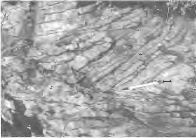
Figure 4. Close-up of chevron folds within the Stuart Lodge cherts.
