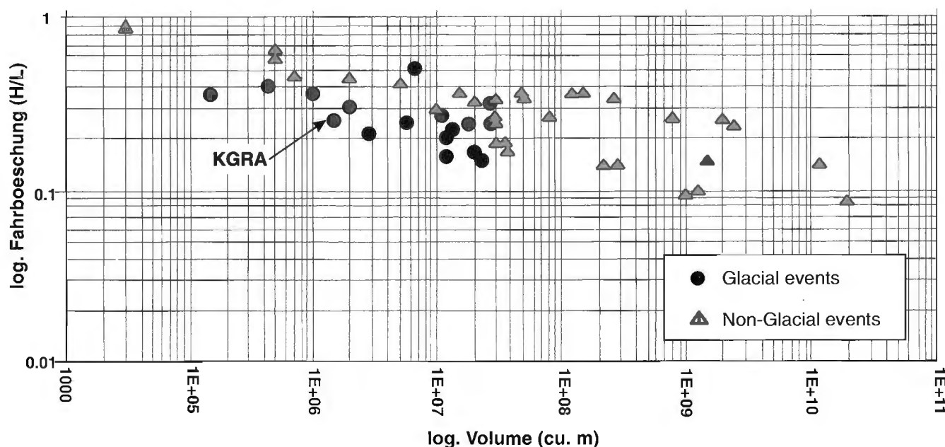
Figure 10. Plot of mobility (log. Fahrboeschung H/L) versus volume (log. volume) of rock avalanches in glacial and nonglacial environments. Data for the graph was taken from Clague and Evans (1988) for "glacial" events, and from Scheidegger (1973) for "nonglacial" events. The arrow points to the data point for the Kshwan Glacier rock avalanche (KGRA).
