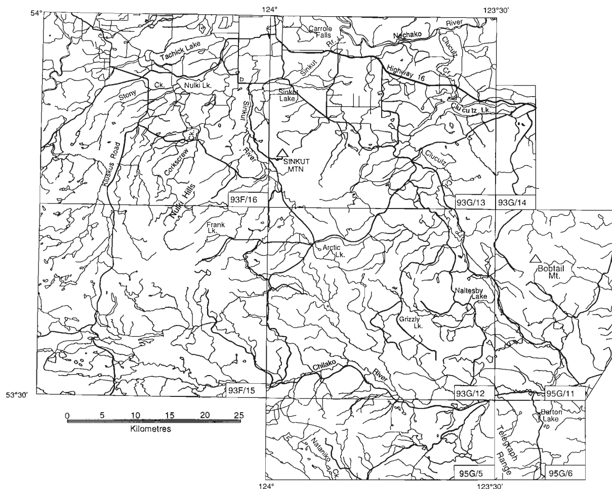
Figure 4. Index map of geographic and geological features of the area referred to in the text.
