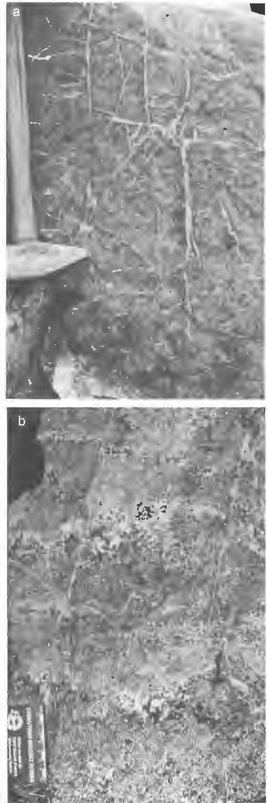
Figure 5. Typical rock types of the Joe Mountain volcanic complex include: a) microdiorite which is typically crosscut by reticulate networks of thin white veinlets; and b) texturally variable, coarsely crystalline pyroxene gabbro.
