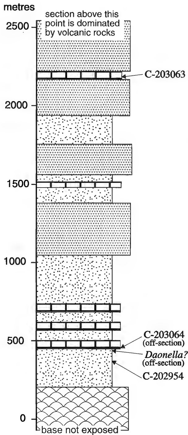
Figure 4. Section and sample localities from the predominantly sedimentary portion of the Joe Mountain volcanic complex. The section is compiled from 1:25 000 mapping by the first author starting from 60°54.5'N, 134°43.0'W. Rock patterns are the same as those in Figure 3.
