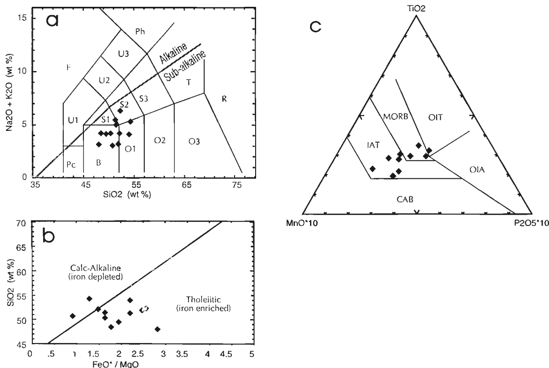
Figure 6. All data are plotted as anhydrous. a) Total alkalis vs silica classification diagram with subdivisions of Le Maitre (1989); B = basalt, O1 = basaltic andesite, S1 = trachybasalt, S2 = basaltic trachyandesite. Alkaline/subalkaline curve from Irving and Baragar (1971). b) Calc-alkaline/tholeiitic discrimination diagram (Miyashiro, 1974). c) Minor element discriminate plot for basaltic rocks (45-54% SiO 2 ; Mullen, 1983). CAB = calc-alkaline basalt, IAT = island arc tholeiite, MORB = mid-ocean ridge basalt, OIT = ocean island tholeiite, OIA = ocean island andesite.
