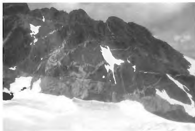
Figure 7. View north of dykes emanating from the Hyder pluton into clastic rock of the Bowser Lake Group; width of view is 800 m.
