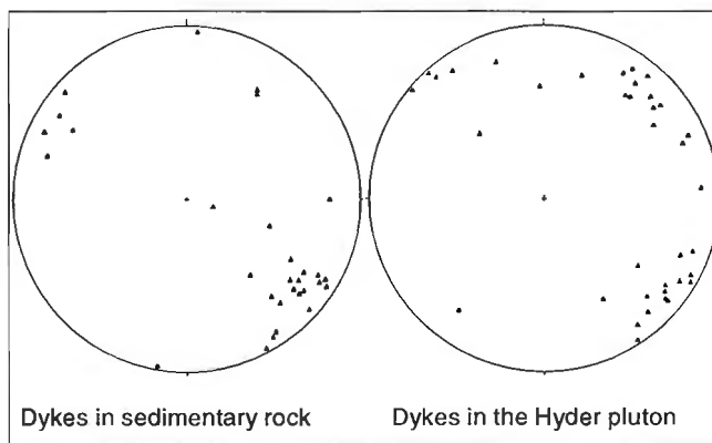
Figure 6. Lower hemisphere projections of poles to dykes (mostly in Alice Arm area).
