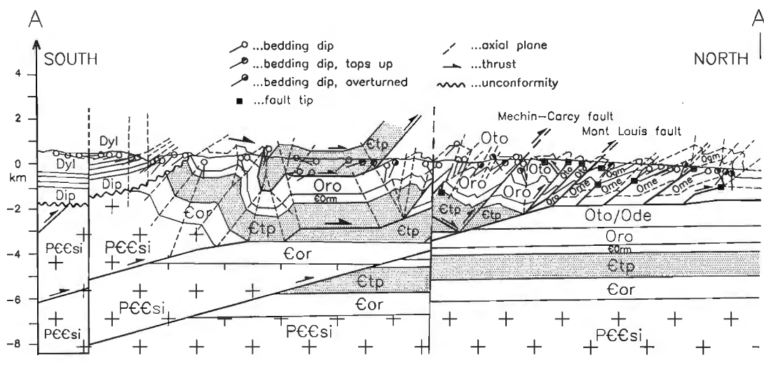
Figure 4. North-south structural cross-section through the Humber Zone in the Gaspésie region. Position of section (A-A') is shown on the map of Figure 2. Legend of stratigraphic units is contained in Figure 2.
