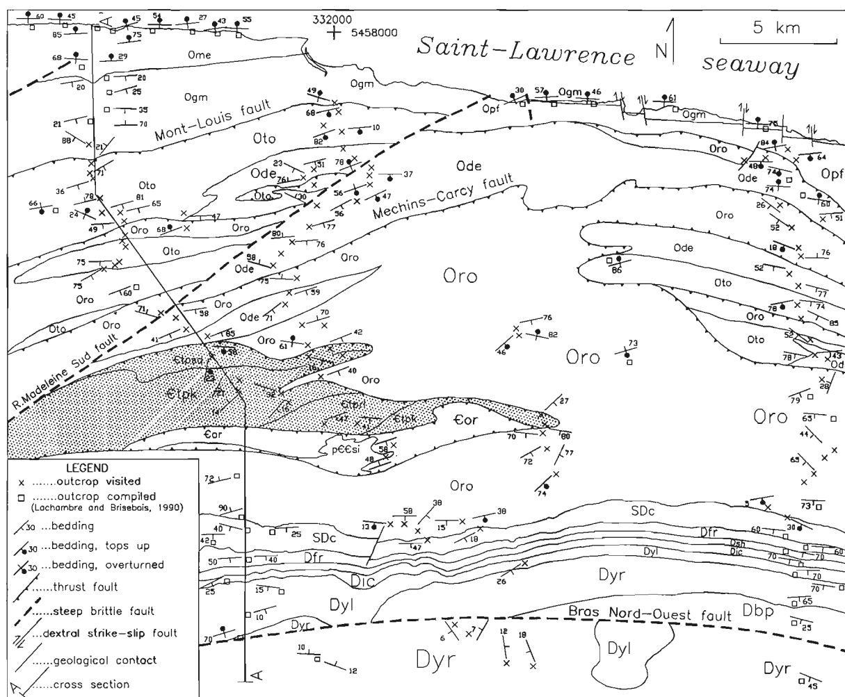
Figure 2. Simplified geology map of Gande Vallée (NTS 22H/03). The x symbol denotes positions of outcrops visited during the course of this study, whereas squares are information taken from compilation of Lachambre and Brisebois (1990). Legend of stratigraphic units is contained in Figure 3.
