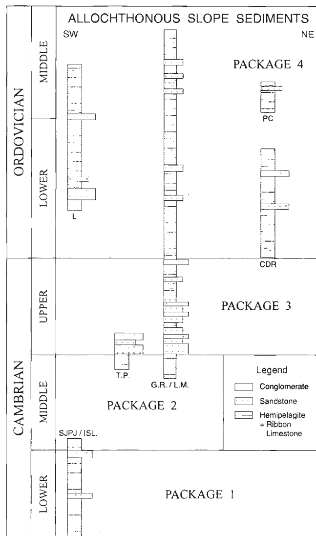
Figure 2. Cambro-Ordovician lithostratigraphic packages proposed for the Humber Zone continental slope deposits in eastern Quebec. SJPJ - ISL is for Saint-Jean-Port-Joli-Islets, L is for Lévis, T.P. is for Trois-Pistoles, G.R. / L.M. is for Grosses-Roches / Les Méchins, CDR is for Cap-des-Rosiers, PC is for Pointe Carse.
