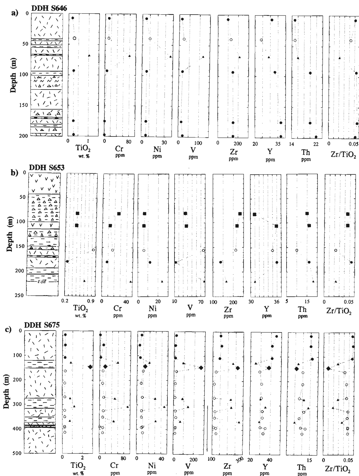
Figure 4. Diamond-drill hole (DDH) profiles for a) S646, b) S653, c) S675, d) S677, e) S710, and f) S1013 illustrating \text{TiO}_2 , Cr, Ni, and V variations that are particularly important for discriminating the lower and upper (footwall) sedimentary rocks, and Zr, Y, Th, and \text{Zr/TiO}_2 contents that are important in identifying hanging wall and footwall crystal tuffs. Interpreted lower footwall sedimentary rocks (Miramichi Group-like) ( \blacktriangle ), and upper footwall sedimentary rocks (Nepisiguit Falls Formation) ( \triangle ), footwall crystal tuffs/tuffites ( \circ ), hanging wall crystal tuff ( \bullet ), and mafic volcanic/dike ( \blacklozenge ).
