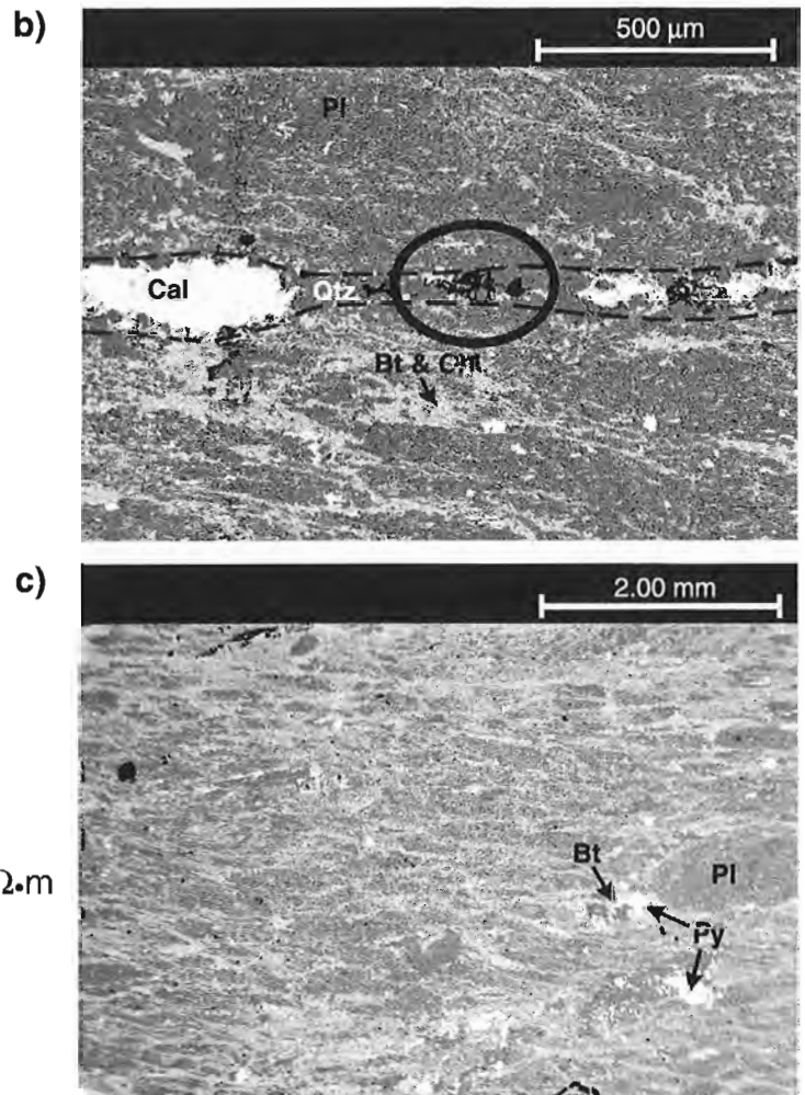
Figure 2. a) Schematic representation for specimens MXF-1a and MXF-1b and b) and c) SEM images for specimen MXF-1a, with \rho_r and \lambda values (lower left-hand section of Fig. 1a). The SEM images (BSI) highlight the quartz (Qtz)-calcite (Cal) vein (dashed line) and displays the distribution of plagioclase (Pl), biotite (Bt), and chlorite (Chl) within the groundmass of b). Disseminated pyrite (Py) grains are also indicated in c).
