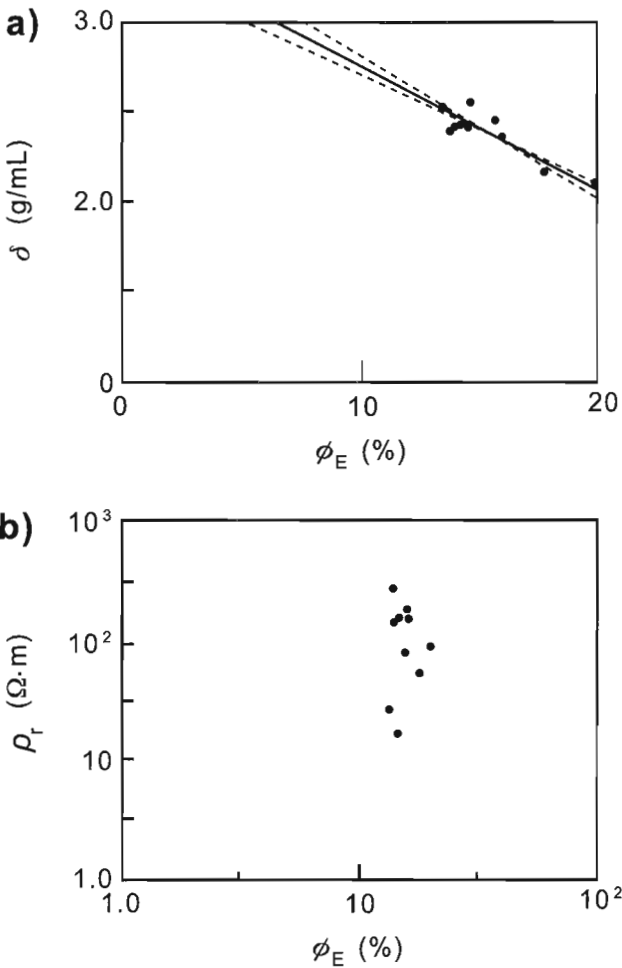
Figure 3. a) Bulk density ( \delta ) as a function of effective porosity ( \phi_E ) (RMA: \delta = -0.068\phi_E + 3.44 , r = -0.88 ); RMA is represented by a solid line and the normal regression lines are represented by dashed lines; b) bulk electrical resistivity ( \rho_r ) as a function of effective porosity ( \phi_E ); RMA is the reduced major axis and r is the correlation coefficient. The principles of the RMA are described in Davis (1986), and examples of related applications are found in Katsube and Agterberg (1990).
