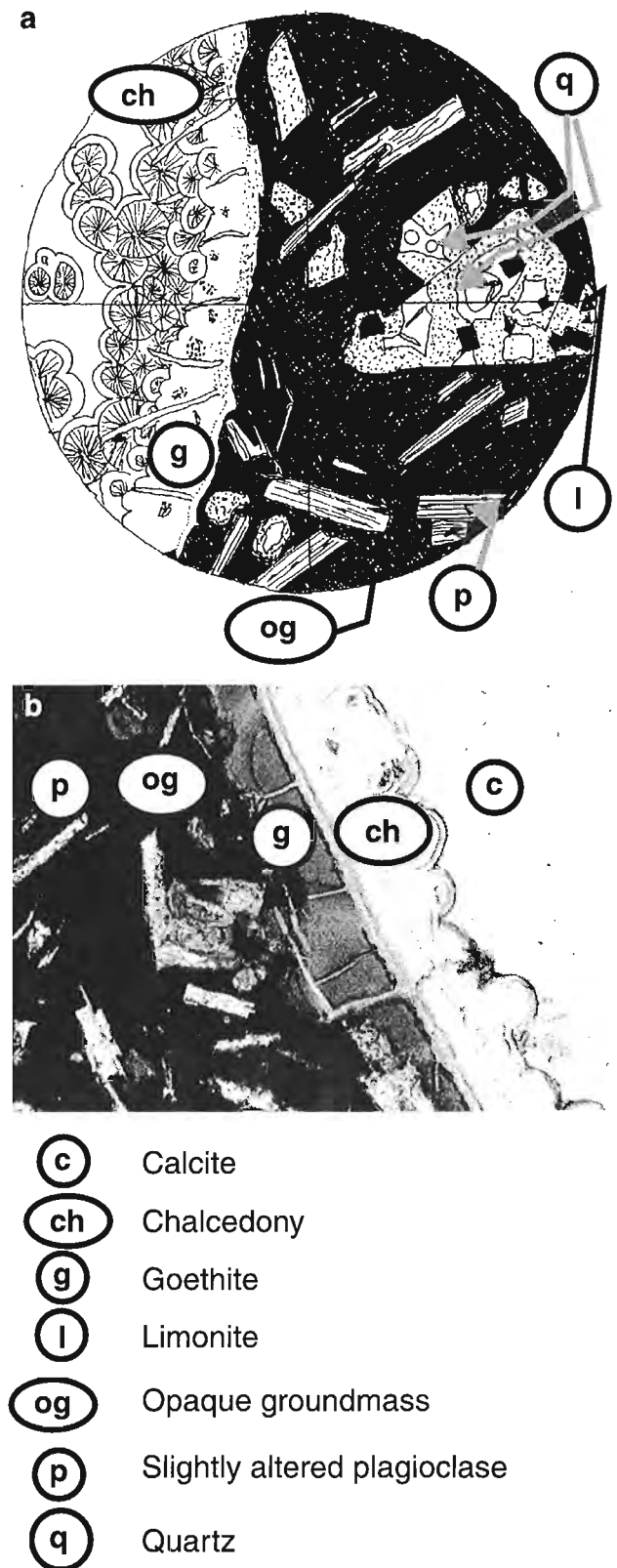
Figure 5. a) Camera lucida sketch, and b) photomicrographs (plane-polarized light) of distinctive petrographic textures for sample 0102G. Note goethite and geopetal structures characterized by shatter cracks as initial vesicle fillings. Iron hydroxides are overgrown by chalcedony and calcite. Magnification in sketch is 10x; width of photomicrograph images is 1.4 mm.
