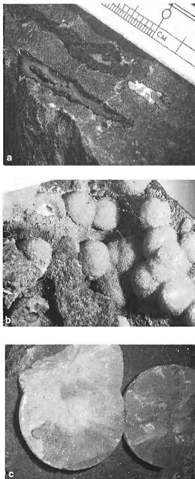
Figure 3. Typical mineral habits for amygdules in hand sample for samples: a) 0101E: flattened vesicle contains black iron hydroxides with shatter cracks and inner zone of chlorite(?); b) 0103F: calcite spherules (greyish orange, 5YR 4/4; field of view 5.5 cm wide); and, c) 0104G: zoned calcite disk-like amygdules (greyish orange, 10YR 7/4; disks 2 cm in diameter).
