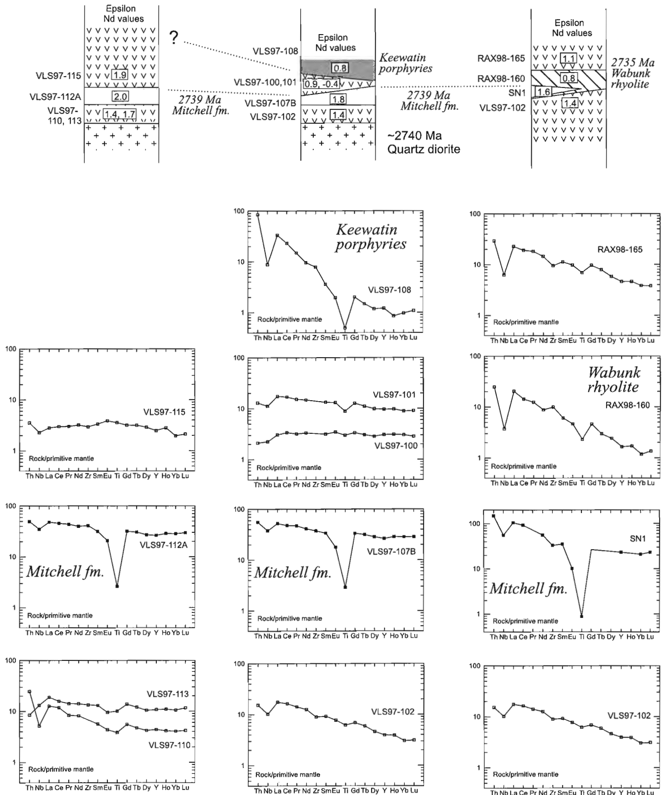
Figure 5. Top: simplified sections showing the relative position of felsic units and mafic units within the Confederation assemblage and the \epsilon\text{Nd} values (at 2.74 Ga) of samples analyzed. (Legend is the same as Figure 4.) Bottom: corresponding mantle-normalized multi-element diagrams for the same samples (and their relative position stratigraphically).
