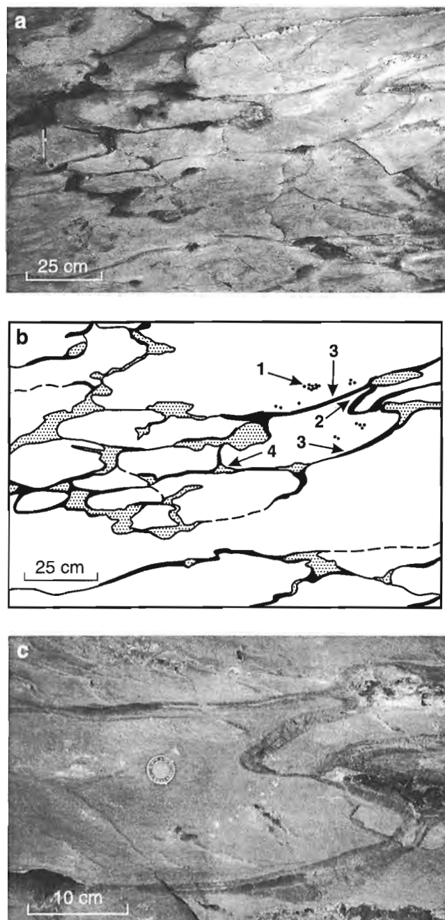
Figure 4. Pillow structure in metabasalt at Mont Tétreault (locality 1.1): a) decimetric size, bulbous, slightly flattened pillows are viewed in section at high angle to the stretching direction. The weathered recessed pillow interspaces are filled with calc-silicate minerals. b) line drawing of a) highlighting the pillow morphology: note that the distribution of the vesicles 1), the pillow peduncle 2), the curvature of the selva 3), and the triangular shape of the interspace 4) indicate a top-side-down facing direction; c) close-up showing the thin pillow selva, coarsening of relict grain size in the pillow core, and a few weathered, recessed calcite-filled vesicles.
