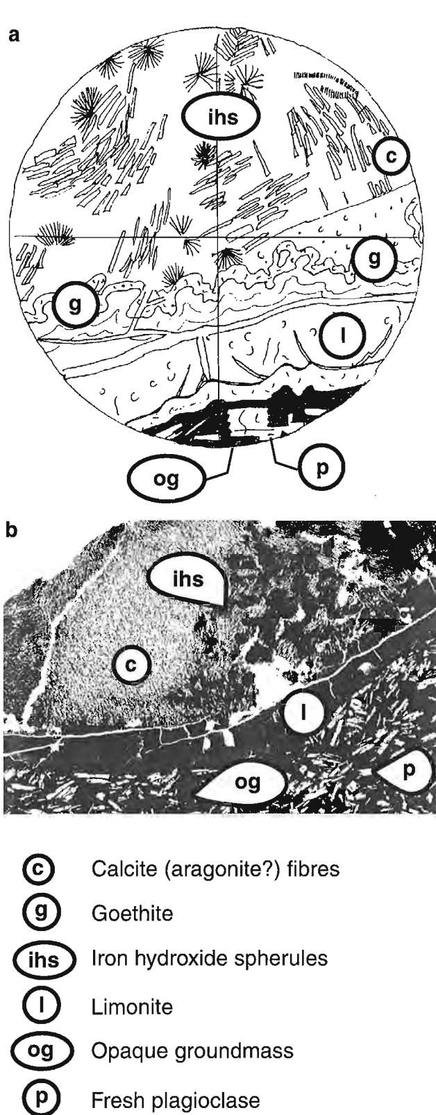
Figure 4. a) Camera lucida sketch, and b) photomicrograph (plane-polarized light) of distinctive petrographic textures for sample 0101E. Note limonite geopetal structure characterized by shatter cracks as initial vesicle filling and later iron hydroxide spherules overgrown by calcite crystal. Magnification in sketch is 10x; width of photomicrograph image is 5.6 mm.
