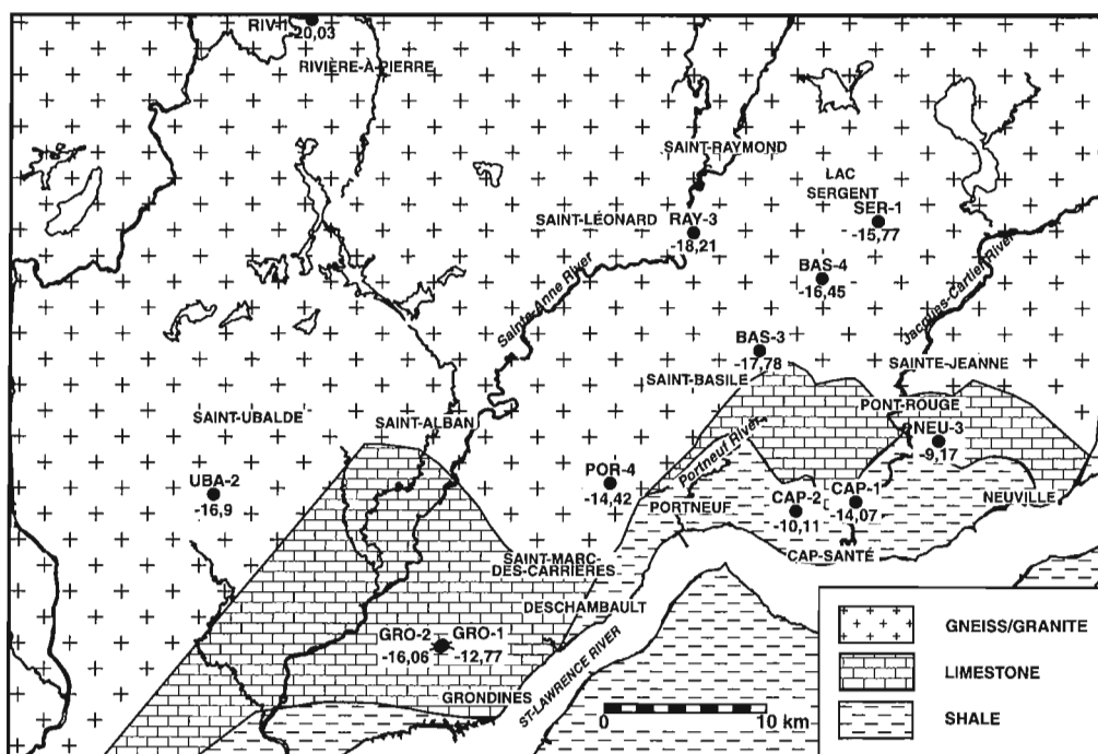
Figure 4. A \delta^{13}\text{C}_{\text{DIC}} map of groundwater in rocks aquifers from the Portneuf region, autumn 1995.
