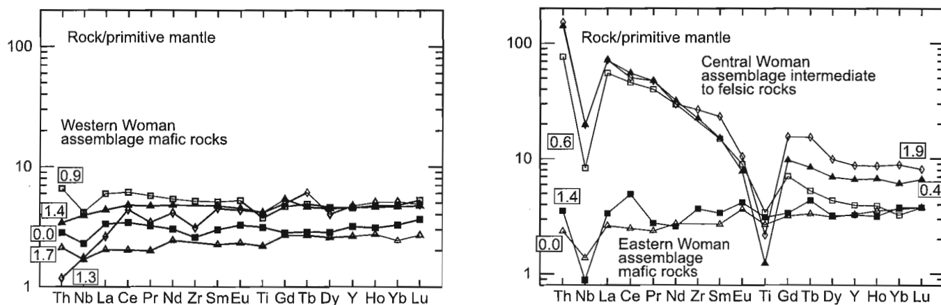
Figure 3. Mantle-normalized multi-element diagrams and epsilon Nd values for Woman assemblage rocks. Labels in boxes are the \epsilon_{\text{Nd}} values of the samples at 2.84 Ga.
