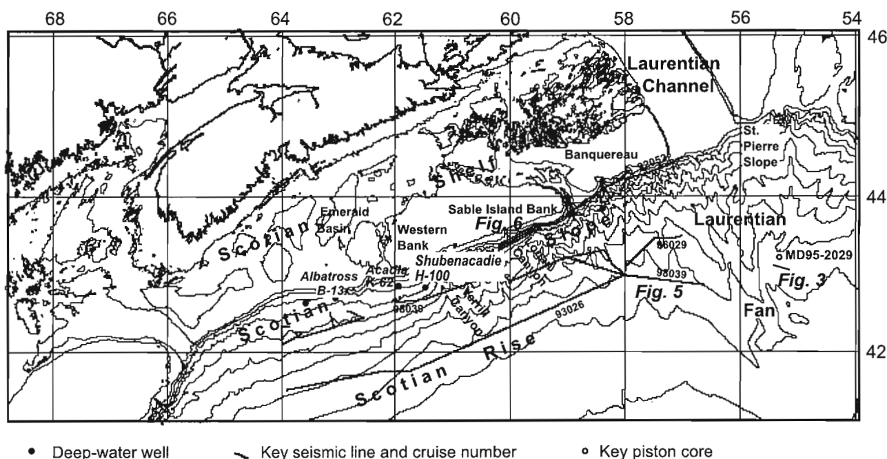
Figure 1. General map of Scotian margin showing deep-water wells, piston core, and seismic lines used for stratigraphic correlation and to map debris-flow deposits.
