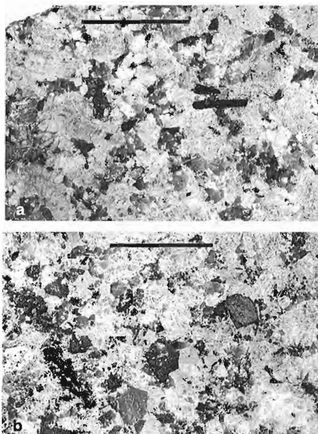
Figure 8. Textures in Tetachuck-north pluton: a) sample SCBF98-4708; scale bar is 1 cm long. Plagioclase is pale grey, quartz is darker grey, and mafic minerals are black. Note the euhedral hornblende crystal. b) Sample SCBB98-0803; scale bar is 1 cm long. Plagioclase is pale grey, quartz is darker grey and mafic minerals are black. Note the euhedral biotite crystals.
