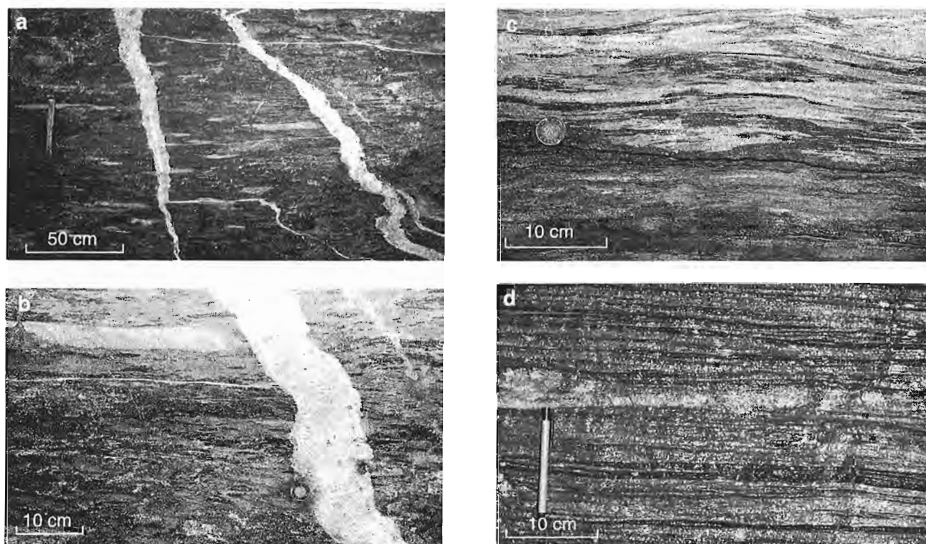
Figure 6. Hydrothermally altered metabasalt with felsic fragments at Lac des Pins (locality 8): a) flattened, matrix-supported, felsic fragments in amphibolite; b), c) close-up highlighting the composite nature of the matrix, and the delicately sutured contact between dark hornblende-rich, and lighter clinopyroxene-rich parts of the matrix; and d) derived straight gneiss.
