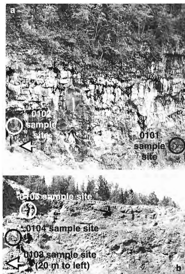
Figure 2. Location of samples: a) Lower part of Endako Group sequence north of, and at the base of, Kenney Dam; figure (see arrow) is 1.8 m tall. Samples 0101 and 0102 locations shown; b) Upper part of Endako Group sequence, south of Kenney Dam; cliff is ca. 70 m tall. Locations of samples 0103, 0104, and 0105 shown. No distinctive amygdaloidal minerals were observed in sample 0105.
