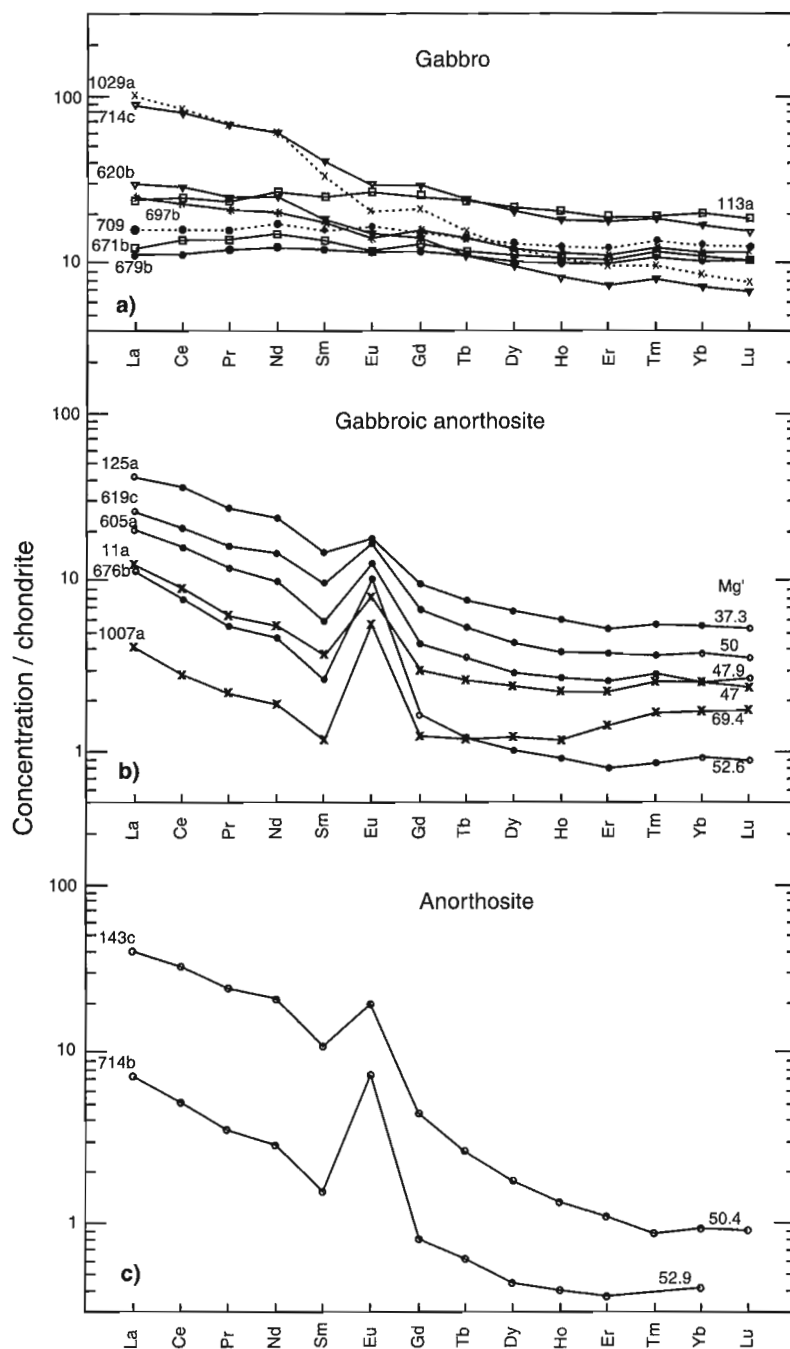
Figure 4. REE abundances for mafic rocks from the Kramanituar Complex normalized to chondrite values of Sun (1980). a) Gabbro. b) Gabbroic anorthosite with Mg number (see Table 1) for each representative sample shown. c) Anorthosite with Mg number.
