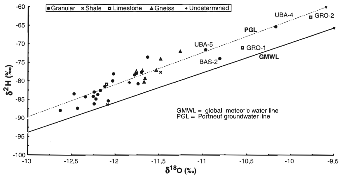
Figure 3. Plot of \delta^2\text{H} versus \delta^{18}\text{O} values from the autumn 1995 campaign classified by origin of aquifer.
