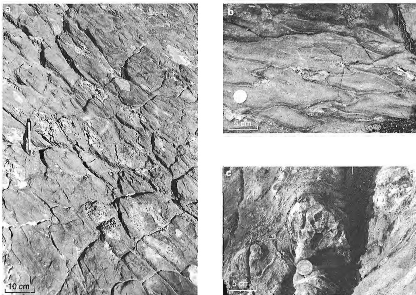
Figure 5. Pillowed metabasalt at Rousseau (locality 3): a), b) deformed pillows in sections respectively oblique and at high angle to the stretching direction; note the decimetric size of the pillows and the thickness of the selvages; c) close-up showing hyaloclastic interpillow matrix.
