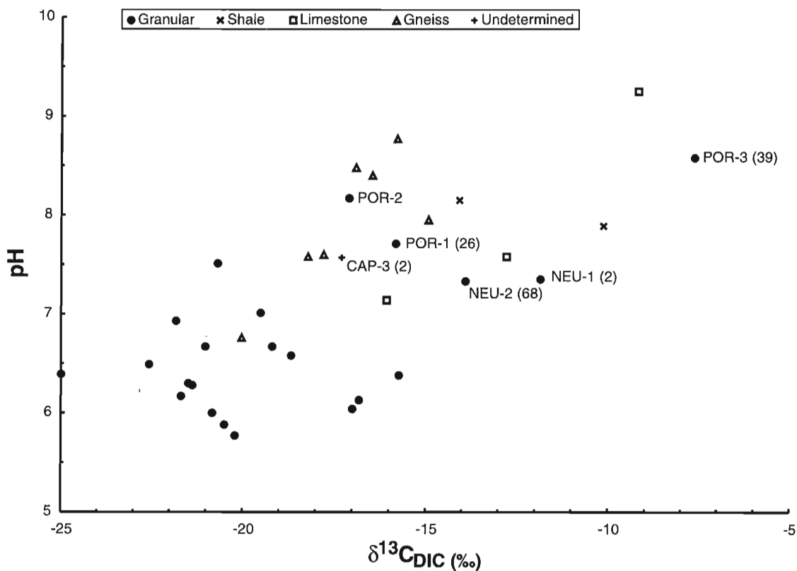
Figure 5. Relationships between \delta^{13}\text{C}_{\text{DIC}} and pH of groundwater from the Portneuf region, autumn 1995.
