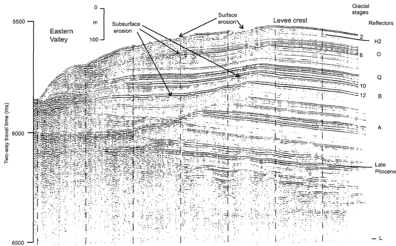
Figure 3. Seismic-reflection profile from the eastern levee of Eastern Valley of Laurentian Fan, showing key stratigraphic reflectors and correlation with core MD95-2029 (Cruise HU84-040).
