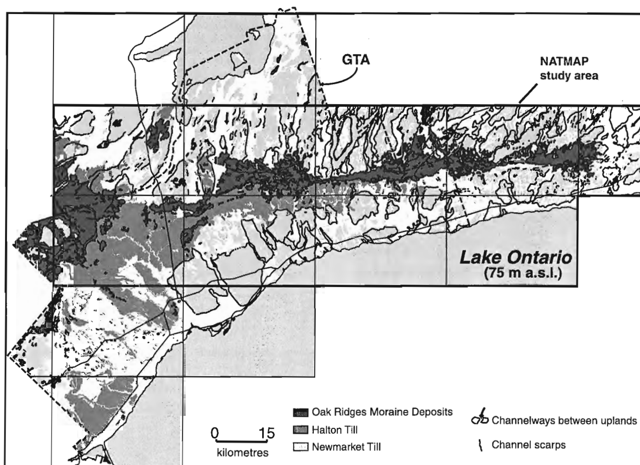
Figure 6. Generalized terrain and geology map of the ORM-GTA emphasizing three regionally extensive units and a channel network of the stratigraphic model, Figure 3. (See Figure 1 for context)
