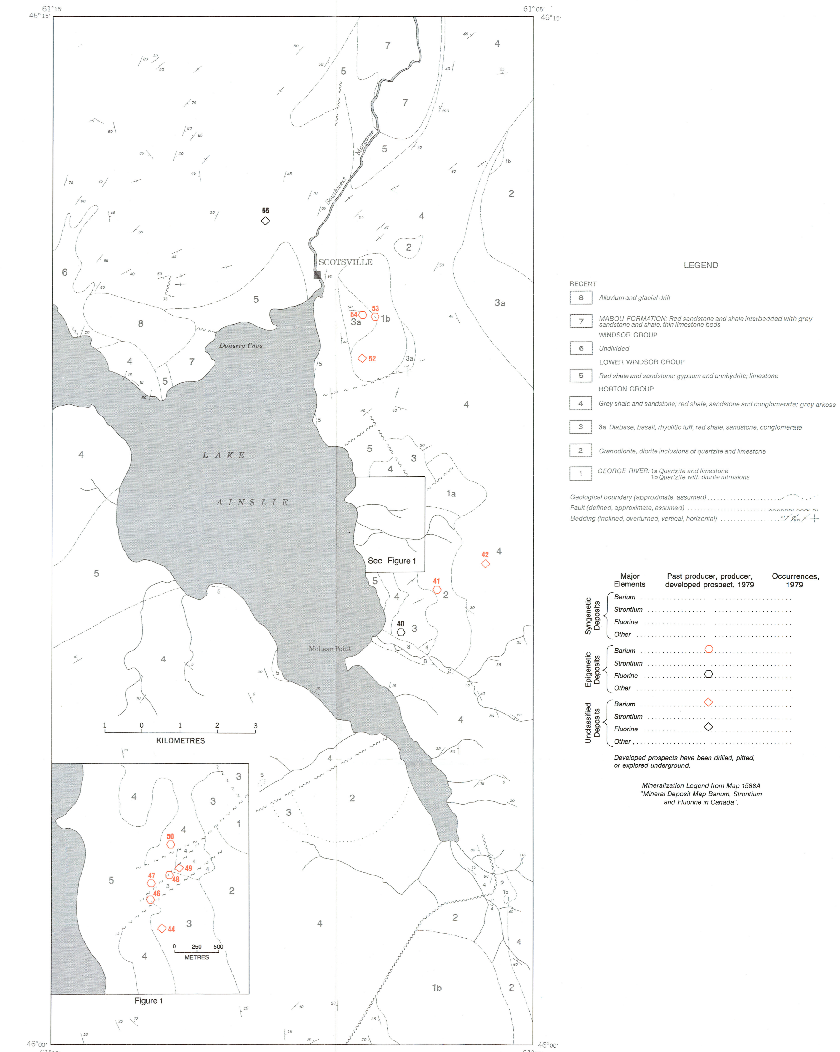
Figure 17. Geology and index to deposits and occurrences of barium and fluorine minerals, Lake Ainslie East, Cape Breton Island, Nova Scotia, after Norman (1935) and Zurowski (1972).
