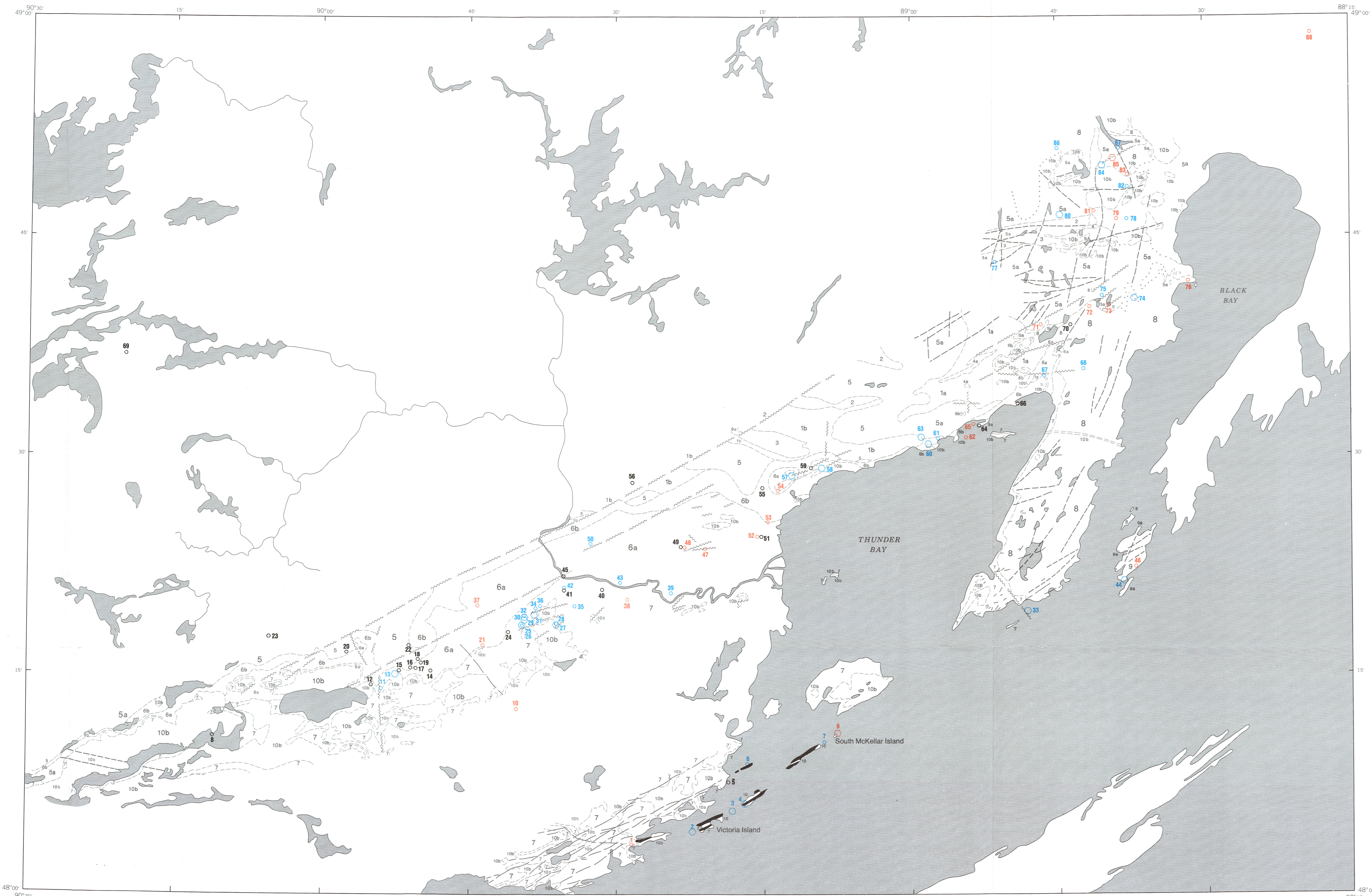
Figure 16. Geology and index to deposits and occurrences of barium and fluorine minerals, Thunder Bay, Ontario, after Pye (1965, 1968).
