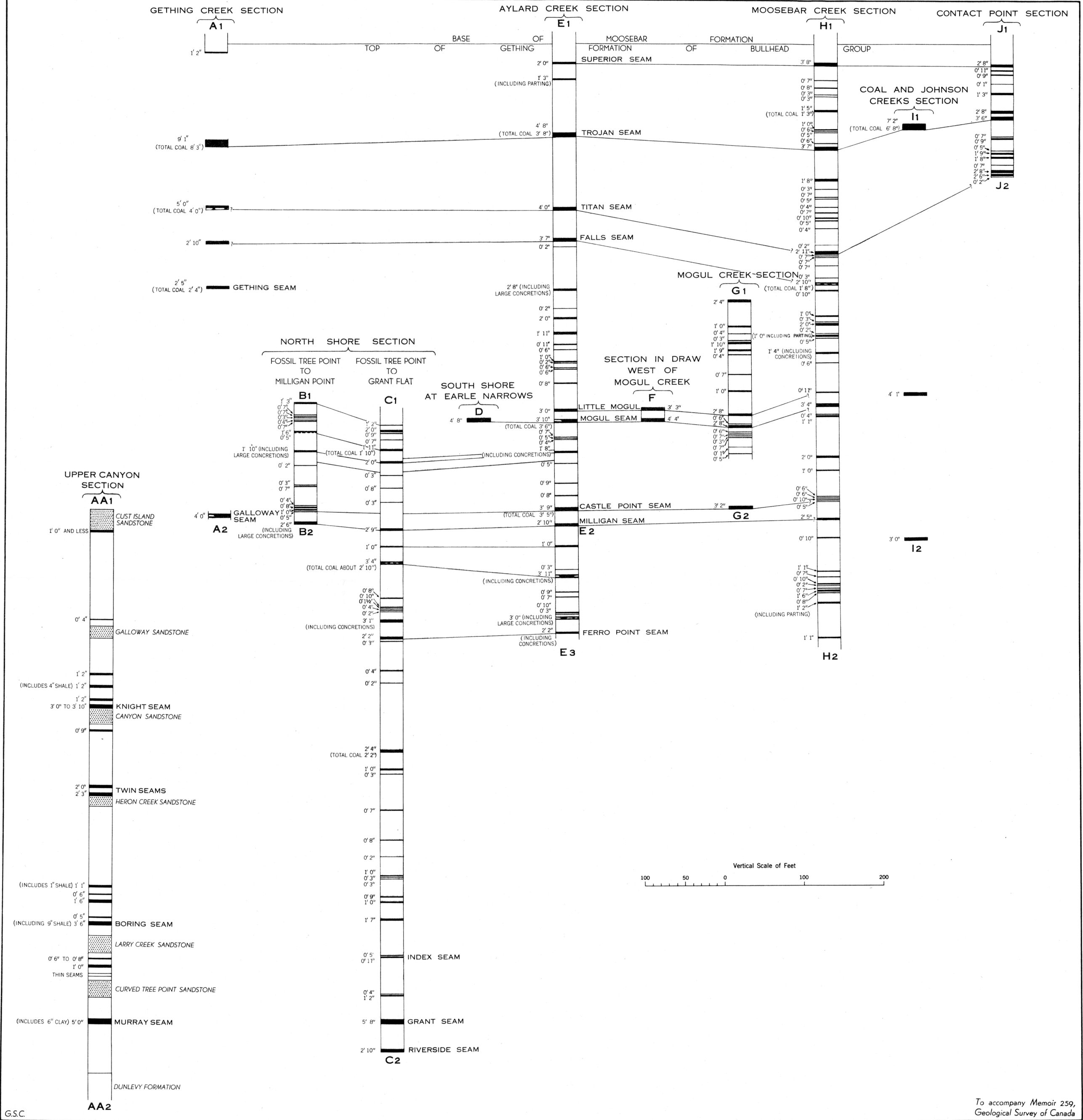
Figure 14. Columnar sections showing correlation of coal seams in Gething formation, Peace River Canyon coal area, British Columbia. For location of sections, see Figure 11. Columnar section AA1-AA2 based on field work by F.H. McLearn and E.J.W. Irish, 1943; sections A1-A2 to J1-J2 reproduced from Sum.Rept.1922 pt.B, by F.H. McLearn.
