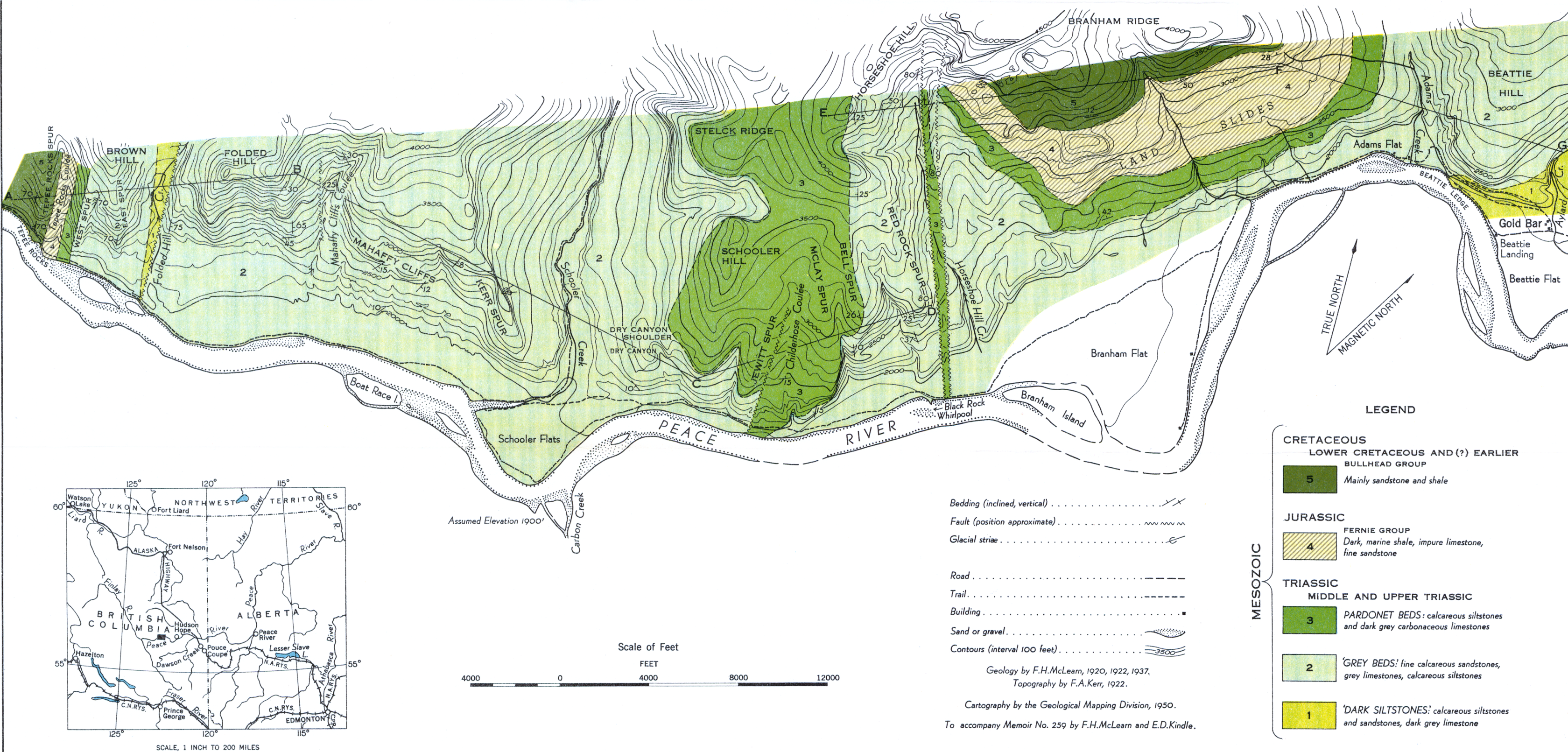
Figure 8. Geological map and structure-sections of area north of Peace River, Tepee Rocks Spur to Aylard Creek, Peace River Foothills, British Columbia.
