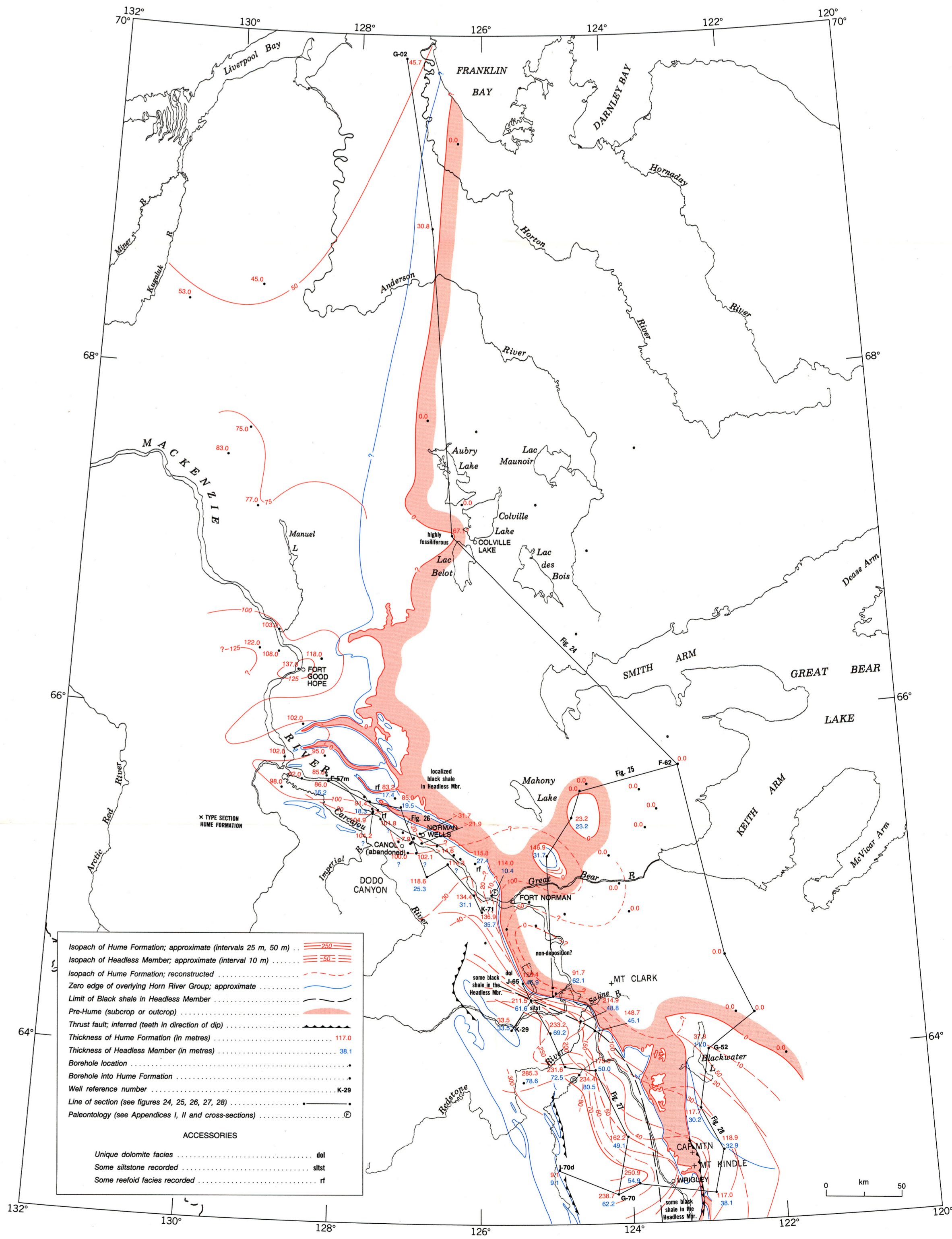
Figure 13. Isopach and lithofacies map of Hume Formation
