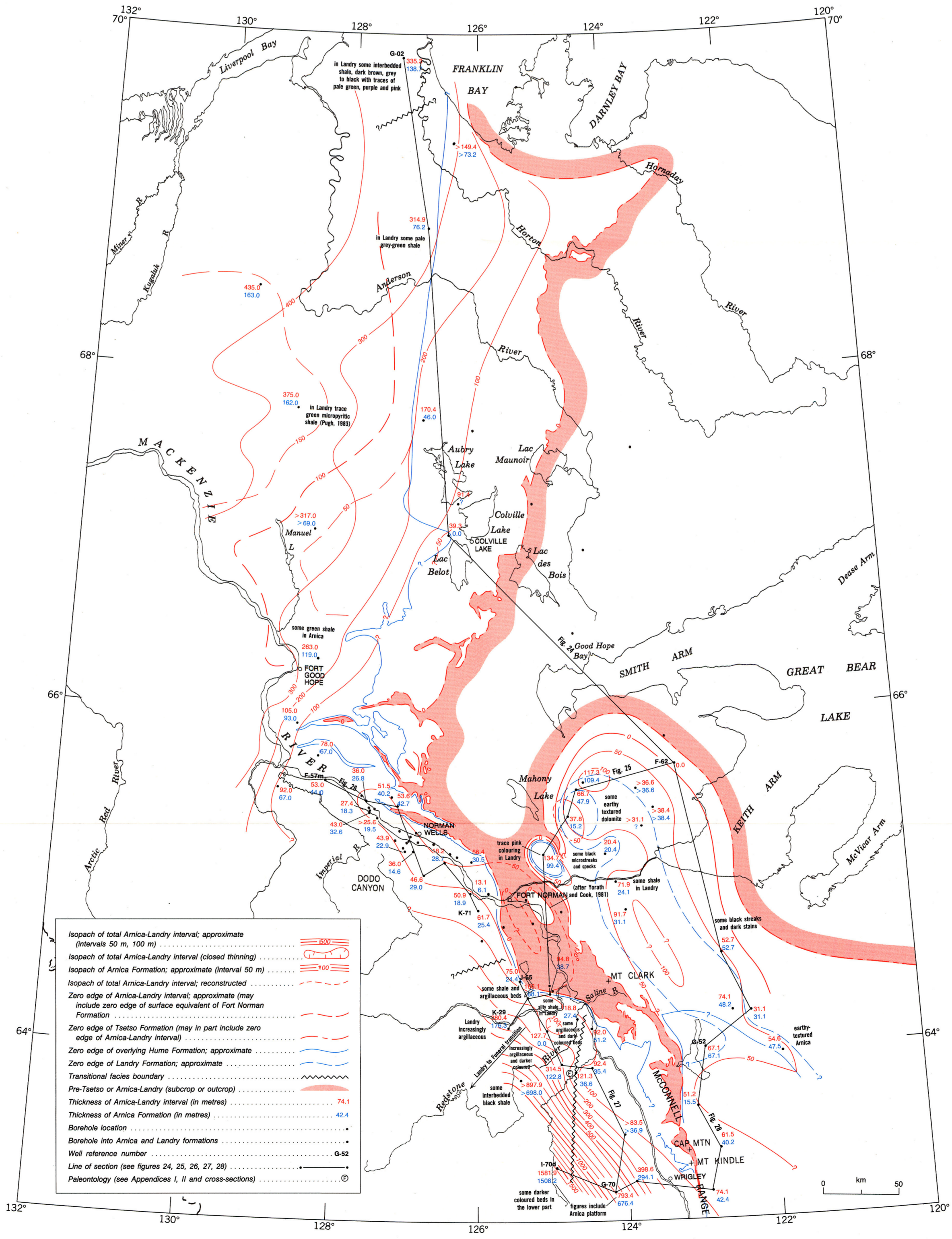
Figure 12. Isopach and lithofacies map of Arica and Landry formations
