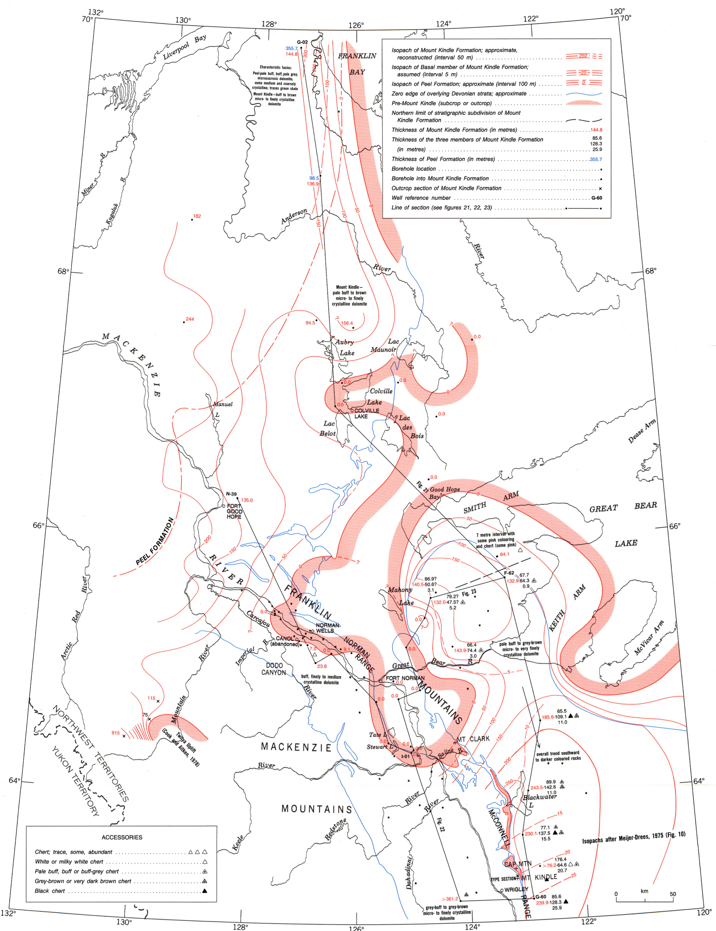
Figure 8. Isopach and lithofacies map of Mount Kindle and Peel formations
