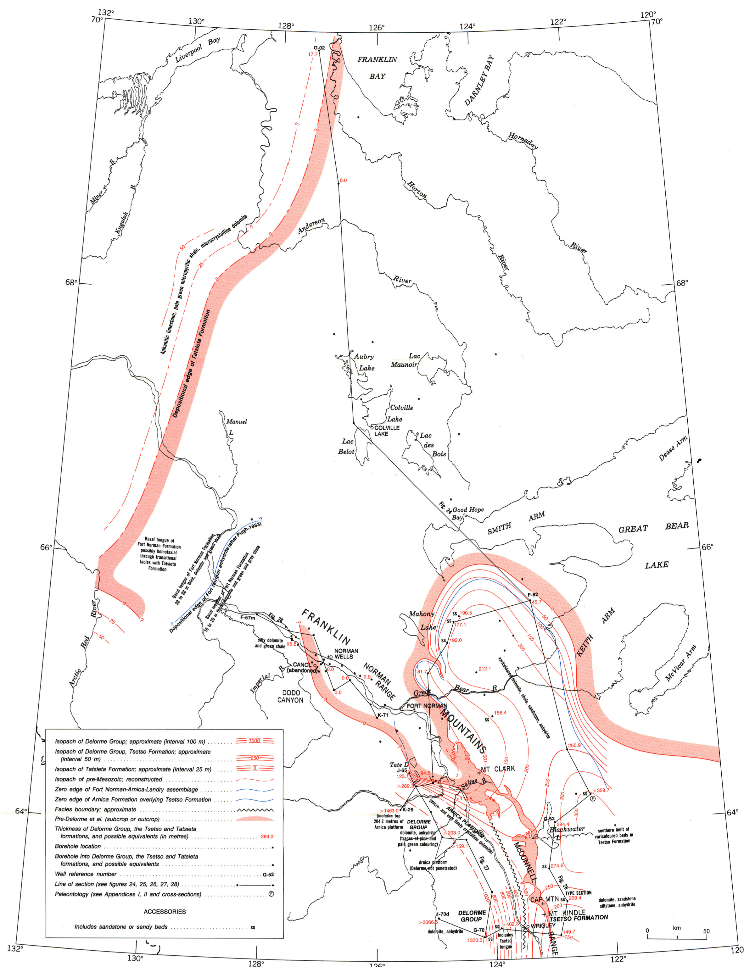
Figure 10. Isopach and lithofacies map of the Delorme Group, Tsetso and Tatsieta formations, and possible equivalents
