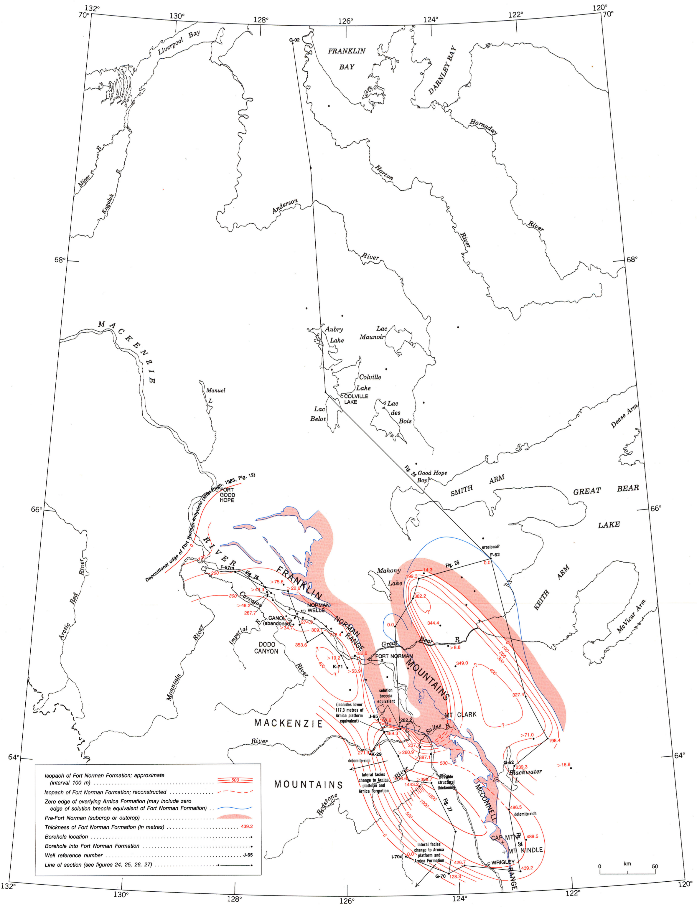
Figure 11. Isopach and lithofacies map of Fort Norman Formation
