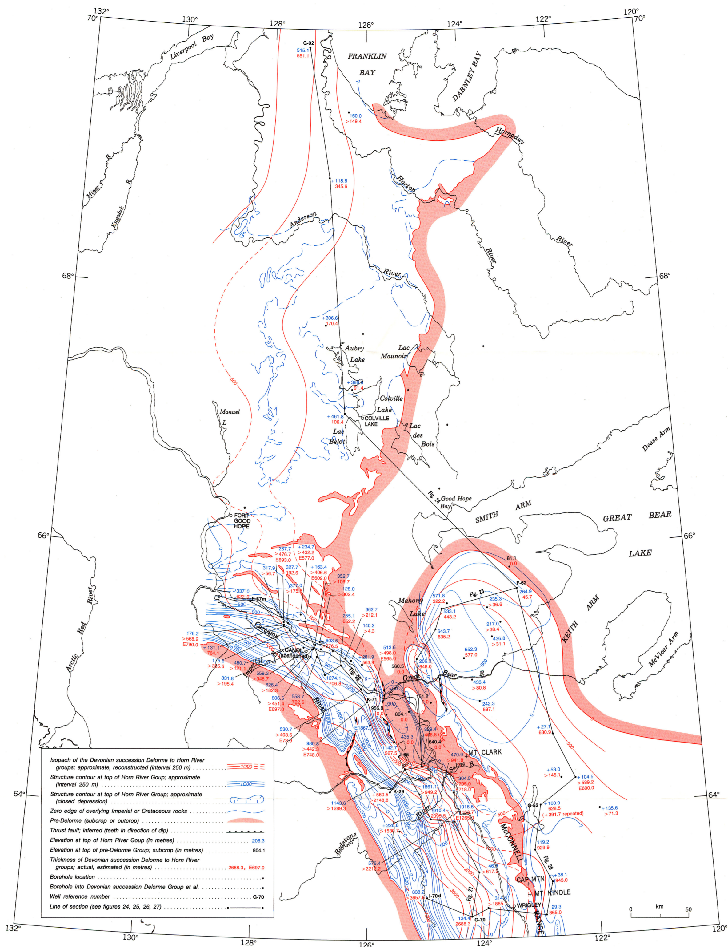
Figure 9. Isopach and structure contour map of the Devonian succession: Delorme Group to Horn River Group
