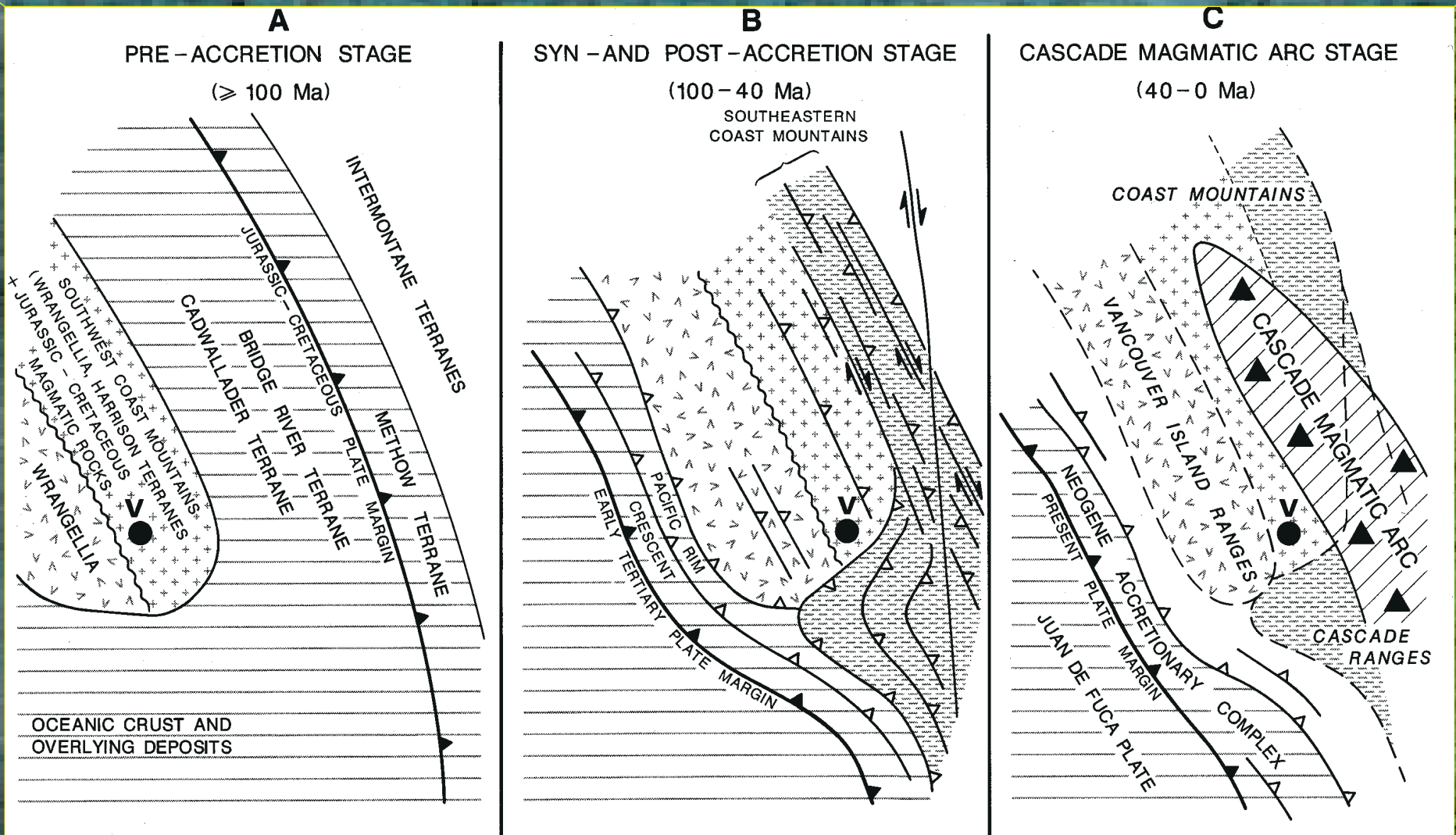
Figure 12: Summary tectonic evolution of southwestern British Columbia. Location of city of Vancouver shown by V. No attempt is made at palinspastic restoration, other than the schematic gap east of the southwestern Coast Mountains- Wrangellian block (= Insular Superterrane) in A ; Orogen parallel displacements may have been large and sinistral before 100 Ma, and dextral after that time (Monger, et. al., 1994; Monger and Journeay, 1994).
