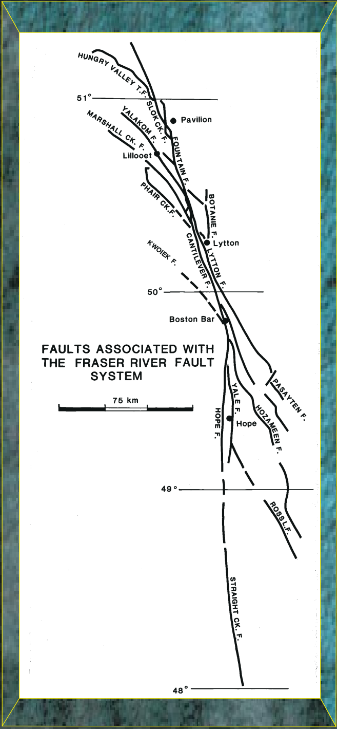
Figure 17: Some faults associated with the Fraser-Straight Creek fault system.
