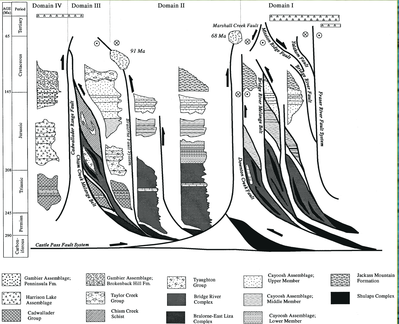
Figure 21: Structural and stratigraphic framework of the eastern Coast belt. Regional correlations and terrane descriptions of these rock units are summarized in Figures 6, 8 and Table 1, respectively.
