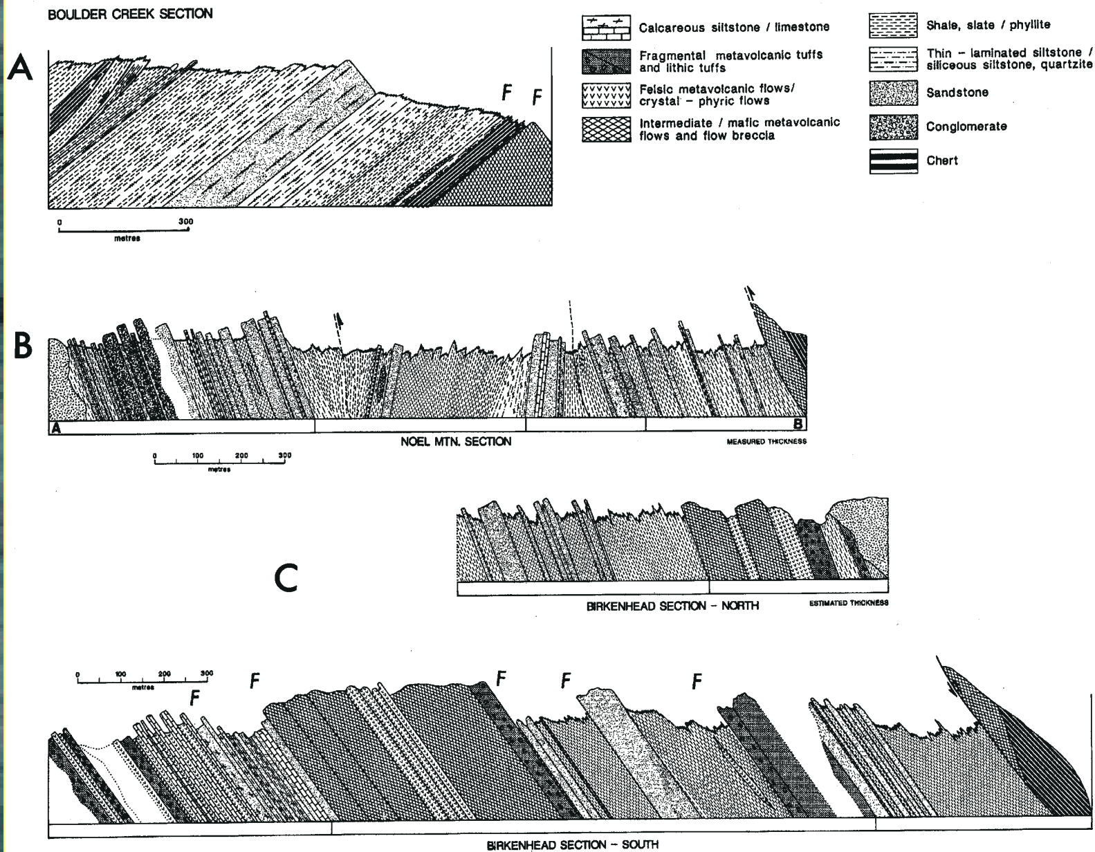
Figure 22: Measured structural-stratigraphic sections of clastic successions overlying Bridge River and Cadwallader terranes in the southeastern Coast belt. Sections are keyed to Figure 20 , and include the Bridge River/ Cayoosh transition along Boulder creek ( Fig 22A ), middle and upper successions of the Cayoosh Assemblage on Noel Mountain ( Fig22B ), and Cadwallader Group/ Harrison Lake Formation/ Cayoosh Assemblage relationships in the Birkenhead Lake region ( Fig22C ).
