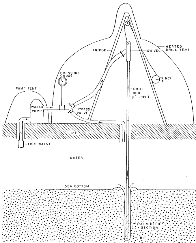
Figure 17.2. Diagrammatic representation of drilling technique.
