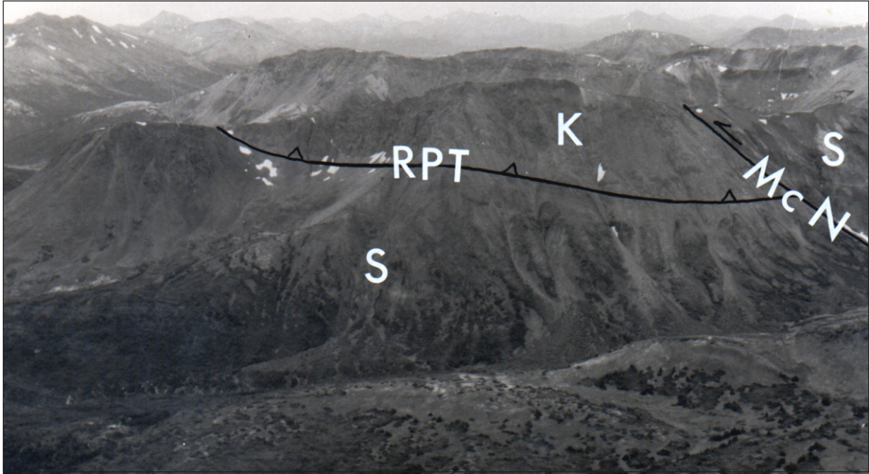
Figure 61. View south-southeast from the ridge east of upper Starr Creek where the McNeil fault (McN) cuts the Ragged Peak thrust (RPT). The Ragged Peak thrust has similar relations to the Porcupine thrust. Here it brings volcanic rocks of the Cloutier formation (K) above intermediate volcanics and black slate of the Seagull group (S). The McNeil thrust (McN) offsets the Ragged Peak thrust. The view is oblique to regional strike, and strata dip to the right.
