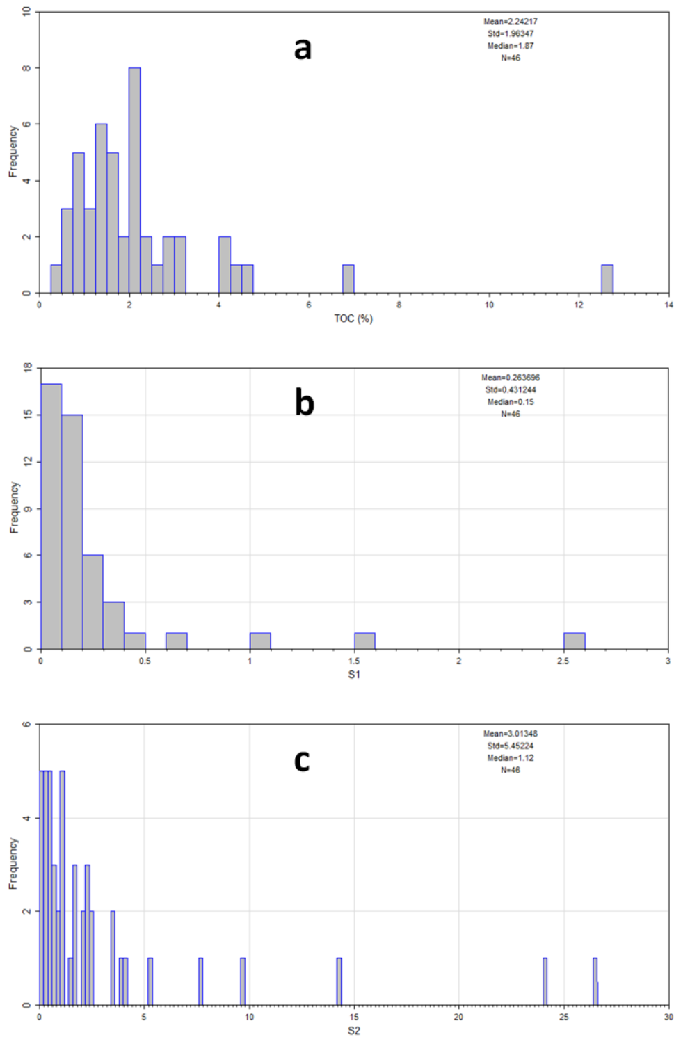
Figure 6. Organic richness as shown by (a) TOC content, (b) S1; and (c) S2 values from Rock-Eval analysis of Cretaceous potential source rock samples from Beaufort-Mackenzie Basin
