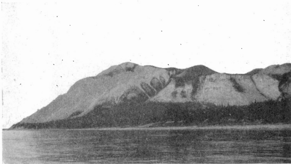
Bear Rock at the junction of Great Bear and Mackenzie Rivers at Fort Norman.
