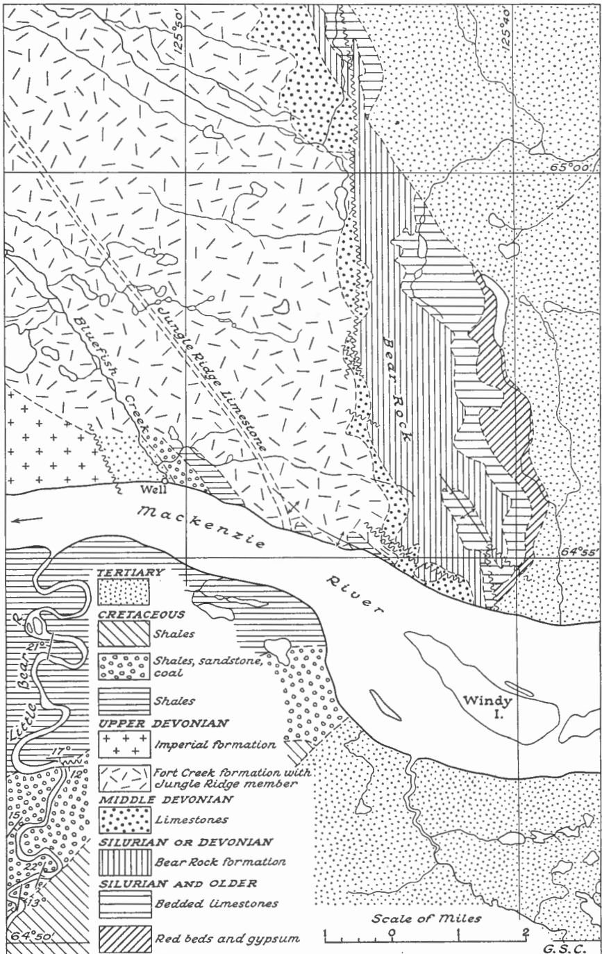
Figure 2. Bear Rock and vicinity.
