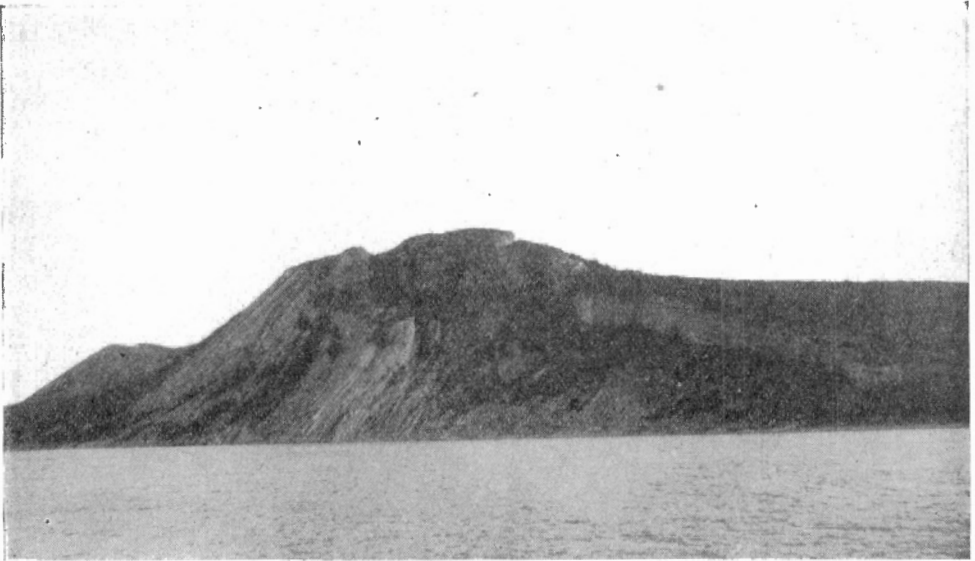
Rock-by-the-River's Side, near Wrigley, showing folding in Middle Devonian rocks.
