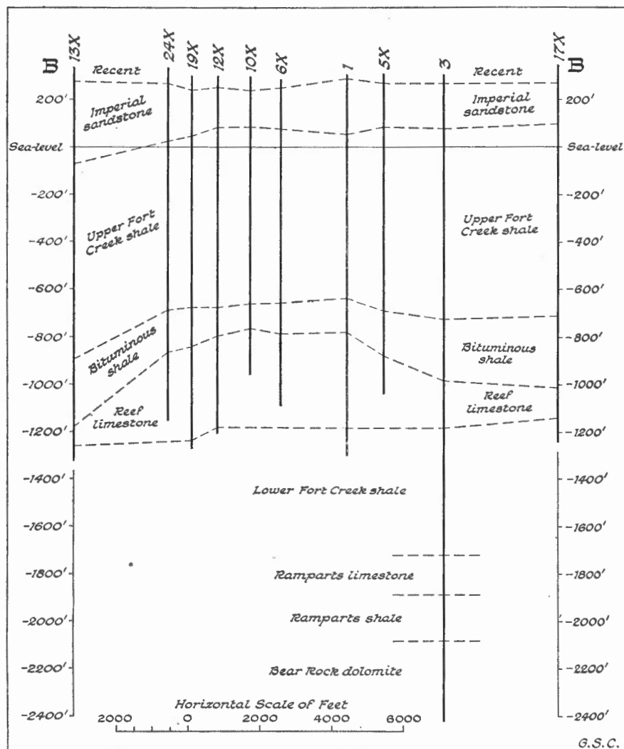
Figure 16. Cross-section B-B, Norman Wells field.
