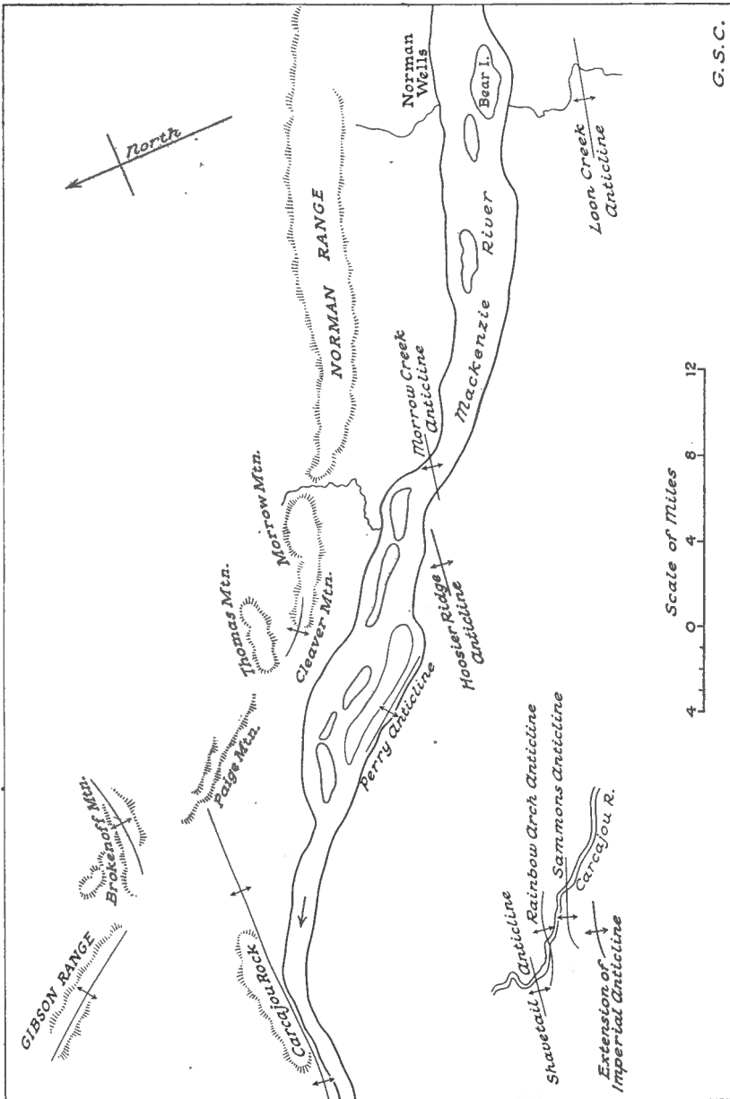
Figure 3. Structural trends, Norman Wells area.
