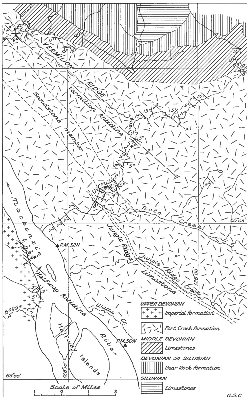
Figure 4. Vermilion and Halfway anticlines.
