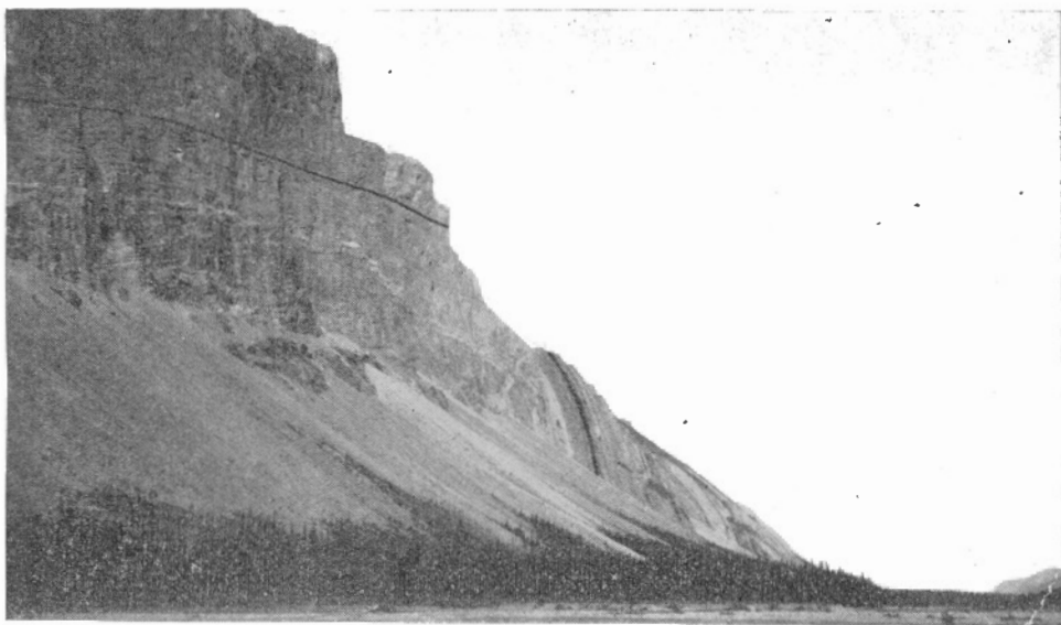
Folded Middle Devonian rocks on North Nahanni River, a few miles west of Mackenzie River.
