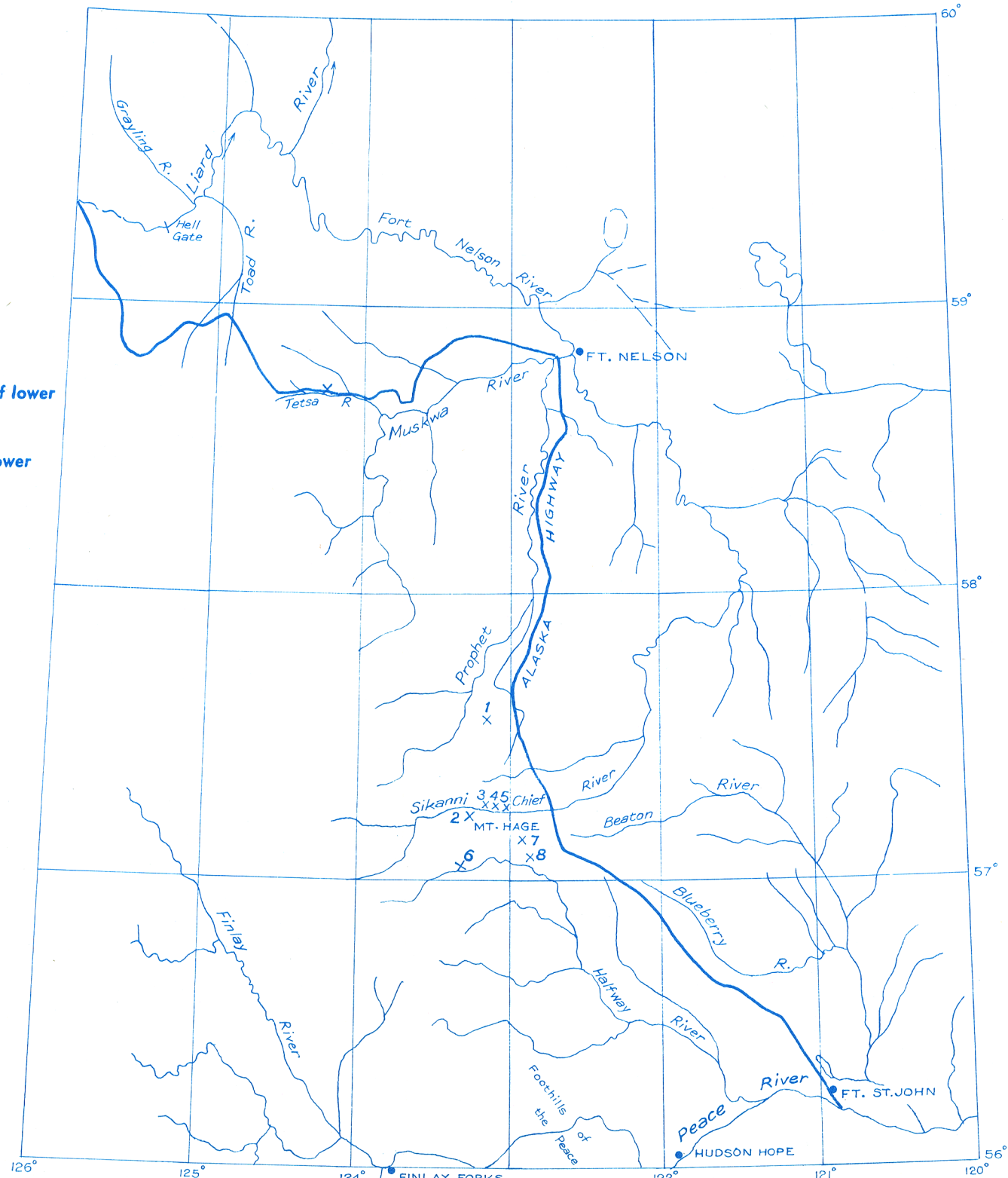
FIGURE 1A: INDEX MAP OF NORTHEASTERN BRITISH COLUMBIA SHOWING GEOGRAPHIC FEATURES AND TRIASSIC FOSSIL LOCALITIES REFERRED TO IN THIS REPORT
