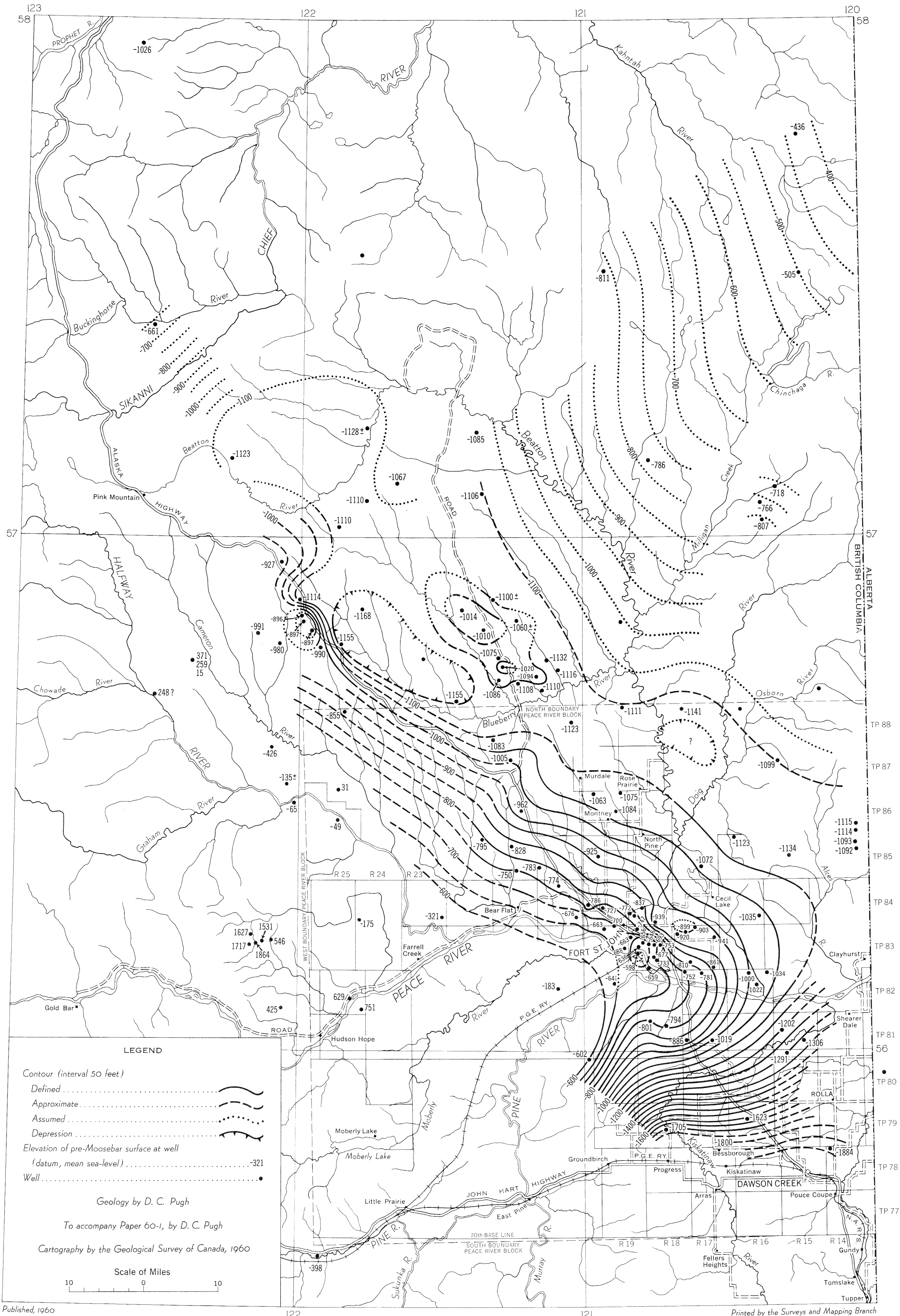
Figure 4. Map of Fort St. John area, Peace River District, British Columbia, showing structure contours on the pre-Moosebar surface
