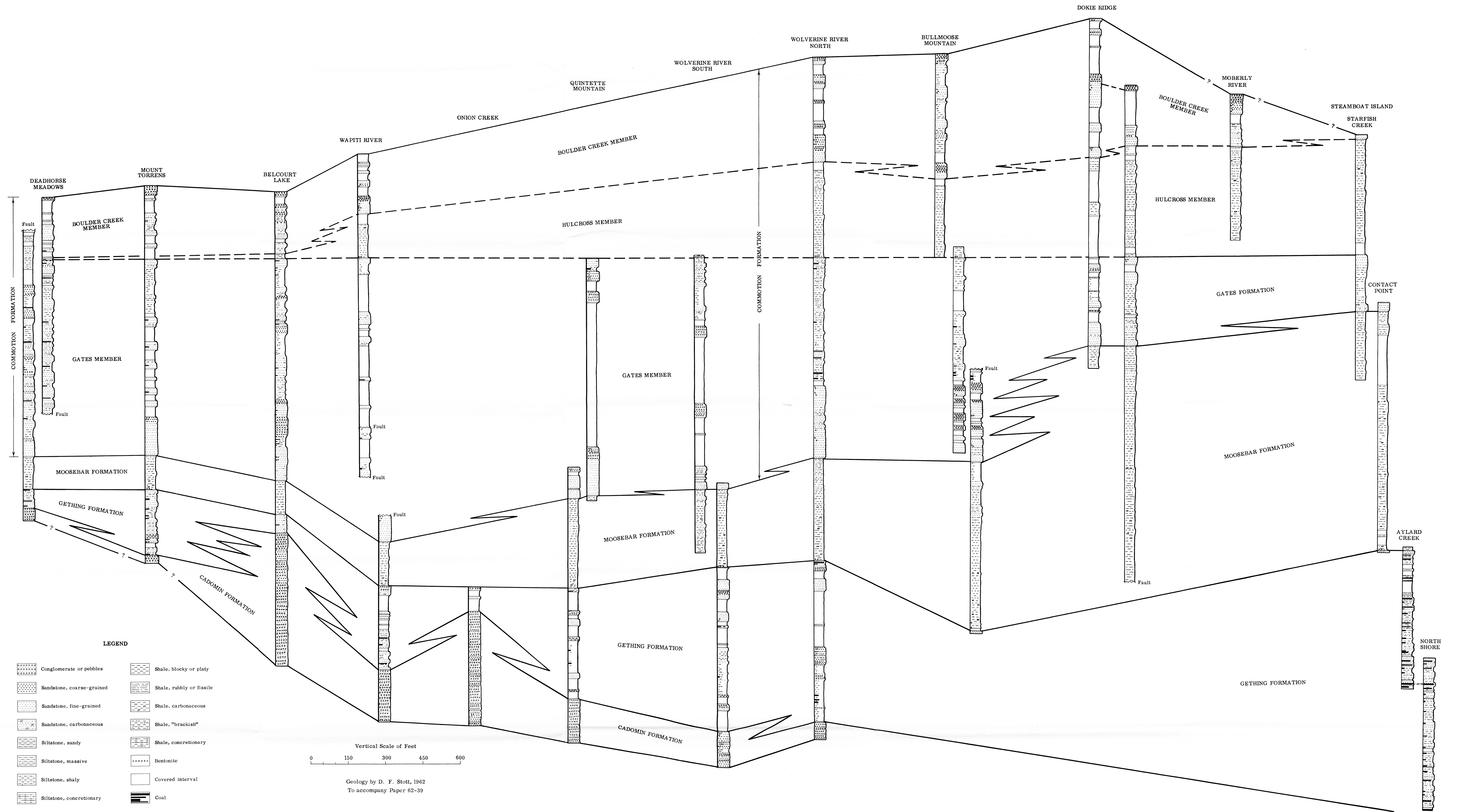
Figure 5. Columnar sections of Cadomin, Gething, Moosebar and Commotion Formations showing variations in lithologies, facies and thicknesses, northern British Columbia and northwestern Alberta
