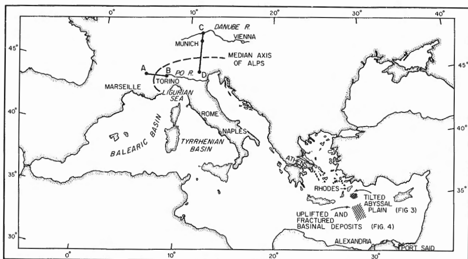
Figure 1. The Alps and Mediterranean Sea, showing locations of sections of Figures 2a and 2b, and of reflection profiles of Figures 3 and 4.
