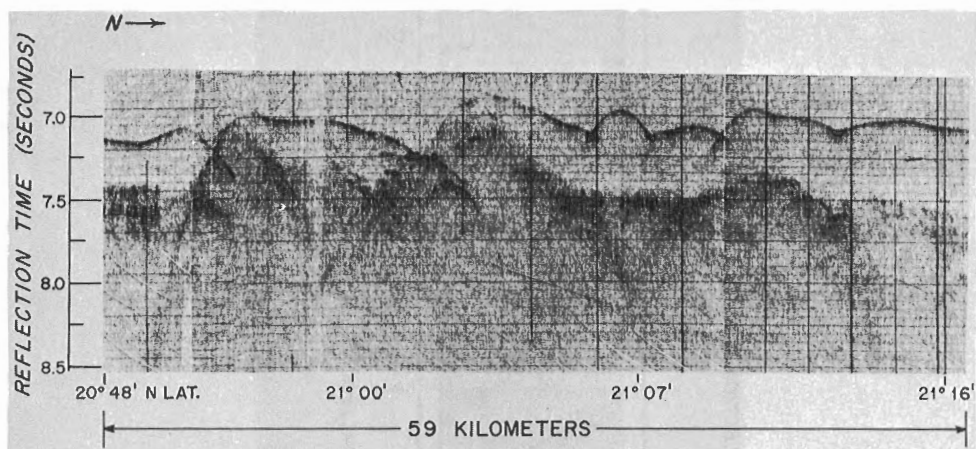
Figure 8. The transparent layer on the outer ridge as recorded along a north-south section along longitude 65^{\circ}12'W . Note the apparent lack of correlation between the sea-floor relief and that of the underlying surface. (After Bunce and Hersey, 1966)
