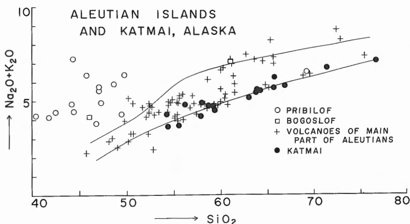
Figure 8. Total alkalies-SiO 2 relation in rocks of Quaternary volcanoes in the Aleutian Islands and southwestern Alaska.
