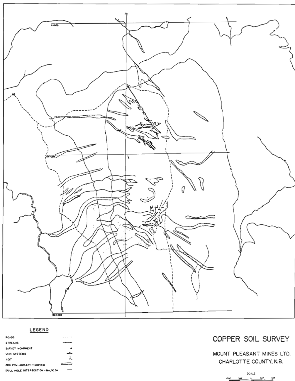
Figure 3. Distribution of copper in soil, Mount Pleasant Mines Ltd., Charlotte County, N.B.
