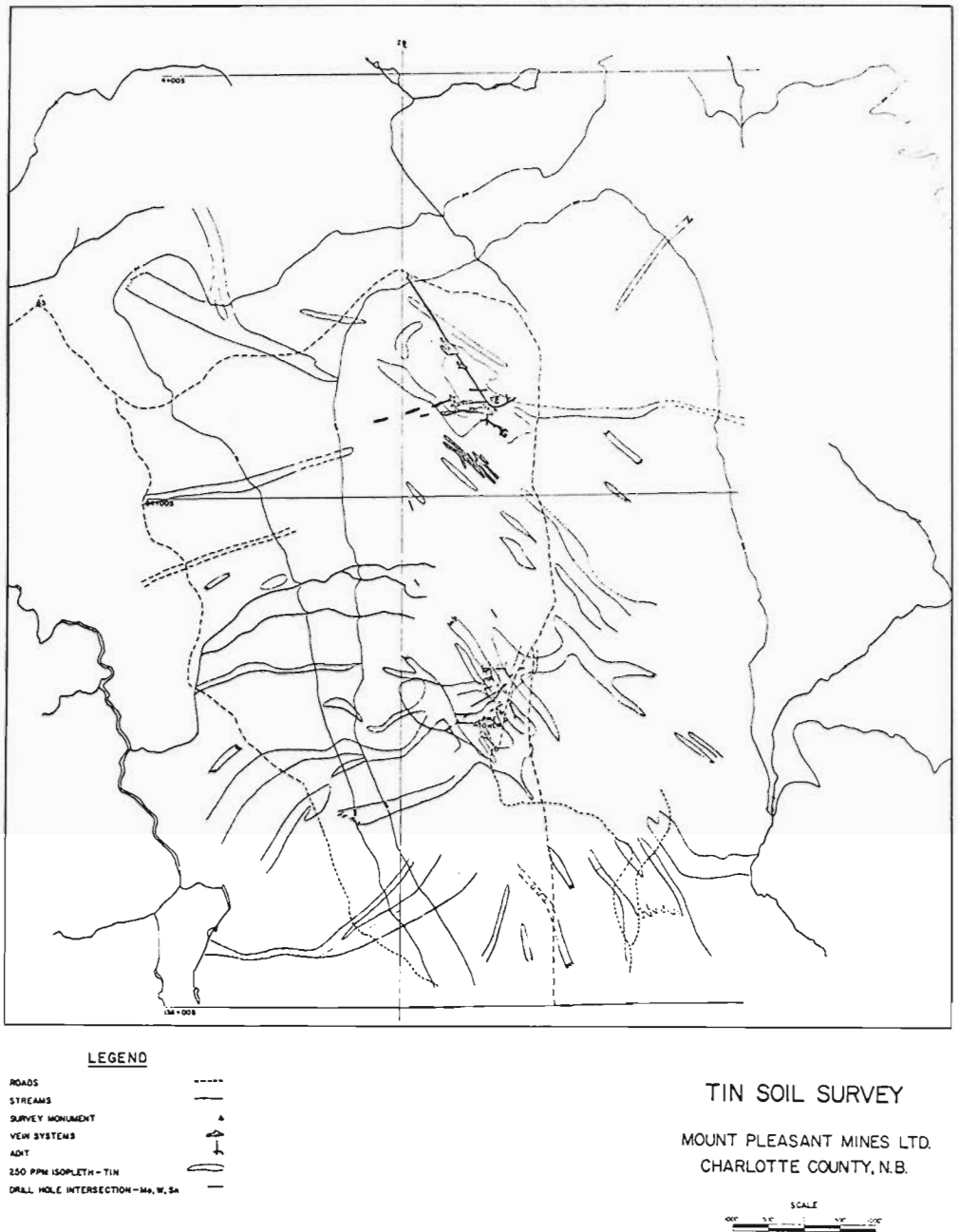
Figure 1. Distribution of tin in soil, Mount Pleasant Mines Ltd., Charlotte County, N. B.
