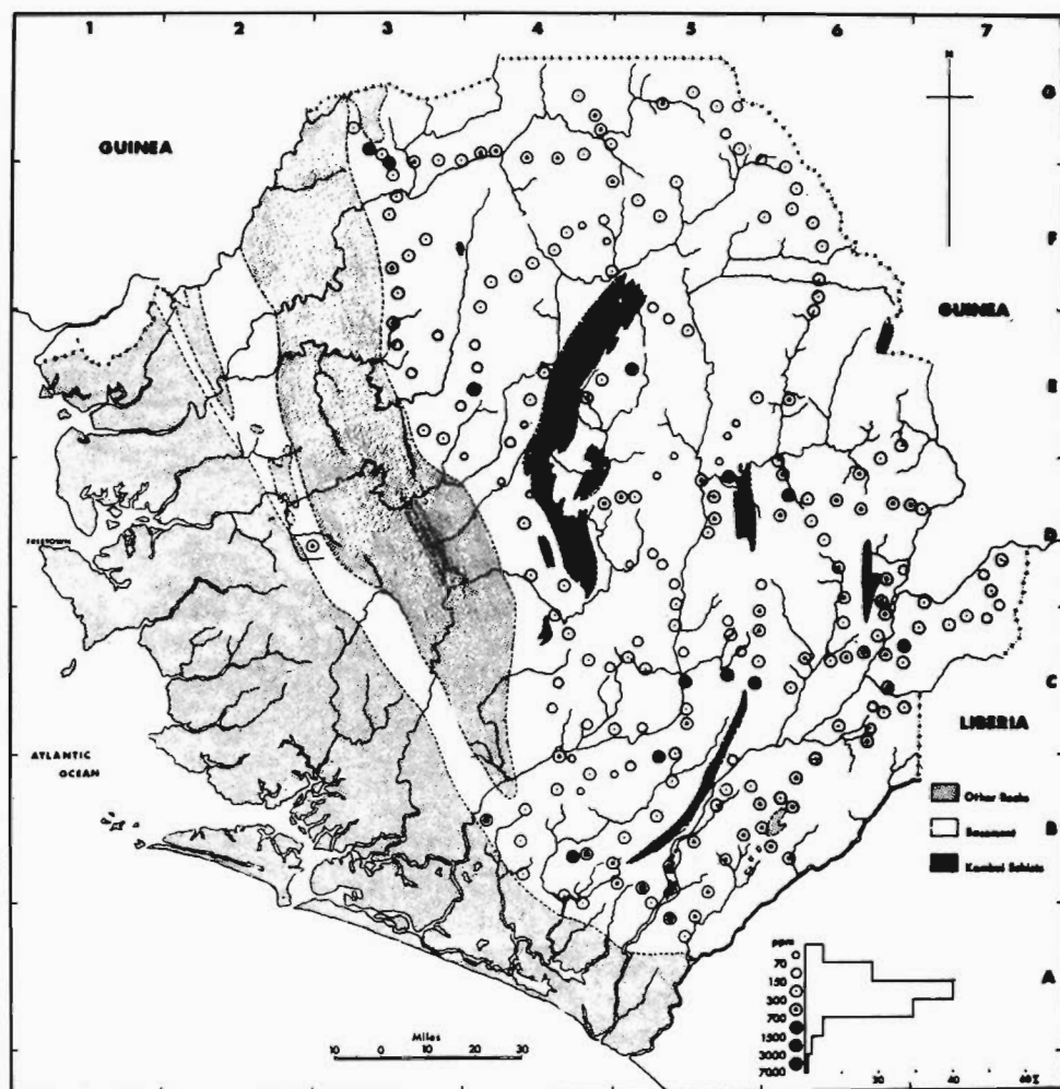
Figure 7. Ni content, ppm, in -80 mesh fractions, of stream sediment over Basement Complex.
