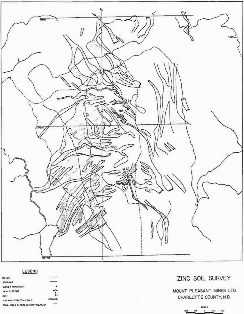
Figure 2. Distribution of zinc in soil, Mount Pleasant Mines Ltd., Charlotte County, N. B.
