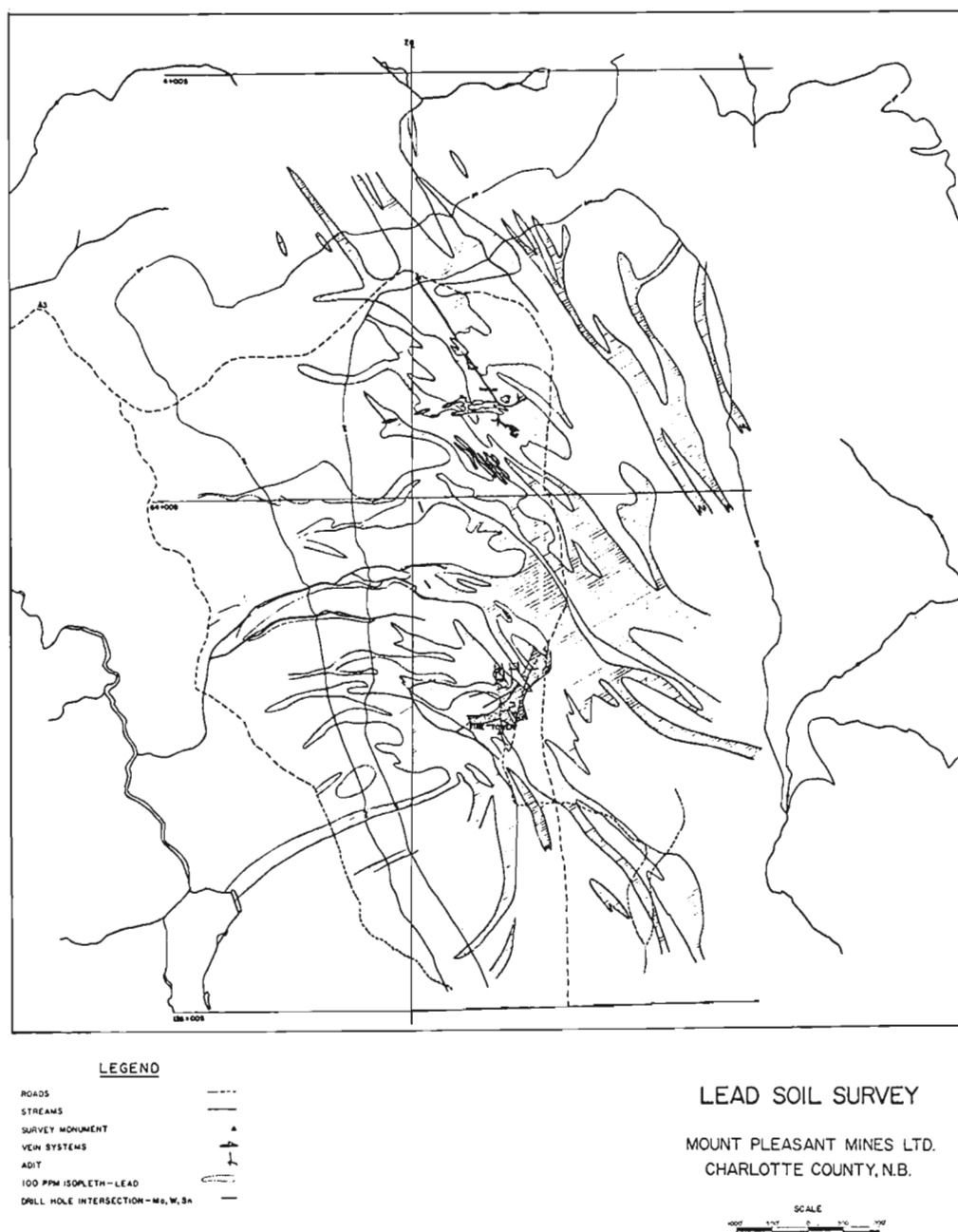
Figure 5. Distribution of lead in soil, Mount Pleasant Mines Ltd., Charlotte County, N. B.
