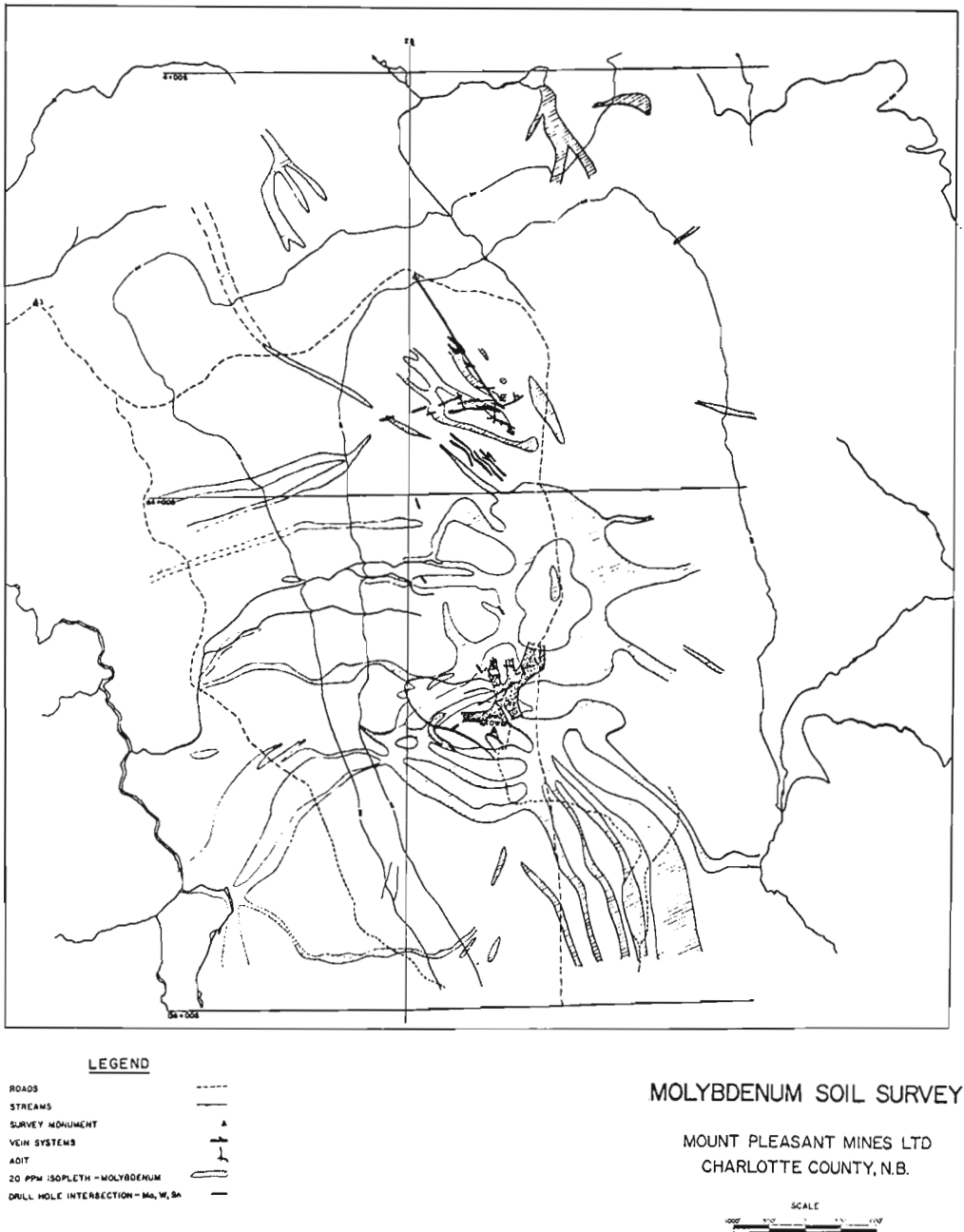
Figure 4. Distribution of molybdenum in soil, Mount Pleasant Mines Ltd., Charlotte County, N. B.
