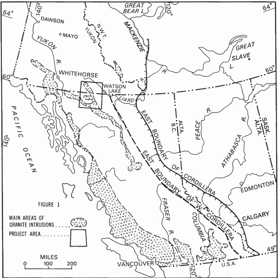
Figure 1. Regional geology
