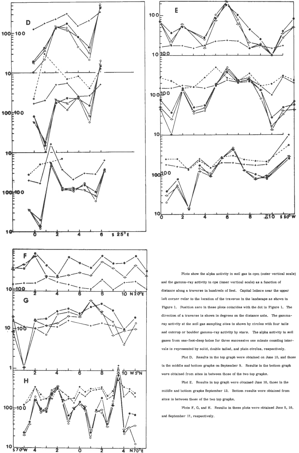
Figure 3. Radioactive emanations from soils in the Gataueau Hills.
