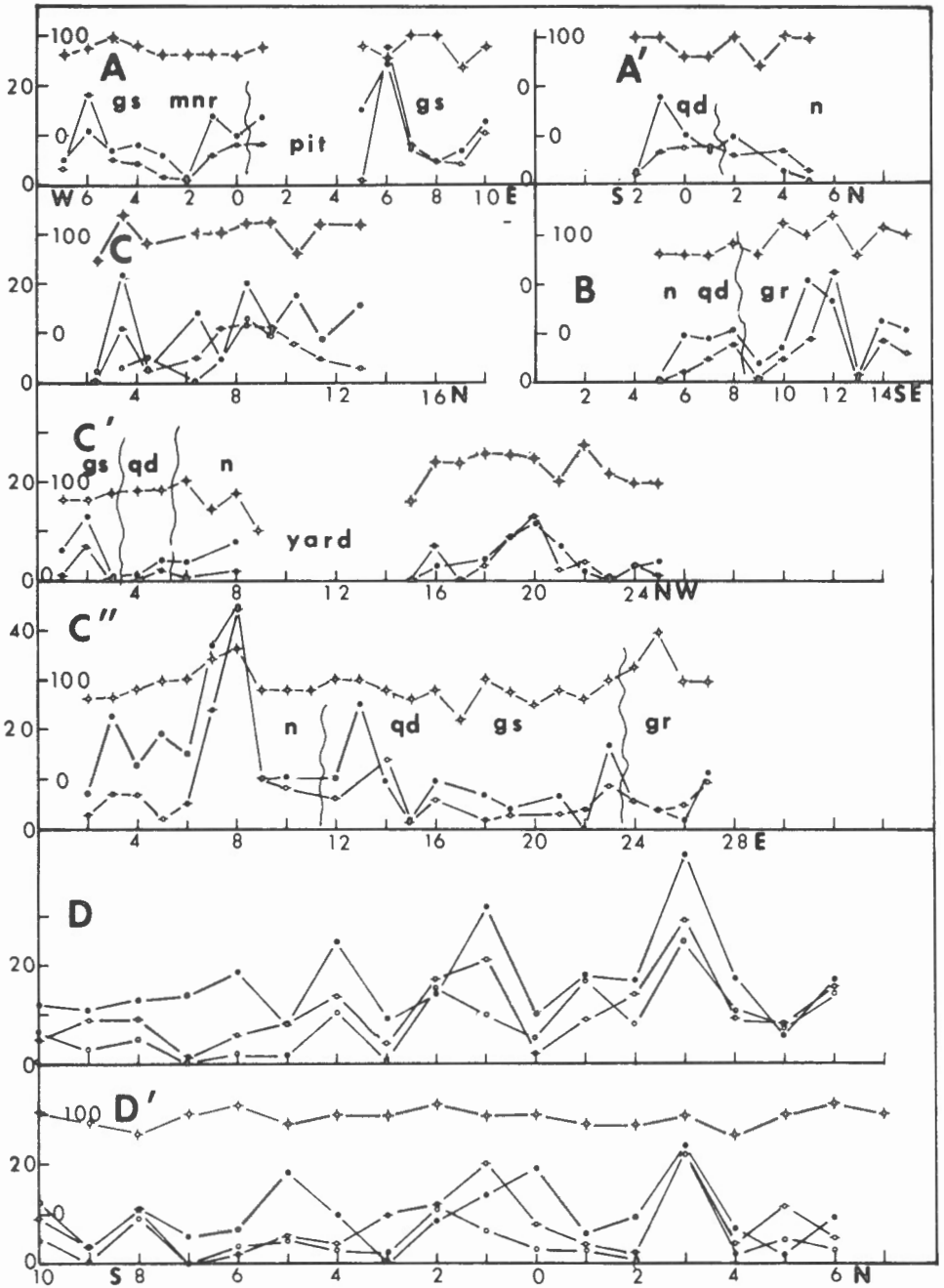
Figure 6. Radioactive emanations from soil in the Sudbury area.
