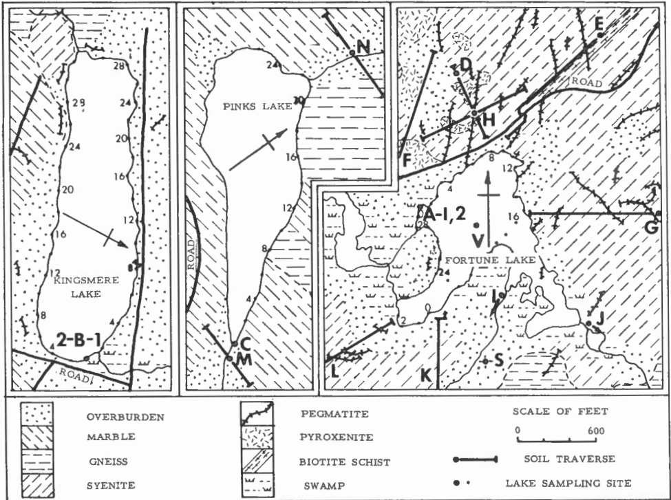
Figure 1. Geology and radon sampling sites in the Gatineau Hills. Water sampling sites are shown by solid dots on the shores. Large dots indicate starting or zero position. Numbers along lake shores indicate distance from zero position in hundreds of feet. The location and direction of soil traverses are shown by heavy straight lines, except for the traverses around the shores of Kingsmere and Fortune lakes. These two coincide with the water sampling sites. Solid circles denote zero or starting position of a soil traverse. Capital letters near the zero position refer to the graphs in Figures 2, 3 and 4.
