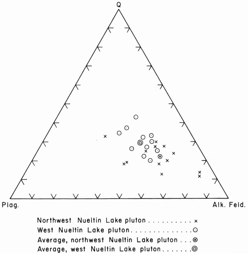
Figure 3. Modal compositions of leucocratic components of two plutons of Nueltin Lake granite. GSC
