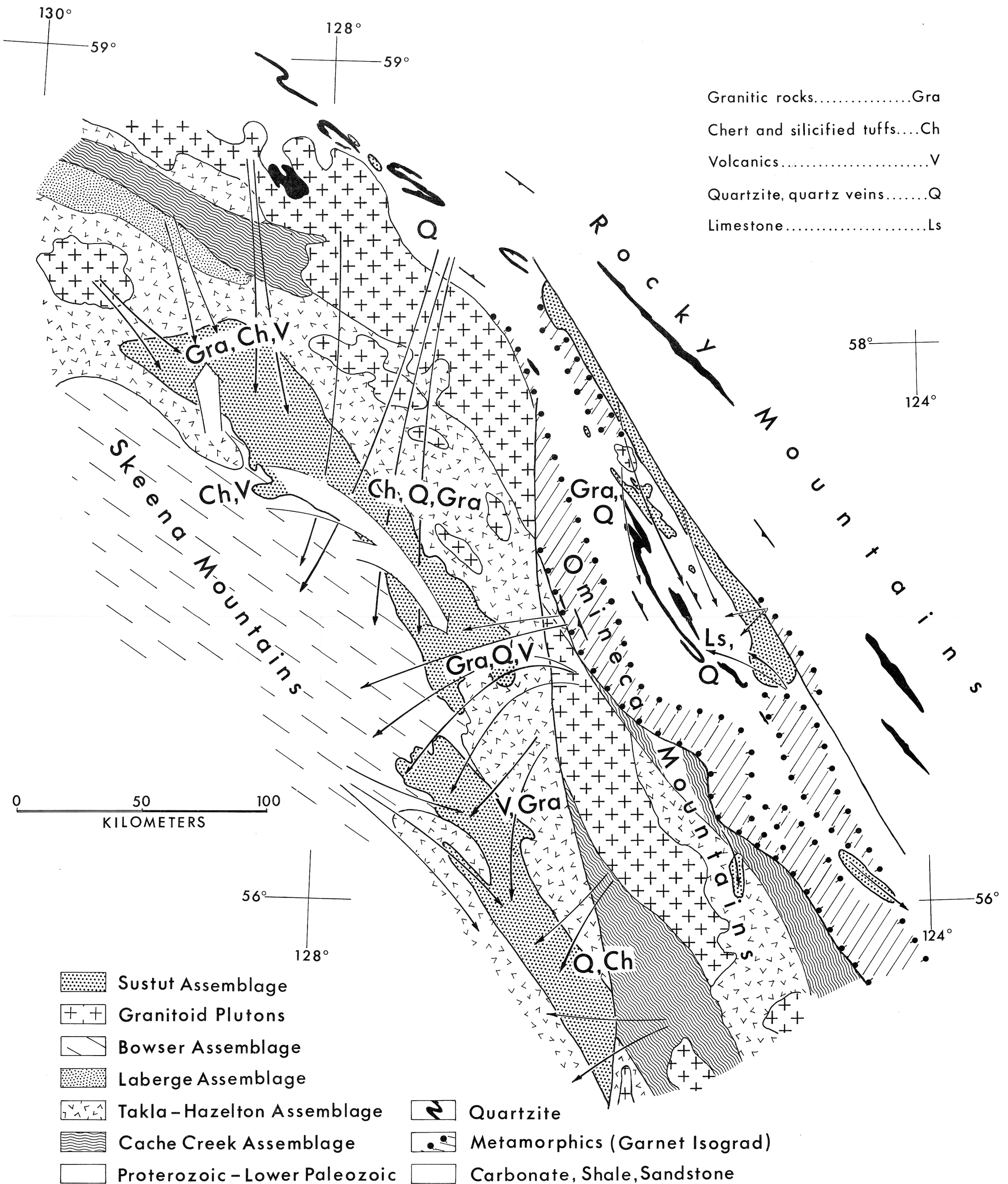
Figure 4. Generalized distribution of the principal lithological units within the inferred source area of the Sustut and Sifton basins, British Columbia
