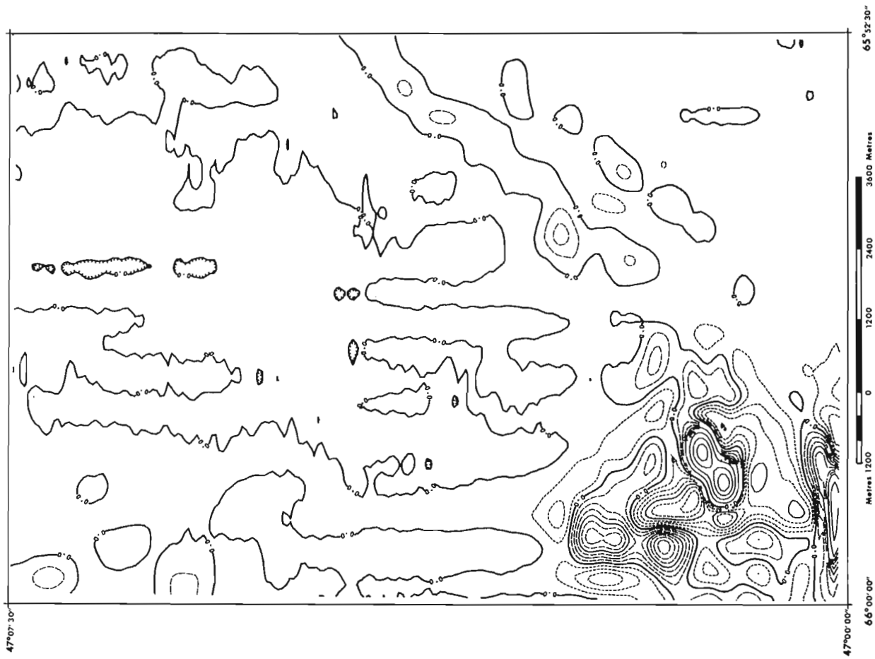
Figure 3.3. First vertical derivative map of Figure 3.1.
