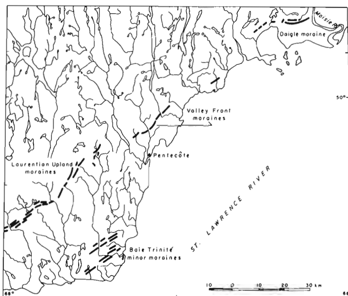
Figure 34.1. Principal moraines along the Quebec North Shore, Godbout — Sept-Iles area.
