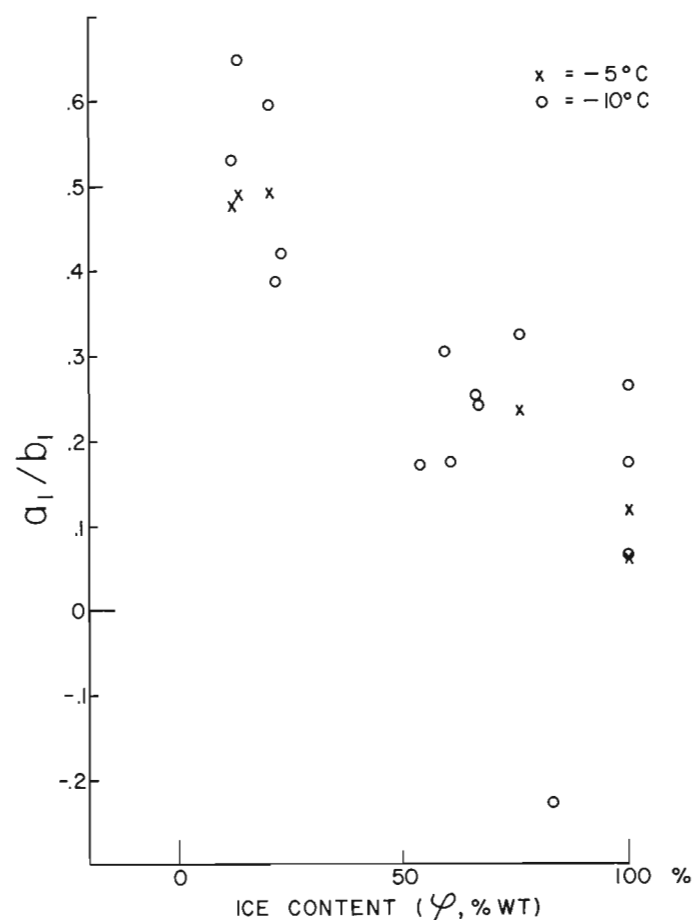
Figure 19.11. a_1/b_1 vs. ice content ( \phi ).
