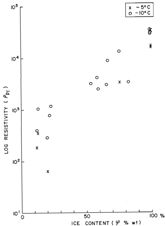
Figure 19.9. \rho_{p1} vs. ice content ( \phi ).
