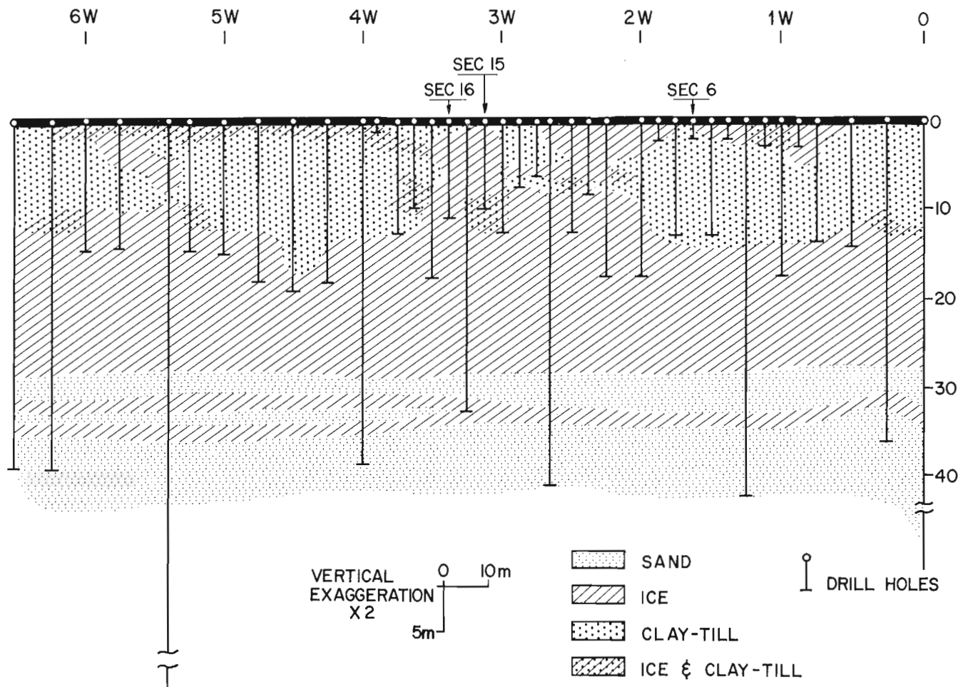
Figure 20.2. Geological cross section of the "Involut Hill" between 0 and 6 W on the base line as inferred from the drilling results. Position numbers are given in units of hundreds of feet.
