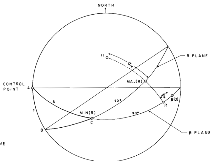
Figure 32.4. Orientation of the reference line by spherical trigonometry.
