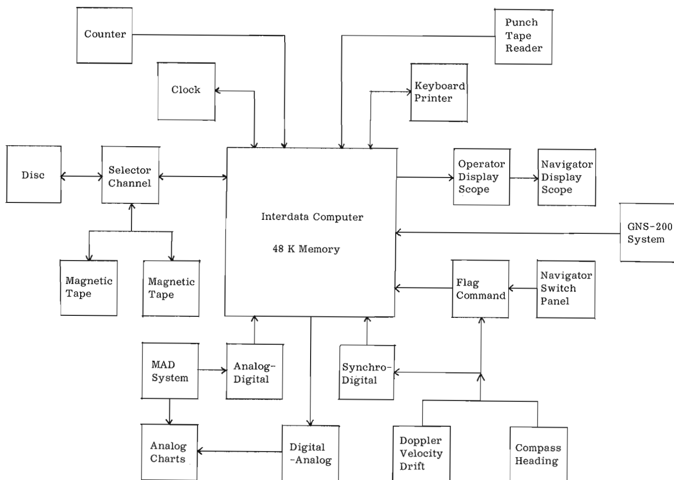
Figure 18.1. North Star Computer System.
