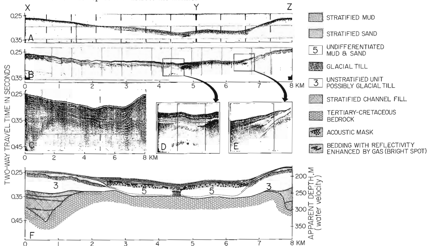
Figure 2.2. Seismic data along Profile XYZ (Fig. 2.1). (A) echogram; (B) Huntic deep tow high-resolution seismic reflection profile, DTS; (C) air gun seismic profile; (D) and (E) enlarged areas of DTS profile (B); (F) composite stratigraphic interpretation using (B) and (C) above. See text for interpretation.
