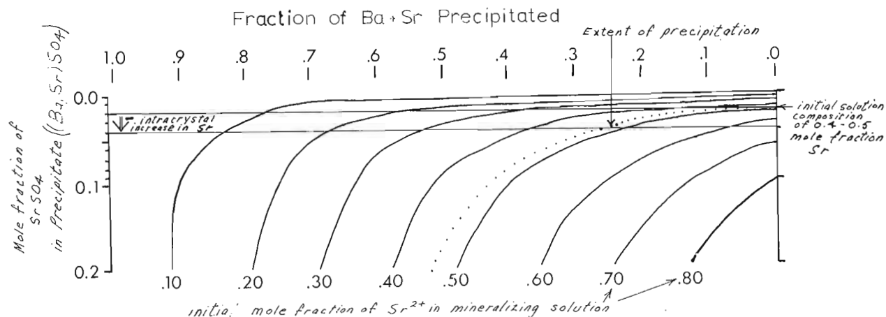
Figure 38. 8. Composition of the last-formed precipitate of (\text{Ba}, \text{Sr}) \text{SO}_4 as a function of the mole fraction of Ba plus Sr precipitated out of solution for a series of initial mineralizing solution compositions. Initial solution compositions are given as the mole fraction of Sr with respect to total Ba + Sr in solution. Two horizontal lines define the amount and variation of \text{SrSO}_4 within barite crystals from Sulphur Creek and the extent of precipitation of Ba + Sr from solution. Adapted from Hanor (1968, p. 1219).
