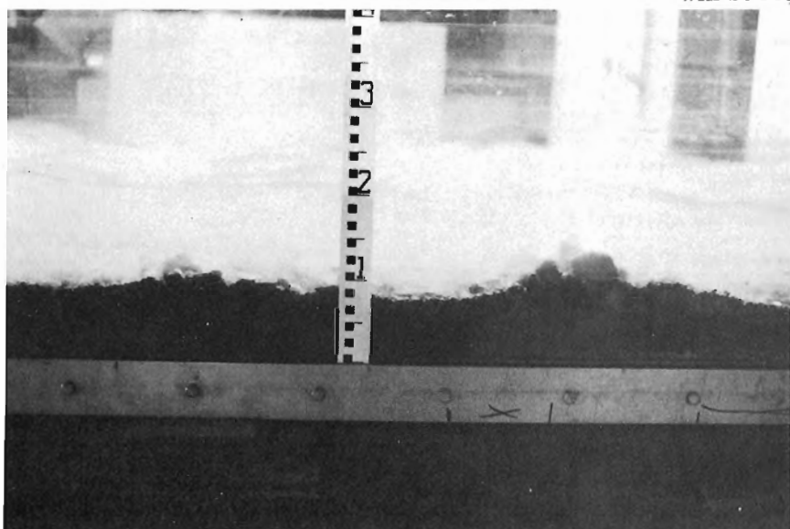
Figure 53. 9. Example of a degrading antidune during test 4 (photograph courtesy of R.J. Gale).
