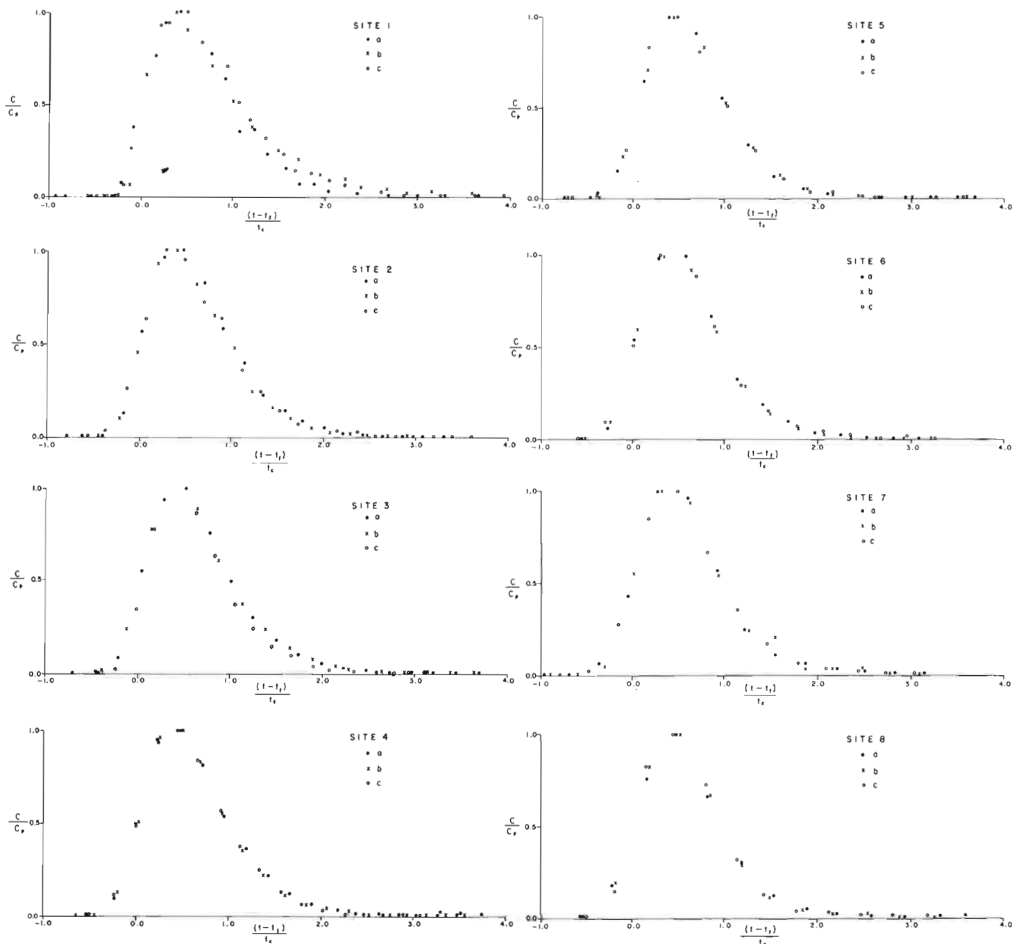
Figure 56.12. Dimensionless time-concentration curves for the eight sampling sites of Lesser Slave River.
