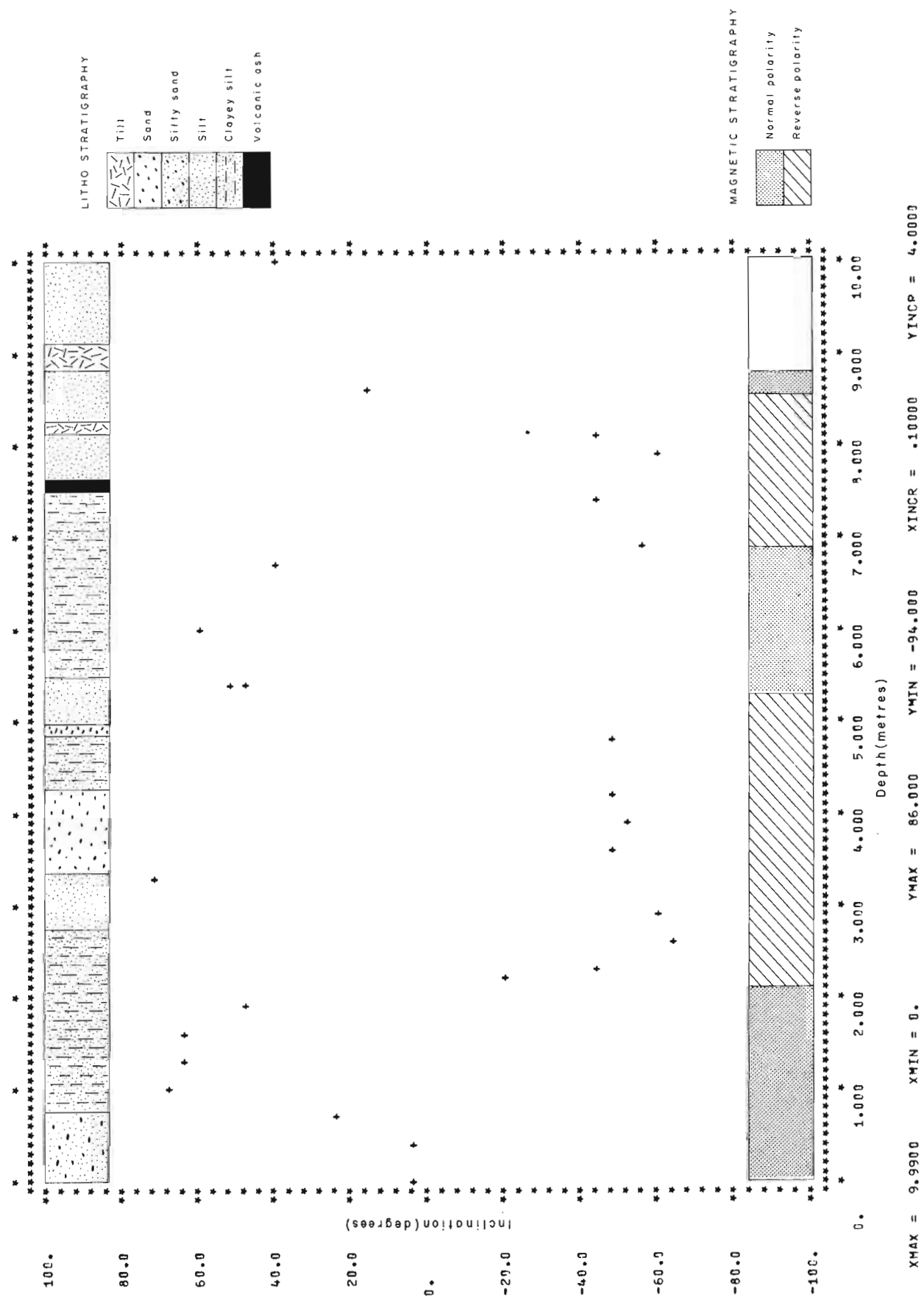
Figure 37.1. Plot of inclination of the remanent magnetism of Wellsch Valley sediments.
