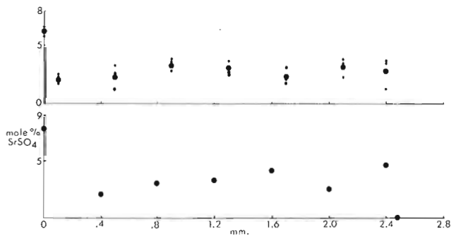
Figure 38.7. Plots of strontium content along the growth direction of blades of space-filling barite from the sample shown in Figure 38.4. The first \text{SrSO}_4 determination in each traverse is on the barite crust adjacent to the dolomite wall rock. The last \text{SrSO}_4 determination is from the central calcite fill.
