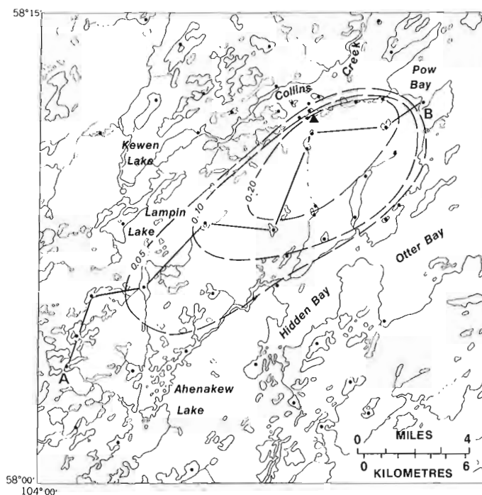
Figure 44.4. Uranium in lake waters, as parts per billion, Rabbit Lake area, Saskatchewan.
