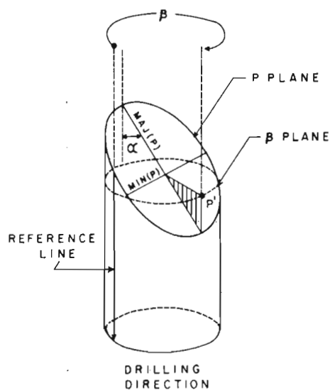
Figure 32.1. Angles \alpha and \beta and the reference line.
