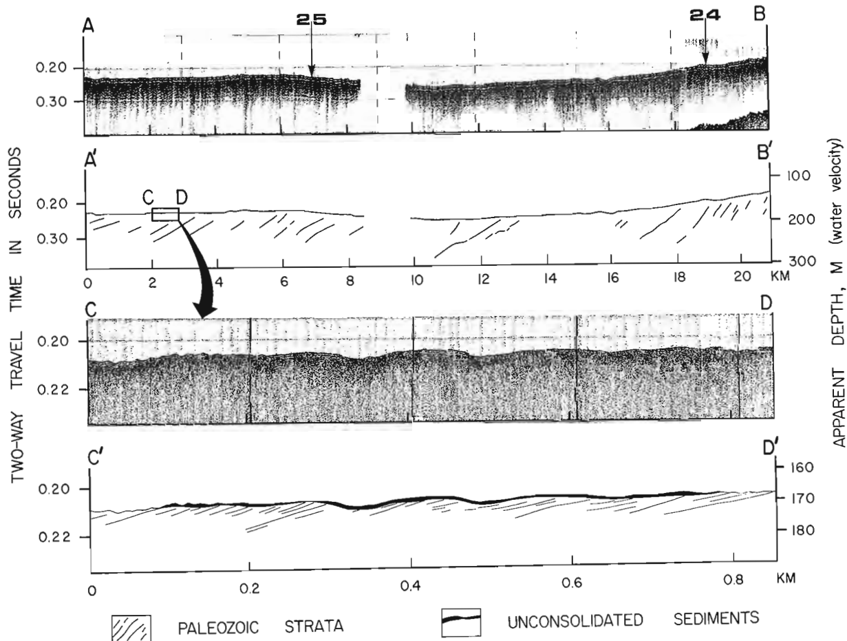
Figure 2.3. Seismic data along Profile AB (Fig. 2.1). (AB) air gun seismic reflection profile; (A'B') line interpretation of seismic reflection profile; (CD) Hunttec deep tow high-resolution seismic profile, DTS; (C'D') line interpretation of DTS profile. CD on Profile A'B' represents area shown by DTS Profile CD. Some of the detail on the DTS profile has been lost through reduction and reproduction.
