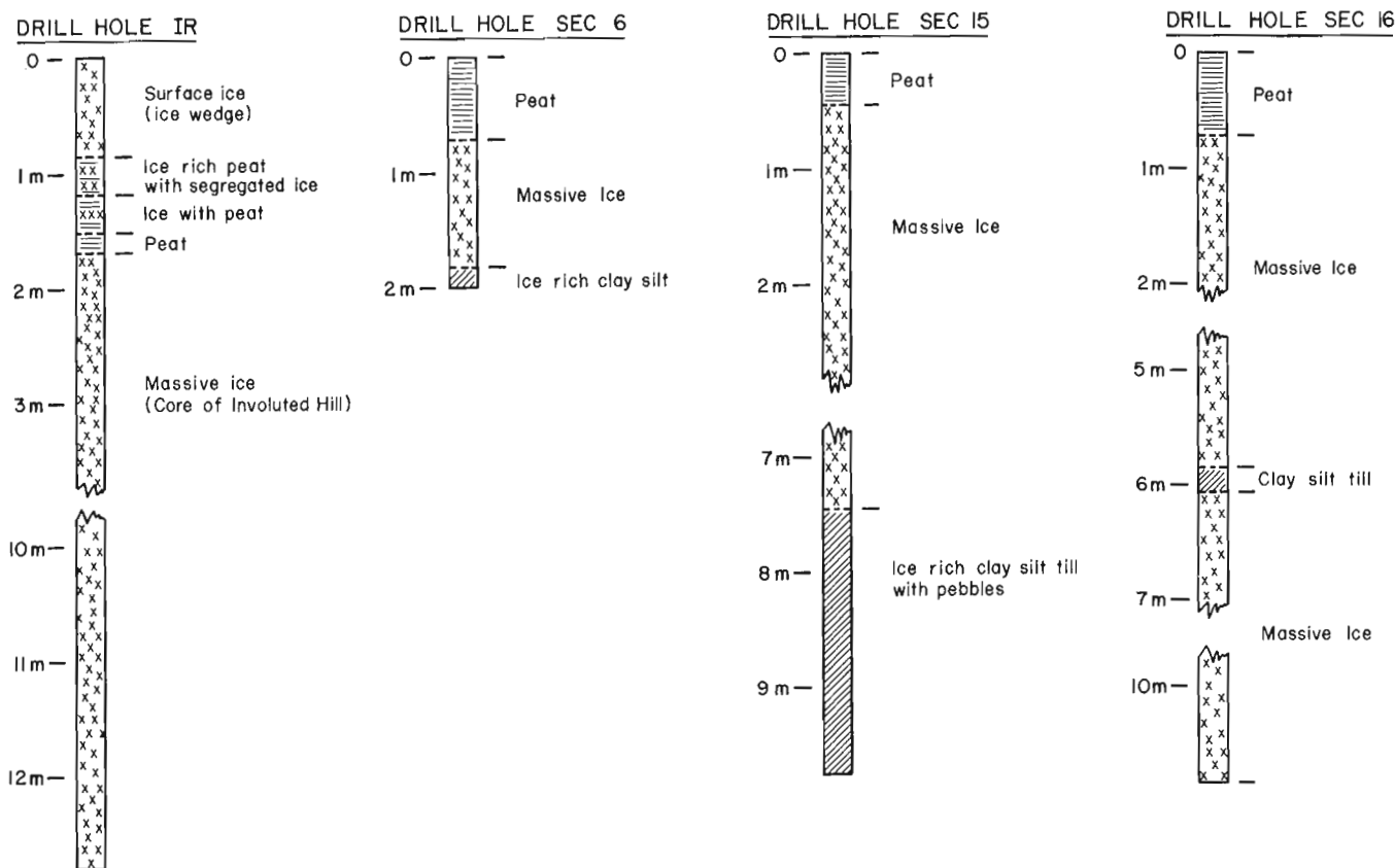
Figure 20.3. Drill logs for holes IR, SEC 6, SEC 15 and SEC 16.
