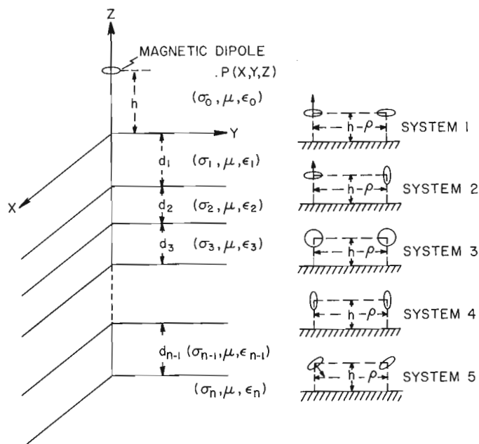
Figure 12.1. Magnetic dipole source over an n-layer earth and the five coil configurations.
