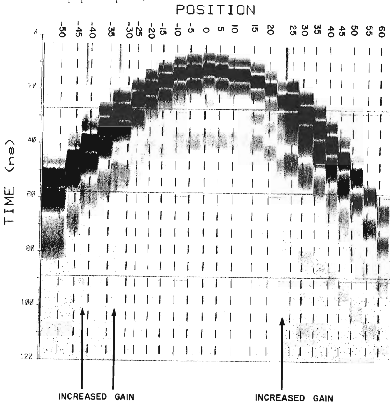
Figure 18.2 Typical transillumination record obtained in a potash mine. The position is indicated in feet.
