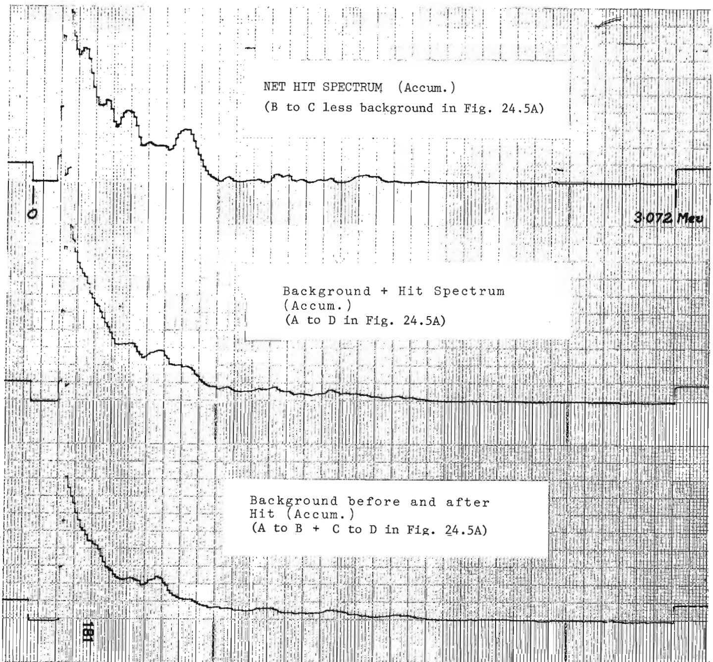
Figure 24.6 These three spectra were generated by the "hit detector" and analysis program (see text) when it encountered the man-made source shown in Figure 24.5.
