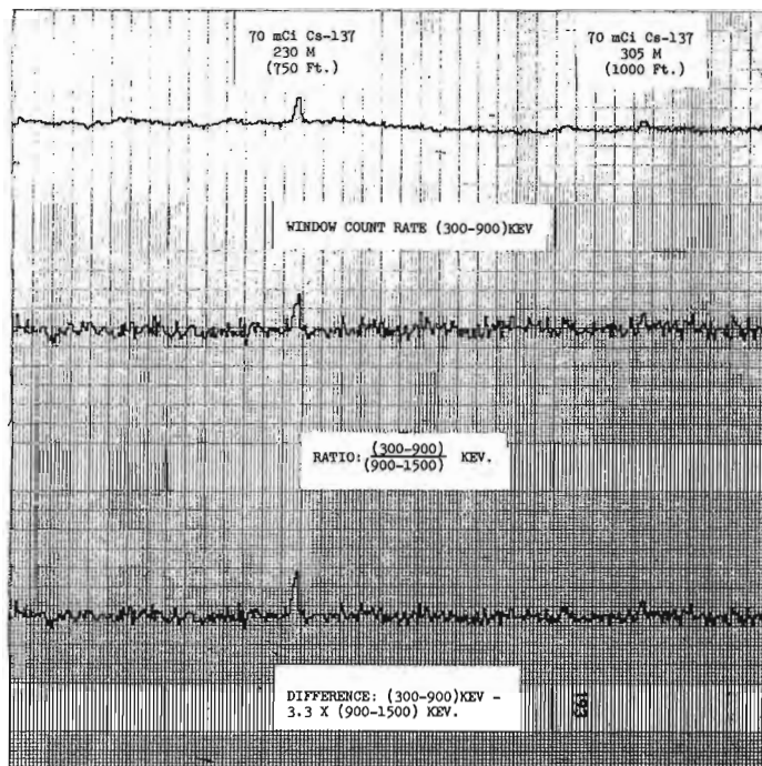
Figure 24.8 Strip chart profiles for consecutive overflights of a ^{137}\text{Cs} source at 230 m and 305 m.
