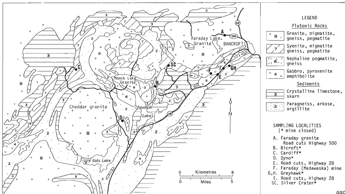
Figure 9.2. Geological sketch map showing location of samples in the Bancroft area, Ontario (after Ontario Department of Mines, Map 1957b, Haliburton-Bancroft area, Ontario).
