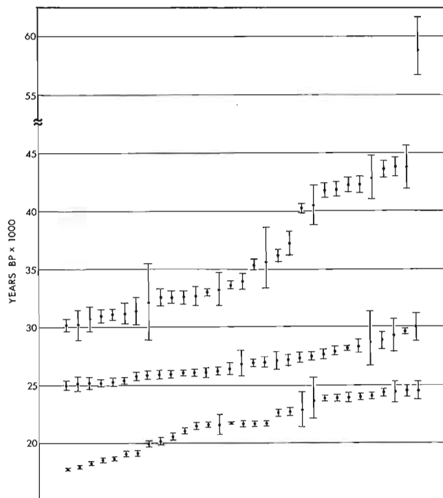
Figure 16.2. Finite radiocarbon dates from mid- and late-Wisconsinan stratified sediments (Besette sediments, Cowichan Head Formation, Quadra Sand, and unnamed correlatives) in British Columbia. The bar indicates the possible range on either side of the date. The five youngest dates are from stratified sediments occurring between two late Wisconsinan tills in the Fraser Lowland east of Vancouver. Dates are from Anderson (1968), Fulton (1971), Harrington et al. (1974), Clague (1975, 1977), Westgate and Fulton (1975), Fulton et al. (1976), Armstrong (1977), and Armstrong and Clague (1977).
