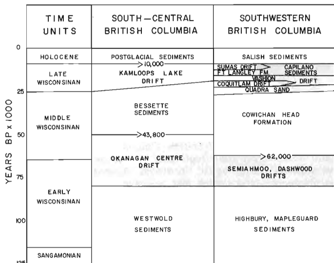
Figure 16.1. Late Quaternary stratigraphic framework of British Columbia. Drift units are stippled. References: south-central British Columbia, Fulton (1975); southwestern British Columbia, Fyles (1963), Armstrong (1975, 1977).
