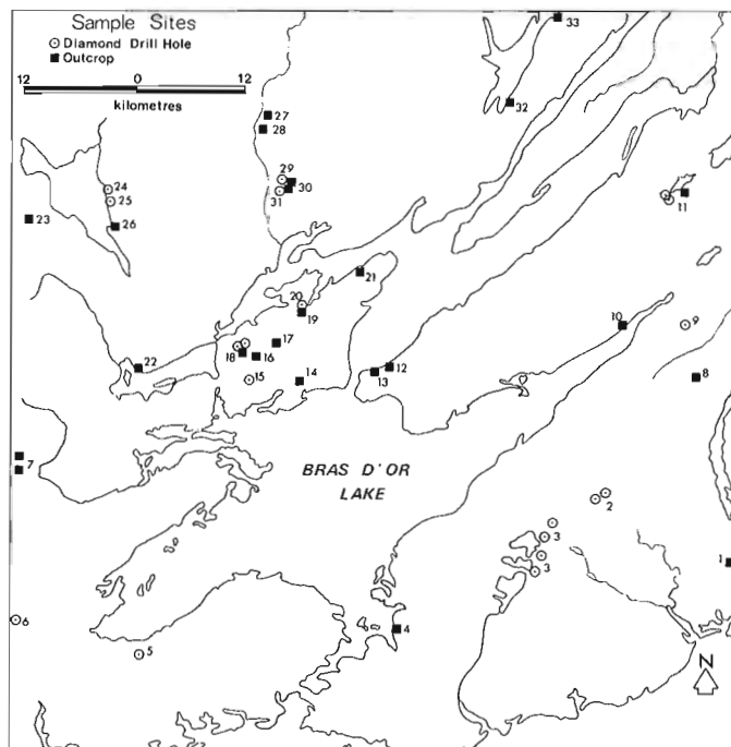
Figure 21.2. Map showing sample sites and localities referred to in text. Locality names are listed in Tables 21.1 and 21.2.
