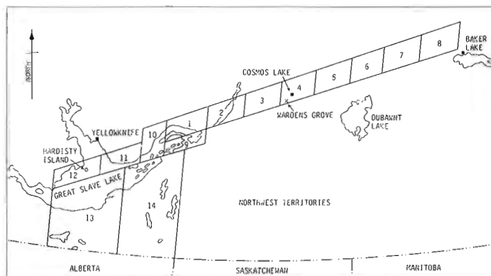
Figure 24.1 The impact trajectory of the satellite stretches from Great Slave Lake northeast toward Baker Lake. Sectors 13 and 14 were established with wind borne material in mind.
