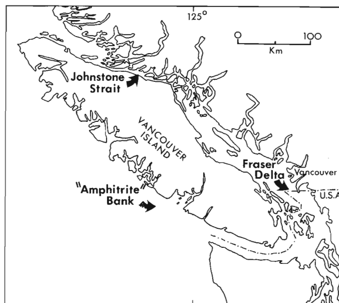
Figure 1. Index map identifying locations of study areas.
