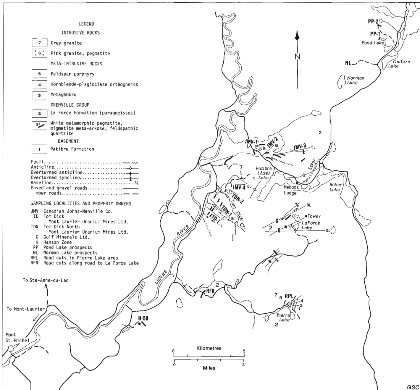
Figure 9.1. Sketch map showing radioactive occurrences and location of samples in the Patibre Lake area, 60 km north of Mont-Laurier, Quebec (after L. Kish, 1977, map DPV-487, and Tremblay, 1974).
