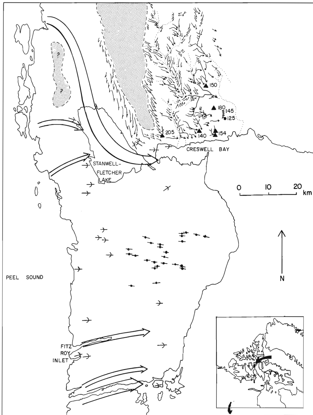
Figure 1. A map of southern Somerset Island showing nonglacial terrain (dotted areas), lateral meltwater channels (arrows with single barbs which indicate the down-ice side), subglacial meltwater channels (arrows with double barb), glacial grooves and striae (arrows with crescentic barbs), flutings in till (shafts with dots), fiords and troughs (large open arrows), pre-Holocene marine deltas (black triangles), a pre-Holocene marine beach (hachured line), a delta marking the Holocene marine limit (black dot), and the elevations of raised marine deposits in metres (numbers beside symbols).
