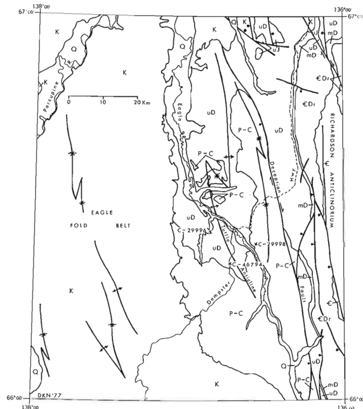
Figure 1.1. Geological map of Eagle River area (116 I), Yukon Territory, showing the stratigraphic and structural setting of GSC loc. C-46794 from which the two phyllocarid specimens were recovered.
