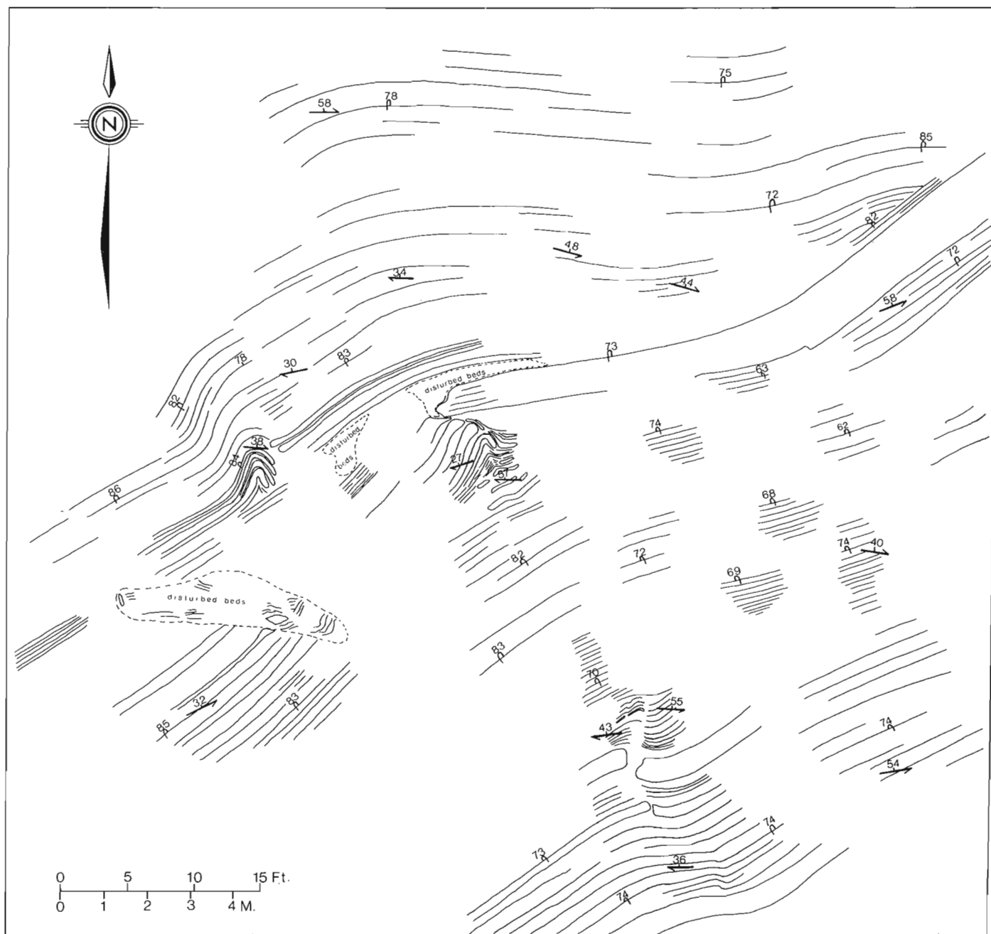
Figure 2. F_0 folds in turbidite, sedimentary rocks 900 m north-northeast of South Porcupine. Attitude of S_1 shown by barbed lines.
