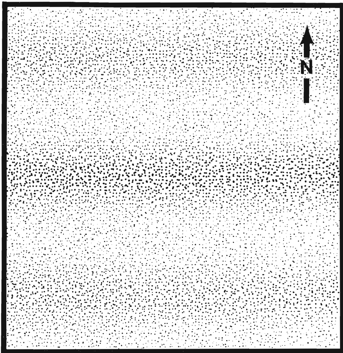
Figure 25.1. Sketch illustrating the concept of parallel belts of radioelement enrichment by remobilization due to metamorphism. The density of dots is proportional to the intensity of metamorphism and thermal remobilization and also radioelement enrichment. The illustration shows three parallel belts (two of minor intensity, one of major intensity) striking in an east-west direction. The centre belt contains the highest degree of radioelement enrichment.
