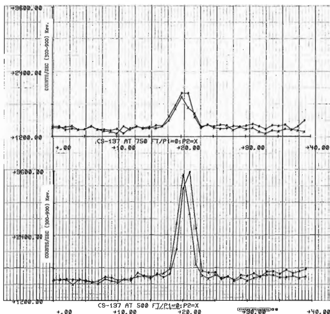
Figure 24.7 Count-rate profiles in the (300-900) keV window are shown against time (one second per point) as the spectrometer was flown over a ^{137}\text{Cs} source at two altitudes, two passes at each one.
