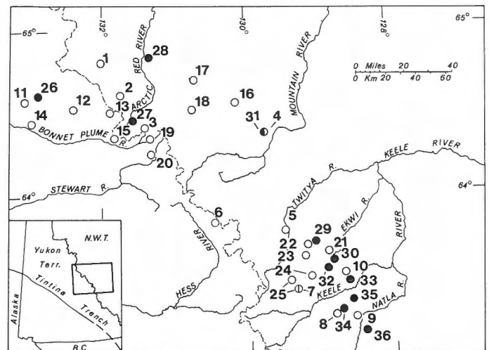
Figure 1. Index map. Solid circles locate sections described in this paper. Open circles locate sections described in previous papers (Fritz, 1976b, 1978).
