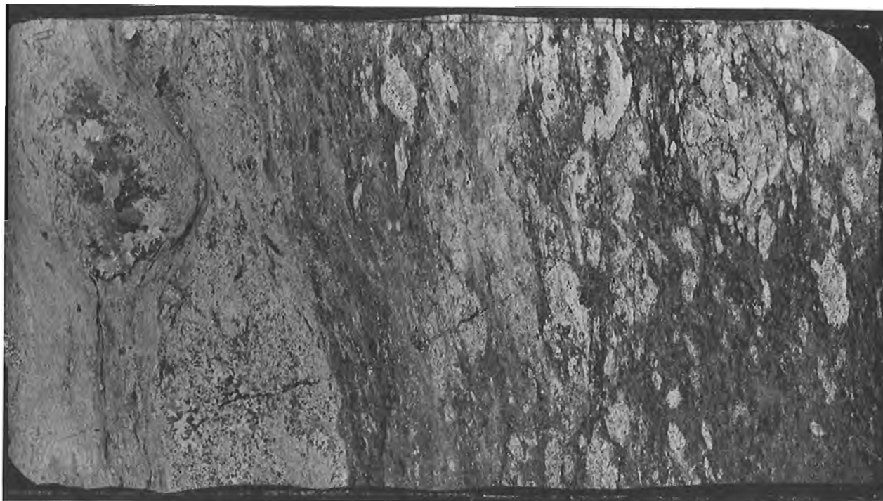
Figure 14.6a. Photomicrograph of a fragmental rock. Note two possible bedding contacts. Sample 17-19, magnification is 4X, crossed nicols.
