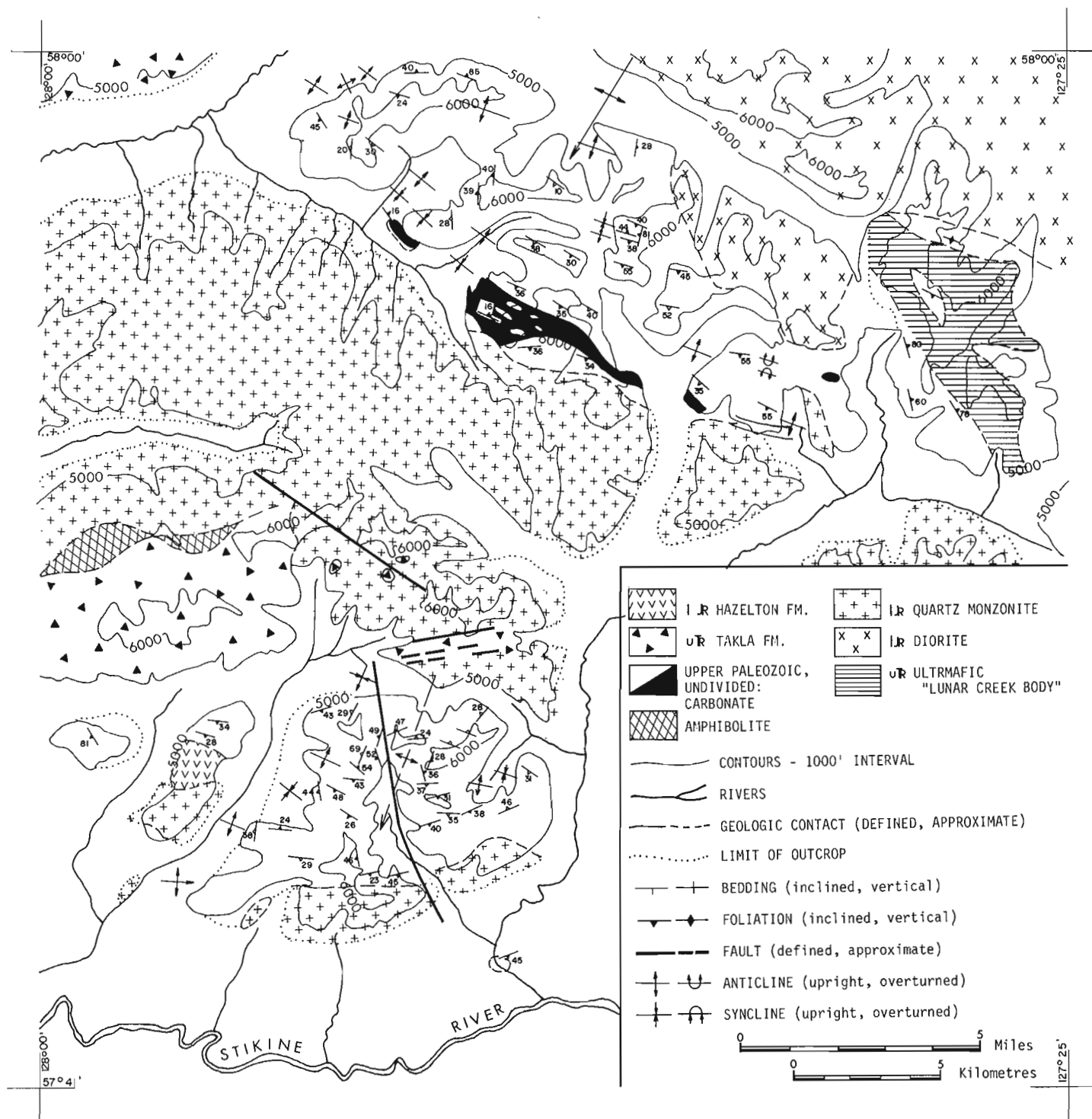
Figure 23.2. Geologic sketch map showing distribution and major structural elements of Upper Paleozoic rocks and relations to other rocks in the northwest Toadoggon map area.
