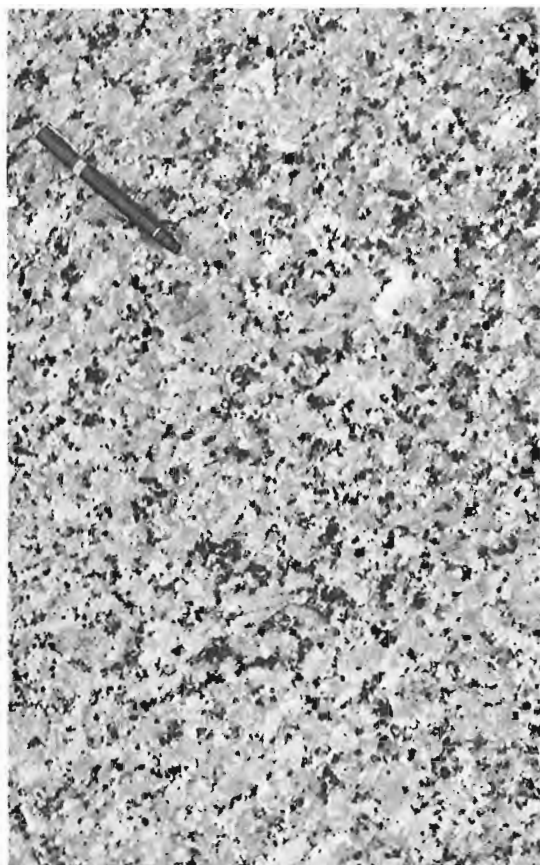
Figure 2.3. Coarse grained biotite granite of Islands from Figure 2.4. (GSC 177326)
