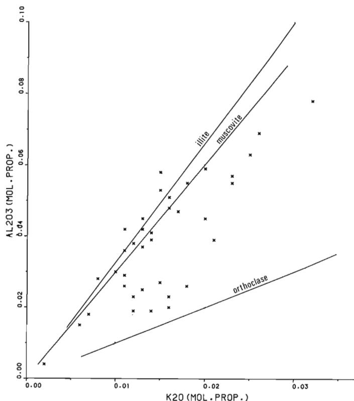
Figure 16.7. Binary plot of the molecular proportions of \text{Al}_2\text{O}_3 and \text{K}_2\text{O} in shales, cherts and carbonates from Section 44. The stoichiometric compositions of illite, muscovite and orthoclase are also plotted.
