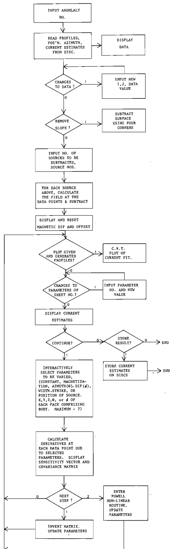
Figure 7.3. Relaxation program.
