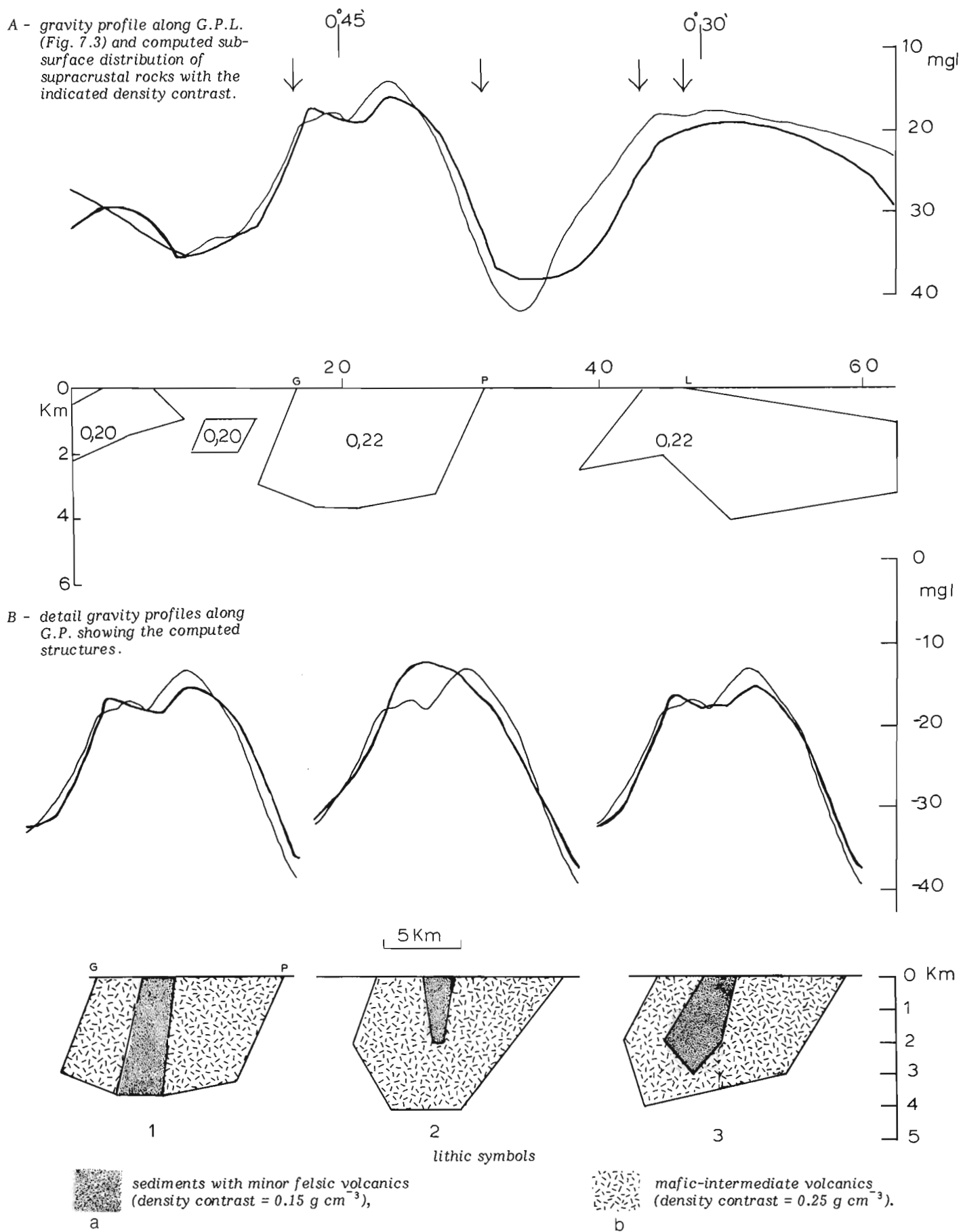
Figure 7.4. Bouguer gravity models for the Nangodi volcanic belt; observed (thin line), computed (thick line).
