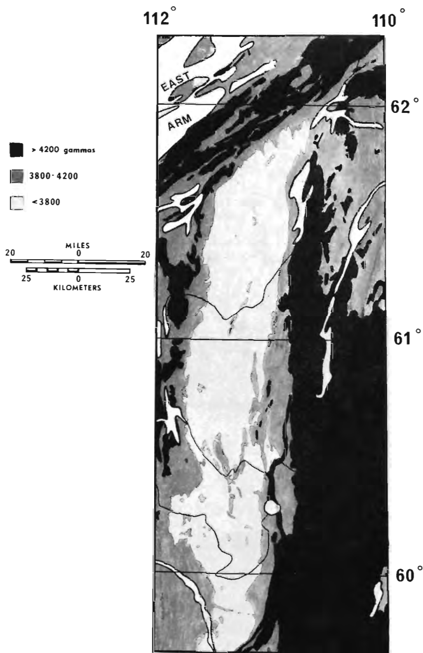
Figure 5.3. Aeromagnetic map of the Fort Smith Belt.
