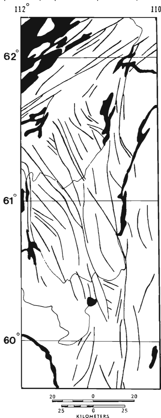
Figure 5.2. Major lineaments from satellite image.
