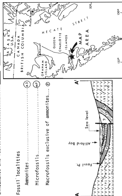
Figure 4.1. Geology of Alliford Bay Syncline.
