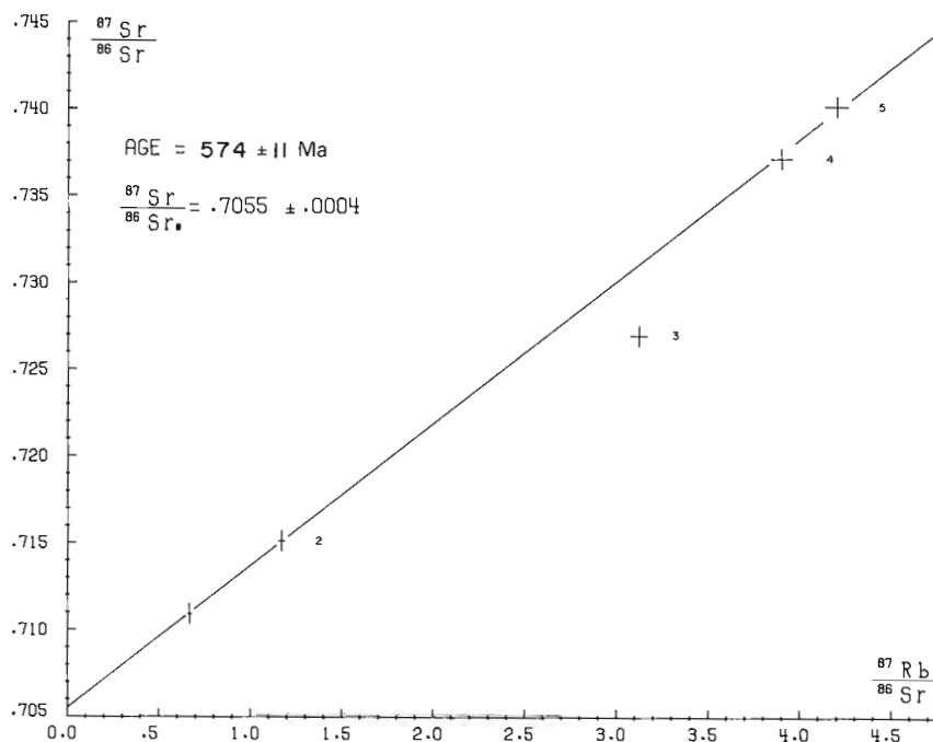
Figure 1. Rb-Sr isochron, Shunacadie pluton, central Cape Breton Island, Nova Scotia.
