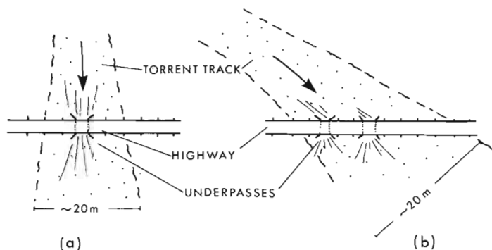
Figure 3.10. High-angle (a) and low-angle (b) intersection of roadbed and torrent track. In case (b) damage tends to be much greater than in case (a).
