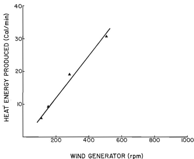
Figure 2. Heat produced by the heating coil with the generator operating at various speeds.
