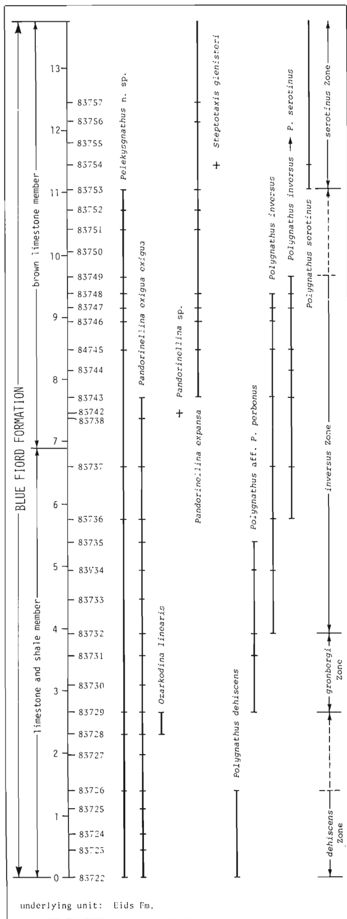
Figure 8.2. Conodont distribution and zonation of the Blue Fiord Formation exposed along creeks located 2.5 km east of the type section, and of the Bird Fiord Formation at its type section.
