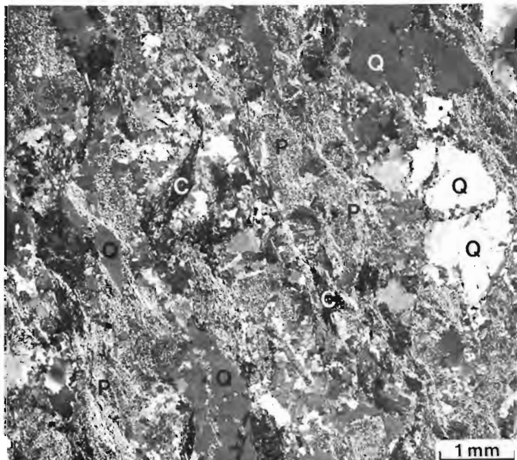
B. Schistose variety common in the southwestern part of the sample area. Sample 8, metatrandhjemite. Muscovitic schistose surfaces define a schistosity, saussuritized plagioclase (P) is deformed, quartz (Q) is more intensely deformed and some is polygonized, and mafic mineral (C) is completely altered to chlorite. (GSC 203617C)
