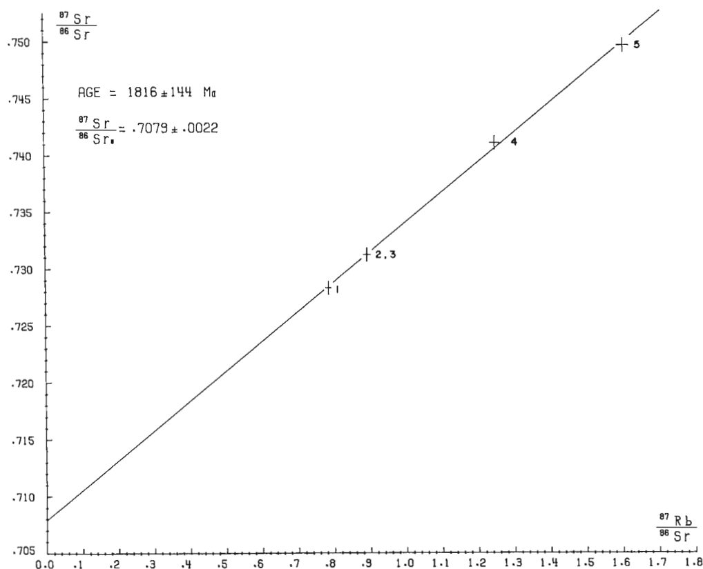
Figure 1. Rb-Sr isochron, Peninsular sill, Takijuk Lake, District of Mackenzie.
