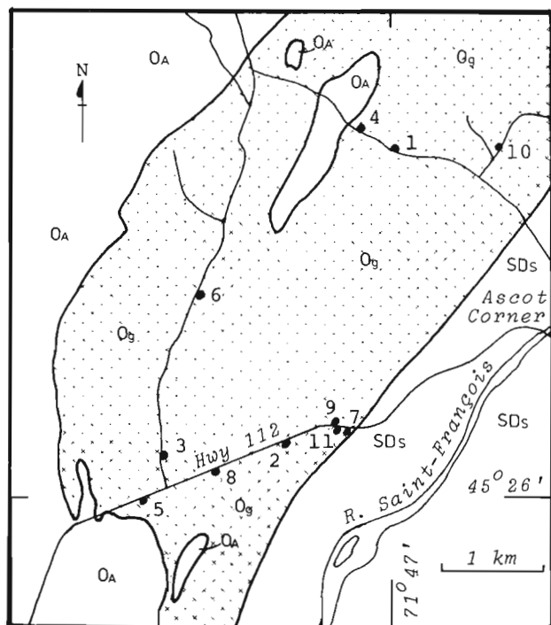
Siluro-Devonian SDs St. Francis Gp. Lower and Middle Ordovician Og Moulton Hill granite OA Ascot Fm.
