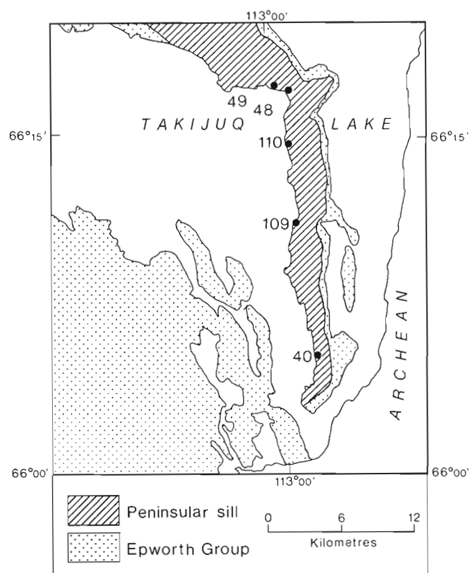
Figure 2. Sketch map of Peninsular sill, Takijuu Lake and sample locations.
