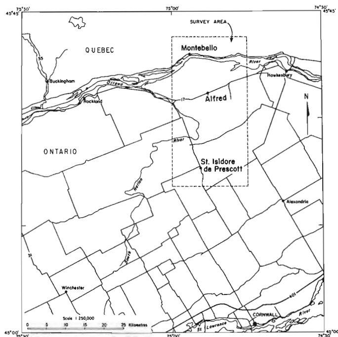
Figure 1.1. Location map for the Schlumberger resistivity survey in the Alfred-Hawkesbury area.
