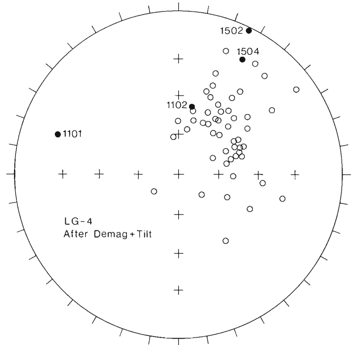
Figure 1. All core directions after alternating field and/or thermal testing of stability of natural remanent magnetization. Beds rotated to horizontal. Open and closed symbols indicate directions up and down respectively (latter are indicated by site number followed by specimen number).
