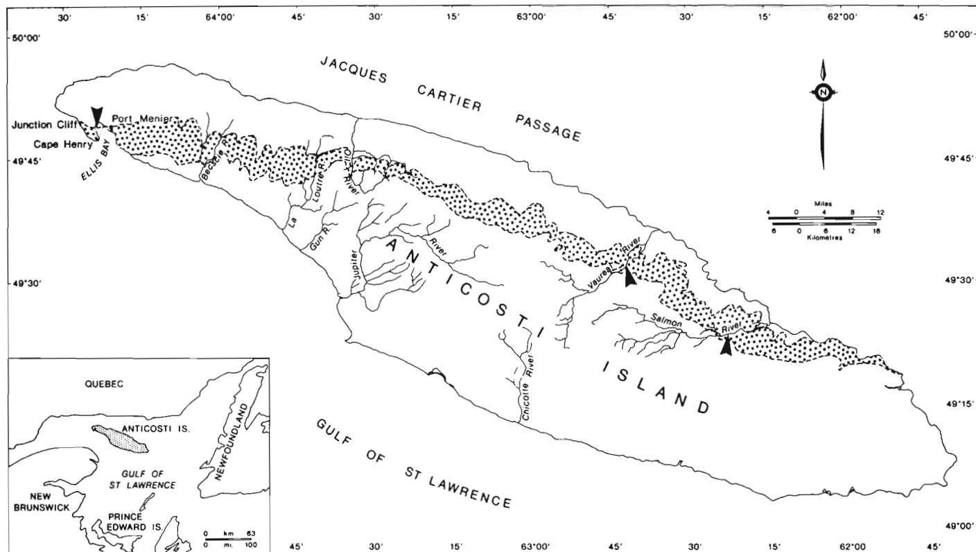
Figure 10.1. Index map of Anticosti Island showing the distribution of the Ellis Bay Formation (stippled) and locations of sections studied (arrows). Sections studied include those on the west and east sides of Cape Henry and the east side of Ellis Bay, and along the Vauréal and Salmon rivers. The Vauréal Formation outcrops to the north of the Ellis Bay Formation and was examined at the west end of the island, and on the Oil, Vauréal and Salmon rivers.
