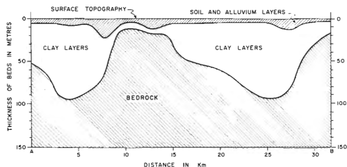
Figure 1.15. Cross-sectional profile along the line AB based on Schlumberger sounding in the area.
