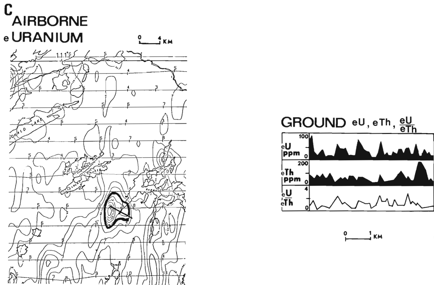
Figure 5.11. Ground gamma ray spectrometry across high eU and eU/eTh anomaly near Gagnon Lake (Area C, Fig. 5.7).
