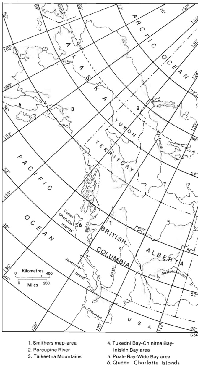
Figure 4.2. Locations of Iniskinites occurrences in British Columbia, southern Alaska and northern Yukon.
