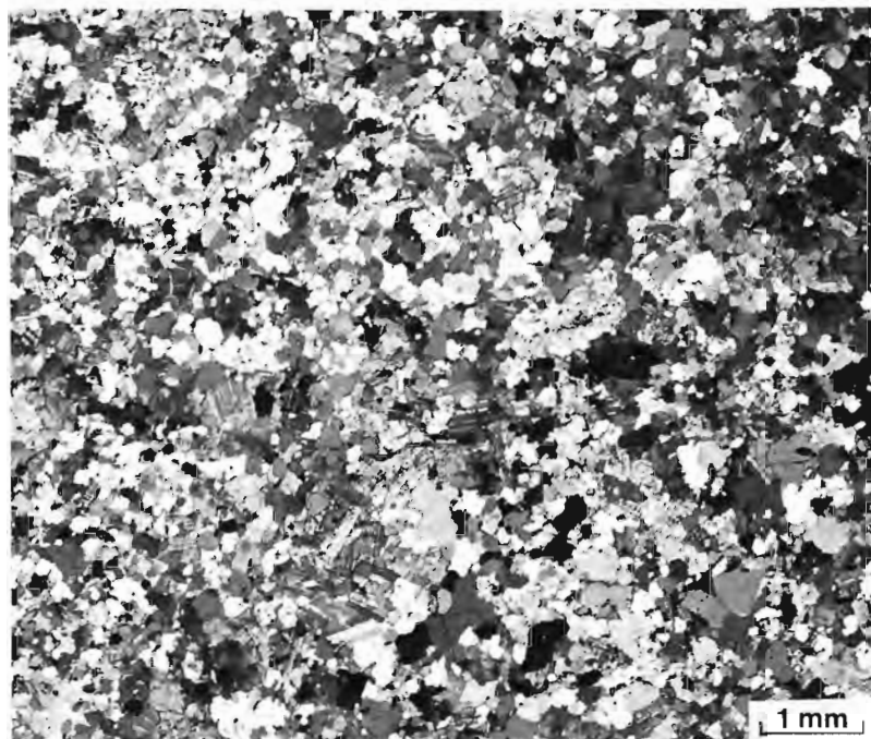
Figure 3. Photomicrograph of typical "Sugar" granite showing fine grained allotriomorphic granular mosaic (granoblastic) texture of undeformed albite, microcline, quartz and biotite. Sample A8. (GSC Photo 203617)
