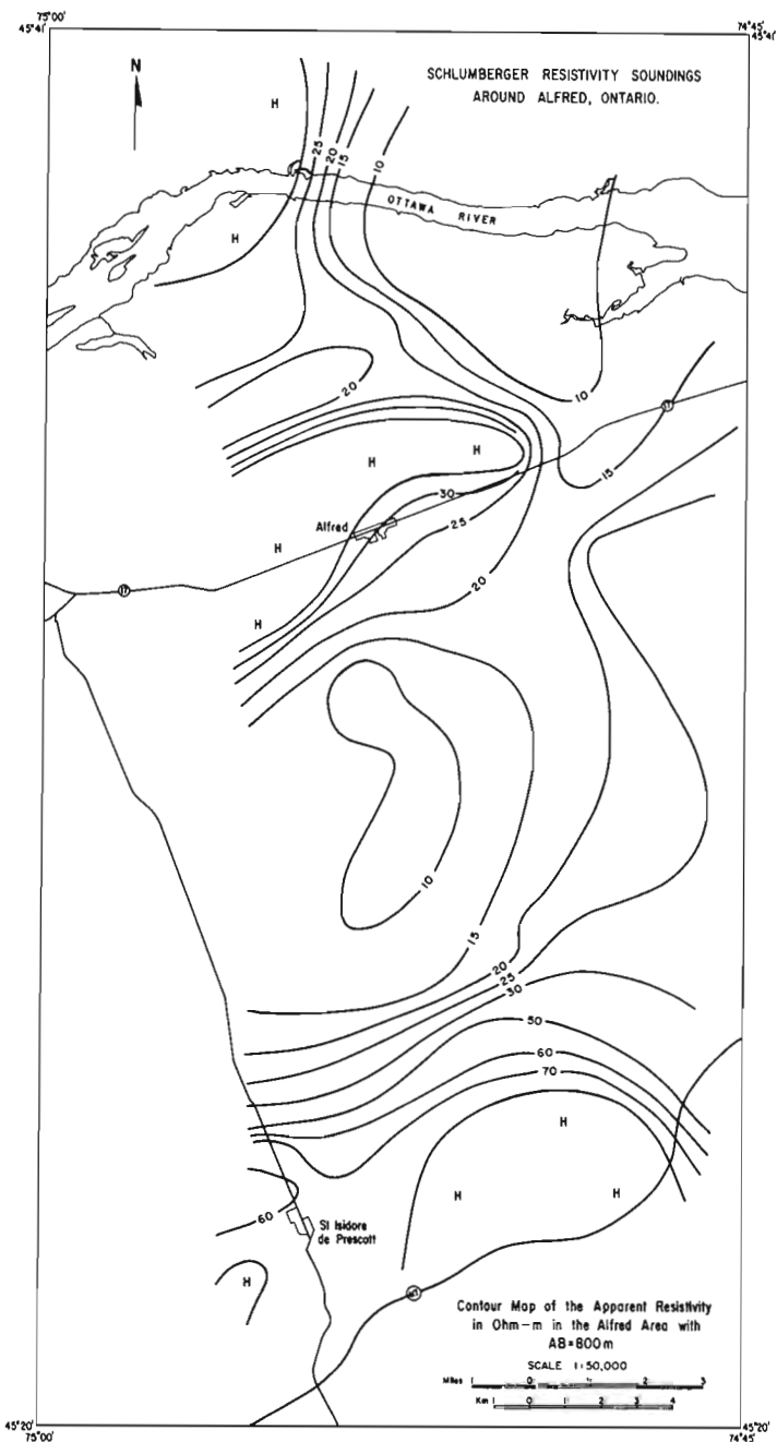
Figure 1.9. Equirestivity map of the area with current electrode separation of 800 m.
