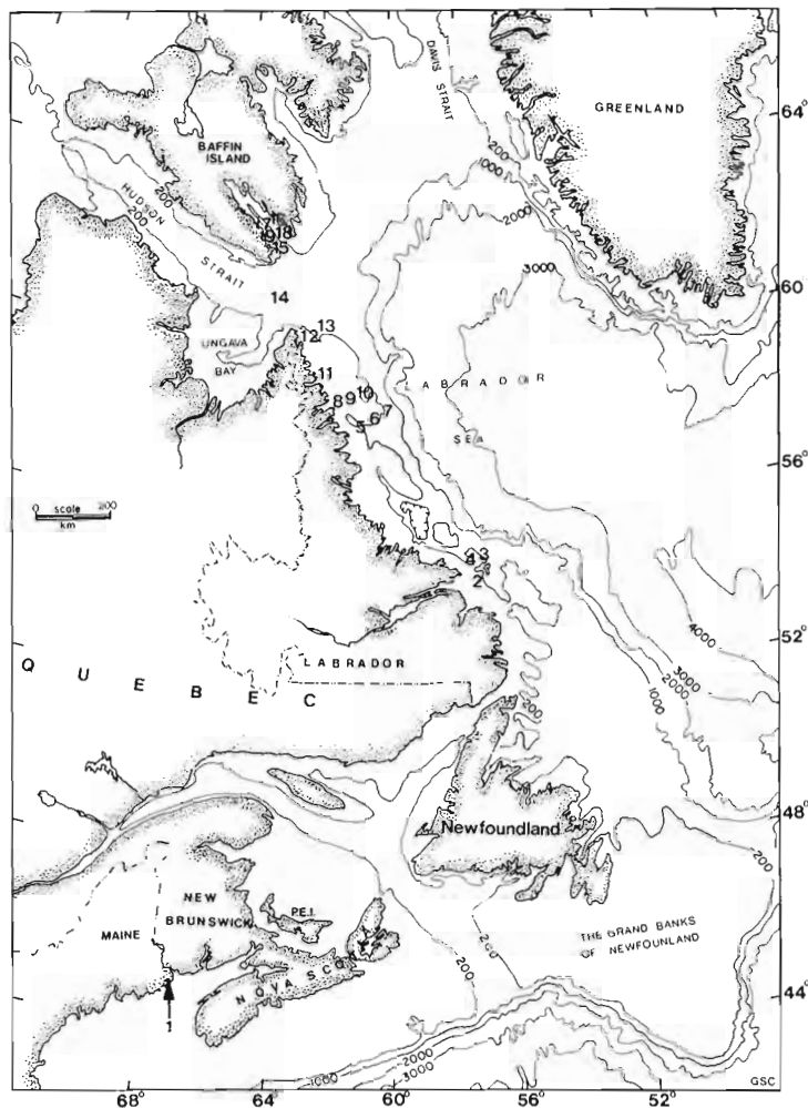
Figure 13.1. Location map for shell and total organic-matter ^{14}\text{C} dates. Numbers correspond to locations given in Table 13.1.
