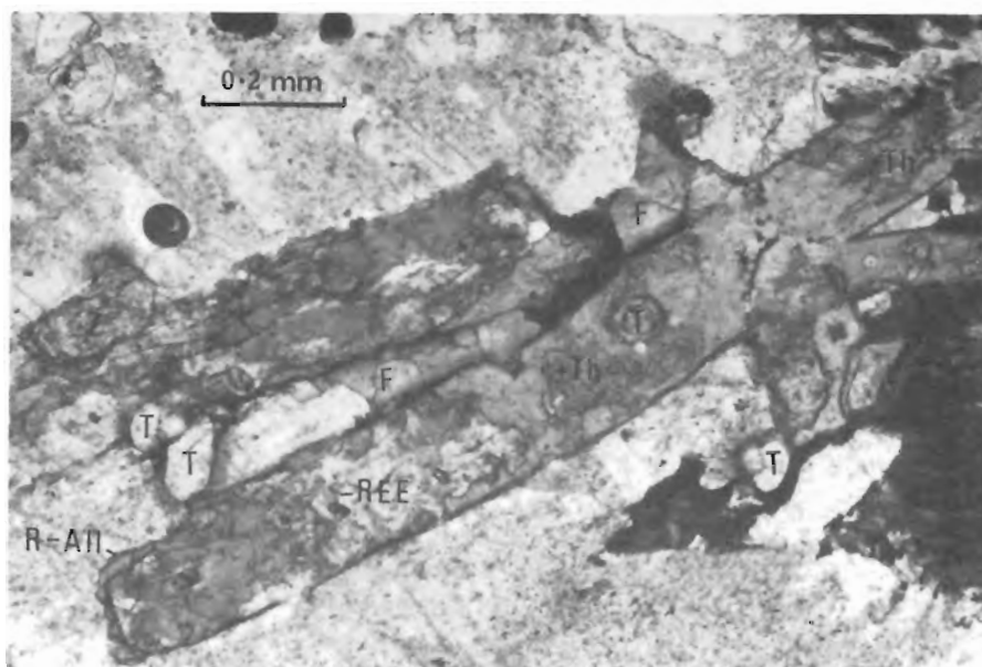
Figure 12.6. Sample 64N762152, Sharman Lake, Manitoba. "Allanite" with associated fluorite (F), in feldspar. Domains of thorium enrichment and REE depletion are indicated by +Th and -REE respectively. Thorite (T), zircon (Z), and regenerated allanite (R-All) are also present.
