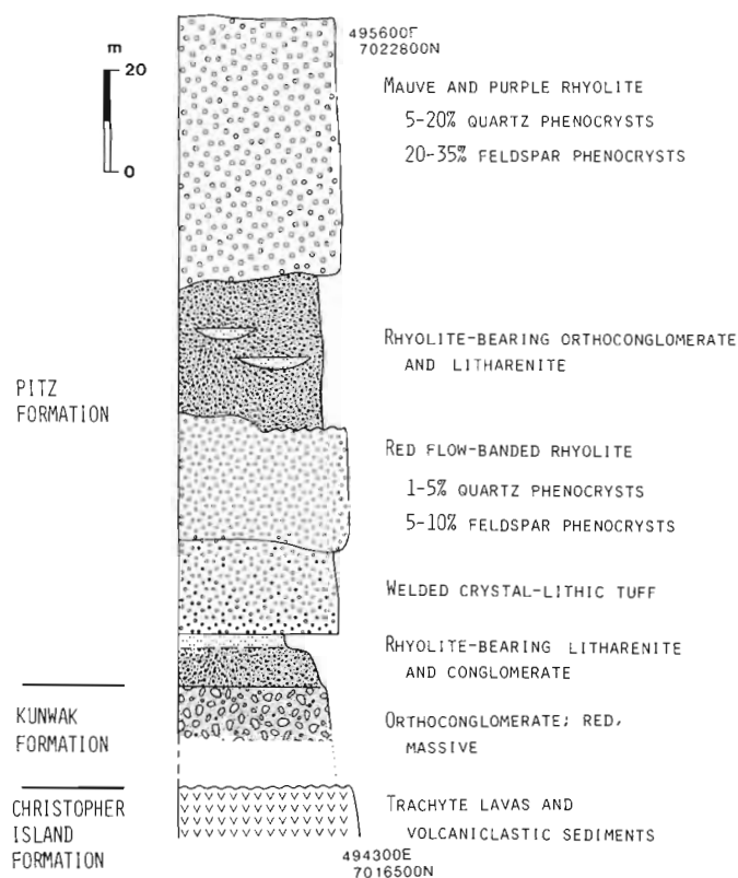
Figure 14.8. Diagrammatic section of the Pitz Formation along the Kunwak River north of Tulemalu Lake. Section location from approximately UTM 494300E, 7016500N to 495600E, 7022800N.
