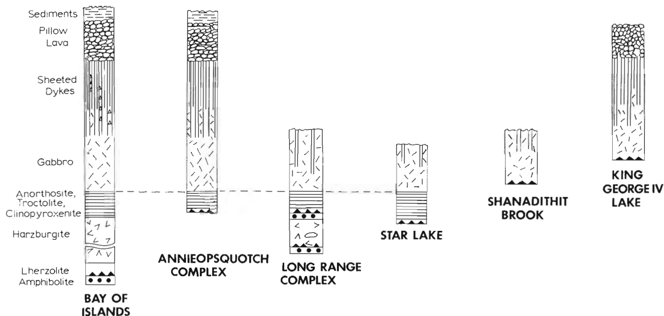
Figure 2.4. Schematic cross sections of west Newfoundland ophiolites. Thicknesses uncertain as some lithological units are separated by faults. Bay of Islands complex modified from Malpas and Strong (1975); Annieopsquotch complex after Dunning and Herd (1980); Long Range complex after Brown (1976); King George IV Lake ophiolite after Kean and Jayasinghe (1981).
