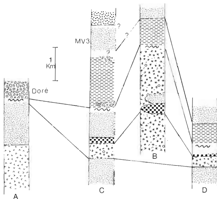
Figure 7.4. Stratigraphic correlation charts for the south-western part of the Wawa belt based on the map units in Figures 7.2 and 7.3. Lithic symbols are the same as on the maps. The unconformity at the base of the Doré and equivalent formations is indicated by wavy line.
