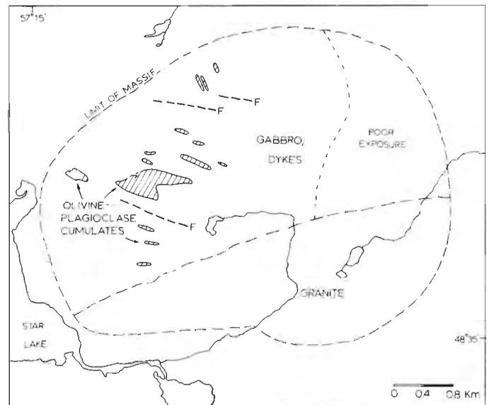
Figure 2.3. Preliminary geological map of the Star Lake ophiolite.
