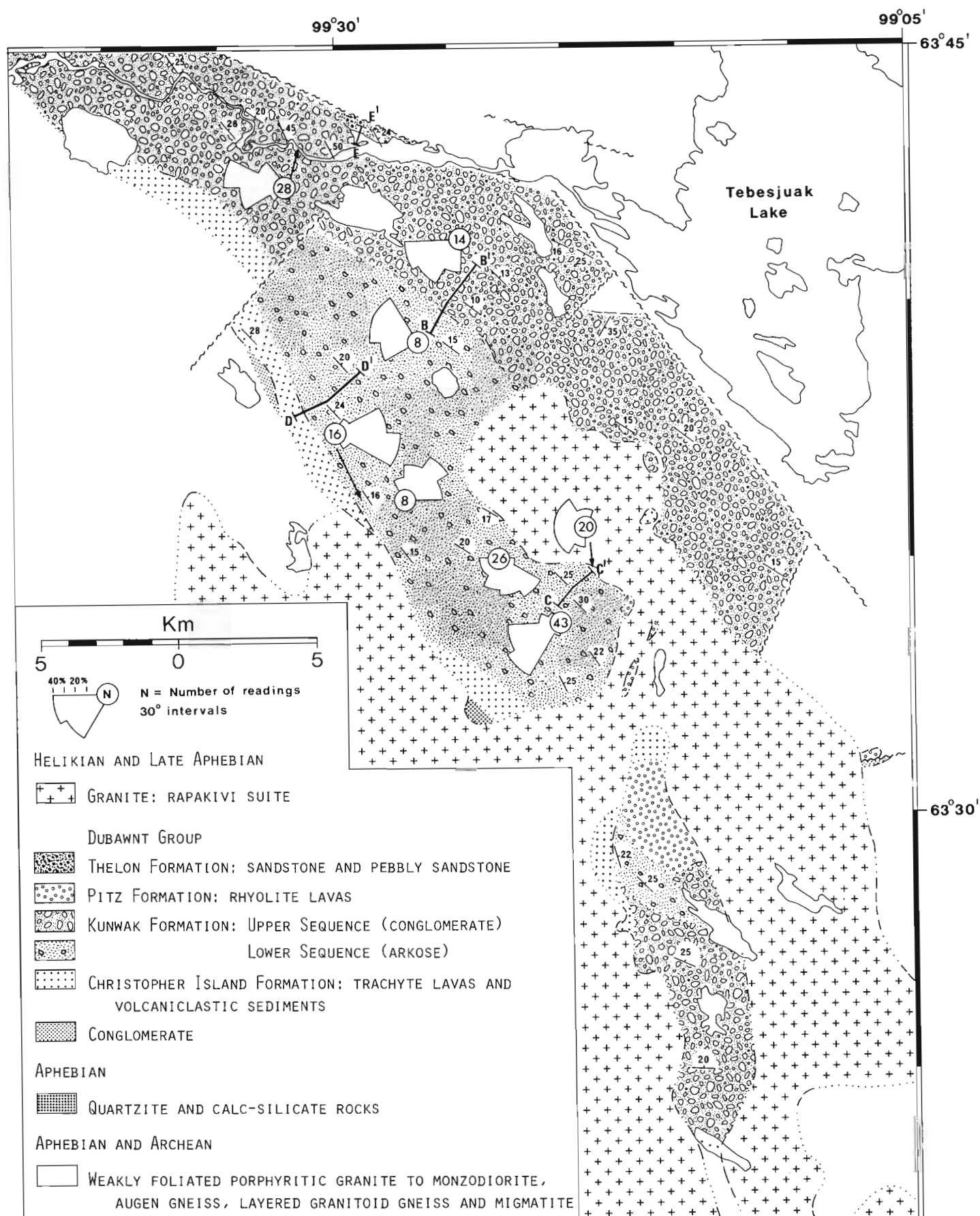
Figure 14.5. Geological map of southern parts of the Wharton Basin with rose diagrams of paleocurrent measurements.
