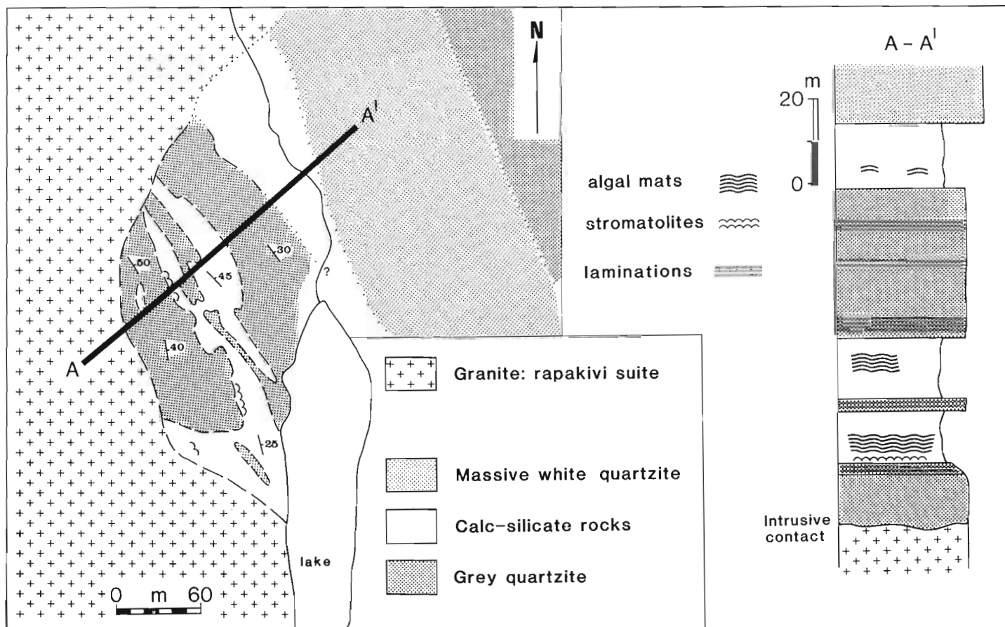
Figure 14.3. Geological map and generalized columnar section of a calc-silicate-quartzite sequence northeast of Pukik Lake. Detailed mapping by K.A. Roberts.
