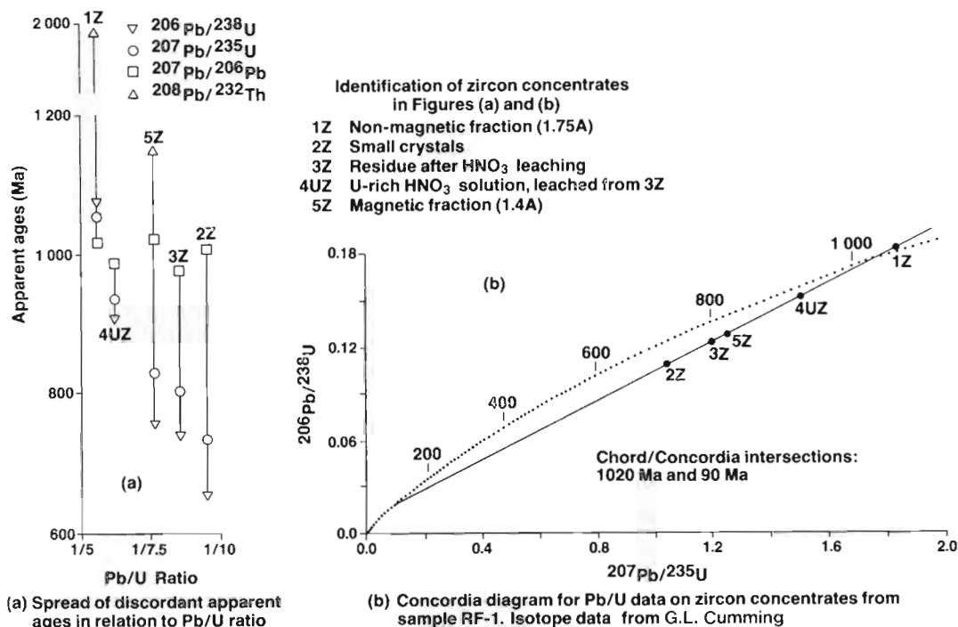
Figure 4.1. Diagrammatic representation of isotopic data for zircons from high grade uranium ore RF-1 at the Madawaska uranium mine, Bancroft area, Ontario.
