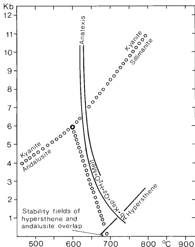
Figure 10.10. Metamorphic grid (Winkler, 1979) illustrating the stability fields of the aluminosilicates and hypersthene, and showing a small field where both andalusite and hypersthene may be expected to form in rocks of appropriate composition.
