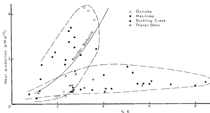
Figure 1. Heat production versus K for samples from the northern Hagem batholith. Boulder Batholith trend line is adapted from Tilling et al., 1970. Dashed lines outline the fields for Osilinka-Mesilinka and Duckling-Thane/Detni suites.
