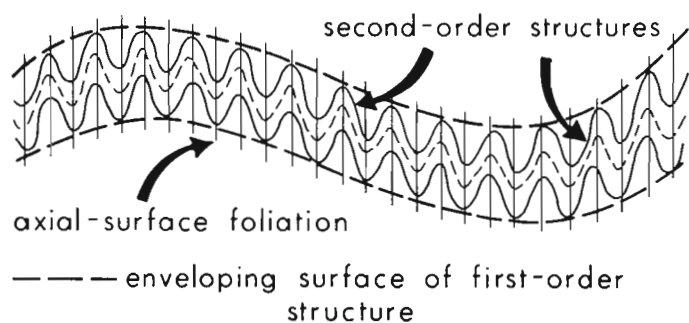
Figure 2. Sketch illustrating ordering of tectonic structures, and the relationship of layering to enveloping surfaces.
