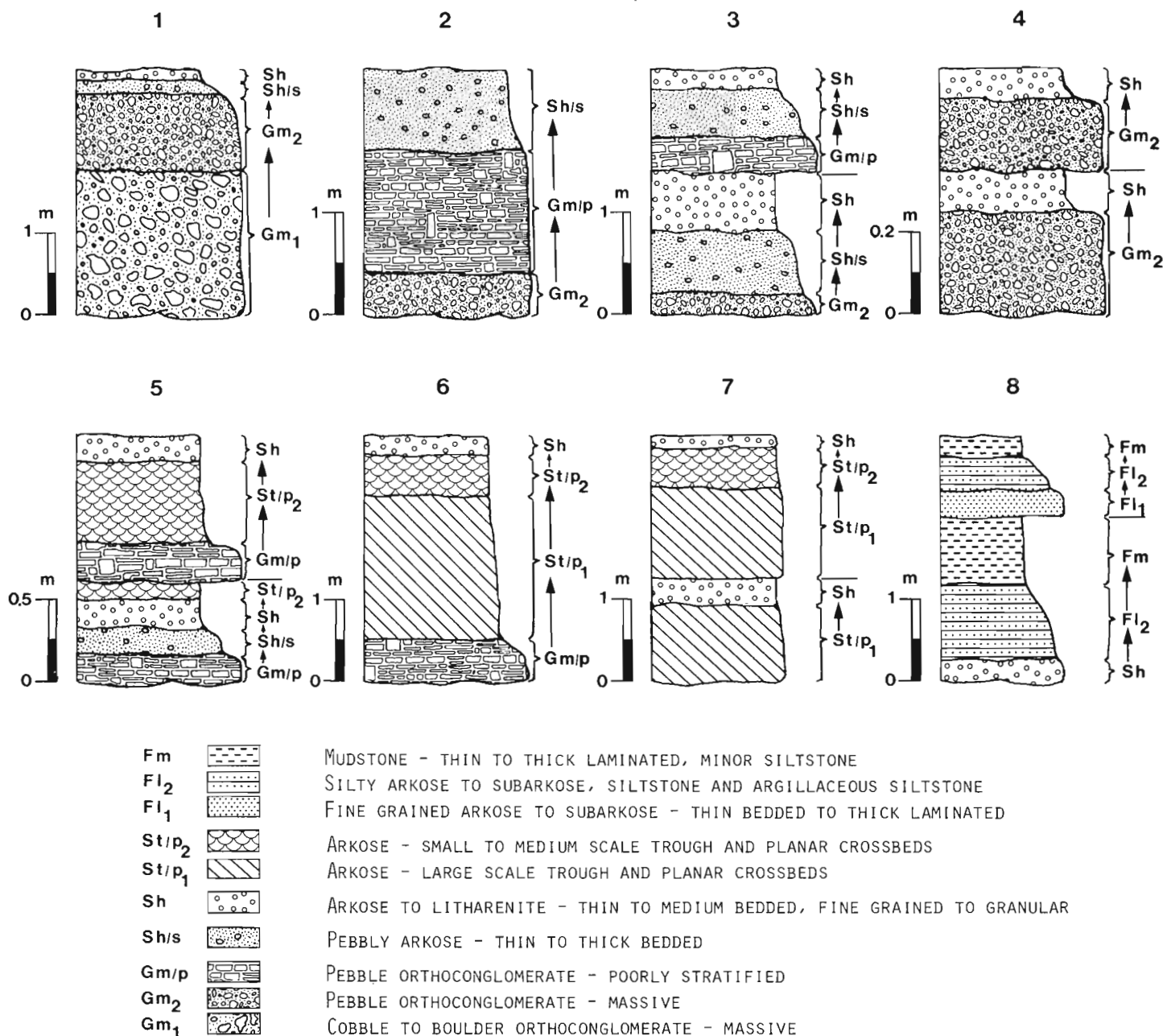
Figure 14.7. Representative fining-upward cycles for the Kunwak Formation. All types occur in the Wharton Basin except for 8, which is located south of 637 Lake. Facies identifiers adapted from Miall (1977).
