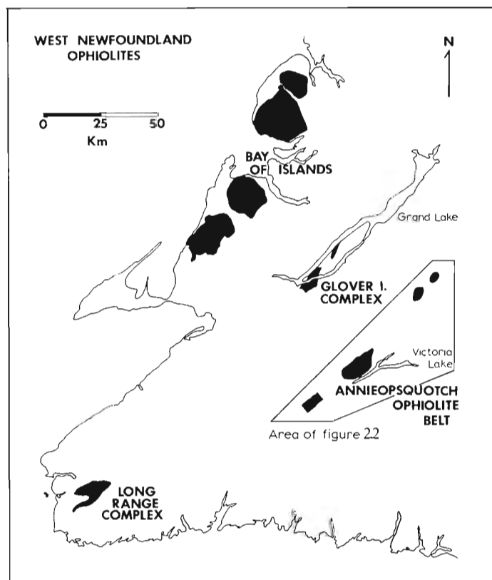
Figure 2.1. The Annieopsquotch ophiolite belt and other ophiolite complexes of western Newfoundland.
