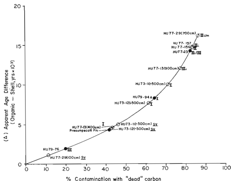
Figure 13.3 Nomogram for estimating contamination by "old" carbon, that is carbon with no detectable ^{14}\text{C} . \Delta equals difference between an assumed correct age based on ^{14}\text{C} dated shells and significantly older dates based on total organic-matter (t.o.m.). The curve shape has been derived using the Libby half-life of 5568 years. Solid dots indicate contamination estimates based on shell - t.o.m. data sets from individual samples. Open dots indicate differences between other t.o.m. dates and the median ages (Table 13.2) of the acoustic-morphological units in which these samples are located. Cores Hu 73-11 and Hu 73-12 (Table 13.1) have multiple t.o.m. dates in both the exceptionally thick surficial veneer (<500 cm) and acoustic-morphologic unit I (>500 cm). For simplicity in this figure the plotted age differences were calculated from averages of all the ^{14}\text{C} dates in each unit. Roman numerals refer to acoustic-morphologic units (Fig. 13.2). SV = surficial veneer.
