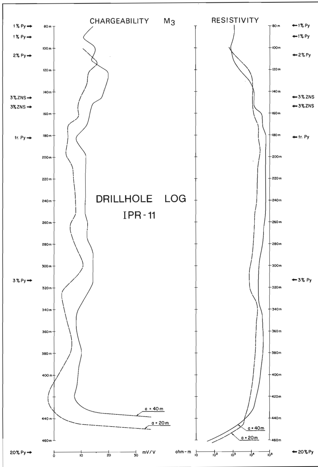
Figure 12.7. Far-hole results ('a' spacing 20 m and 40 m) for the Nanisivik drillhole IP logs.
