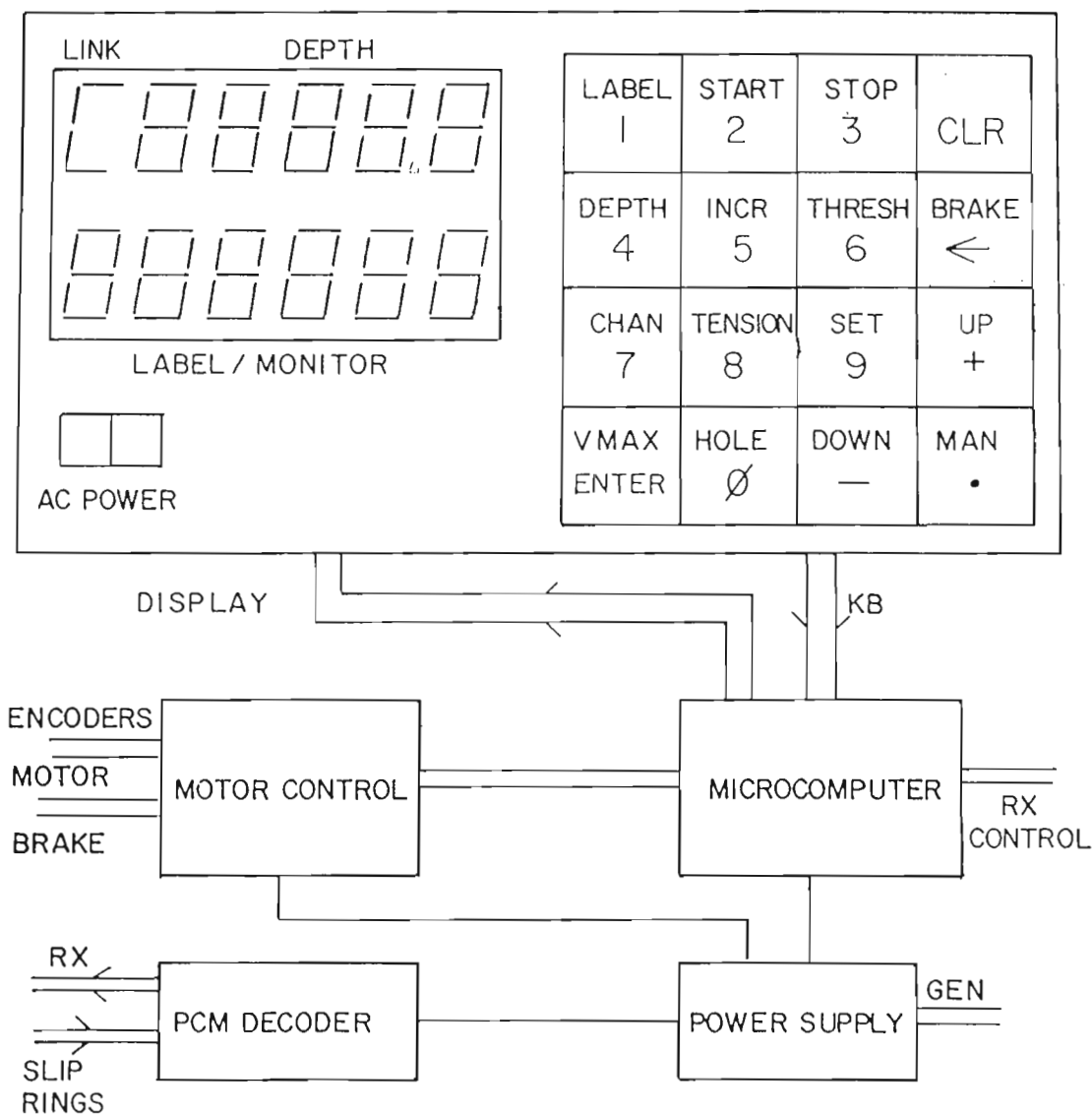
Figure 11.5. Schematic diagram of the UTEM borehole system controller.
