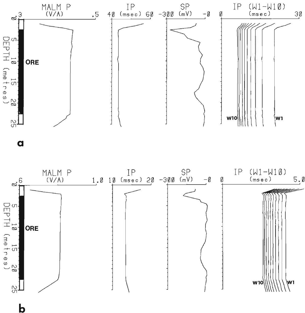
Figure 15.13. Mise-à-la-masse potential and IP measurements made along hole 3295-W2400. (a) with the current electrode in ore at a depth of 9 m in hole 3065-W2300. (b) with the current electrode in hole 3316-W2350 at a depth of 24 m.
