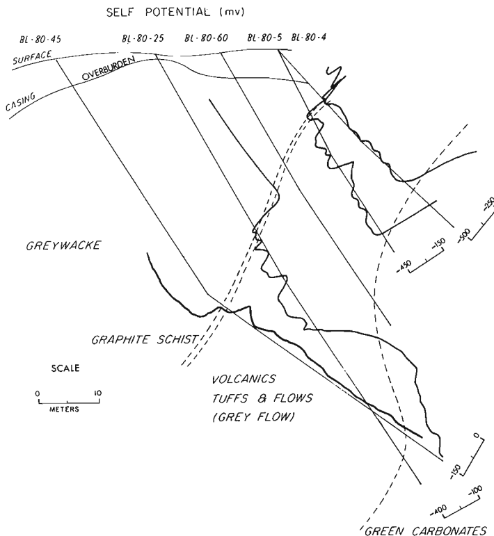
Figure 2.7. Portable SP results plotted along the boreholes (dark lines) for a fence of boreholes across the main ore zone. Measurements were taken every 0.2 m.
