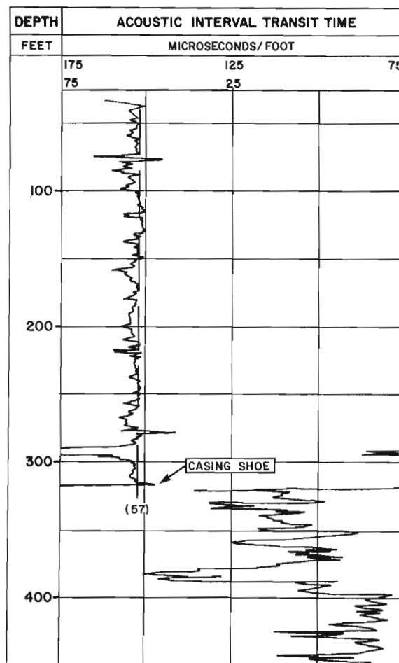
Figure 12. Acoustic tool casing signal: high integrity data.
