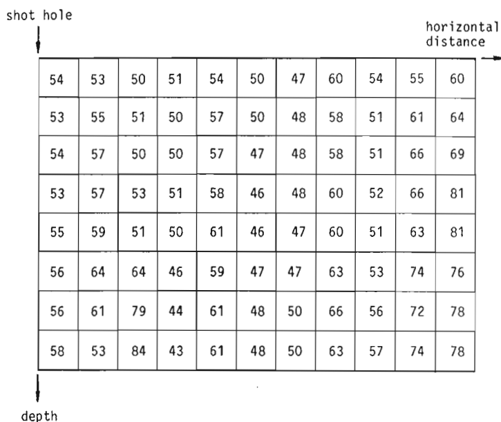
Figure 18.5. Velocity solution, for Kråkemåla; cell-velocities in hectometre/second.
