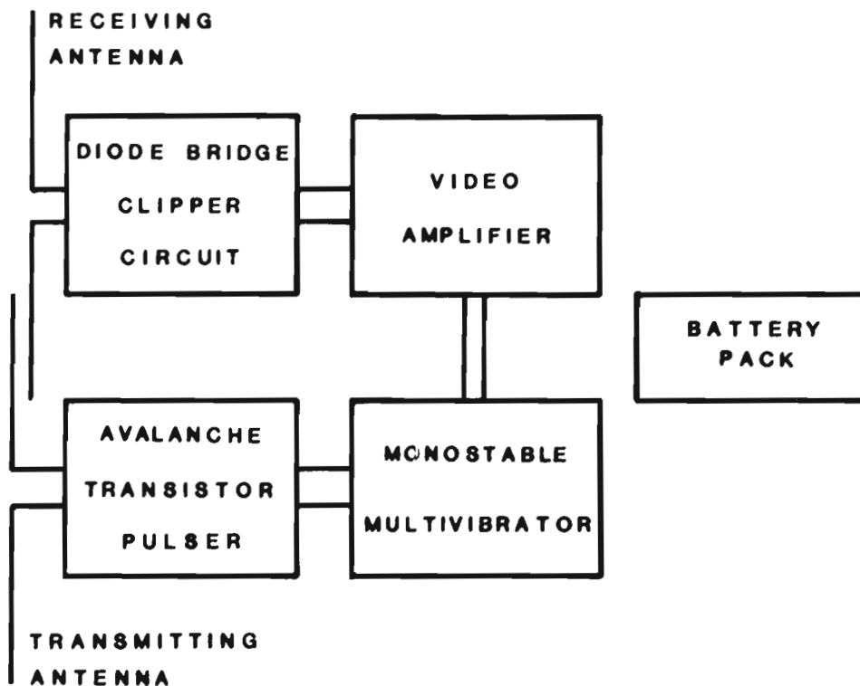
Figure 23.11. The transponder consists of only four electronic functional blocks. All power is derived from batteries to minimize internally generated electronic noise.
