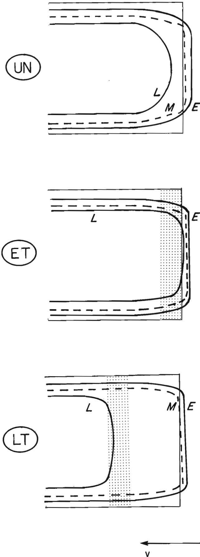
Figure 35.15. Migration of zero crossings with time over the three plate models. The plane of measurement is raised 0.1W above the plate where W is the width of the plate.
