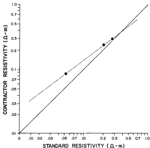
Figure 22. Fluid resistivity bridge field calibration check, indicating improper calibration.
