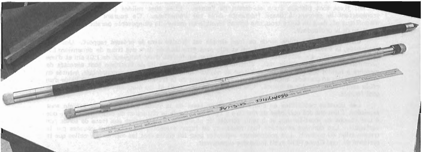
Figure 32.2. The downhole probe.
