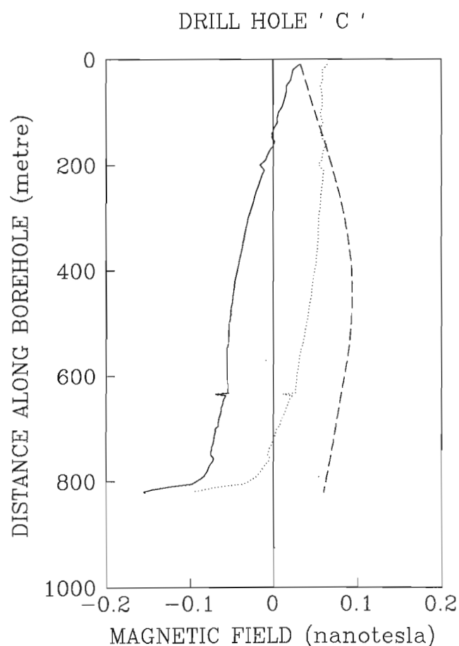
Figure 32.6. Plots of the magnetic field measured in the hole direction (dotted line), correction for non-vertical hole effects (dashed line), anomalous magnetic field (solid line).
