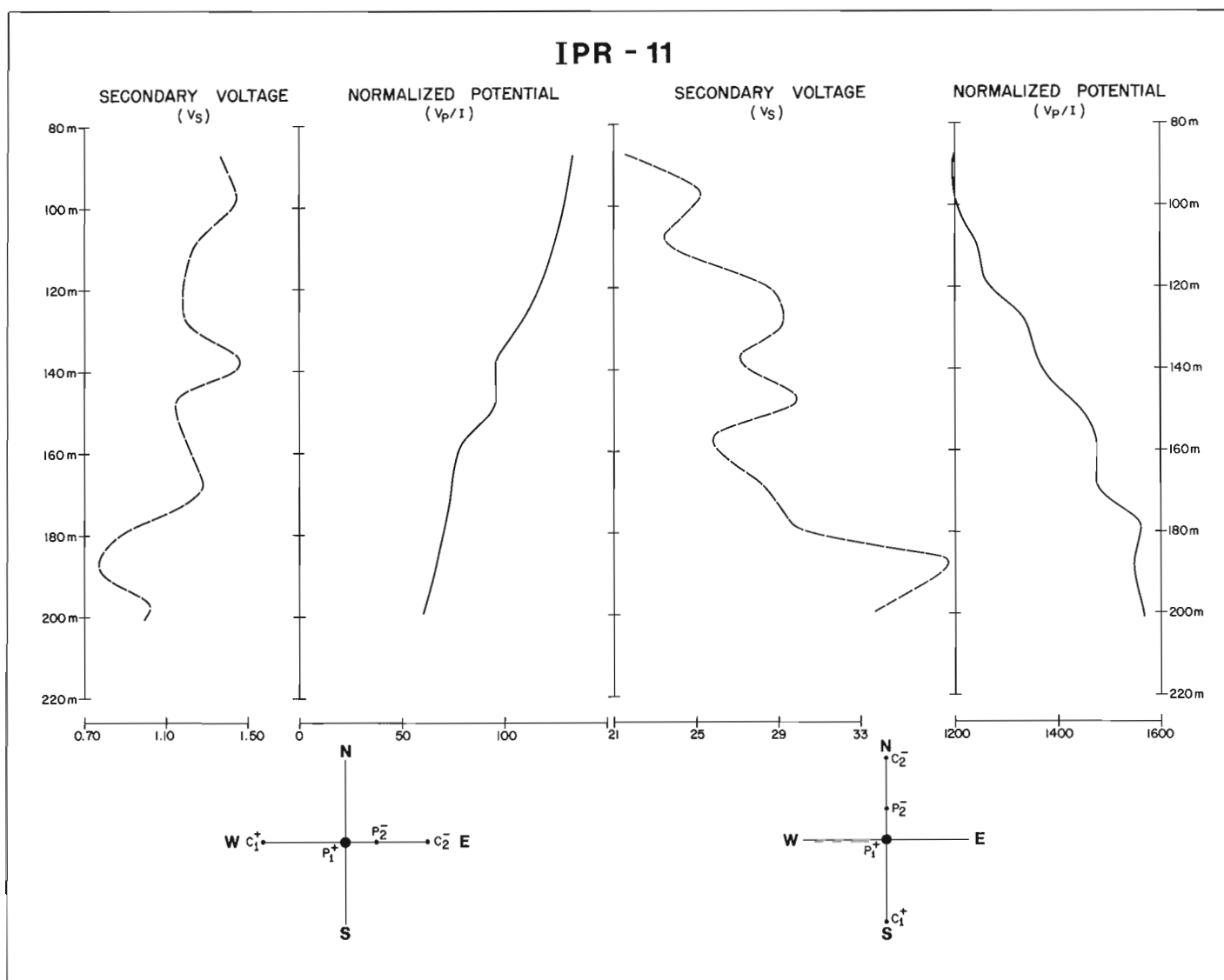
Figure 12.8. Directional array results of drillhole IP logging of the Nanasivic deposit.
