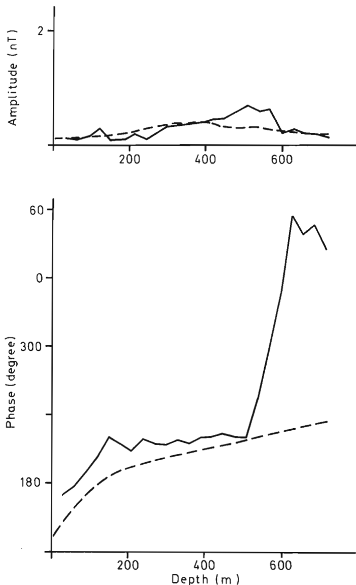
Figure 9.9. Kankberg Bh 109. A comparison between the theoretical model and the measured data for the y-component at 2000 Hz. The solid line represents the measured data and the broken line the theoretical model.
