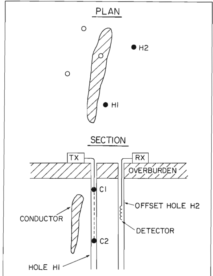
Figure 32.1. The geometry of the crosshole MMR method.
