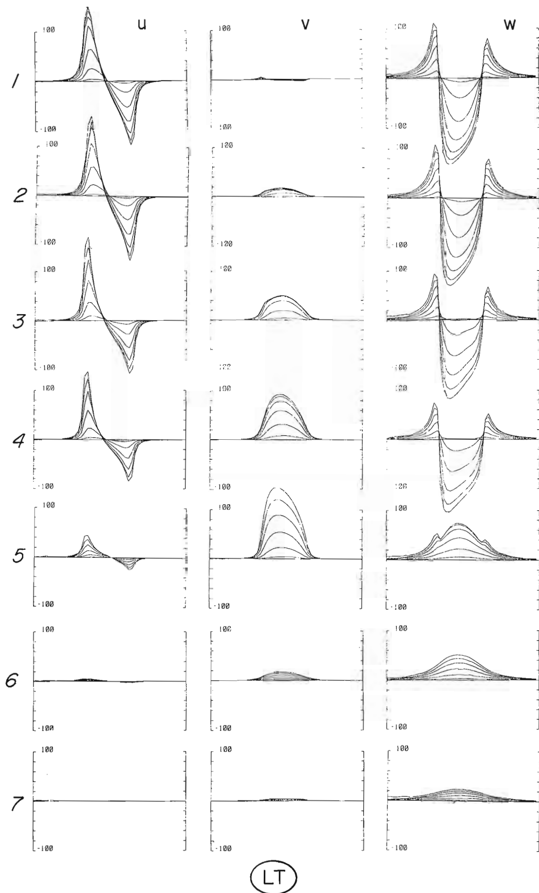
Figure 35.13. UTEM response across the locally thickened conductor. Since the profiles are all parallel to the thickening, the anomaly is less obvious on these profiles than those in Figure 35.10.
