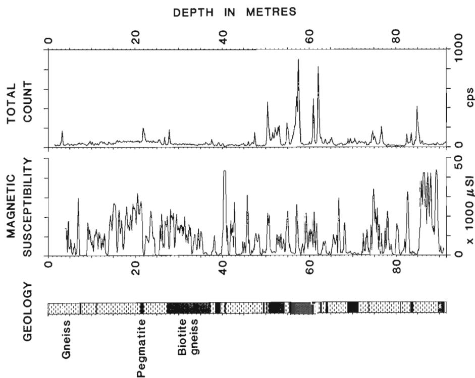
Figure 3.9. Geological log, magnetic susceptibility (MS) log and total count (TC) log recorded in Bancroft test hole BN-81-1 with the GSC research logging system. The MS log was recorded at 6 m/min and a sample time of 0.2 s. The TC log was run at 3 m/min and a sample time of 1 s using a 19 x 76 mm NaI (TI) detector.
