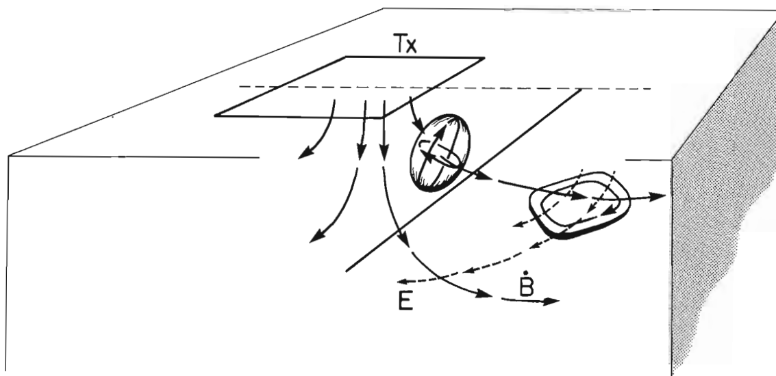
Figure 8.6. Current flow for the situation of a confined conductor showing induced currents and secondary electric and magnetic fields at the receiver.
