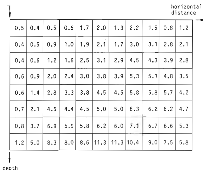
Figure 18.4. Relative statistical errors, for Kråkemåla; the numbers are estimator-standard deviations, in per cent of the velocity 5000 m/s at a true velocity of 5000 m/s and an error in travelttime-measurements of 0.5 ms.
