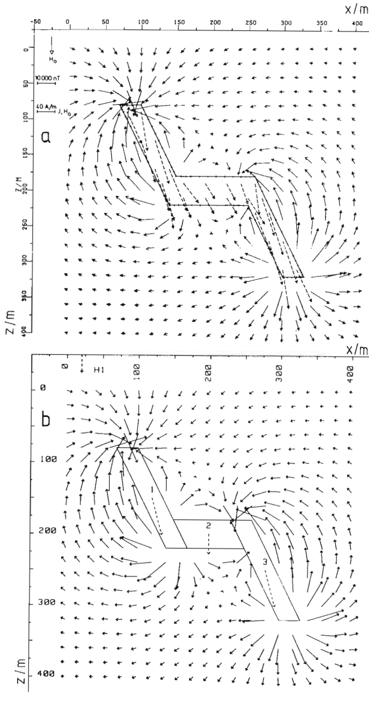
Figure 26.7 (left)-26.8 (right) Magnetic anomaly field vectors maps of some models computed a) by the method of subsections and b) by the method based on homogeneous magnetization with demagnetization correction. The susceptibility of each model is 4 SI units. The point grid is 20 x 20 m. (Avdeyev et al., 1981).
