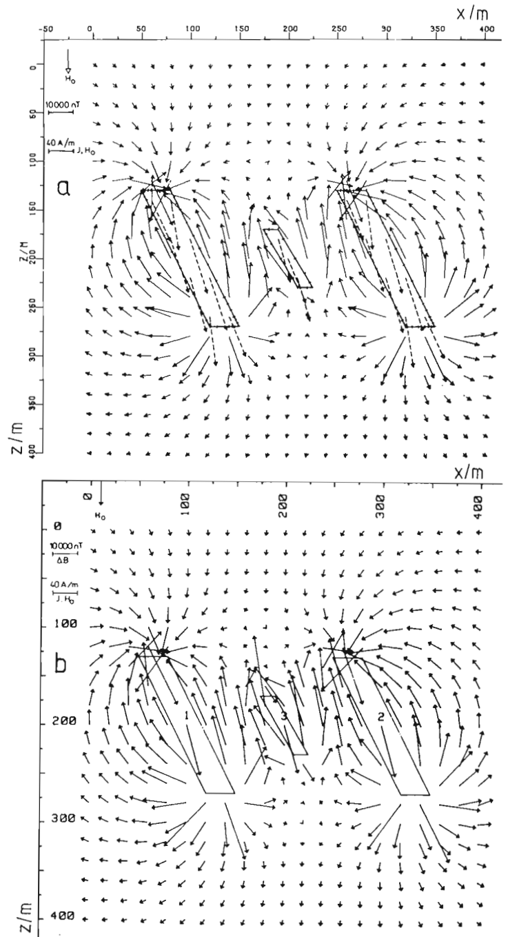
Figure 26.7 (left)-26.8 (right) Magnetic anomaly field vectors maps of some models computed a) by the method of subsections and b) by the method based on homogeneous magnetization with demagnetization correction. The susceptibility of each model is 4 SI units. The point grid is 20 x 20 m. (Avdeyev et al., 1981).
