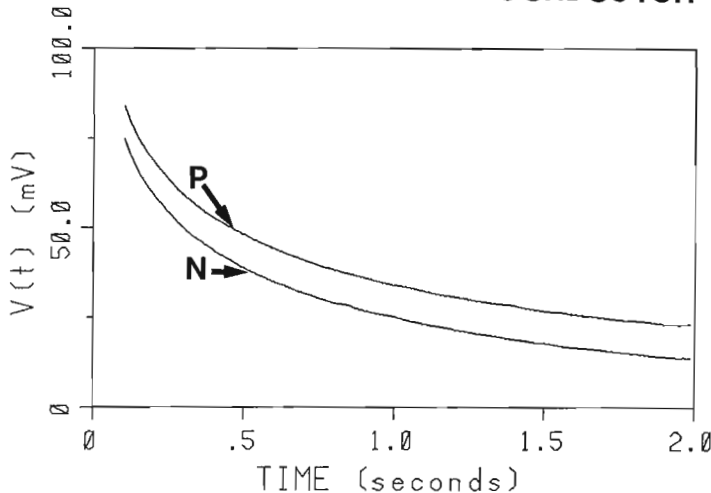
Figure 15.10. IP decay curves observed outside and inside the energized sulphide conductor illustrating that the IP is not completely reversible with polarity reversal of the charging current. The decay curves for the negative charging current are inverted for ease of comparison.
