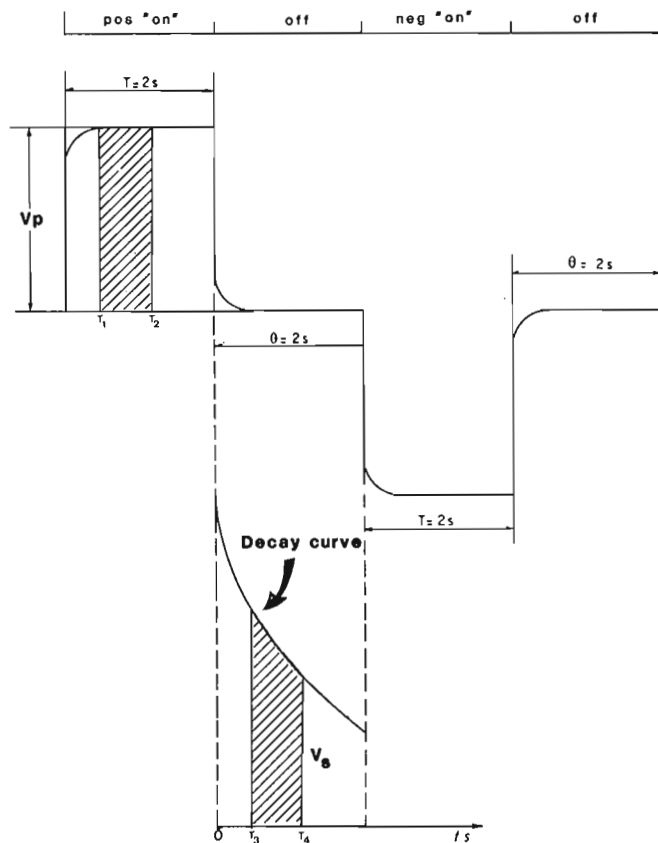
Figure 2.5. Typical Newmont type IP and resistivity waveform consisting of a T second positive polarity current pulse 'on' time, a second 0 current 'off' time, a T second negative polarity 'on' time and a second 0 'off' time where T and 0 are set to 2 s. The primary voltage is obtained from the area between T_1 (0.45T) and T_2 (0.85T). The secondary voltage is obtained from the area between T_3 (0.280) and T_4 (0.50). V_p is used in the calculation of resistivity and V_s is used in the calculation of IP (after Bertin and Loeb, 1976).
