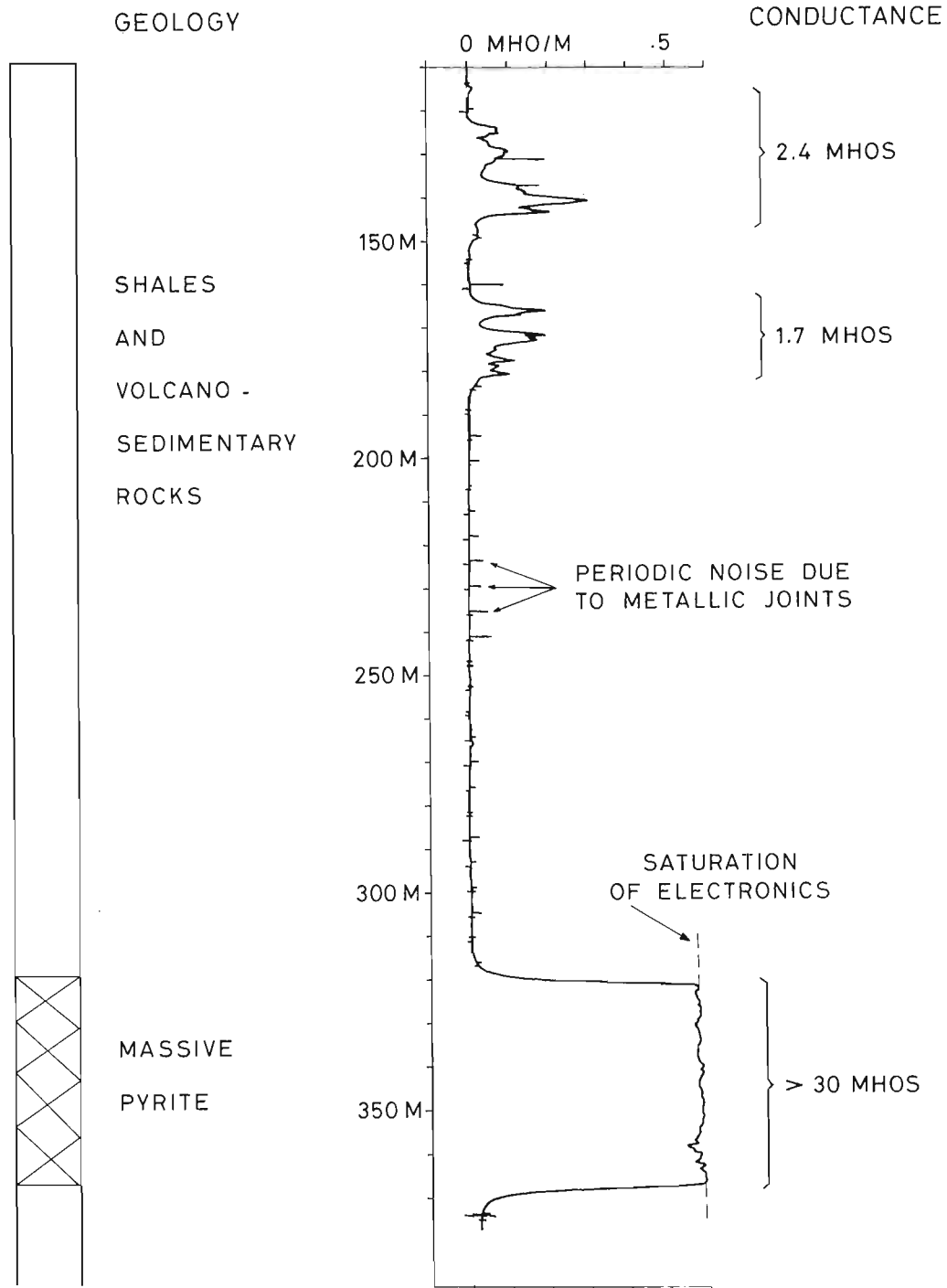
Figure 10.7. Example of ROMULUS conductivity log in hole 1 intersecting a thick massive pyrite zone surrounded by volcano-sedimentary cover. Conductance contrast between mineralization ( > 30 mhos) and graphitic shales (2.4 mhos, 1.7 mhos) suggests that remote detection of the ore body by EM or resistivity techniques is possible from the surface.
