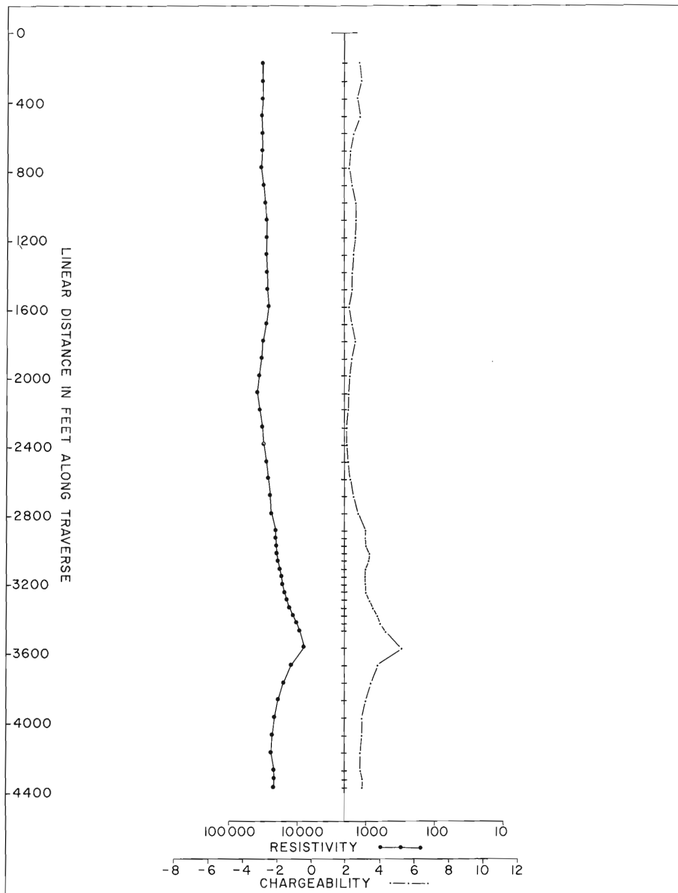
Figure 2. Modified Schlumberger array with one pole starting in B.H.'A' at 100 feet and a second pole starting in B.H.'B'. at 250 feet using north-south current line.
