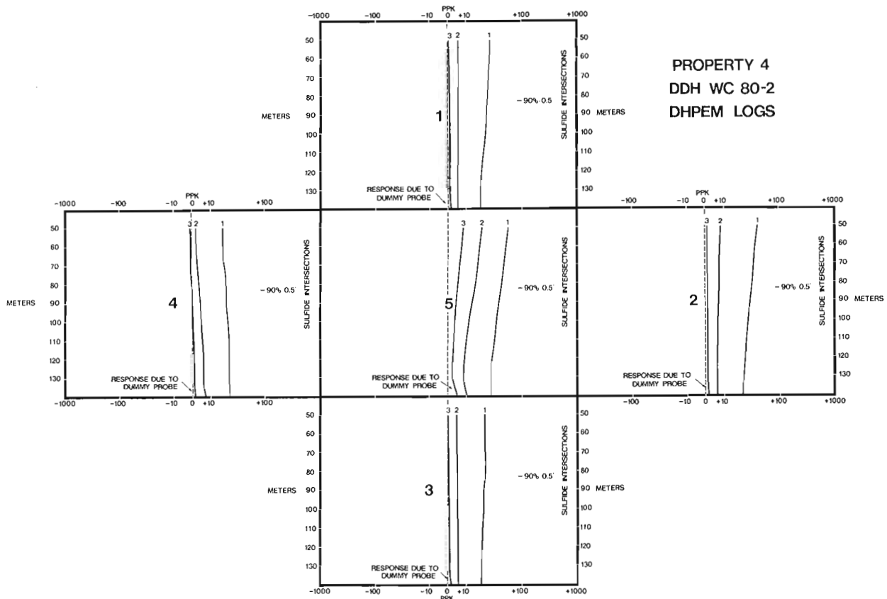
Figure 25. Property 4: DHPem logs in WC-80-2.
