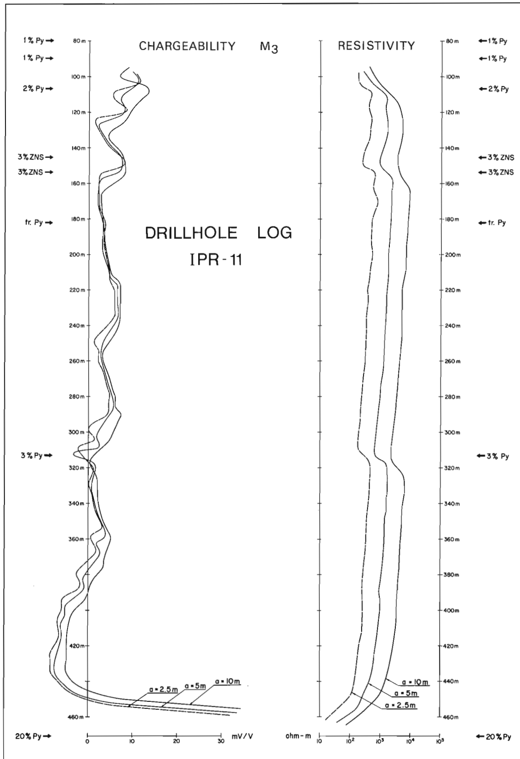
Figure 12.6. Near-hole results ('a' spacing 2.5 m, 5 m, and 10 m) for drillhole IP logging of the Nanasiv carbonate hosted lead-zinc deposit.
