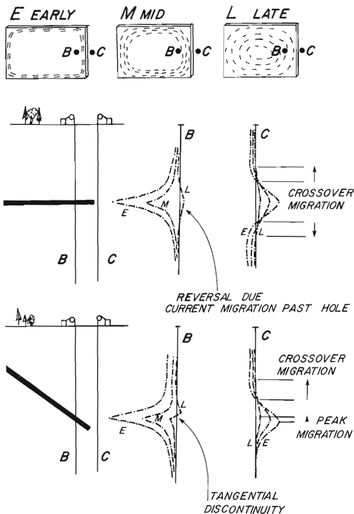
Figure 35.4. In time domain EM systems with step or pulse excitation the induced currents at early delay times are concentrated at the edges of a conductor, and spread inwards with time at the same time as their amplitude decreases. The effects of this current migration on measured axial component borehole data are schematically shown here.
