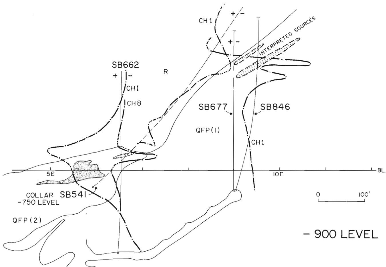
Figure 34.4. -900 level. The line of the drillholes, along with their electromagnetic data profiles are projected to the plane of the level. Profile scale is in Figure 34.5. CH1 and CH8 are channels 1 and 8, R - rhyolite, QFP(1) - quartz-feldspar porphyry, QFP(2) - altered quartz-feldspar porphyry. Fine stippled units are massive sulphides. Coarse stippled units are bodies interpreted from the PEM data.
