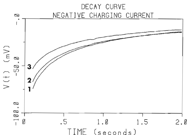
Figure 15.9. IP decay curves for the positive and negative charging currents. The curves correspond to the off-cycle voltages of the waveforms presented in Figure 15.8.
