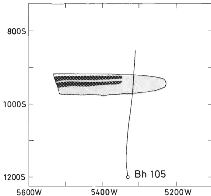
Figure 9.16. Horizontal projection of the interpreted situation around Kankberg Bh 105. The alteration zone is shaded and the structures of high conductivity are black.
