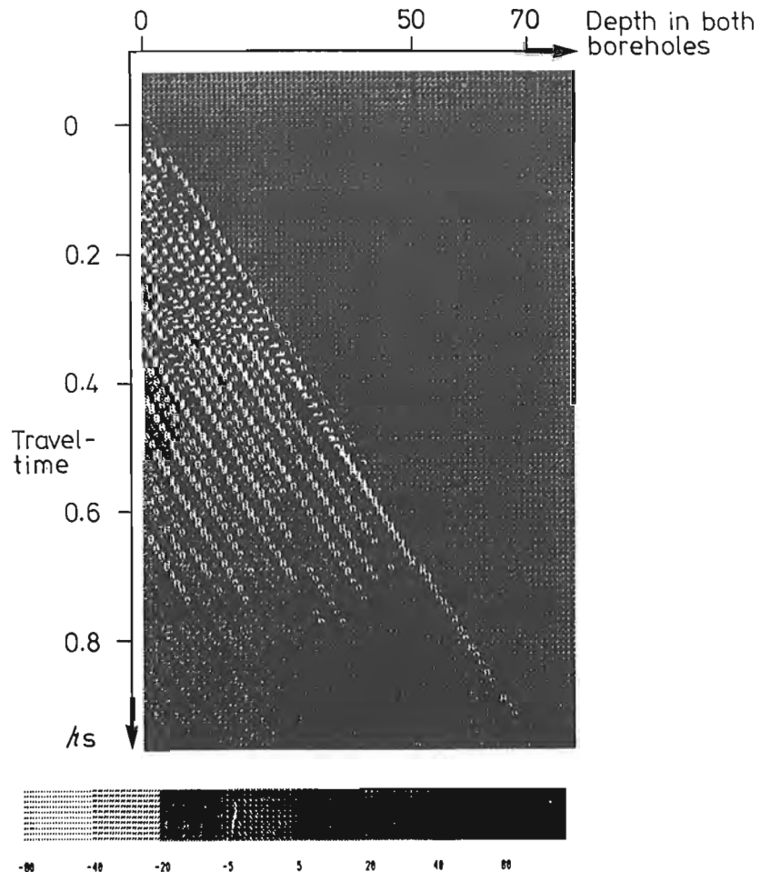
Figure 22.7. Radar plot from the crosshole measurement between E1 and N1 in Stripa.
