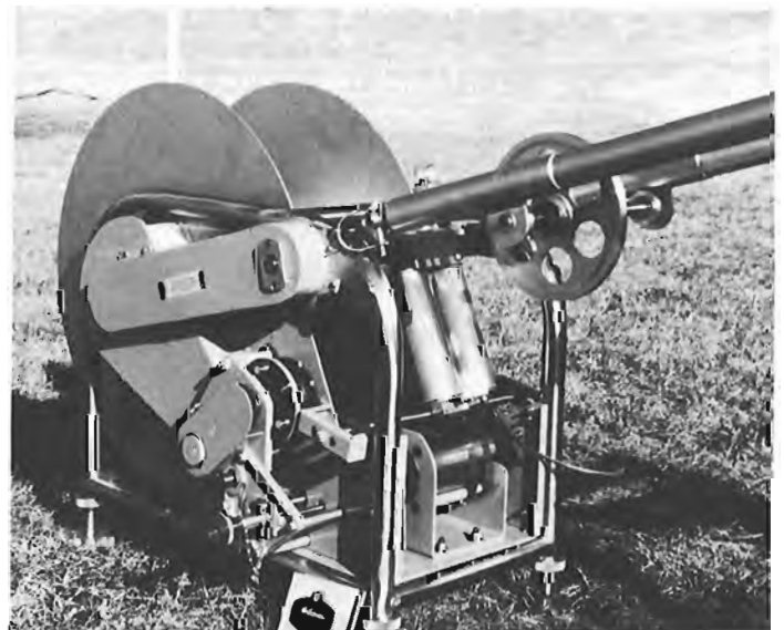
Figure 11.4. The winch. (GSC 203811)
