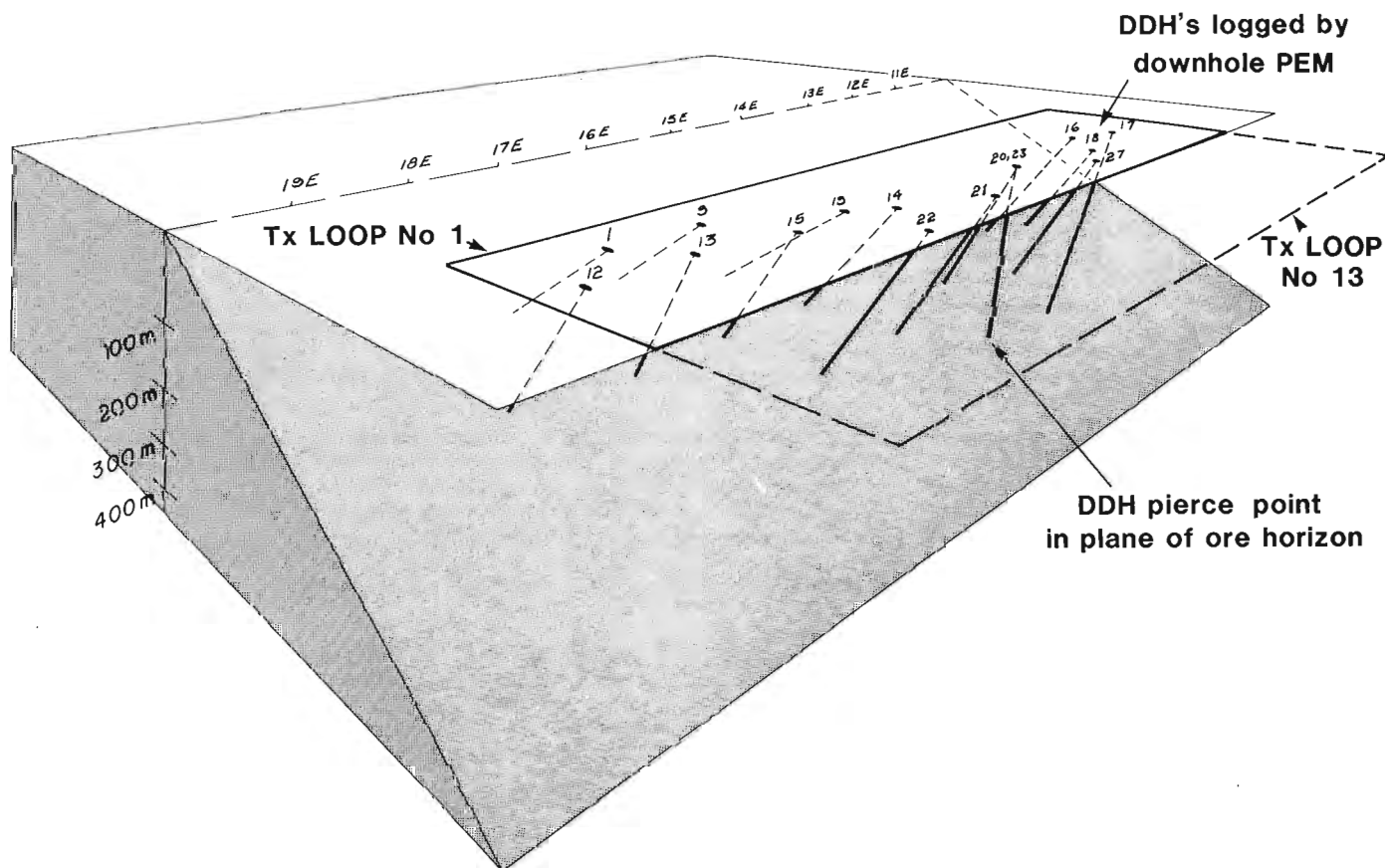
Figure 33.2. Schematic showing transmitter loop locations relative to the diamond drill holes (DDH) for the Eastmain Project.
