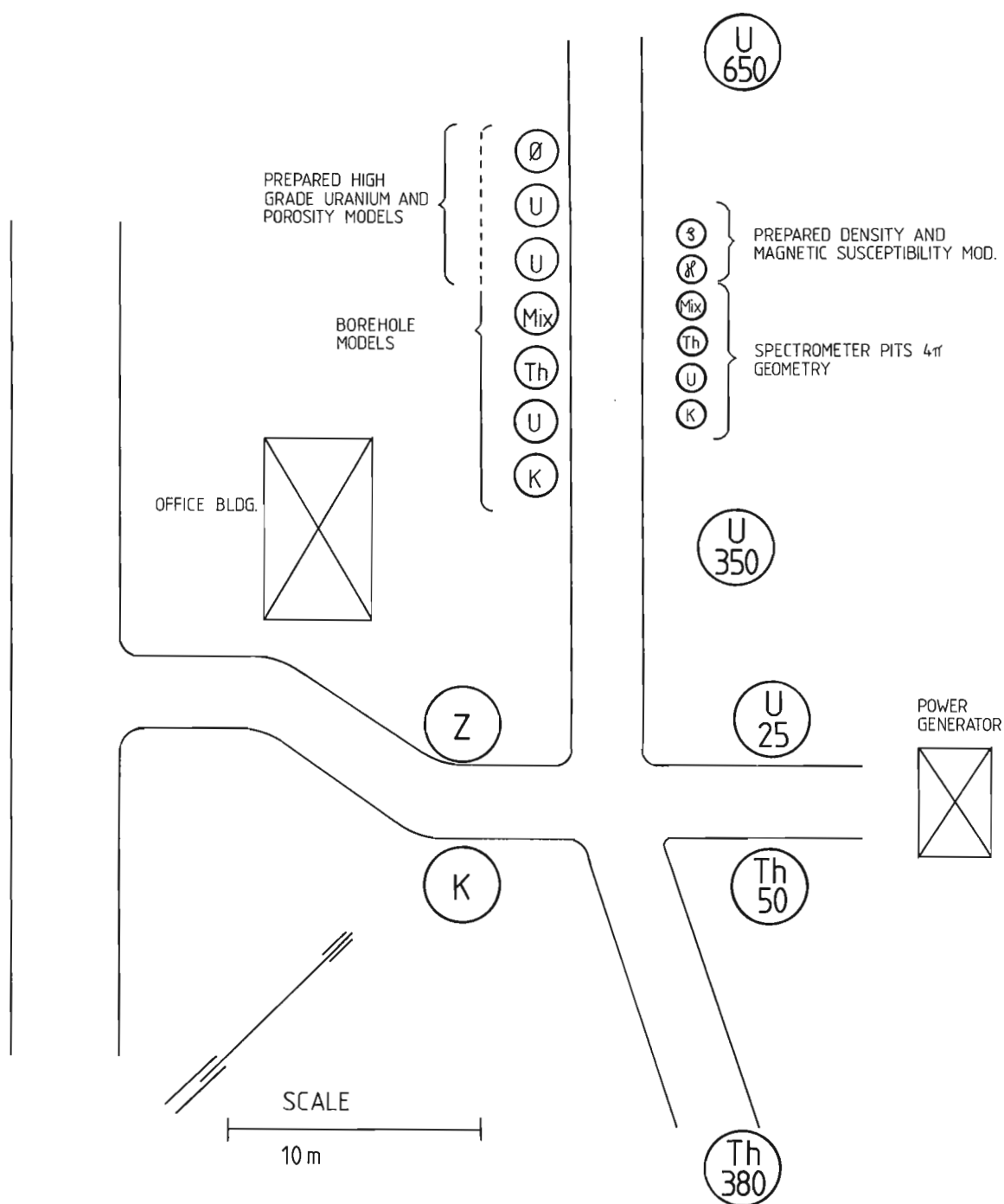
Figure 5.1. Calibration facilities at Malå, Sweden.
