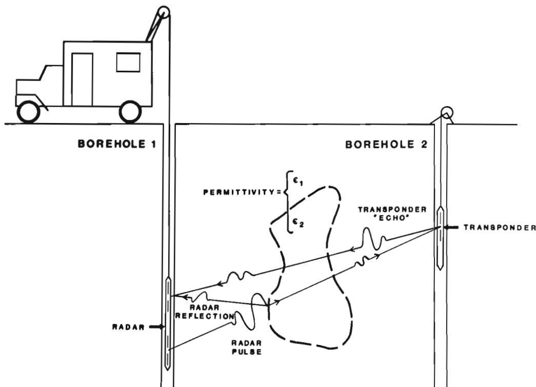
Figure 23.10. A borehole transponder extends the capability of a short-pulse radar system so that both single-hole and crosshole data may be acquired simultaneously. Since the transponder transmits when it senses a signal incident from the radar, the requirement for a timing cable in the transponder borehole is eliminated.
