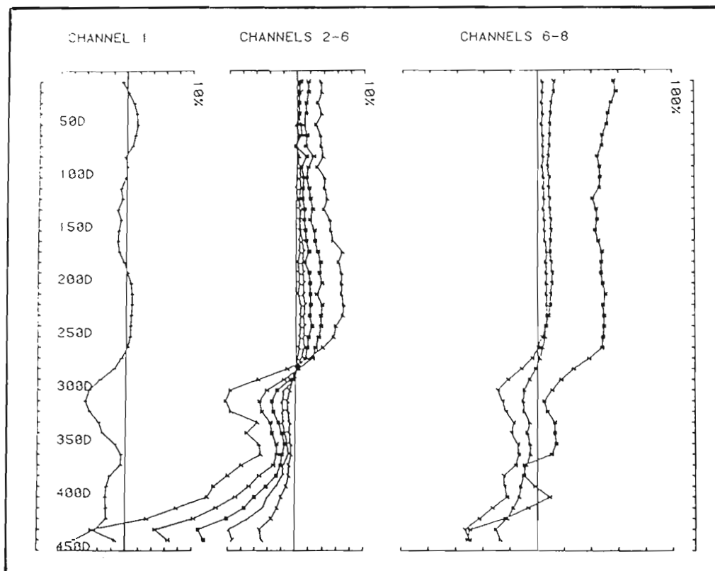
Figure 11.6. Results from the first test logging using the UTEM system.
