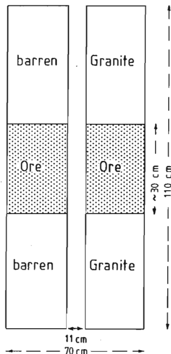
Figure 4.1. Model borehole with ore-mix between two barren zones. Material compounds and mixing ratios are indicated.
