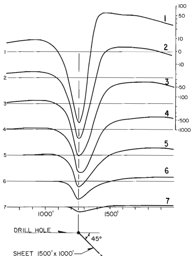
Figure 34.6. PEM model response profiles (after Woods, 1975, p. 205), in a hole passing a body at its top edge. For model data, the amplitude scale in the upper right hand corner gives the induced voltage in microvolts at the receiver.
