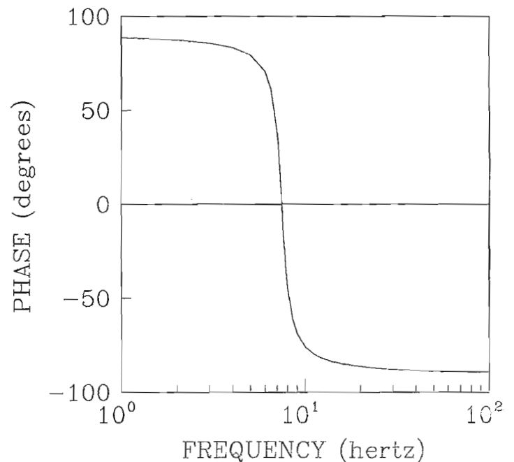
Figure 32.3b. Bode plot of the first stage.
