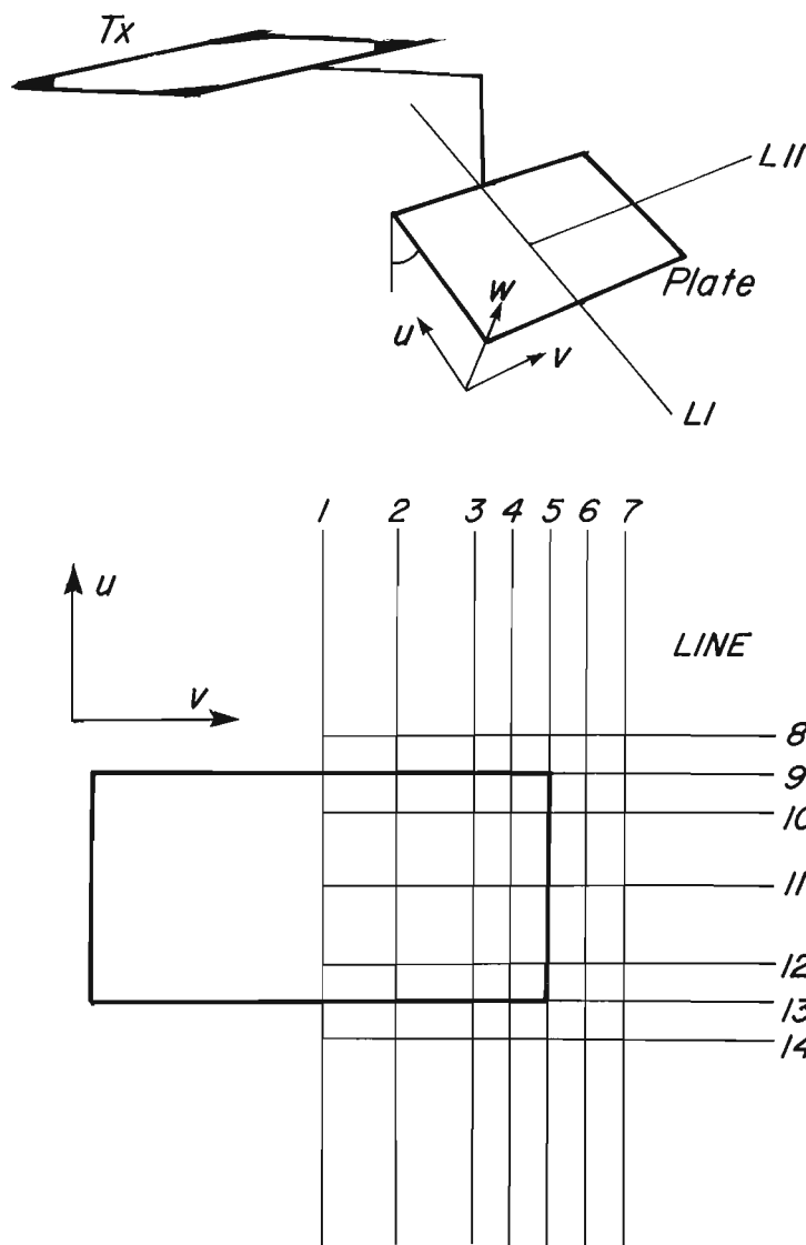
Figure 35.7. Scale model geometry. Profiles were measured over half the u - v plane on 14 survey lines.
