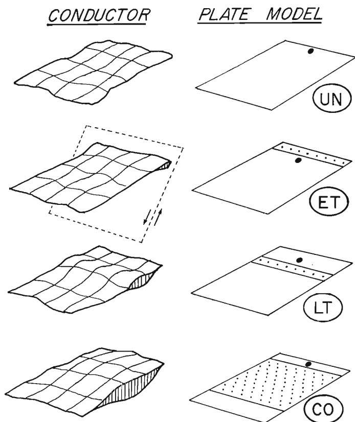
Figure 35.6. Four geological models and corresponding thin plate conductors, from top to bottom Uniform, Edge Thickened, Locally Thickened and Conductive Core.
