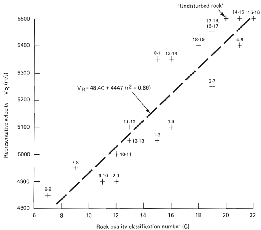
Figure 19.7. Correlation of representative velocity with rock quality classification.
