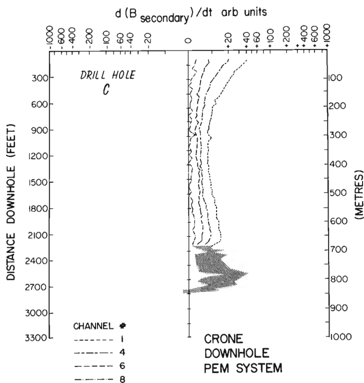
Figure 32.7. Plots of Crone Pulse EM data collected previously for the same drillholes.
