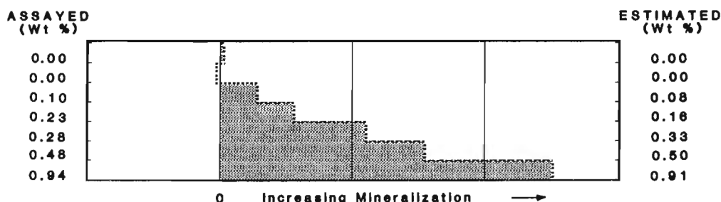
Figure 30.4. Tungsten and molybdenum mineralization plots calculated from spectra of calibration samples. The tick marks on the vertical axes of the plots show the ranges for each of the calibration samples. The assayed weight percentages (wt%) are listed on the left and the estimated weight percentages from the calibration curves (Fig. 30.3) are listed on the right. The mineralization trace is shown as a dashed line and the positive areas under the trace are shaded. The amplitudes of the horizontal deflections are proportional to the relative mineral concentrations.
