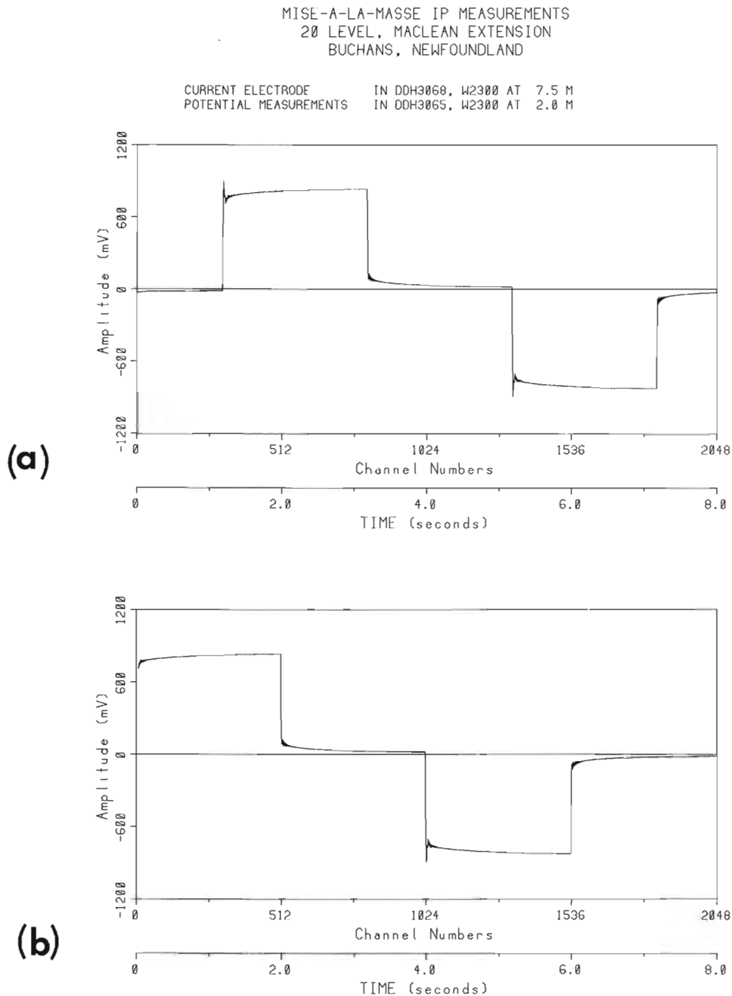
Figure 15.5. Typical time domain complete IP waveform recording with the Huntect IP system. (a) voltage waveform as recorded on cassette tape of the Huntect M4 receiver. (b) rearranged waveform with the onset of the positive current-on time at the beginning of the cycle.
