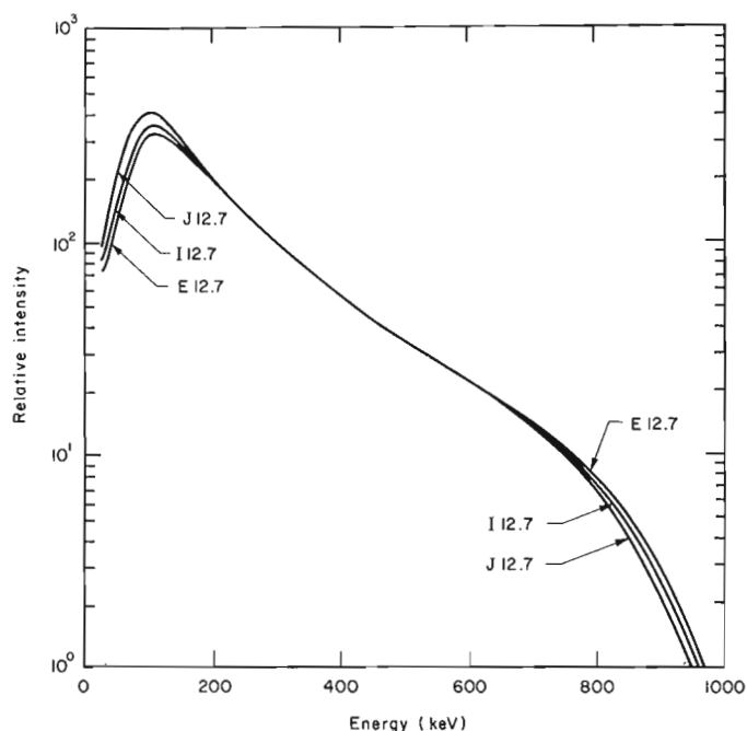
Figure 29.7. Backscattered spectra of ^{60}\text{Co} gamma rays in borehole models E12.7, I12.7 and J12.7 normalized to the same intensity at 300 keV.
