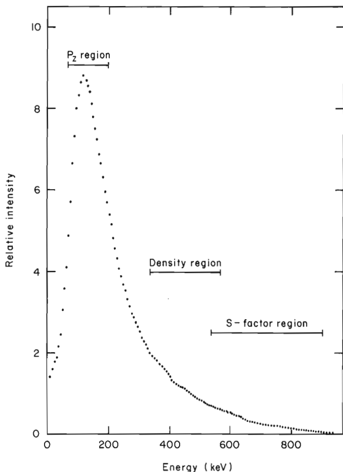
Figure 29.1. Typical backscattered spectrum of ^{60}\text{Co} gamma rays obtained in a borehole of 13 cm diameter.
