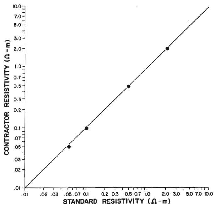
Figure 23. Fluid resistivity bridge field calibration check, indicating good calibration.
