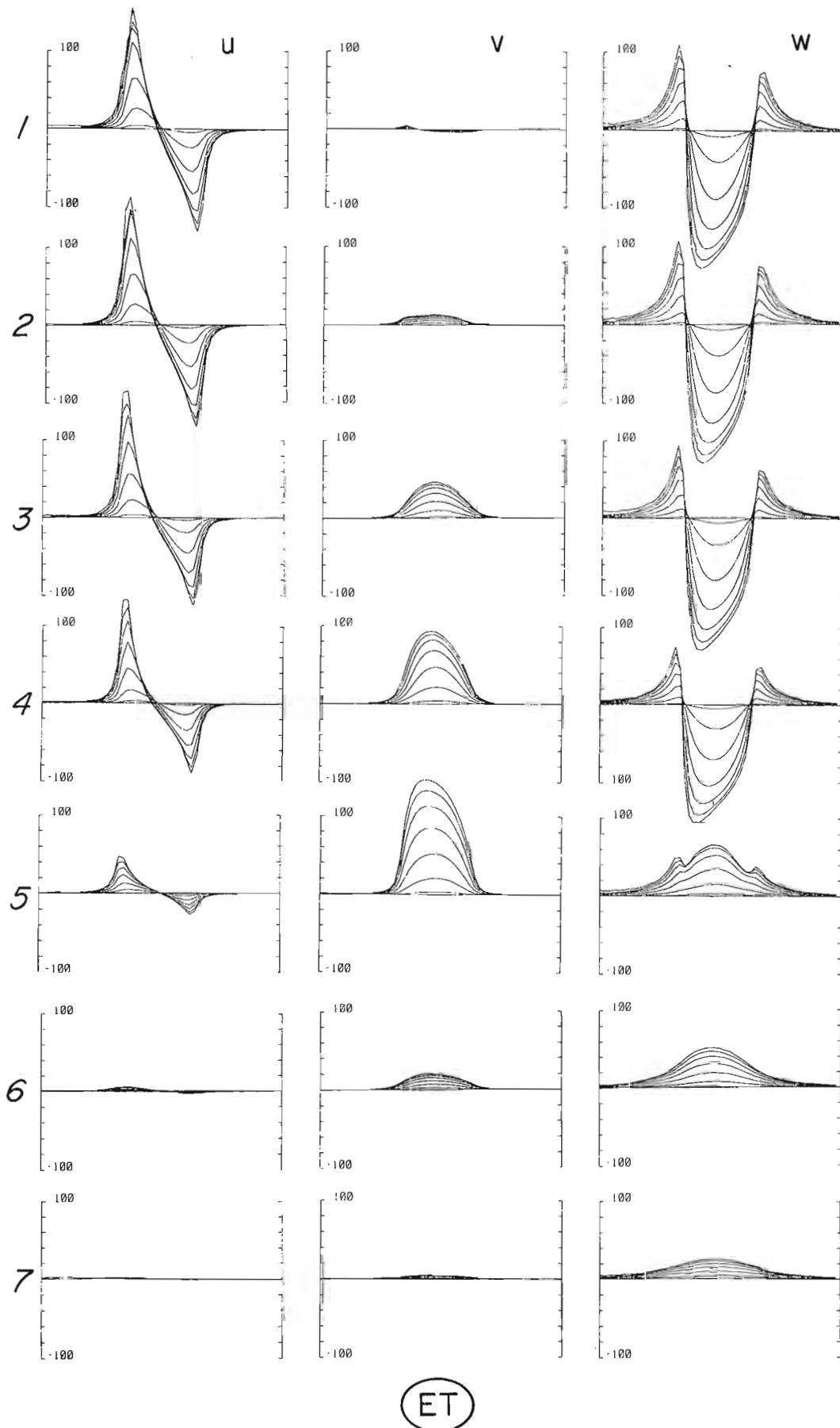
Figure 35.12. UTEM response across the edge thickened conductor.
