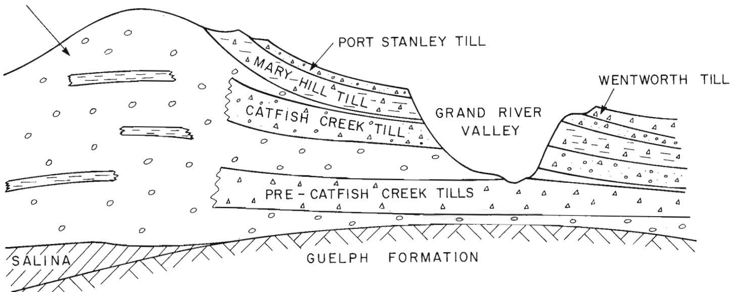
Figure 1.2. Schematic cross-section showing overburden stratigraphy from West (left) to East (right) on a line passing through the Greenbrook well field in Figure 1.1.
