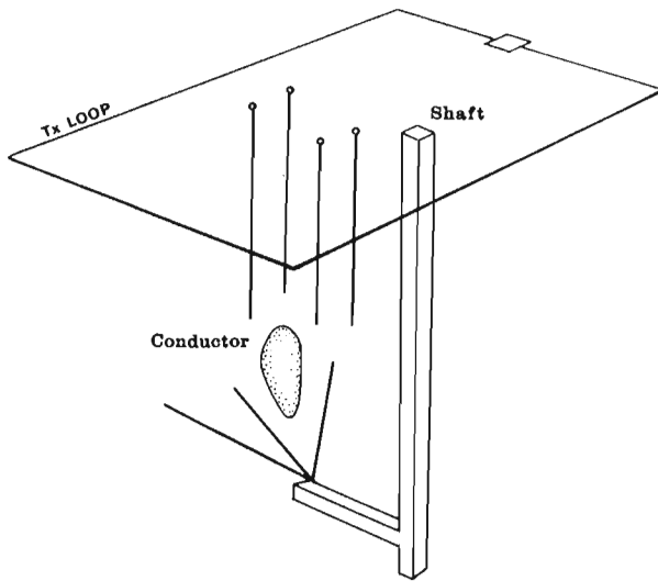
Figure 7.1. Large transmit loop borehole PEM system used for surveying a group of drillholes from surface or underground. The position of a conductor is determined from the response obtained from adjacent holes.
