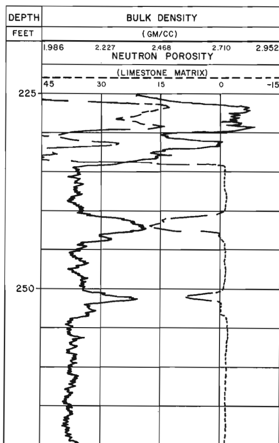
Figure 17. Neutron log halite signal.
