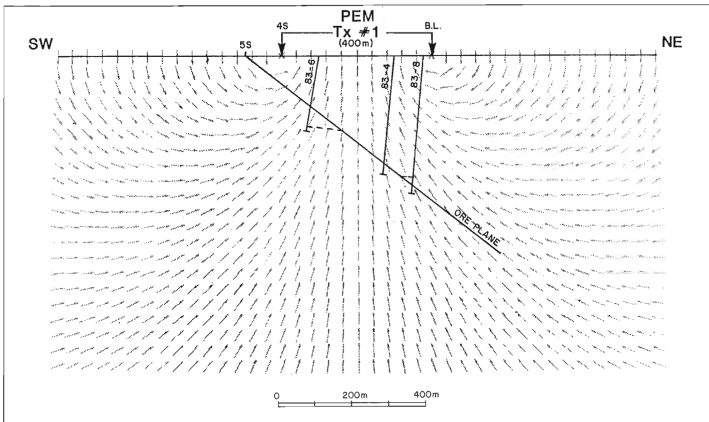
Figure 33.3. Typical pulse EM section showing transmitter no. 1 (Tx no. 1) and coupling of the field lines with the ore plane.
