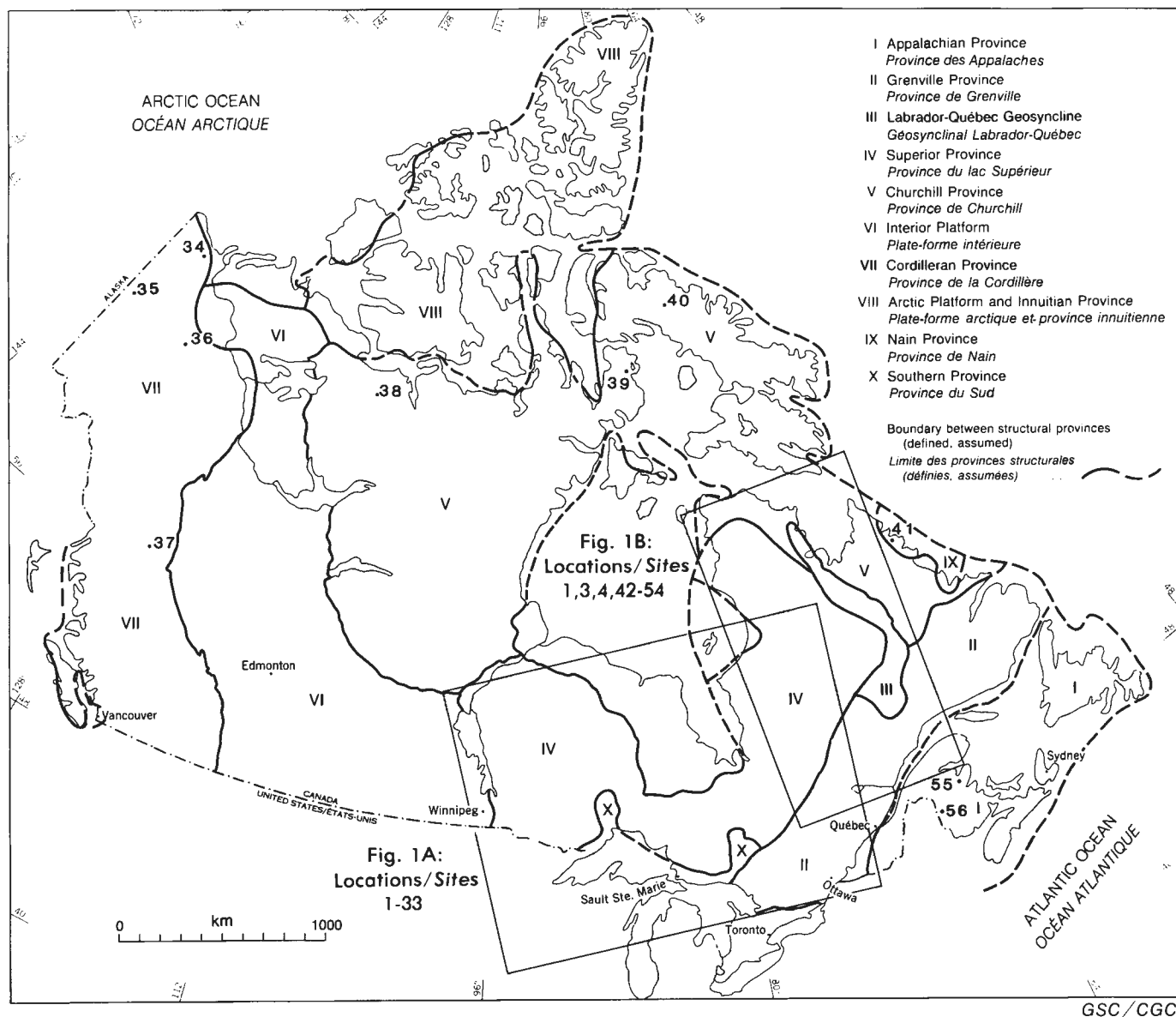
Figure 1. Iron-formations in Canada. Numbers refer to iron-formations identified in Table 1. Figure 1A includes localities 1 to 33, Figure 1B includes localities 1, 3, 4, 42-54.
