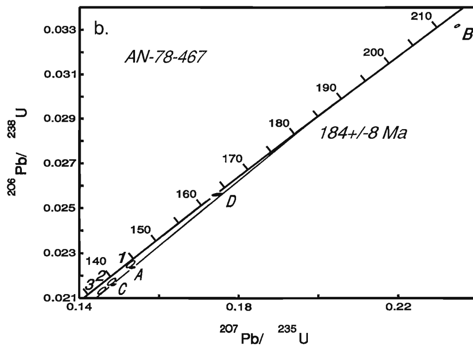
Figure 3. (a) U-Pb concordia plot for Cake Hill Pluton quartz monzonite. (b) U-Pb concordia plot for McBride River granodiorite. Fractions 1, 2, and 3 are from Anderson et al. (1982).
