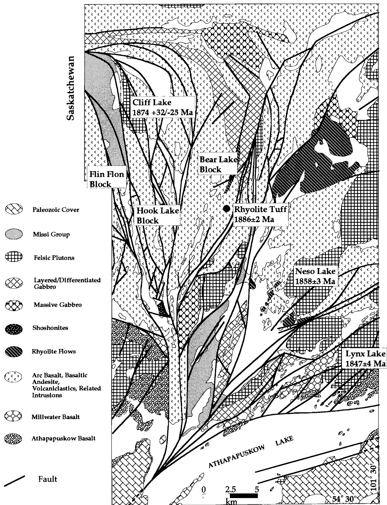
Figure 2. Geology of part of the Flin Flon metavolcanic belt in Manitoba, showing some of the fault-bounded blocks (after Bailes and Syme, 1989; Syme, 1988). References to age determinations are as follows: Lynx Lake pluton, Cliff Lake pluton, rhyolite tuff (Gordon et al., 1990); Neso Lake pluton (Syme et al., 1991).
