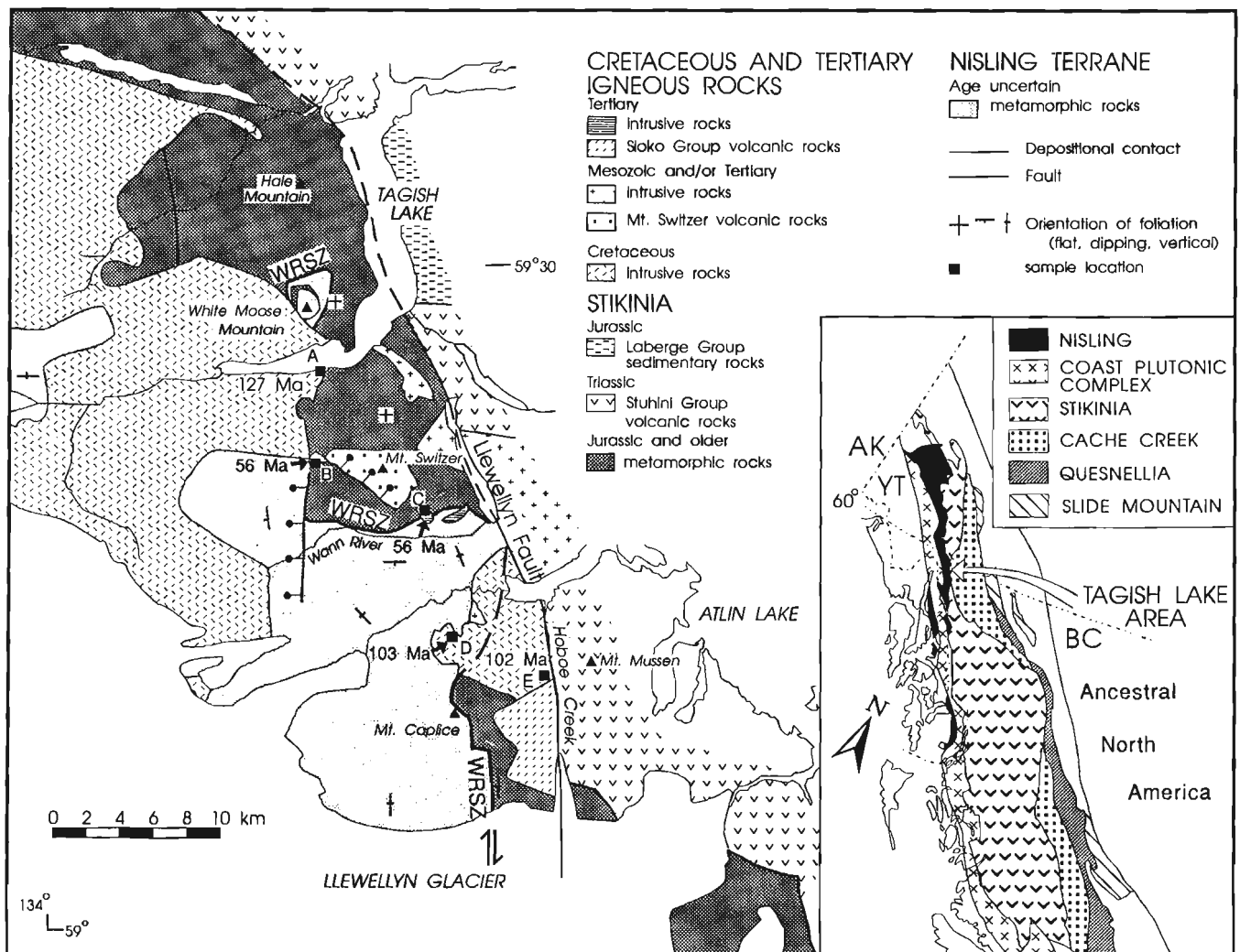
Figure 1. Geological map of the Tagish Lake area showing locations of samples discussed in the text: A, LC-89-35c; B, LC-89-75; C, LC-89-175c; D, LC-90-359; and E, LC-90-261c). Geology is based on Mihalynuk et al., 1989, 1990; Currie, 1990, 1991, 1992). The Wann River shear zone (WRSZ) forms the boundary between Nisling terrane and Stikinia. Inset shows the location of Nisling terrane and adjacent terranes (modified from Wheeler et al. 1991). AK - Alaska, BC - British Columbia, YT - Yukon Territory.
