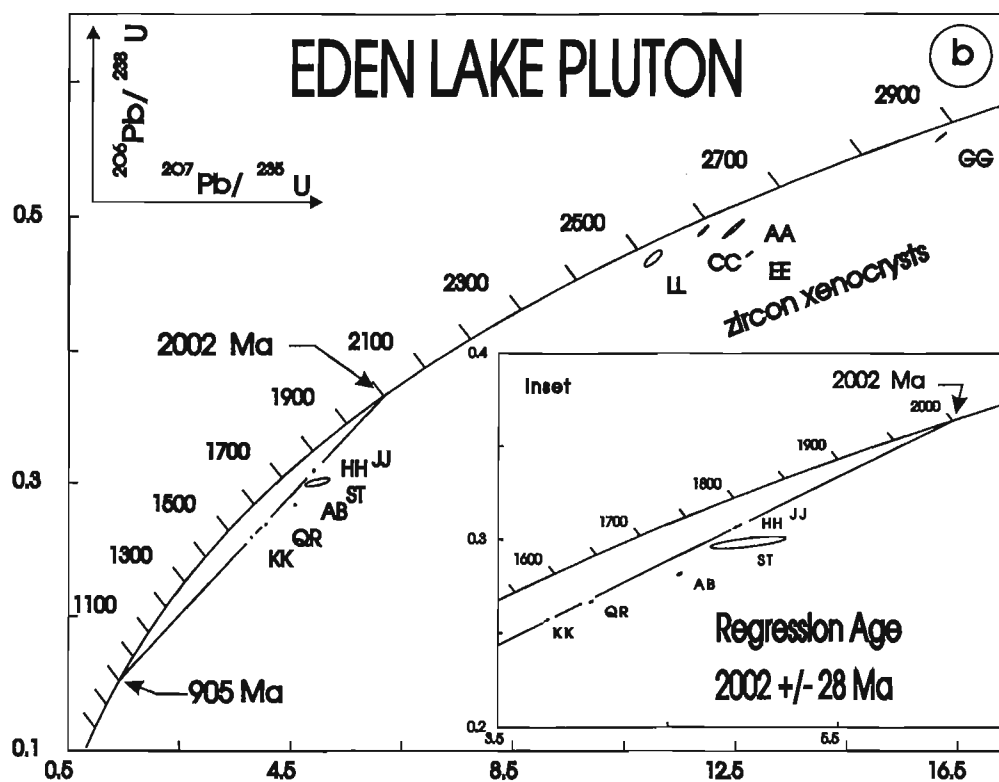
Figure 2. Concordia diagrams for plutons in the Southern Province: a , the Cutler batholith; b , Eden Lake pluton.
