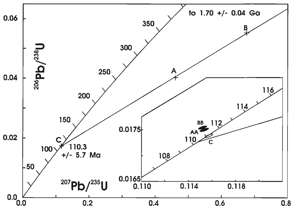
Figure 2. U-Pb concordia plot for zircons (open) and monazites (solid) from the biotite orthogneiss unit.
