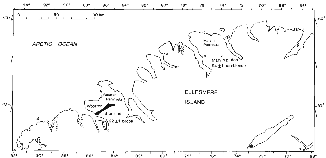
Figure 21. Dated Cenomanian intrusions, northern Ellesmere Island.
