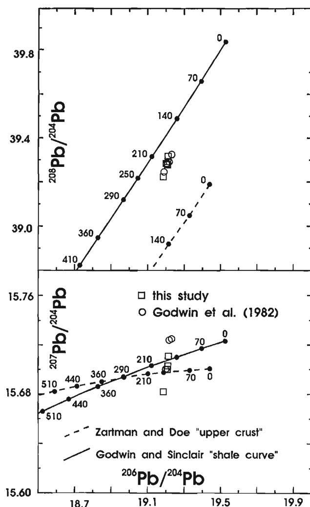
Figure 3. Pb isotopic compositions for galenas from epigenetic mineralization in the northeastern Anvil Range. Crustal growth curves (with ages shown in Ma) are from Zartman and Doe (1981) and Godwin and Sinclair (1982).
