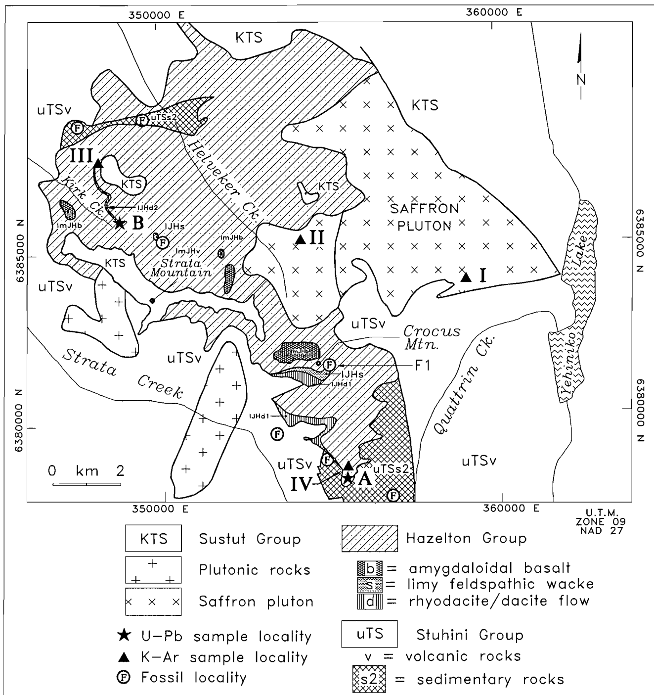
Figure 2. Simplified geology of the study area. U-Pb and K-Ar dating localities are numbered A and B and I to IV, respectively. Geology from Brown et al. (1990). Two distinct felsic units are labelled IJHd1 and IJHd2.
