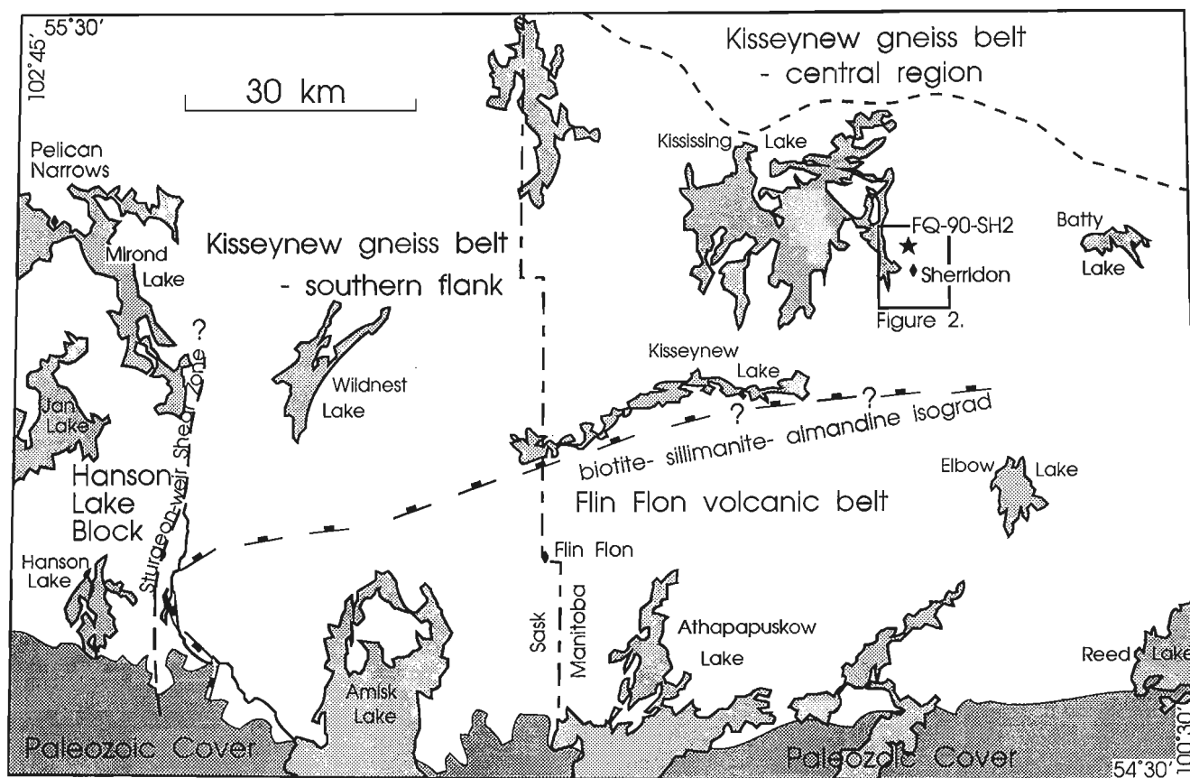
Figure 1. Sketch map of the western Flin Flon volcanic belt and southern flank of the Kisseynew gneiss belt (from Ashton et al., 1992).
