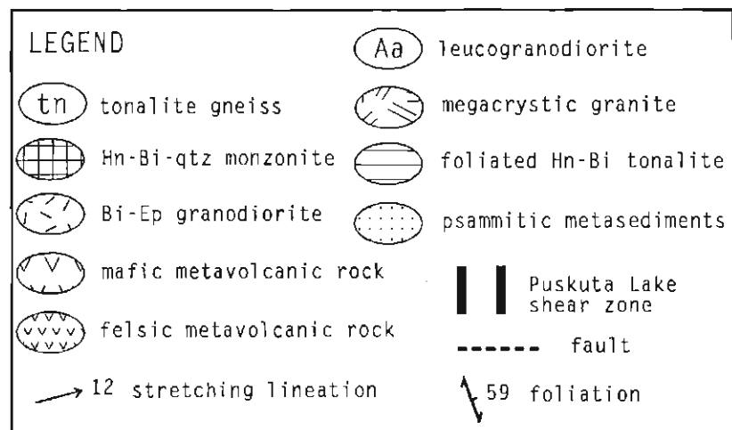
Figure 2. Simplified geological map for the western part of the Kapuskasing-Groundhog-Missinaibi River area (modified from Bennett et al., 1967; Thurston et al., 1977; Leclair, 1992). Geochronology samples are: 1 - granodiorite of the Dishnish batholith (this paper), 2 - granodioritic mylonite of the Puskuta Lake shear zone (this paper; Leclair and Sullivan, 1991) and 3 - leucogranodiorite of the Goat Lake batholith (Leclair and Sullivan, 1991). In the legend Hn = hornblende, Bi = biotite, Ep = epidote and Qtz = quartz.
