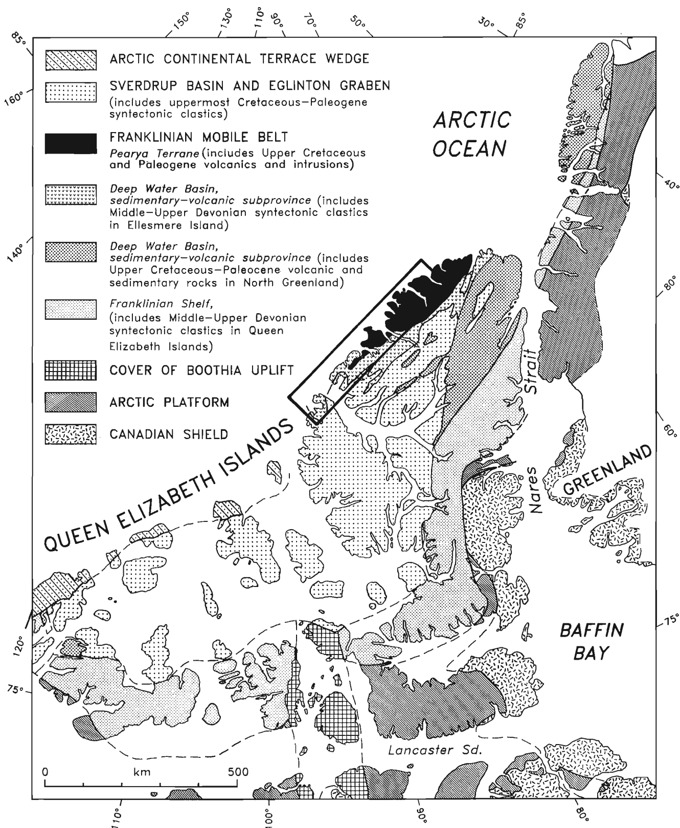
Figure 2. Geological provinces of the Arctic Islands and location of study area.
