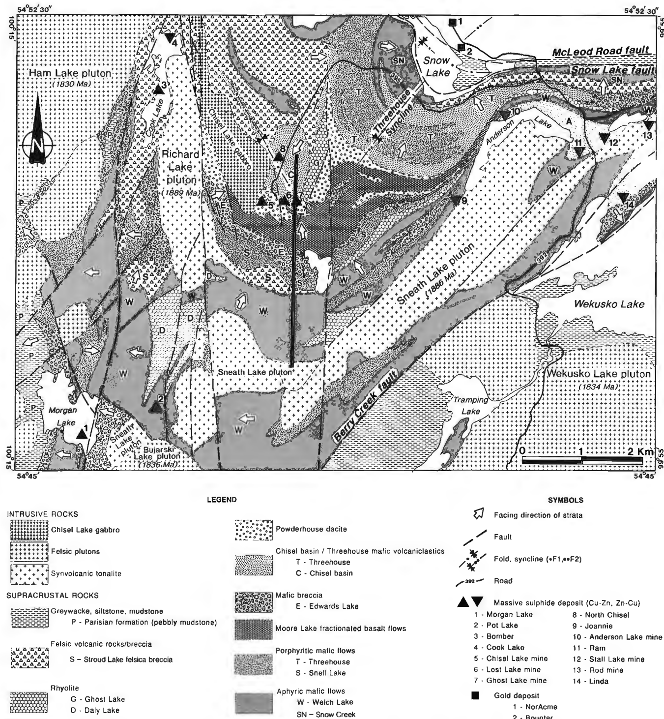
Figure 3. General geology of the Snow Lake area (from Bailes and Galley, 1991). Heavy line marks approximate location of profile shown in Figure 8.
