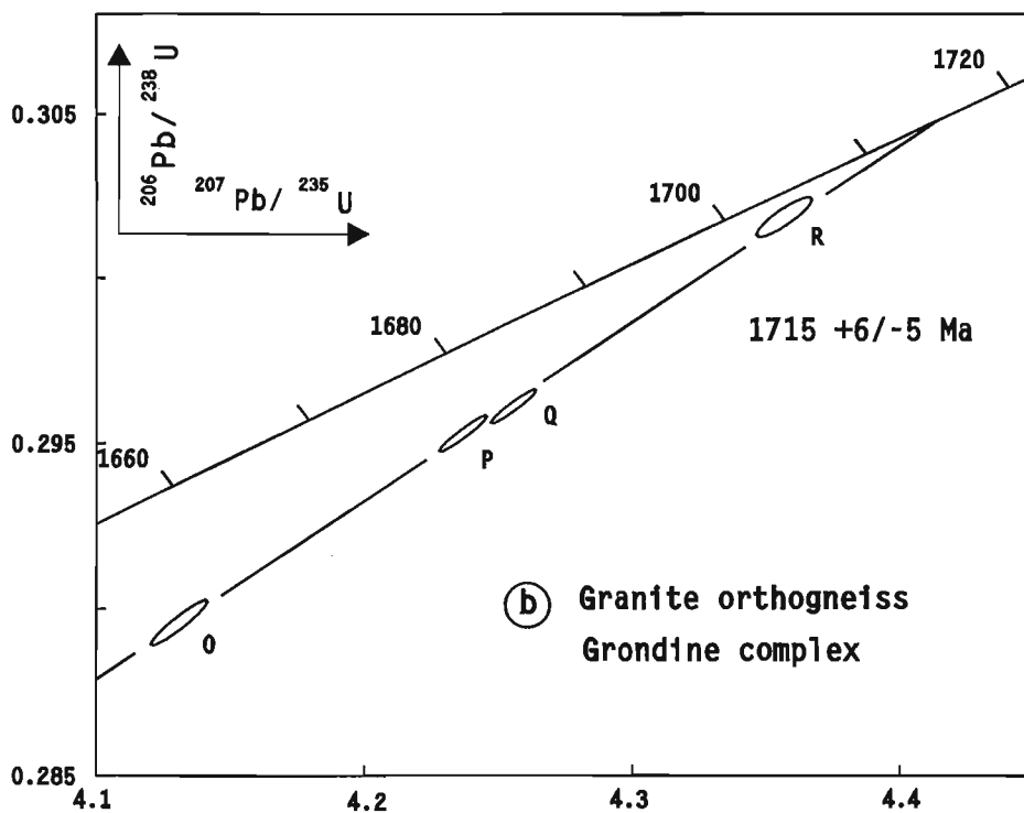
Figure 4. Concordia diagrams for plutons from the Grenville Front Tectonic Zone: a , Fox Islands granite b , granite orthogneiss, Grondine complex; c , quartz dioritic orthogneiss, Grondine complex.
