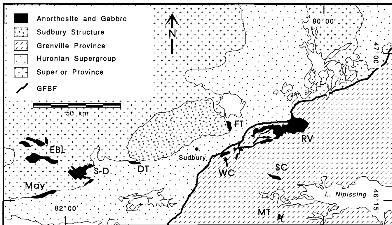
Figure 1. Map of Sudbury area, Ontario, showing gabbro-anorthosite locations (from Ashwal and Wooden, 1989). Abbrev. are GFBF = Grenville Front Boundary Fault; EBL = East Bull Lake; May = May Twp.; S-D = Shakespeare-Dunlop; DT = Drury Twp.; FT = Falconbridge Twp.; WC = Wanapitei Complex; RV = River Valley pluton; SC = St. Charles Anorthosite; MT = Mercer Anorthosite.
