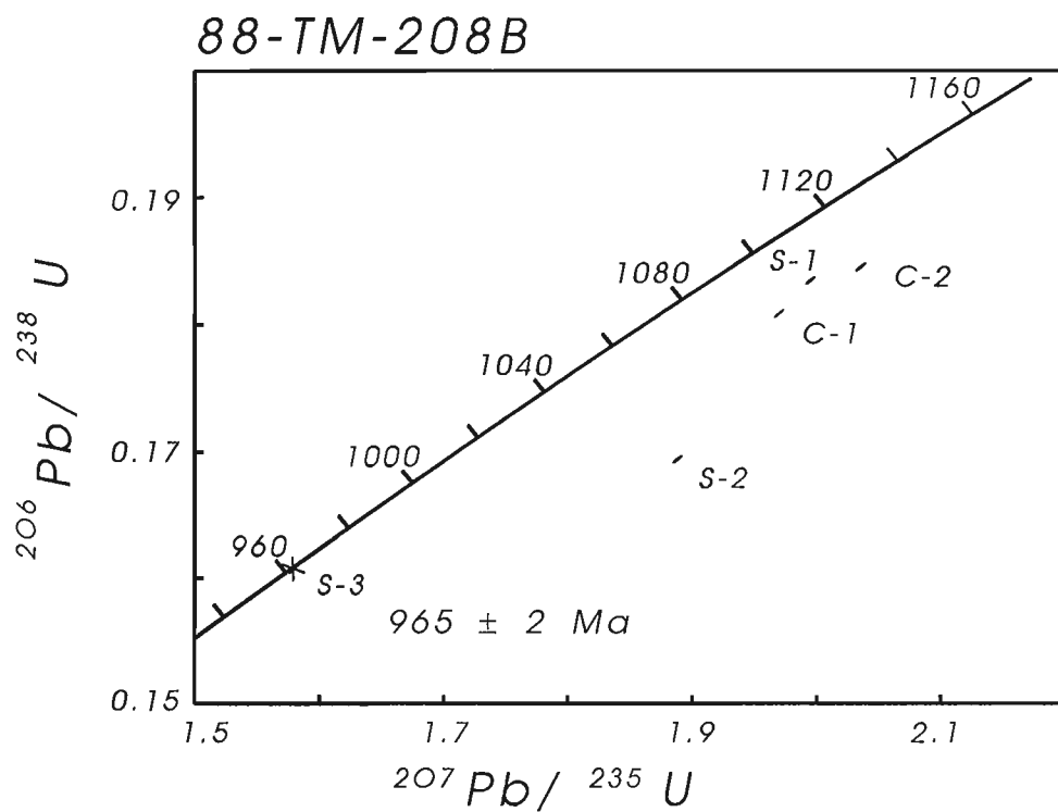
Figure 4. Concordia diagram for Phillips Inlet pluton.
