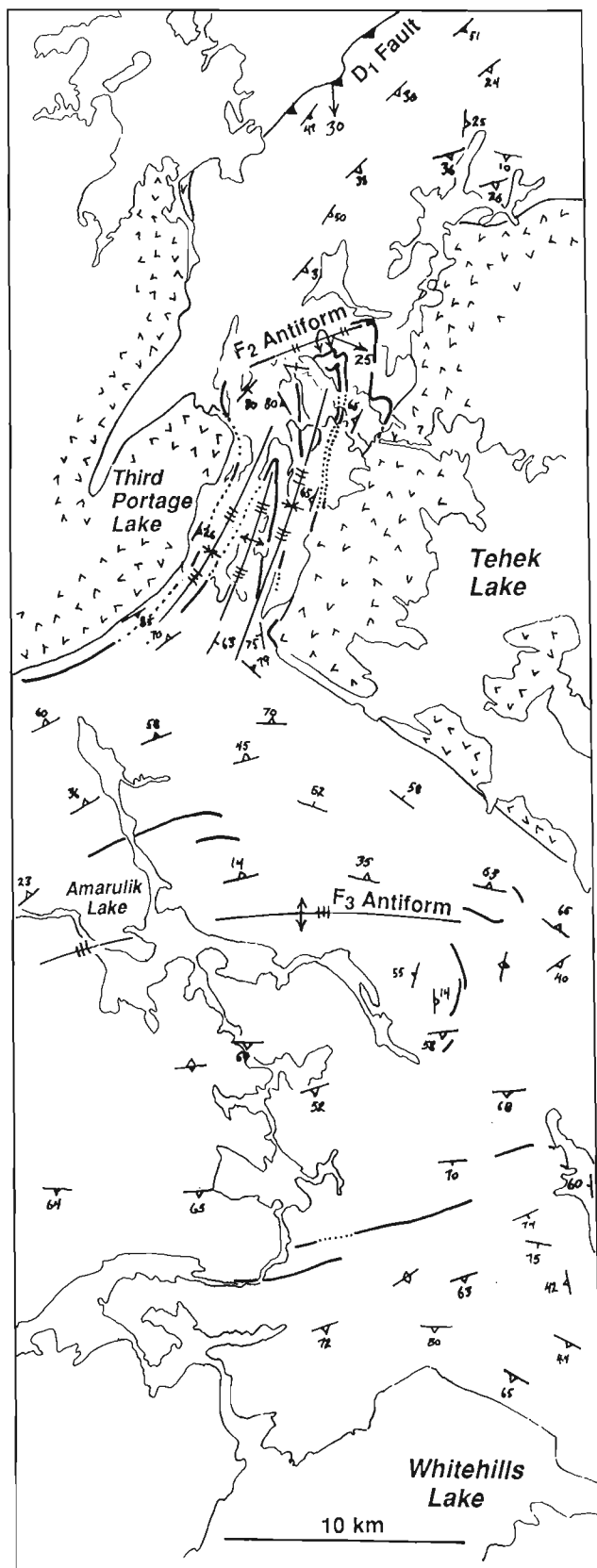
Figure 3. Structural map of the Whitehills-Tehek area showing F2 and F3 fold axial-surface traces, and an inferred D1 low-angle thrust fault. Dotted lines in Third Portage Lake link observed magnetic iron-formation beds that appear to be coincident with aeromagnetic anomalies. Note that both D1 and D2 are northwesterly-vergent, and D3 folds are upright with north-south and east-west trends.
