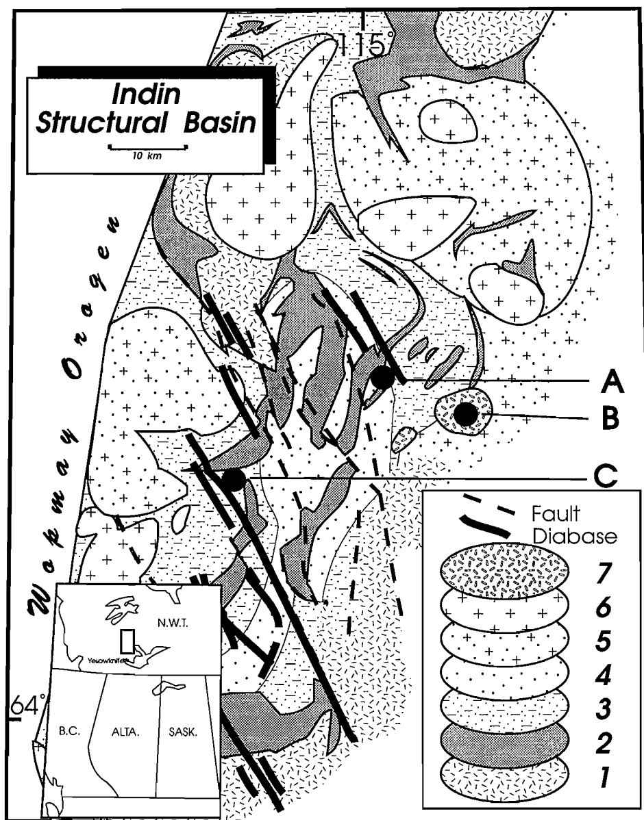
Figure 1. Sketch map of the Indin Structural Basin, western Slave Province showing: (1) the extent of the granitoid basement; (2) the Yellowknife Supergroup volcanic belts; (3) the Yellowknife Supergroup turbiditic greywacke-mudstones (YKS) above the cordierite-staurolite isograd and (4) below the isograd; (5) migmatite derived from 2 and 3; (6) plutonic granites and granodiorites; (7) Proterozoic granodiorite. Site A = this study; B = Frith et al., 1977; C = Wanless et al., 1978.
