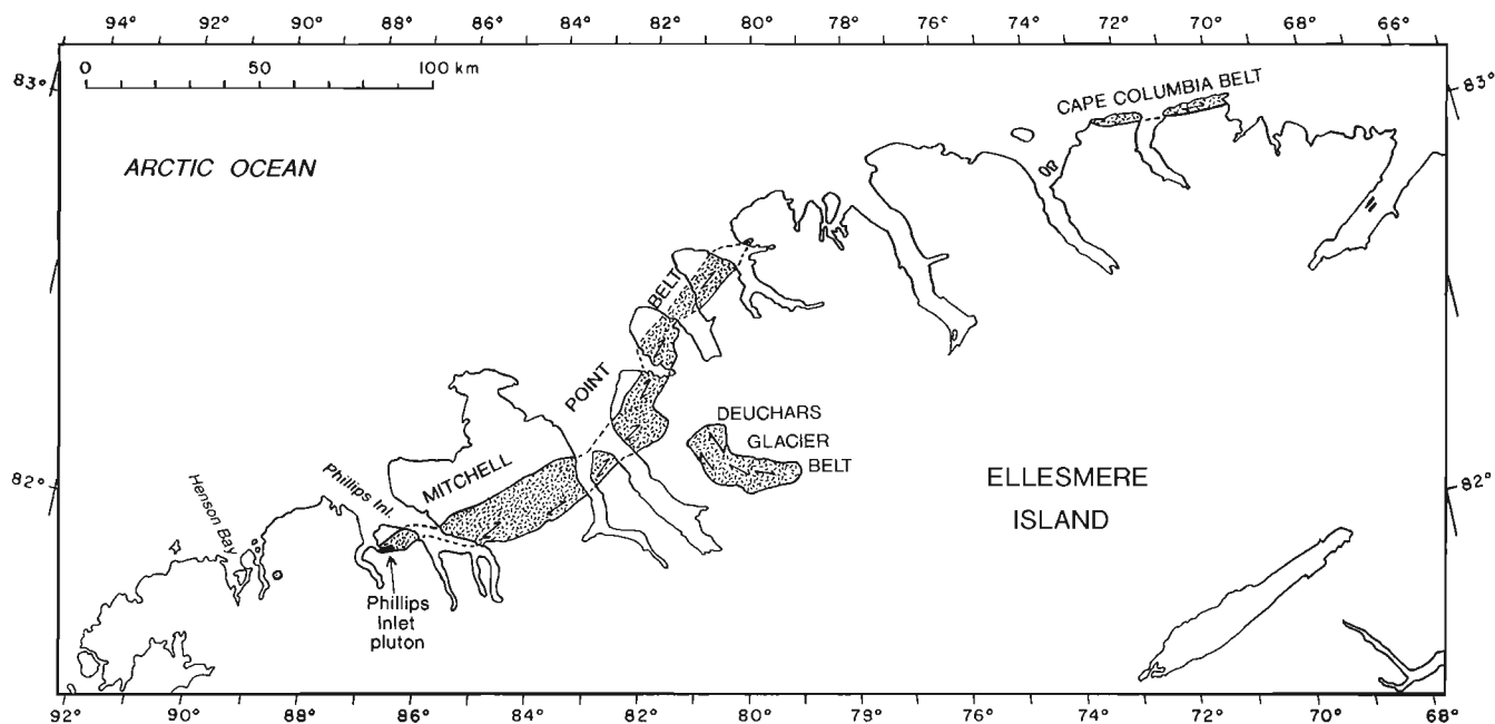
Figure 3. Crystalline basement of Pearya Terrane: generalized outcrop areas, gneissic trends, and location of dated pluton.
