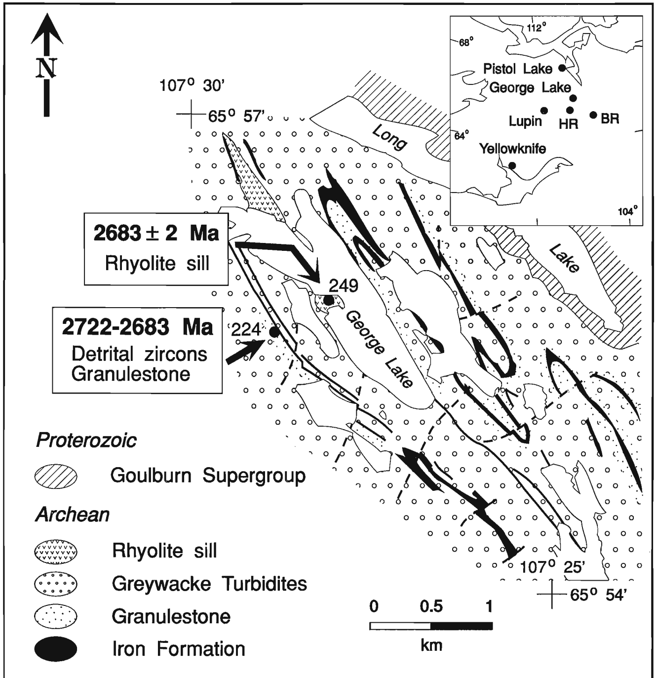
Figure 1. Geology of George Lake area showing localities of samples analyzed: #249, rhyolite; #224, granulestone. Inset: HR – Hackett River, BR – Back River. After Jefferson et al. (1992a).
