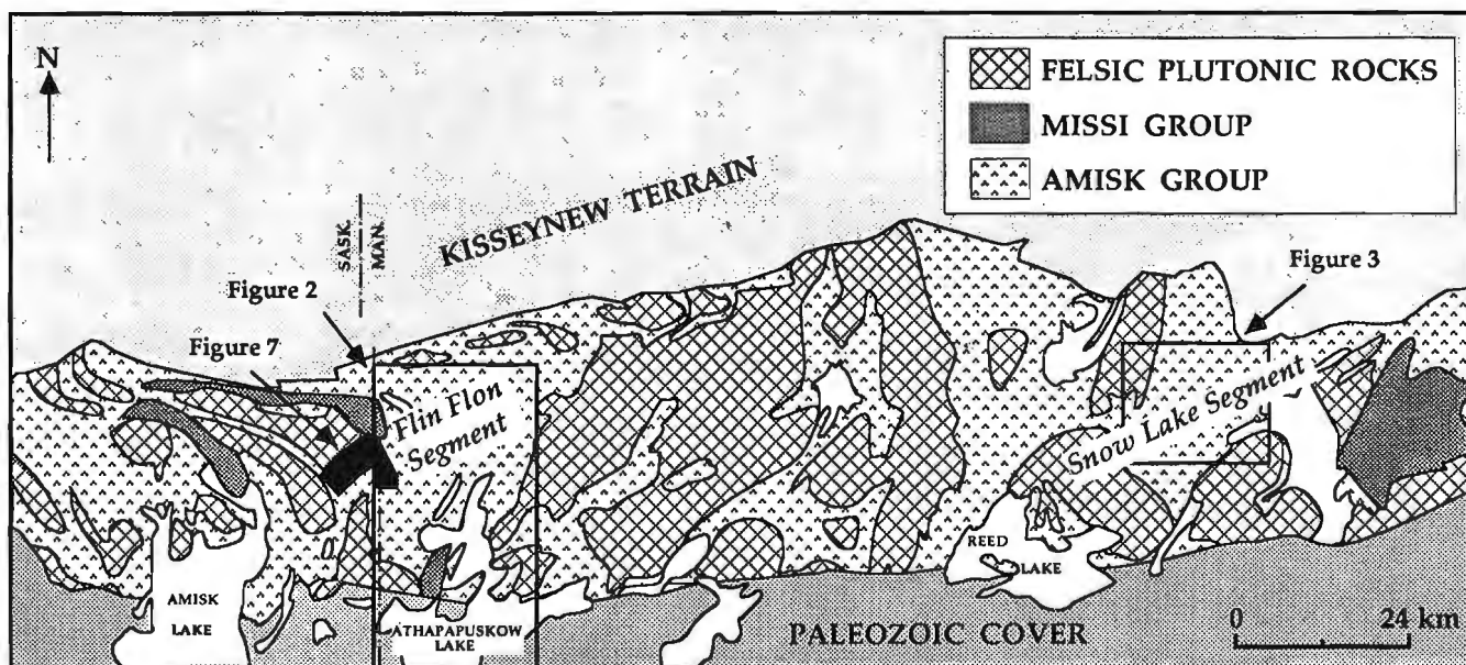
Figure 1. Location map showing the Flin Flon and Snow Lake segments of the Flin Flon metavolcanic belt. Open boxes show location of Figures 2 and 3. Filled region shows the general location of samples used to construct the Nd-isotopic profile of Fig. 7.
