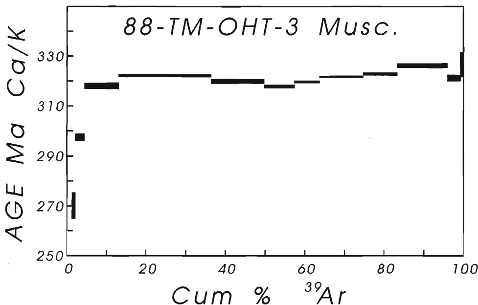
Figure 12. ^{40}\text{Ar} - ^{39}\text{Ar} incremental-release spectrum of muscovite from pegmatite south of Petersen Bay Fault Zone.
