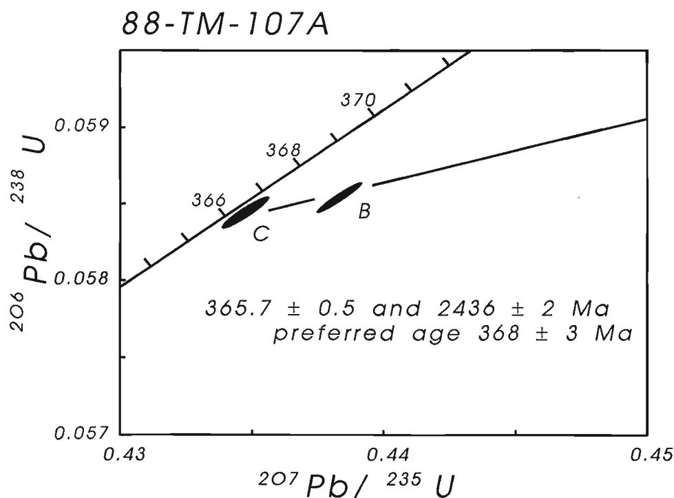
Figure 16. Concordia diagram for trachyandesite south of Rens Fiord.
