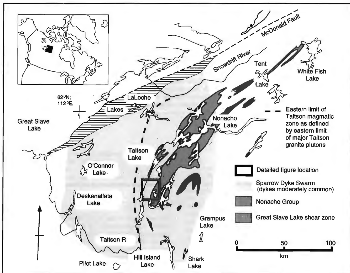
Figure 1. Regional extent of Sparrow dyke swarm.
