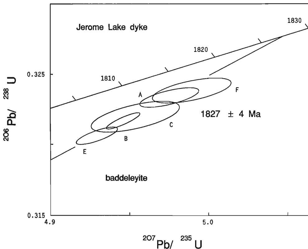
Figure 3. U-Pb concordia plot of baddeleyite fractions from Jerome dyke. Regression line is for fractions A, B and E, and the lower intercept is 277 Ma.
