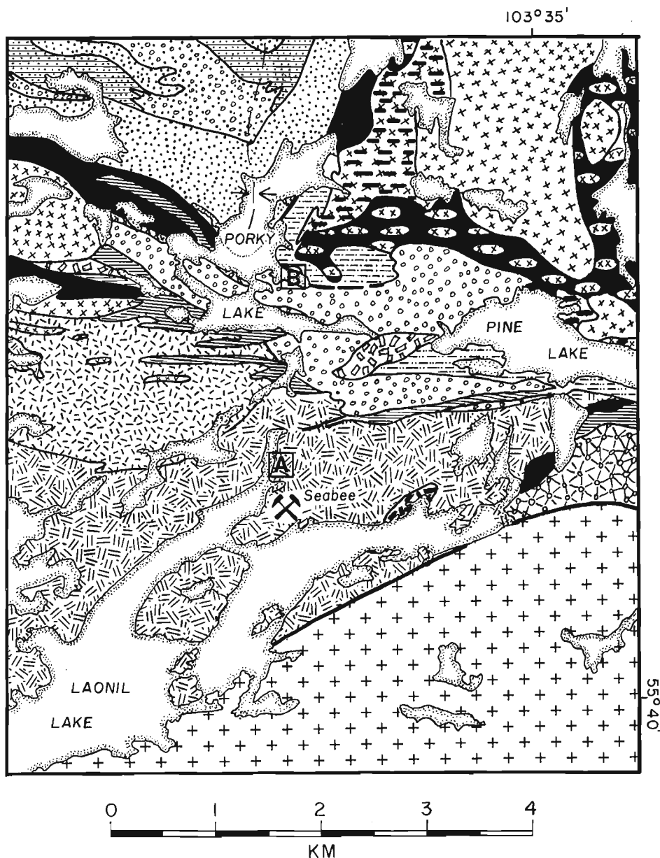
Figure 9. Geological sketch map of the Laonil Lakes area. Letters in boxes show locations of geochronology samples: A = Laonil Lake Intrusive Complex; B = Pine Lake Meta-rhyolite.
