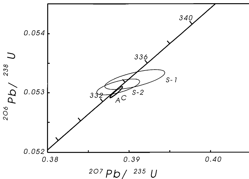
Figure 20. Concordia diagram for Petersen Bay pluton.
