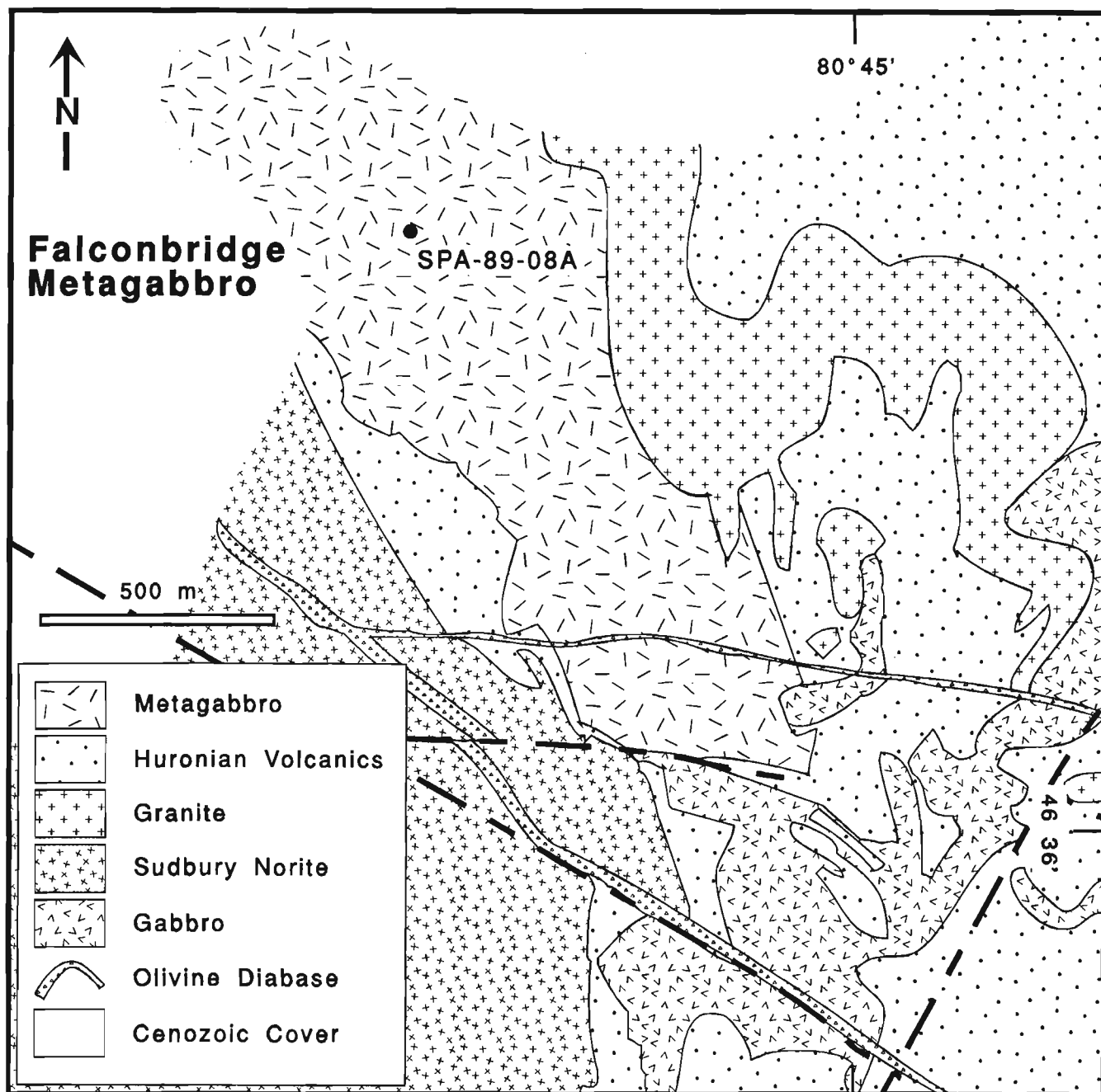
Figure 6. Location map for the Falconbridge Twp. metagabbro sample SPA-89-08A (based on Thomson, 1957). "Olivine diabase" and "Gabbro" are Sudbury dykes and Nipissing Diabase, respectively.
