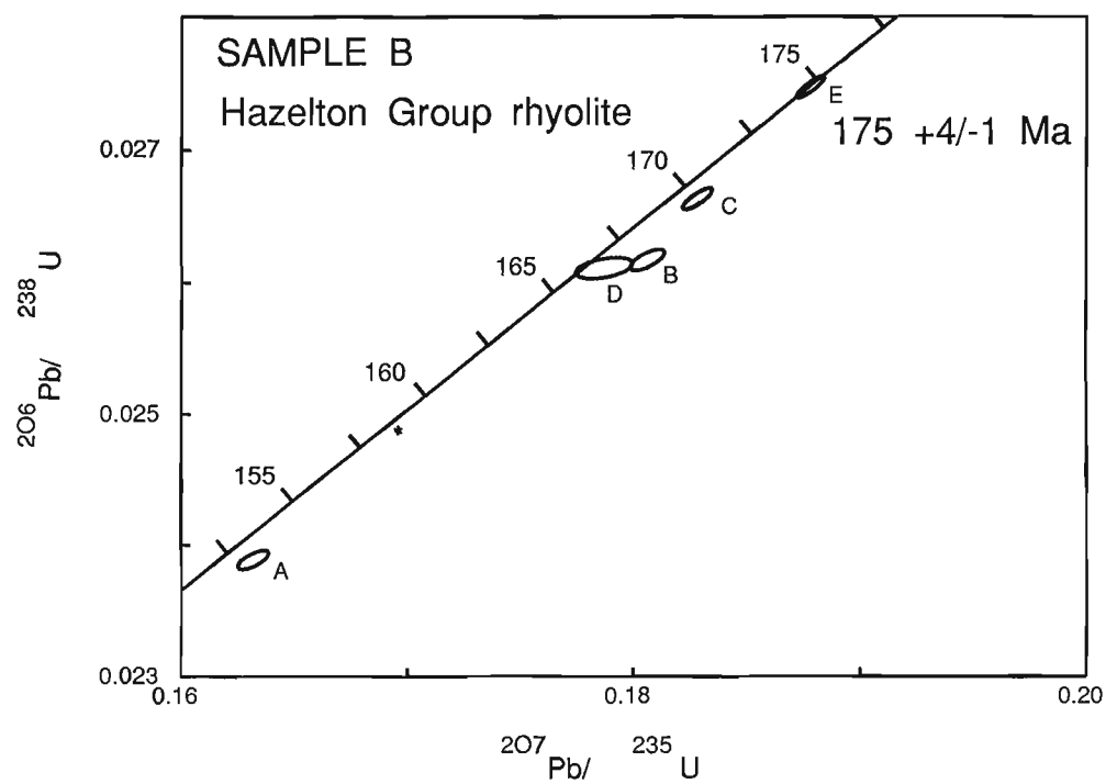
Figure 6. U-Pb concordia plot for sample B, showing 2 \sigma error ellipses.
