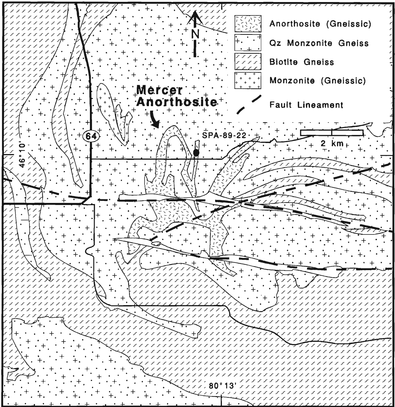
Figure 2. Location map for the Mercer Anorthosite sample (from Lumbers, 1975), showing Highway 64 and other access roads. Lakes are shown beneath fault traces, where present.
