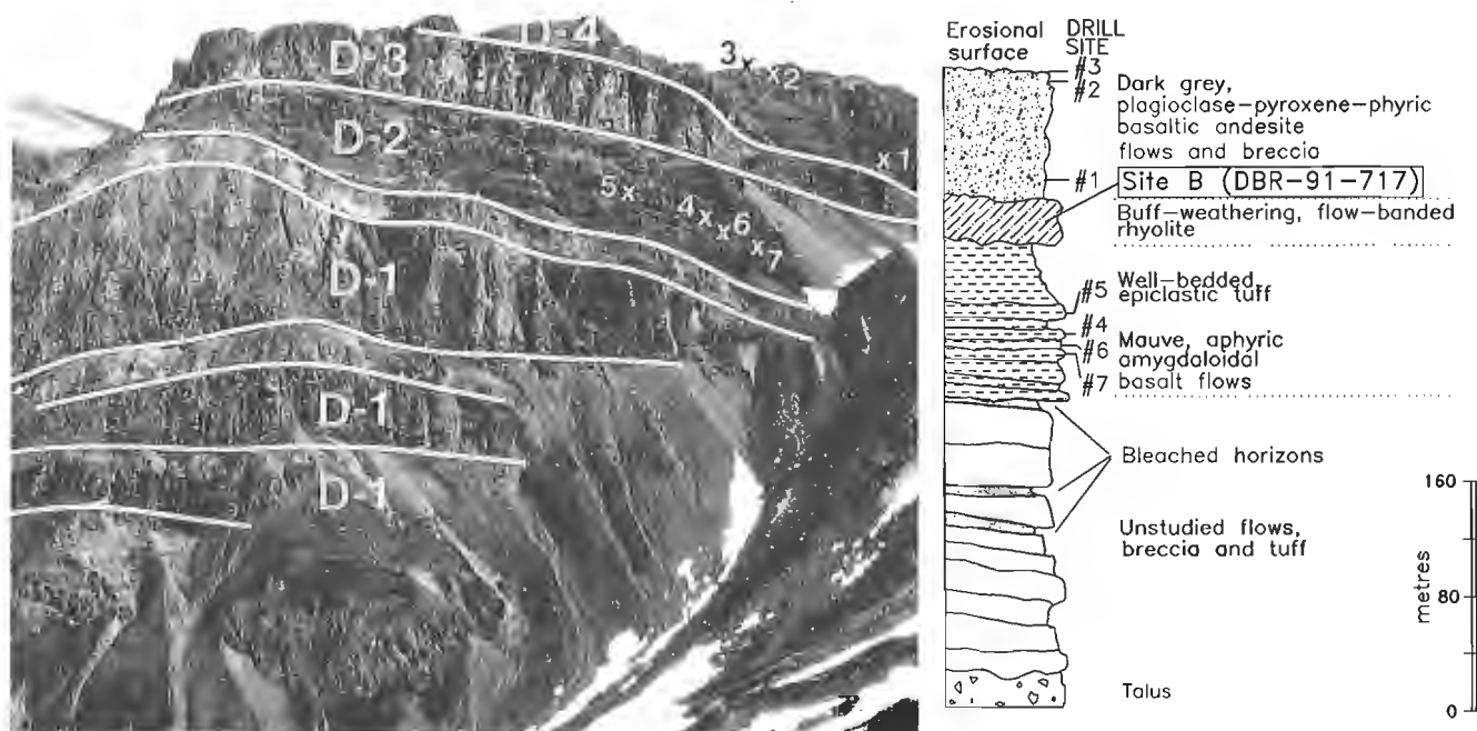
Figure 4. View of rhyolite flow from which sample B was collected, northeast of Kirk Creek, showing the stratigraphic position of this flow relative to paleomagnetic drill sites of Vandall et al. (1992) (small number with x's on photograph). The schematic column for the Kirk Creek cirque area illustrates the local stratigraphic position of the rhyolite (D-3 on photograph) relative to underlying basalt flows and epiclastic beds (D-2) and the overlying pyroxene-plagioclase phyric andesite flows (D-4). D-1 was not examined.
