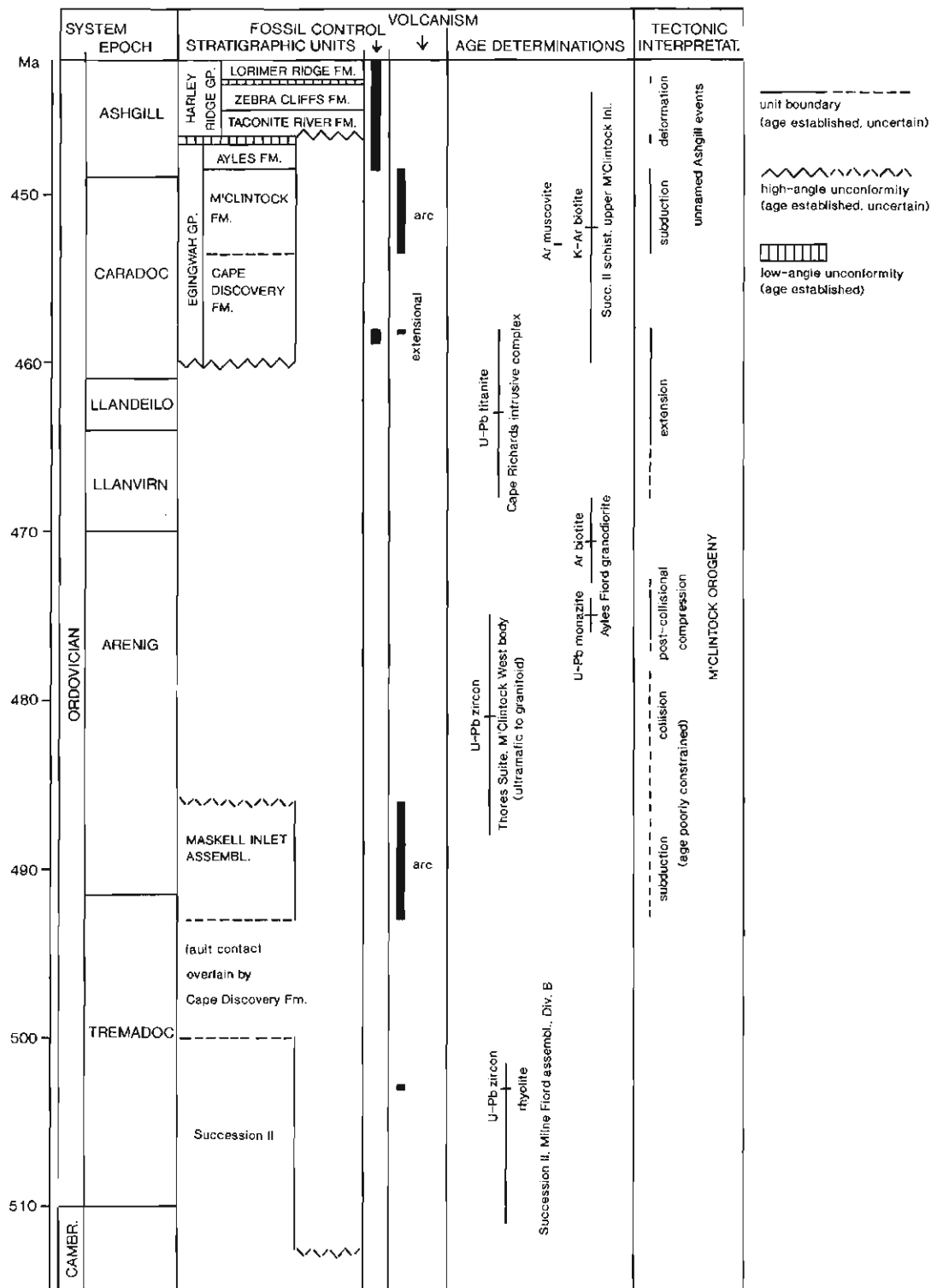
Figure 6. Correlation of Ordovician stratigraphic units and plutons, M'Clintock Orogen.
