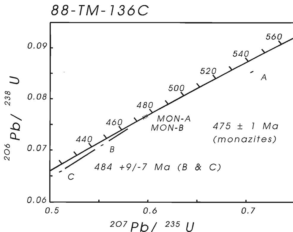
Figure 7. Concordia diagram for Ayles Fiord granodiorite.
