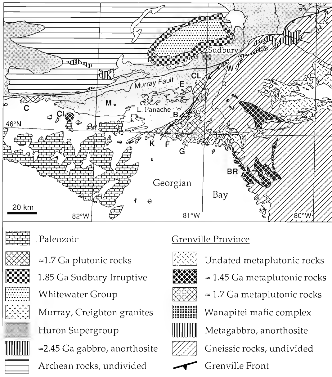
Figure 1. Generalized geology of the Sudbury region. Dated plutonic rock units mentioned in the text are identified as follows: C - Cutler, CI - Croker Islands, M - Mongowin, K - Killarney, B - Bell Lake, E - Eden Lake, CL - Chief Lake, W - Wanapitei Complex, F - Fox Islands, G - Grondine, BR - Britt.
