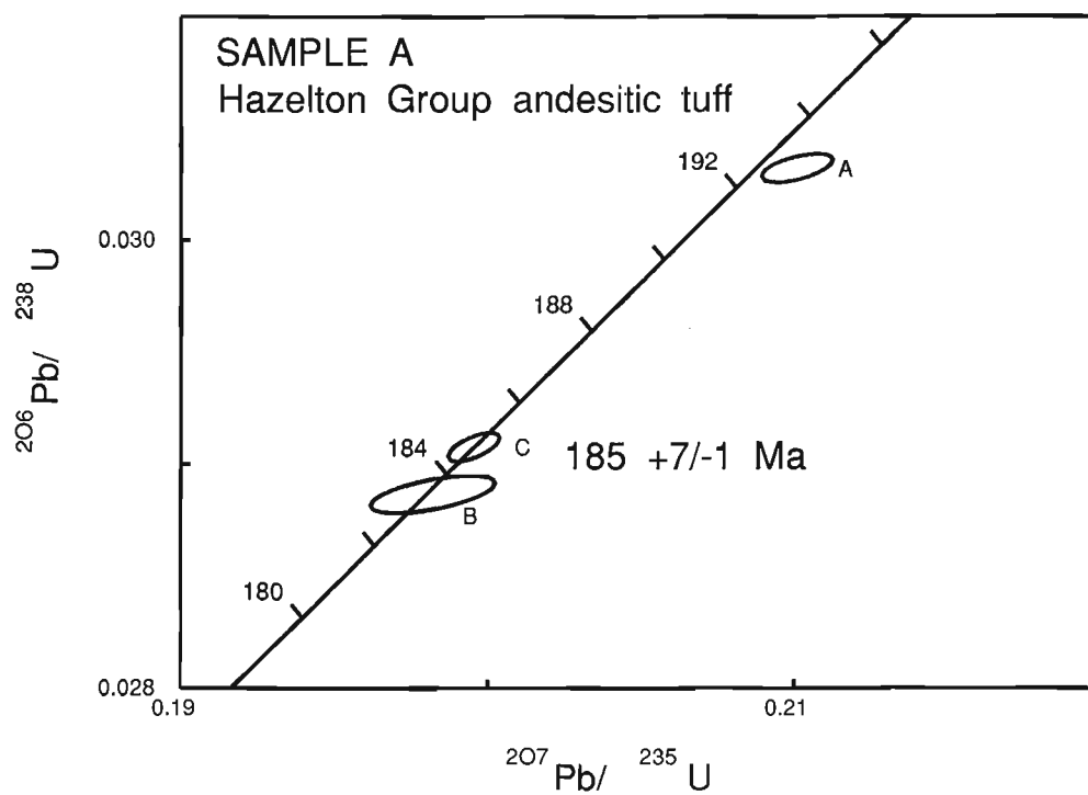
Figure 5. U-Pb concordia plot for sample A, showing 2 \sigma error ellipses.
