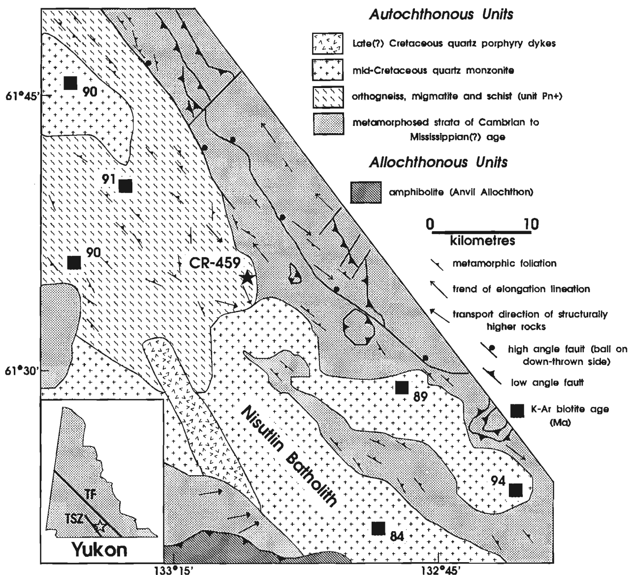
Figure 1. Simplified geology of the west-central part of Quiet Lake map area (modified from Tempelman-Kluit, 1977). Main structures shown on inset map: TF, Tintina Fault Zone; TSZ, Teslin Suture Zone. Star on inset map shows location of the study area.
