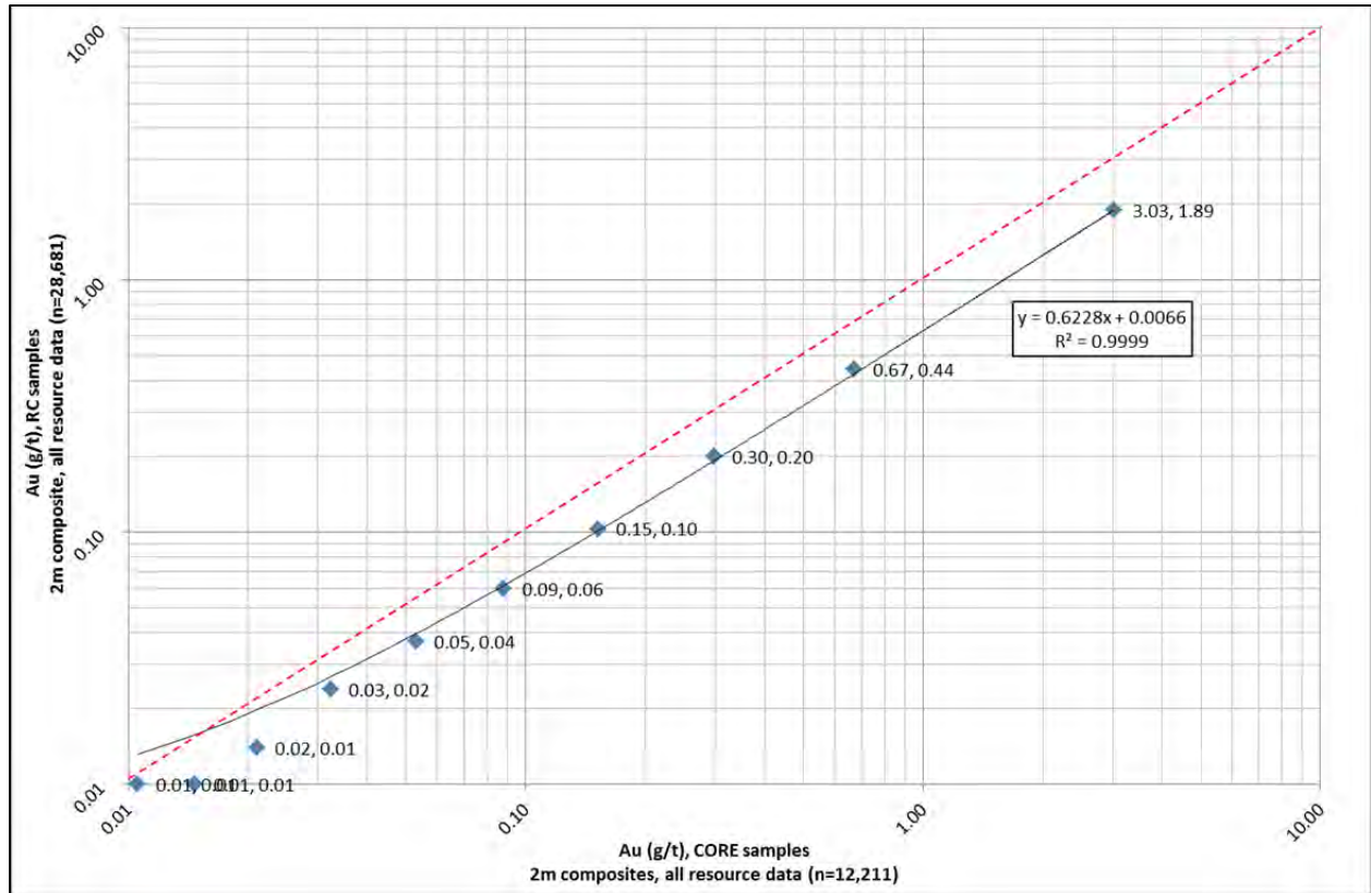
Figure 12-2 Decile-Decile Plot for RC and Core Drilling Data
