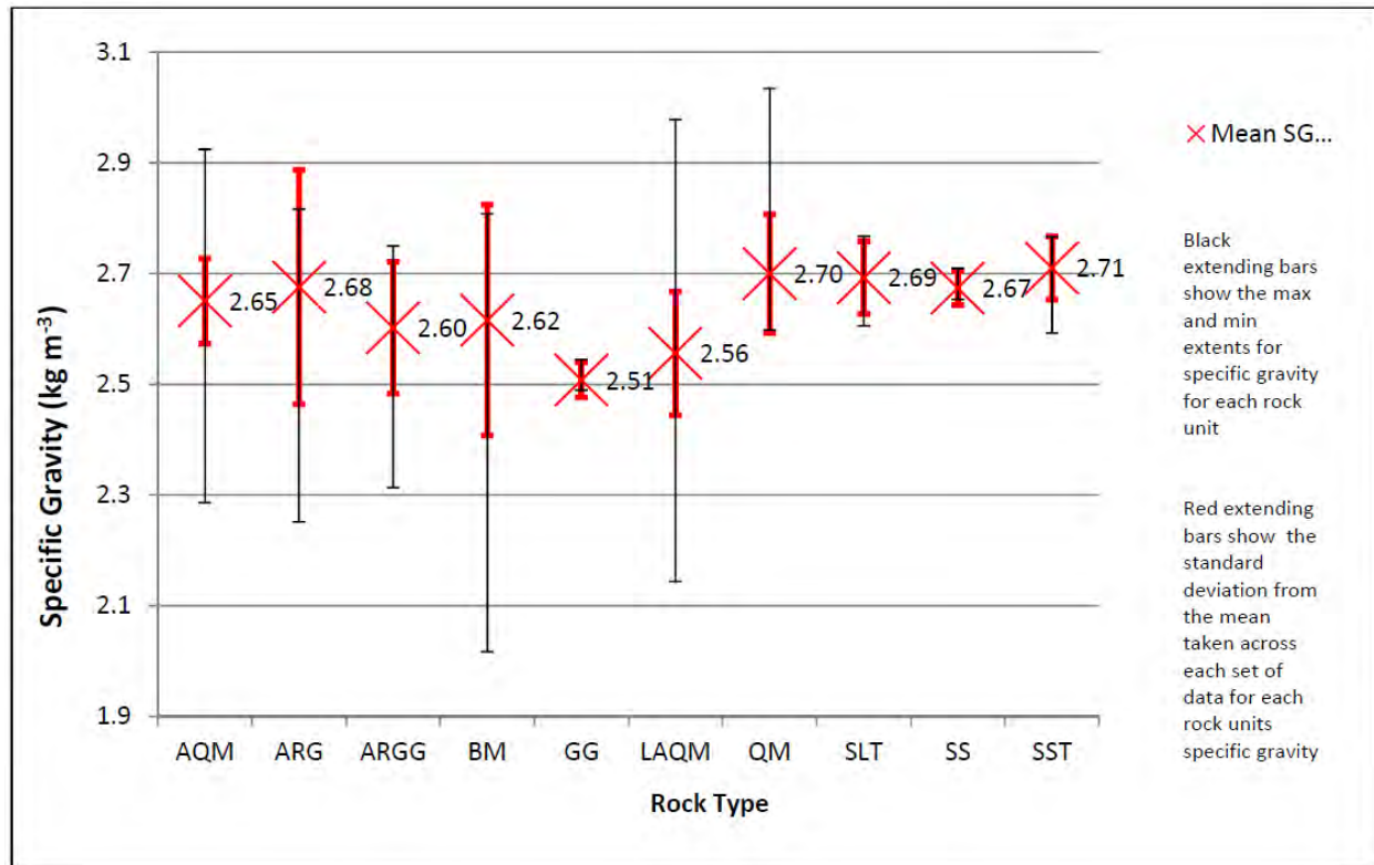
Figure 14-44 Specific Gravity Determination by Rock Type
