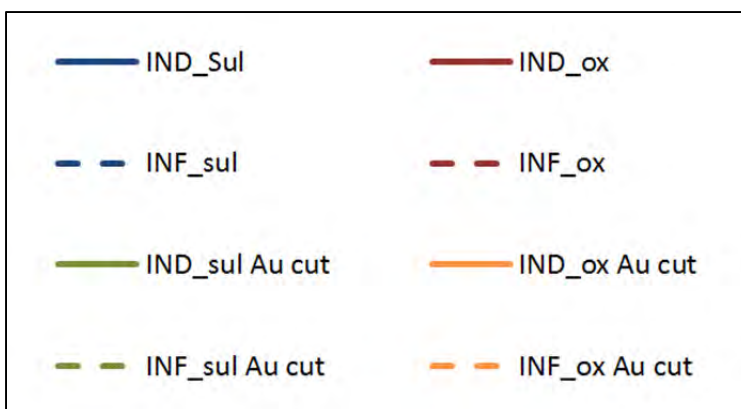
Figure 14-49 Legend for grade-tonnage curve line types
