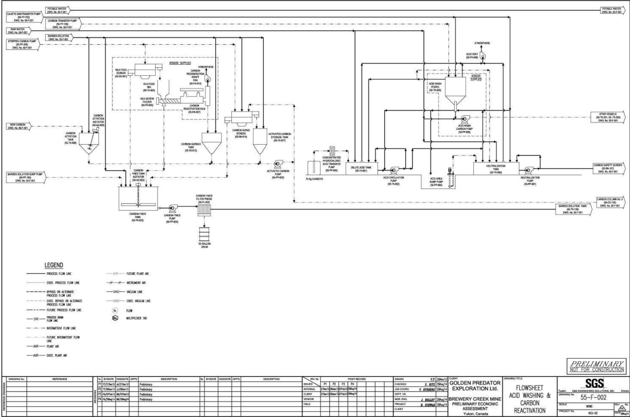
Figure 17–8: Conceptual Acid Washing and Carbon Reactivation Flowsheet (SGS 55-F-002, 2014)
