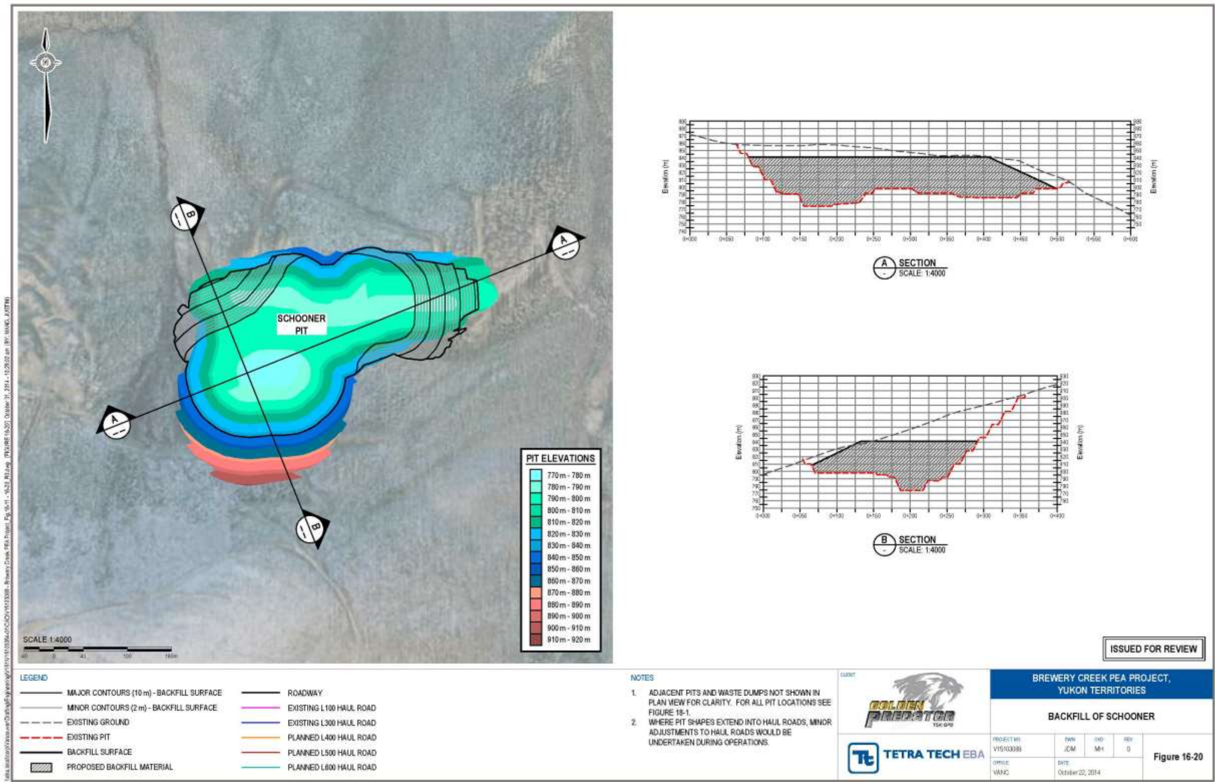
Figure 16–20: Schooner Backfill
