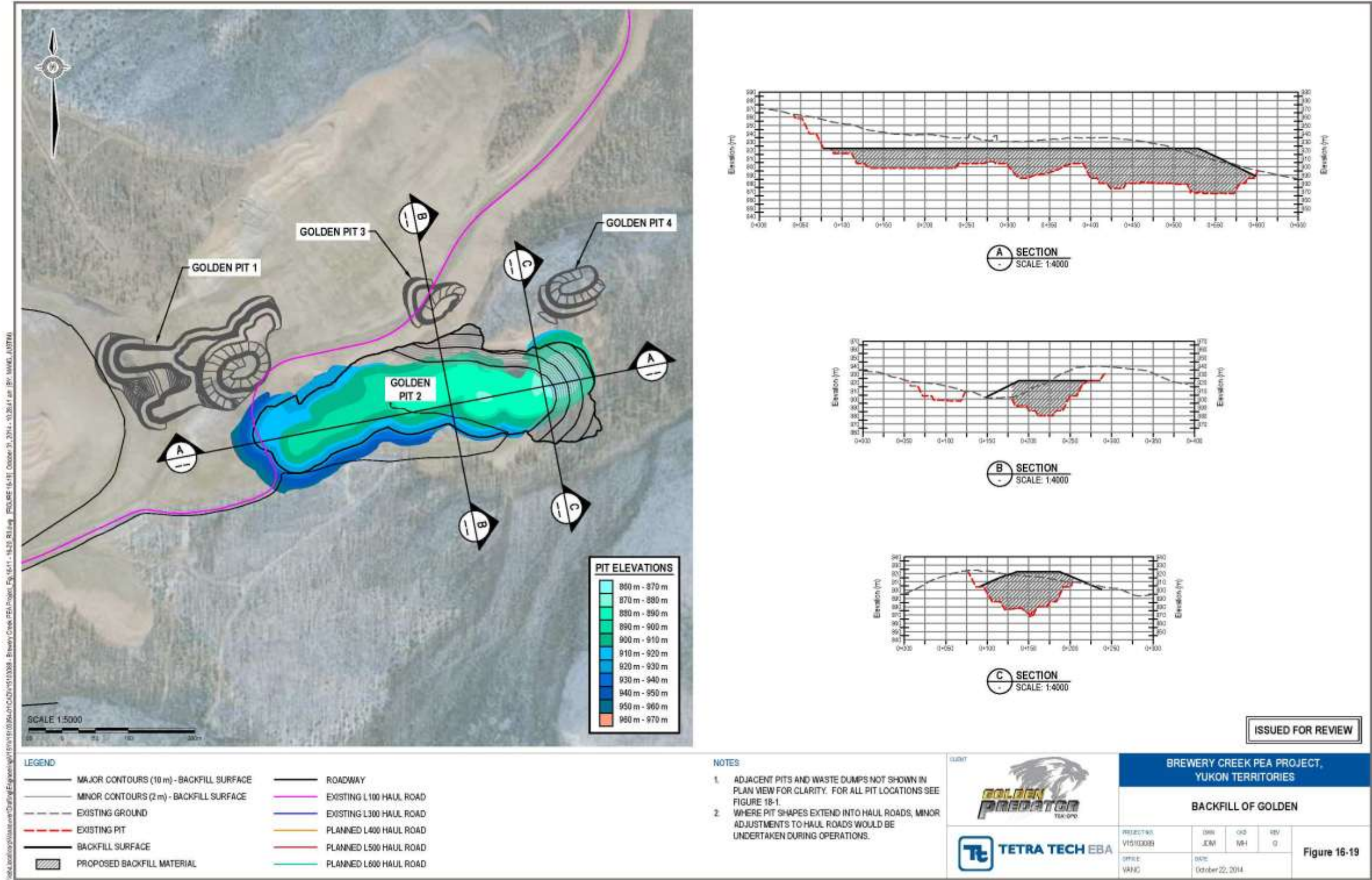
Figure 16–19: Golden Backfill
