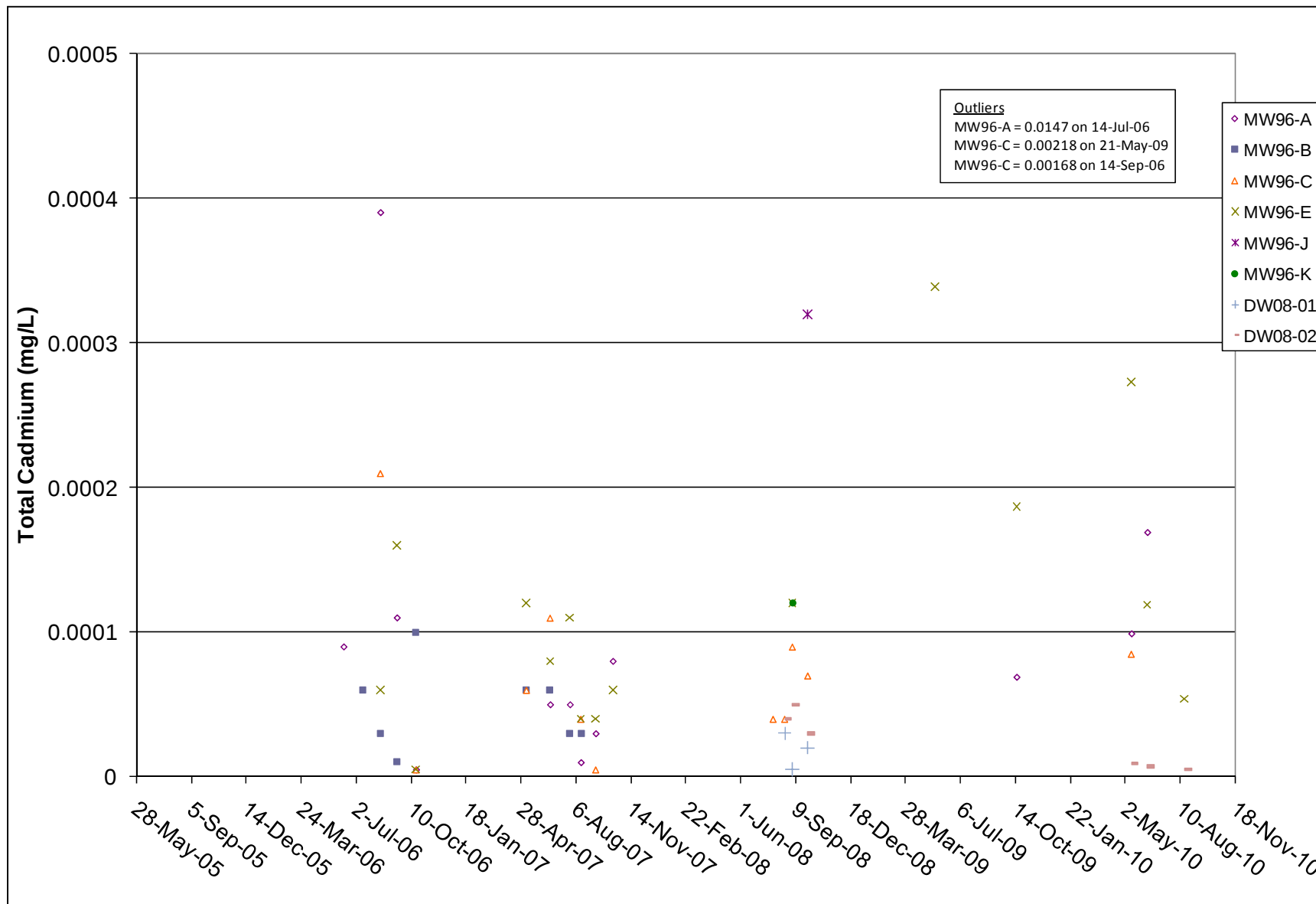
Figure 10 Carmacks Copper Monitoring Wells, Total Cadmium
