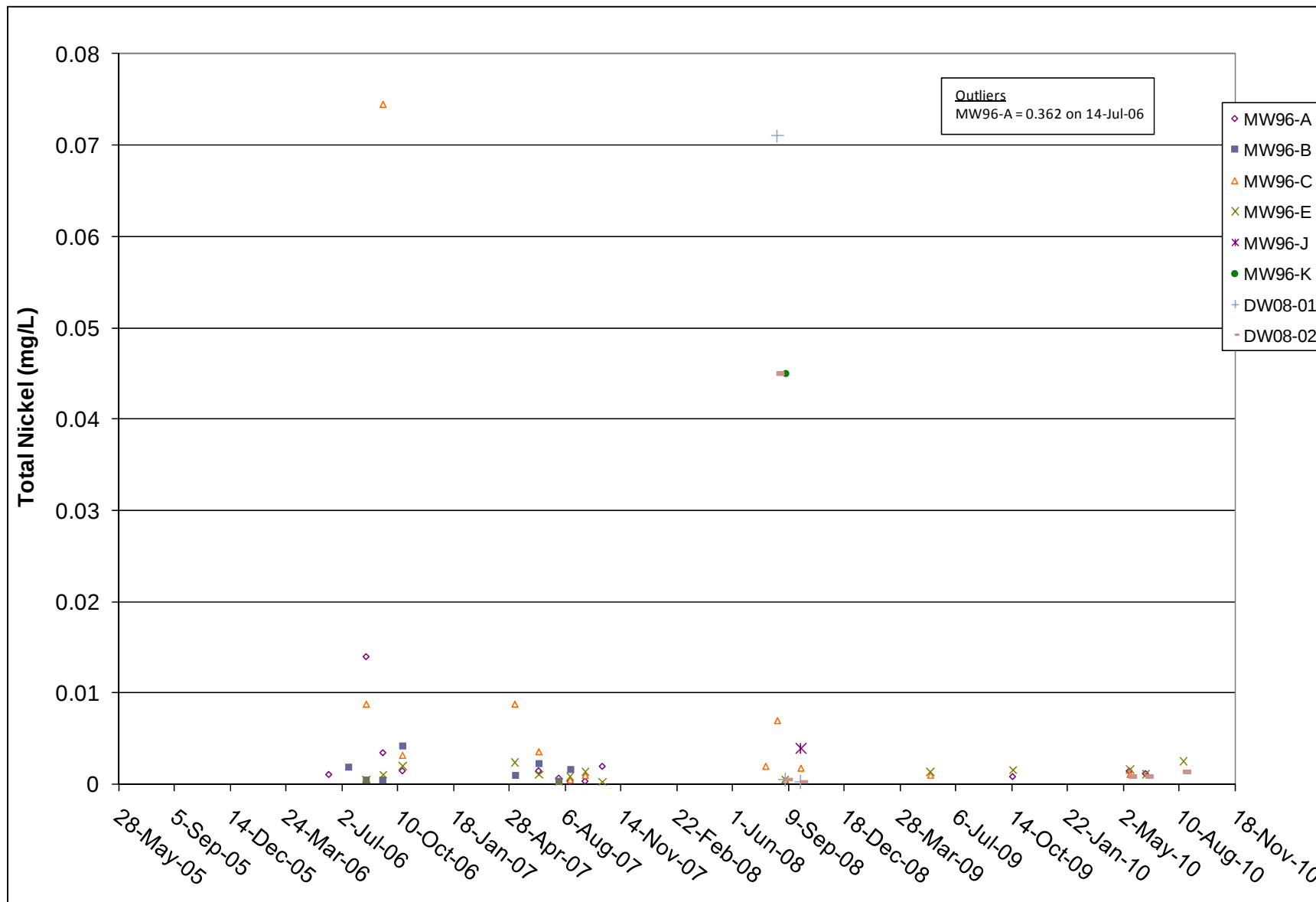
Figure 14 Carmacks Copper Monitoring Wells, Total Nickel
