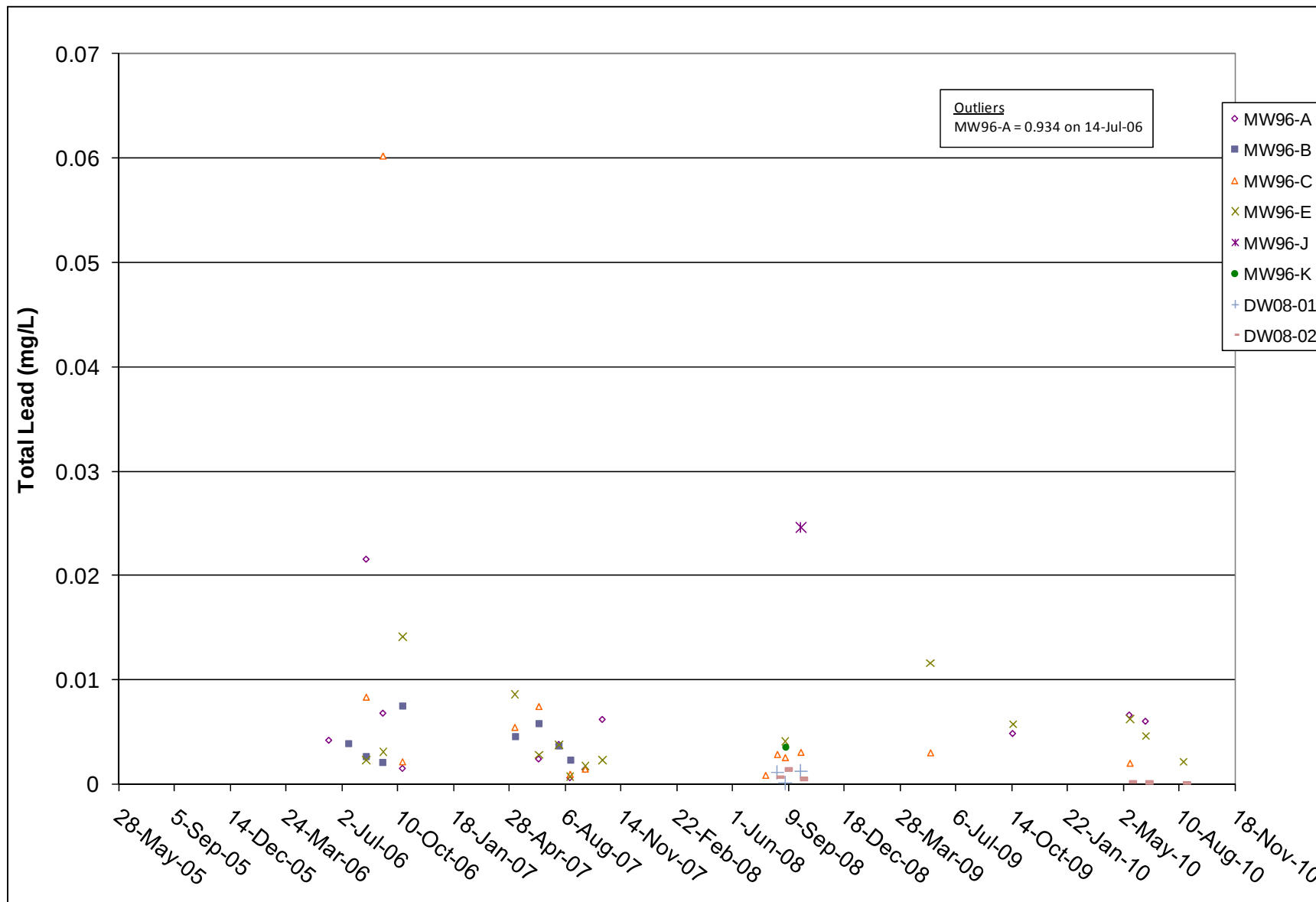
Figure 13 Carmacks Copper Monitoring Wells, Total Lead
