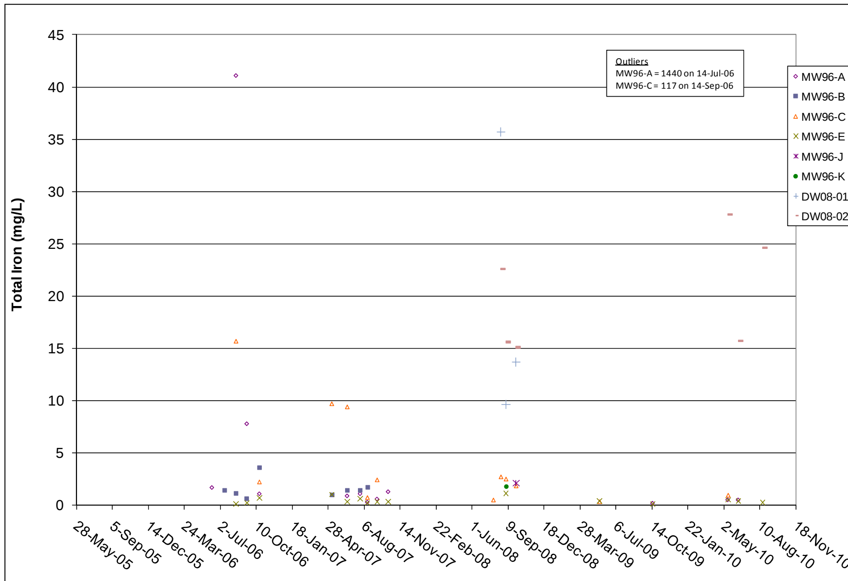
Figure 12 Carmacks Copper Monitoring Wells, Total Iron
