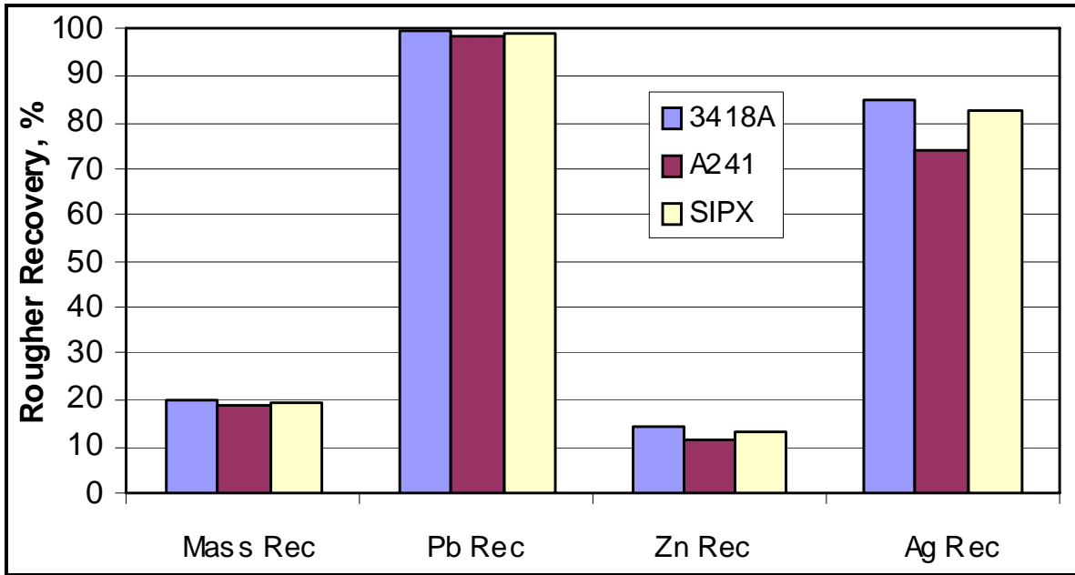
Figure 16.2: Effect of Collectors on Lead, Zinc, and Silver Recovery at Lead Rougher Flotation
