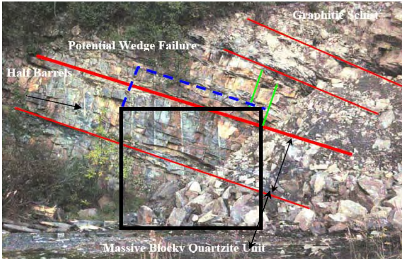
Figure 19.12: Wedge Failure Diagram in the Middle Quartzite Unit
