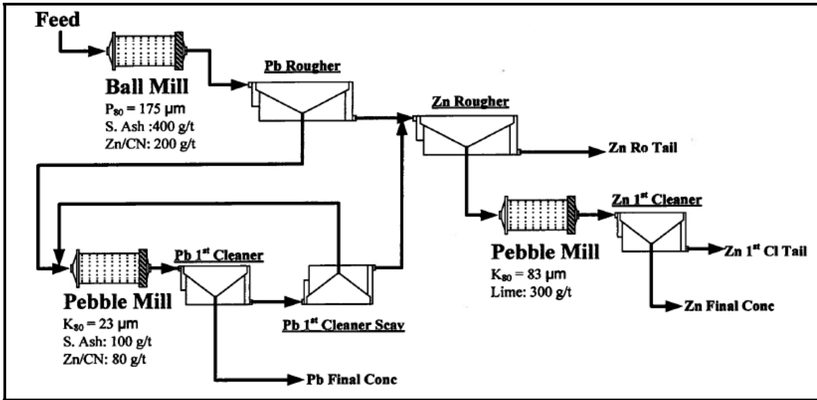
Figure 16.3: Locked Cycle Test Flowsheet - Lakefield
