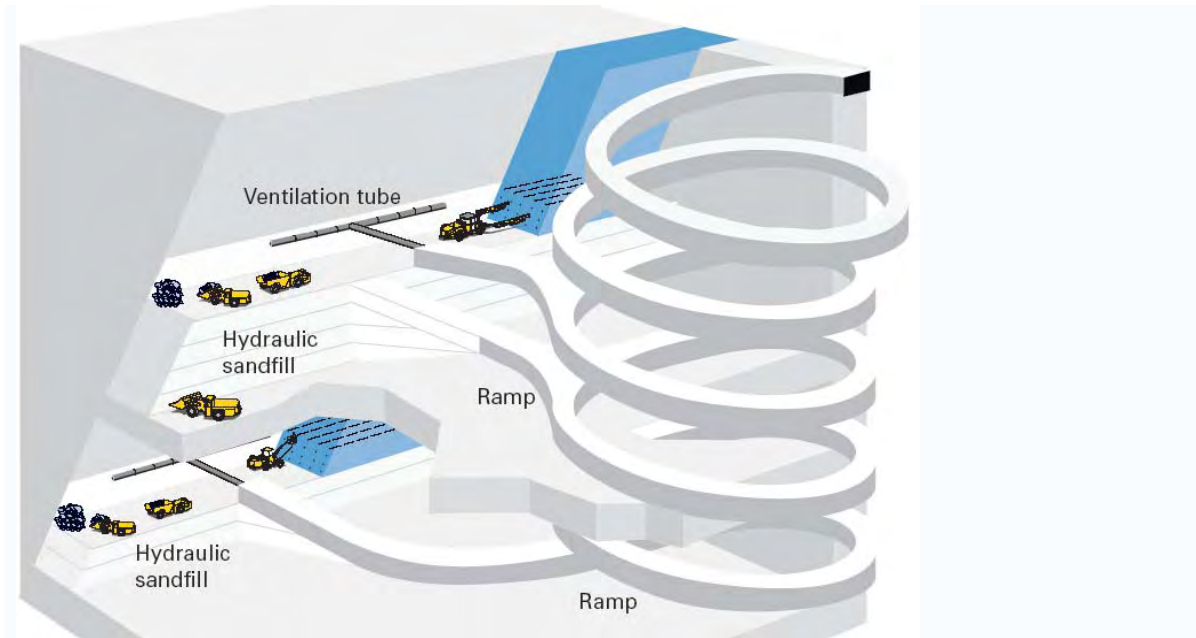
Figure 19.8: Overhand, Mechanized Cut & Fill Mining Method (from Atlas Copco)
