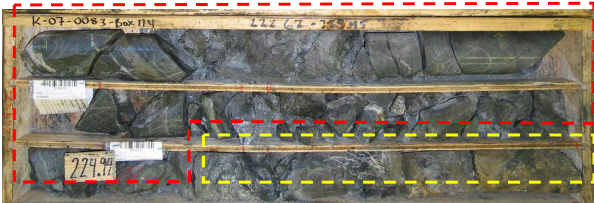
Figure 19.6: K-07-0083 Mineralized Zone (yellow) and Immediate Hangingwall (red) with Poor Ground Conditions
