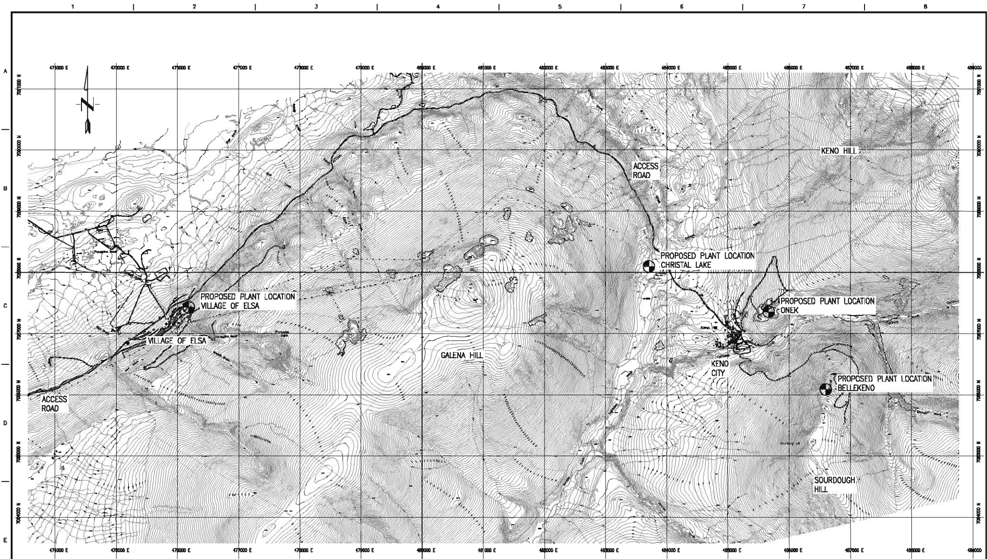
MILL SITE - PROPOSED LOCATIONS PLAN
