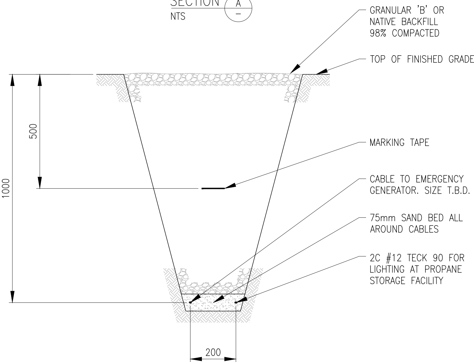
SECTION B NTS
