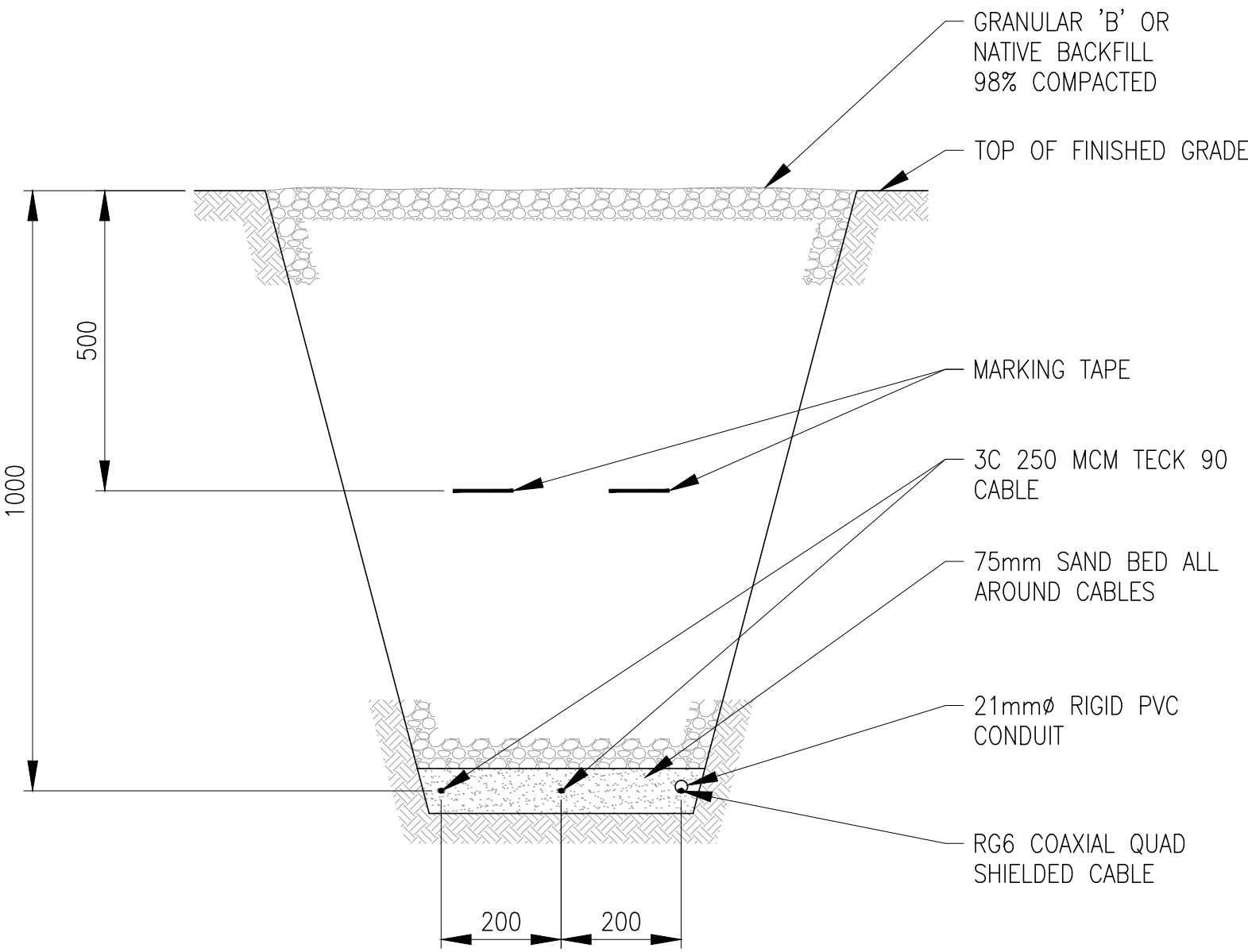
SECTION A NTS
