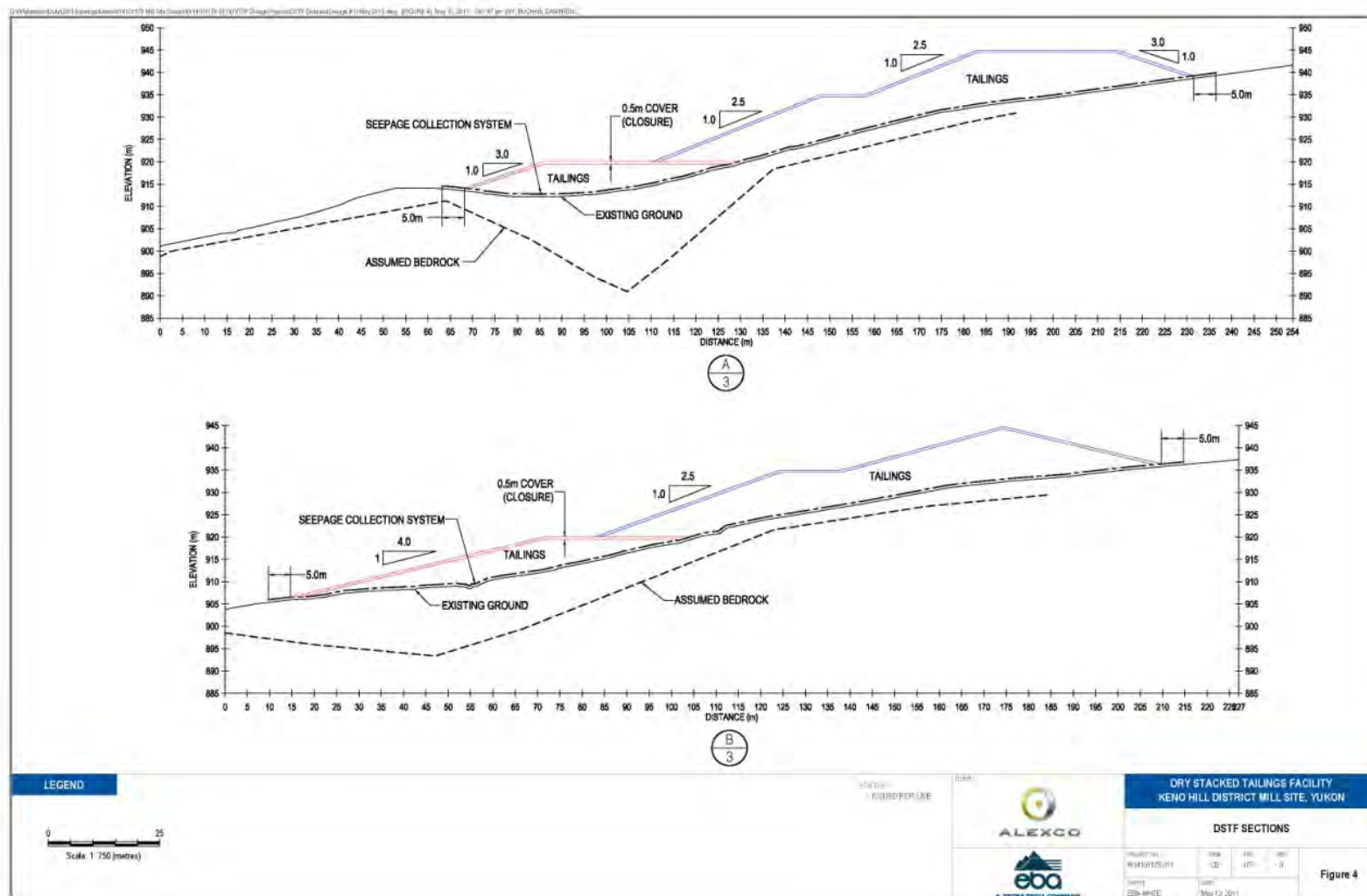
Figure 4-5 DSTF Sections
