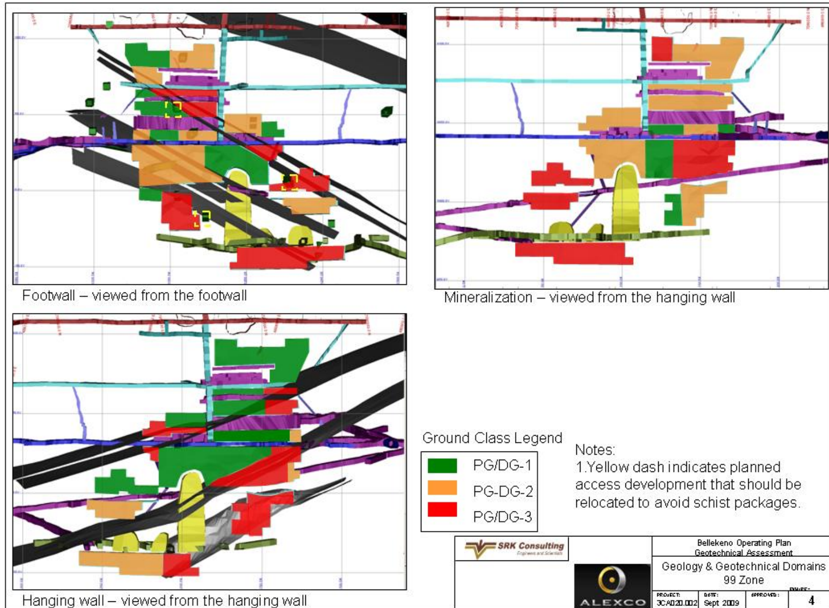
Figure 4: Geology & Geotechnical Domains – 99 Zone vertical projections
