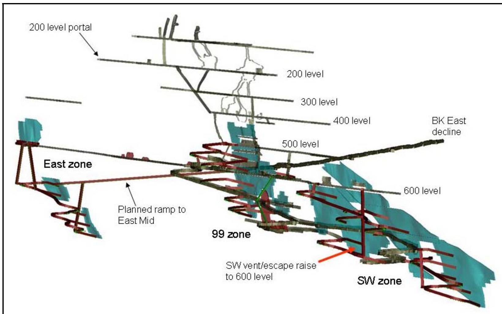
Figure 20: 3D View of Mine Workings looking NE from the footwall side
