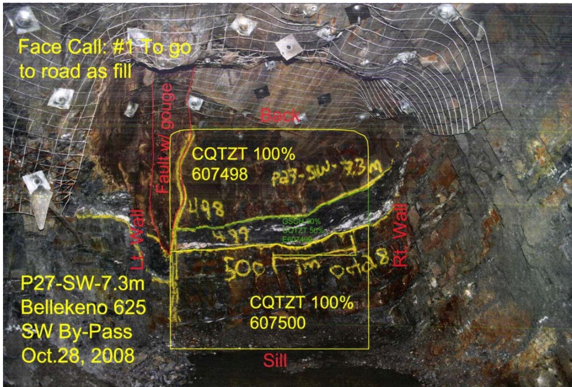
Figure 12 Face Photo of Bellekeno 625 Bypass Showing Sampling According to Lithology and Calculated Sample Areas
