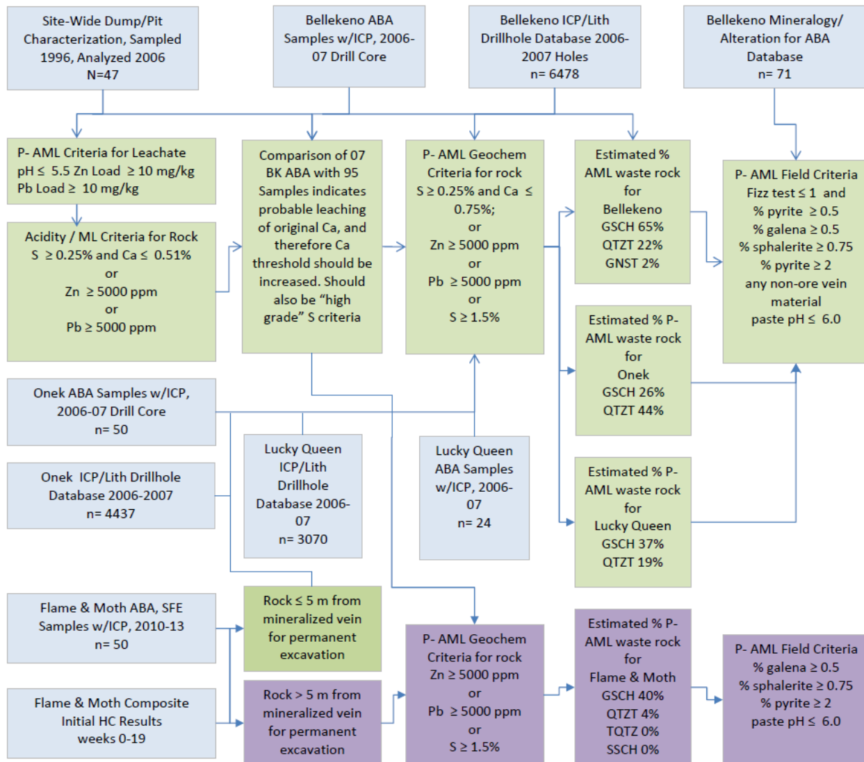
Figure 1: Keno Hill Development Waste Rock Characterization Studies – Components and Key Results
