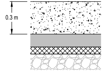
DETAIL 2 - FACILITY FLOOR AND BERMS
