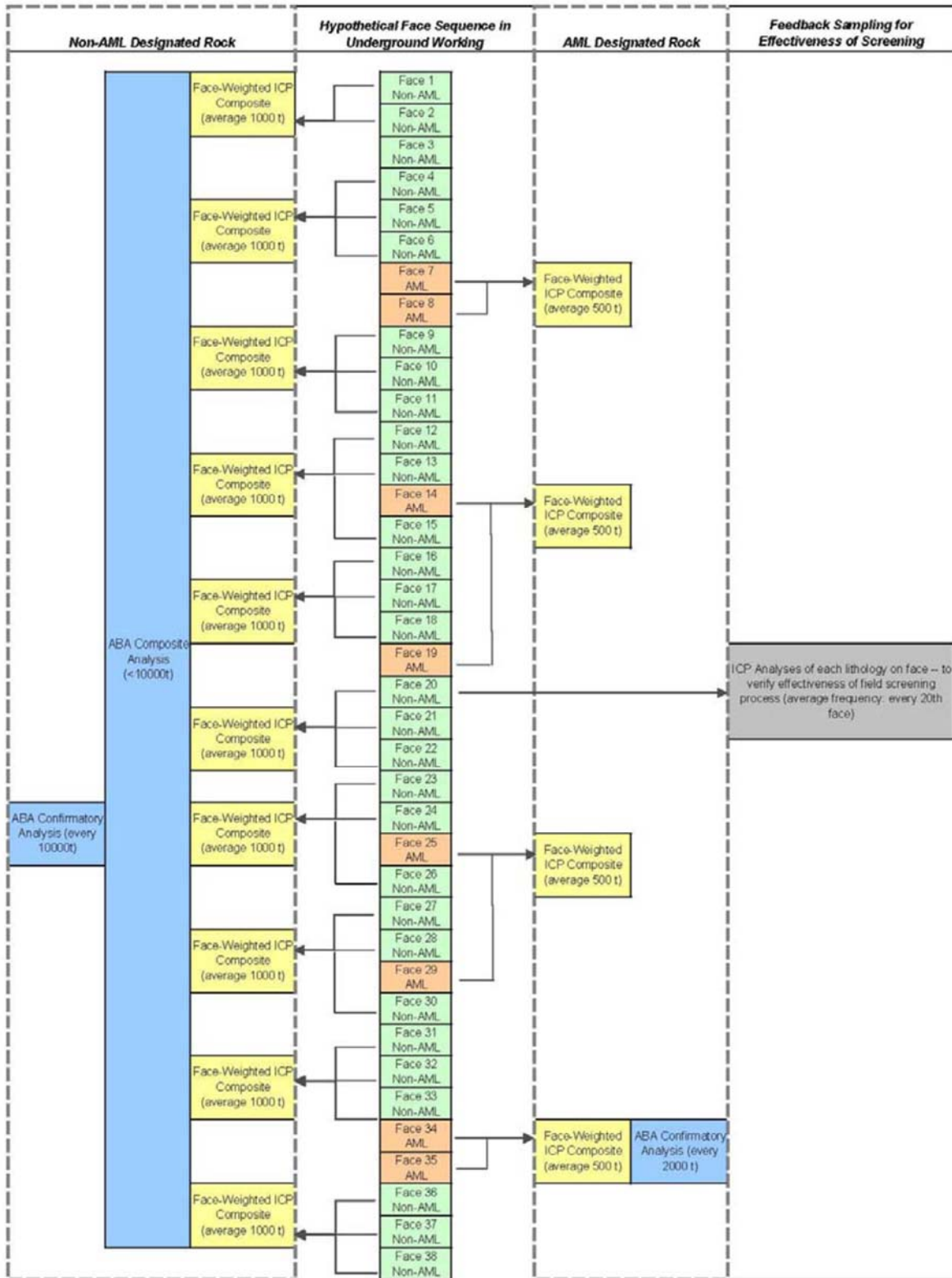
Figure 13 Waste Rock Sampling Schedule
