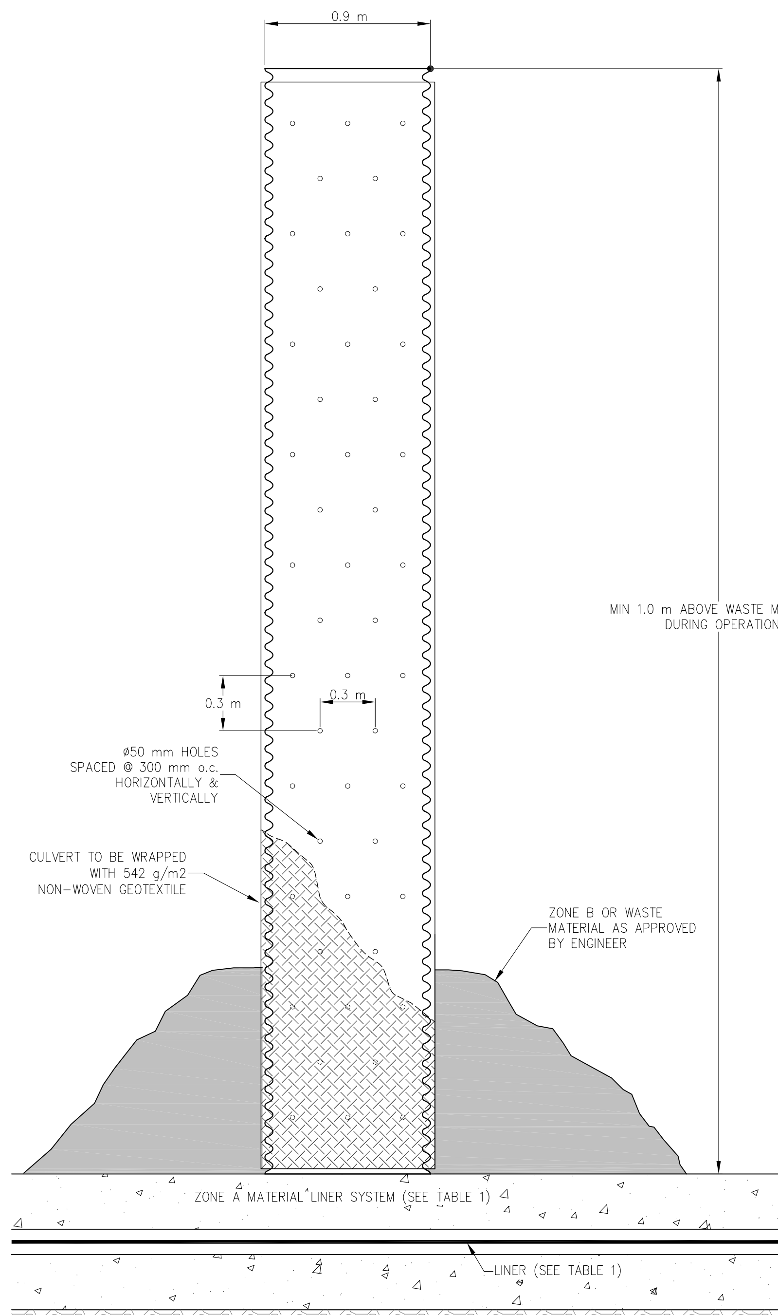
DETAIL 1 - VERTICAL CULVERT 9 SCALE: 1 : 20 WCF-1
