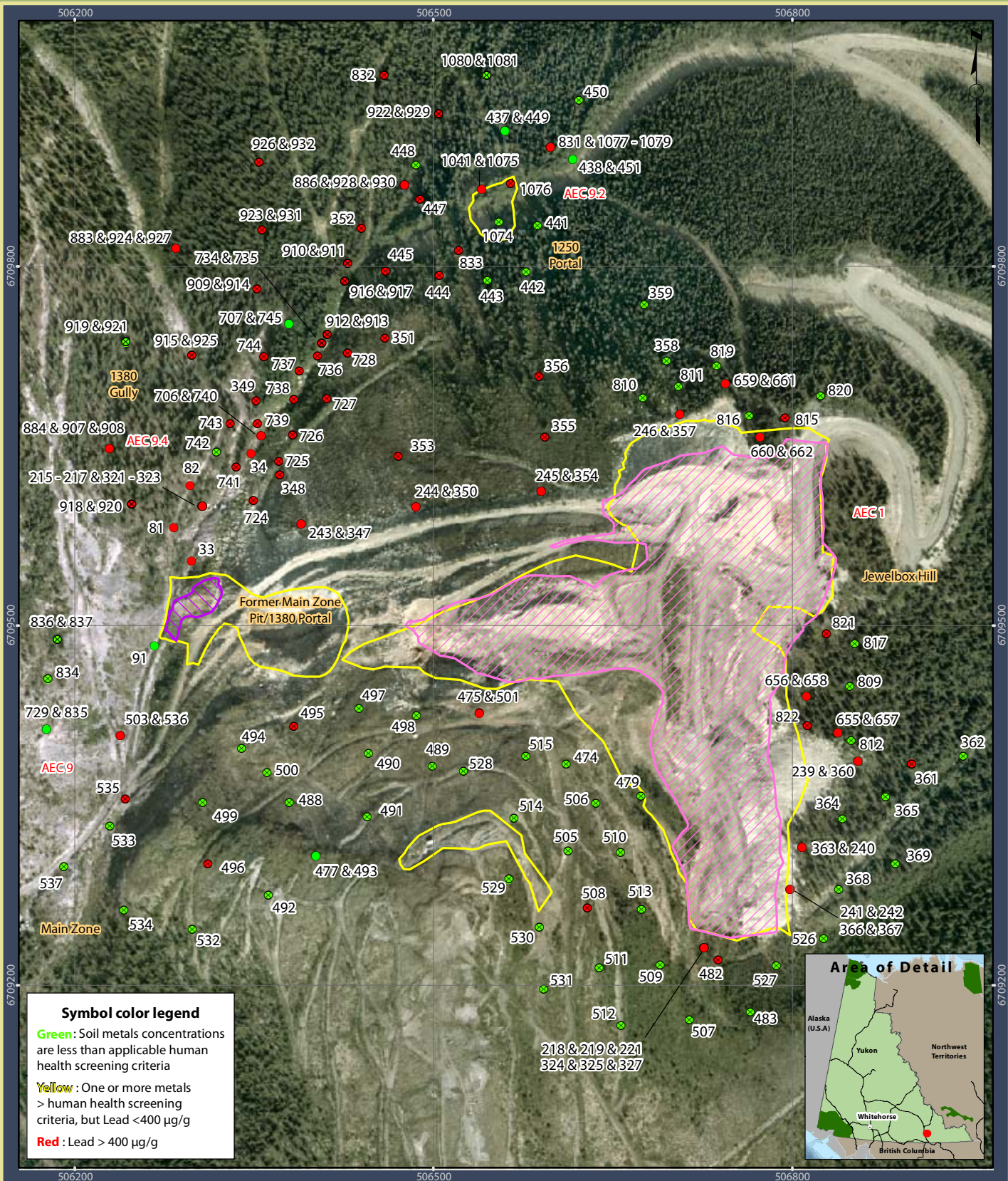
Figure 2. Remediation Cover Areas and Post-Remediation Surface Soil Chemistry for the Main Zone Pit, Jewelbox Hill, 1380 Gully, and 1250 Portal Areas
