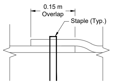
3 Side Seam Overlap Staple Detail Not To Scale
