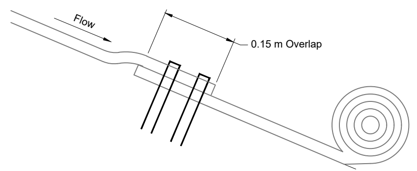
4 Channel Blanket End of Roll Overlap Not To Scale
