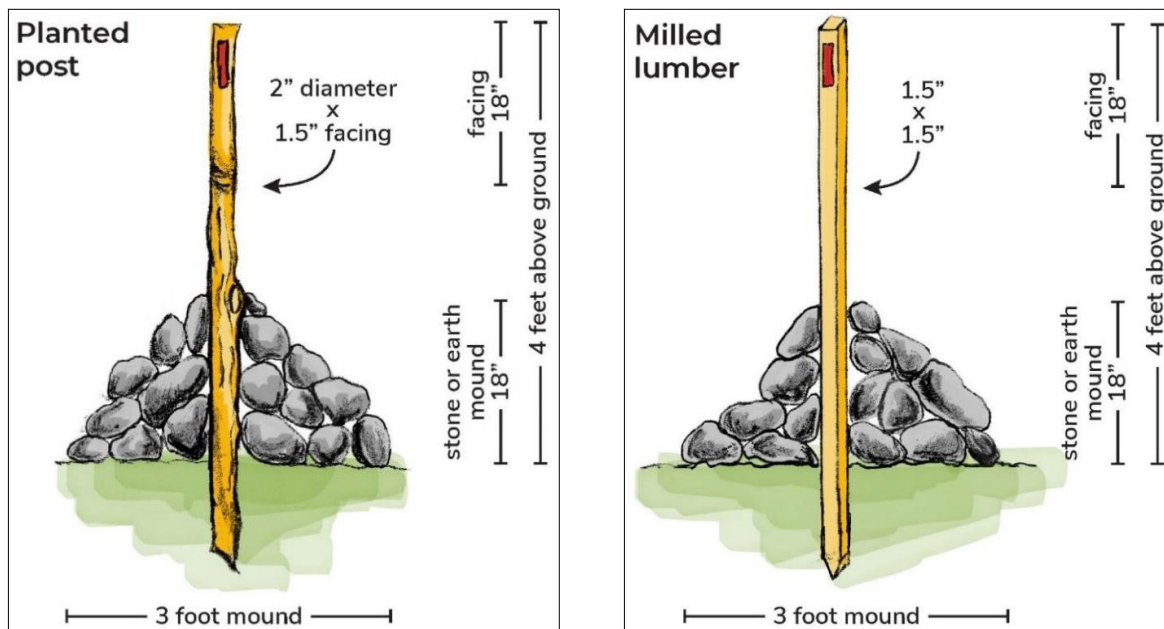
Figure 1a: examples of claim posts
