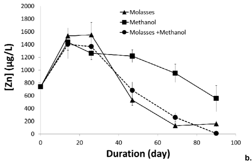
Figure 2-3 Metal concentrations in each batch test. Cd concentration (µg/L) (a.), Zn concentration (µg/L) (b.)
