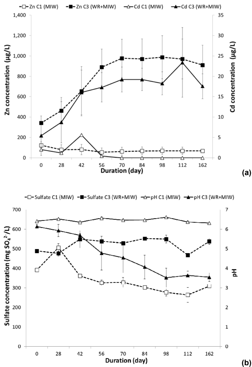
Figure 3-1 Evolution of the concentrations of Zn, Cd (a.) and Sulfate and pH (b.) measured in the control C1 (MIW) and C3 (WR + MIW) during the experimental period
