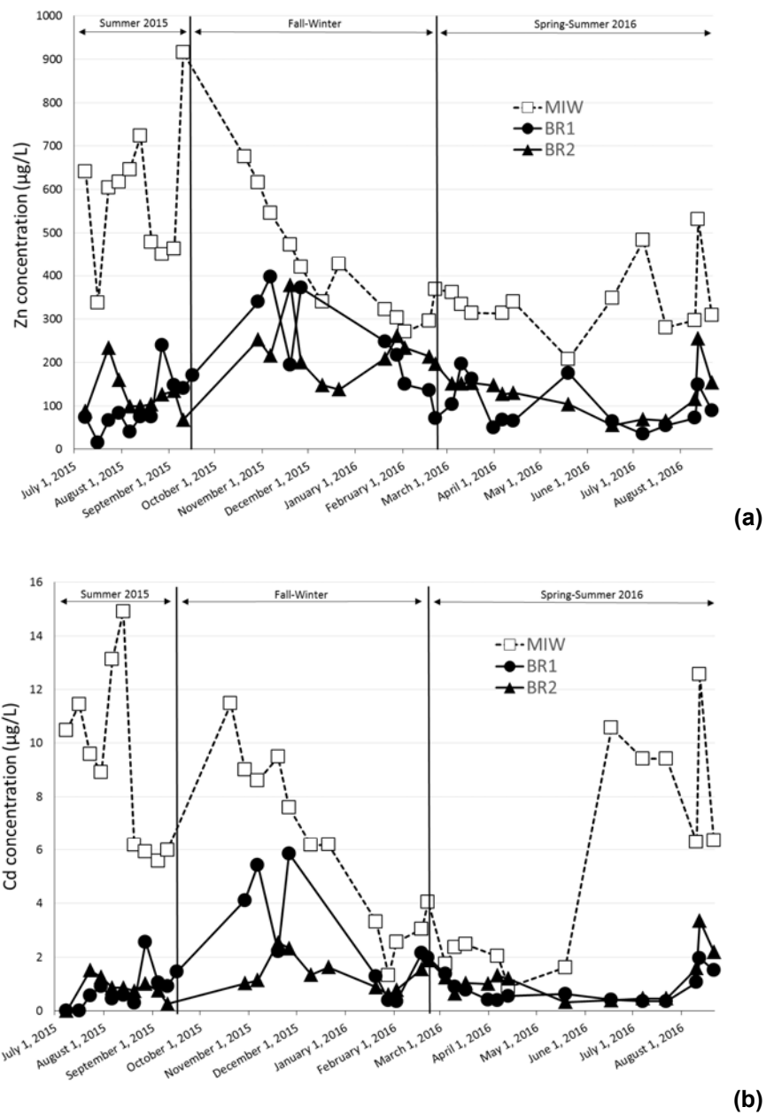
Figure 4-3 Zn (a) and Cd (b) concentrations in MIW, BR1 and BR2 during the 14 months experiment
