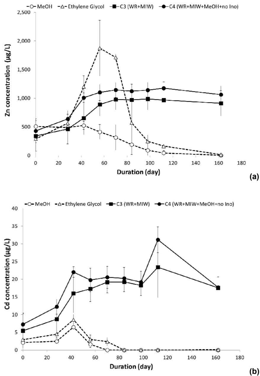
Figure 3-2 Evolution of the concentrations of Zn (a.) and Cd (b.) measured in the bioreactors for the experiments performed in the presence of MeOH and Ethylene glycol and in controls C3 (WR + MIW) and C4 (WR + MIW + MeOH) during the experimental period
