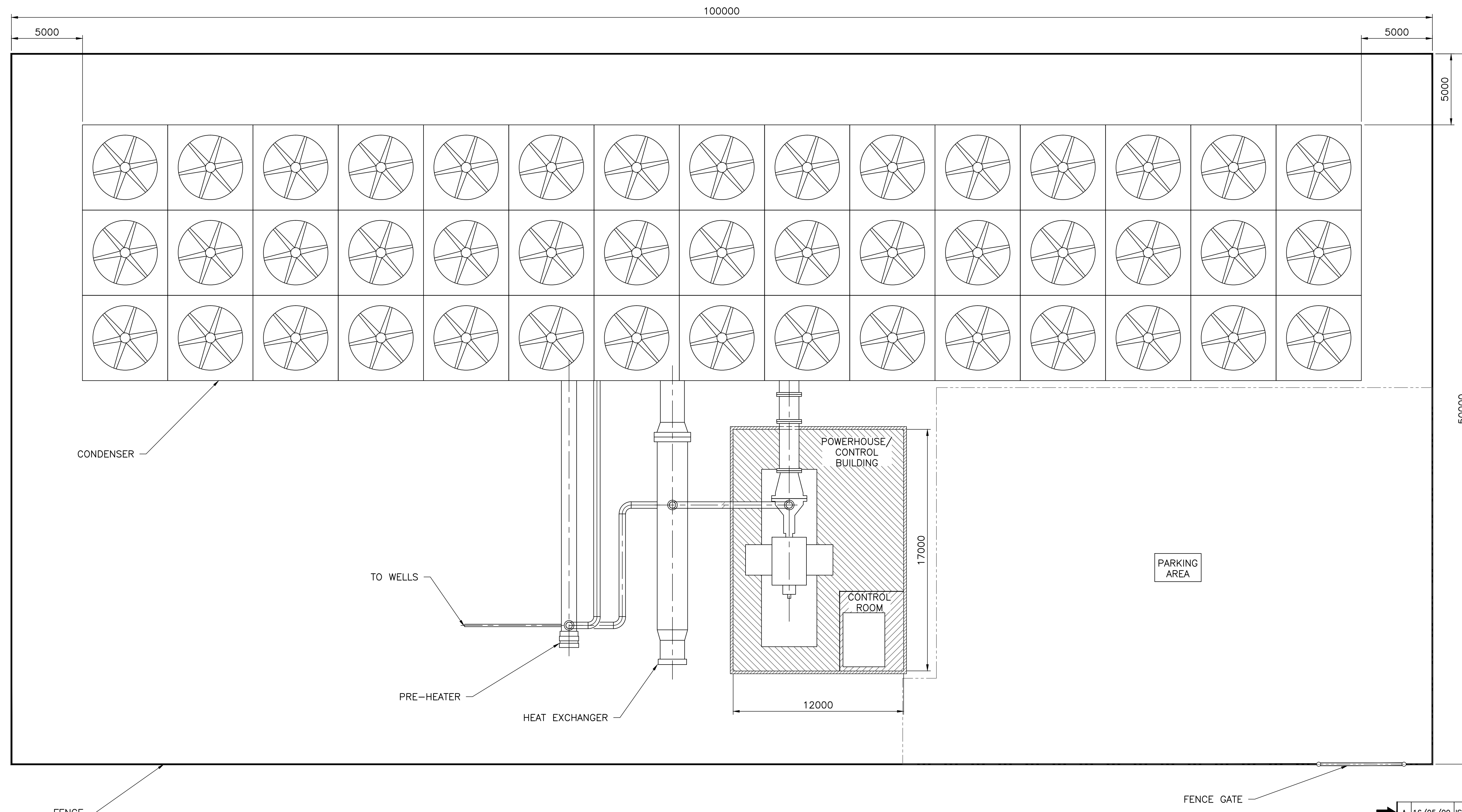
McARTHUR SPRINGS GEOTHERMAL ORC PLANT (7.0 MW) 3000 0 3000 6000 9000 12000 SCALE: 1:150mm (24"x36")
