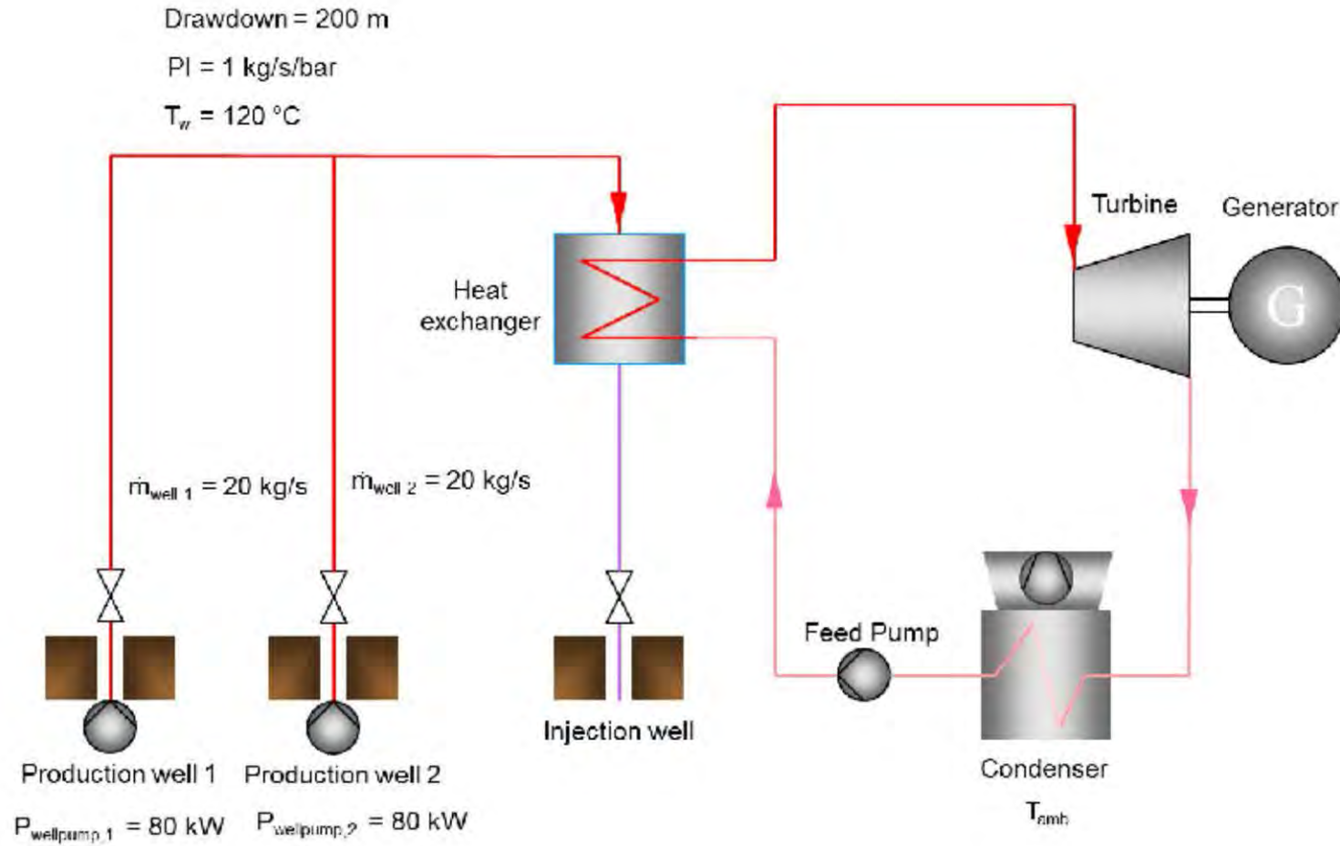
FIGURE 3 CASE 1 ORGANIC RANKINE CYCLE FLOW CHART
