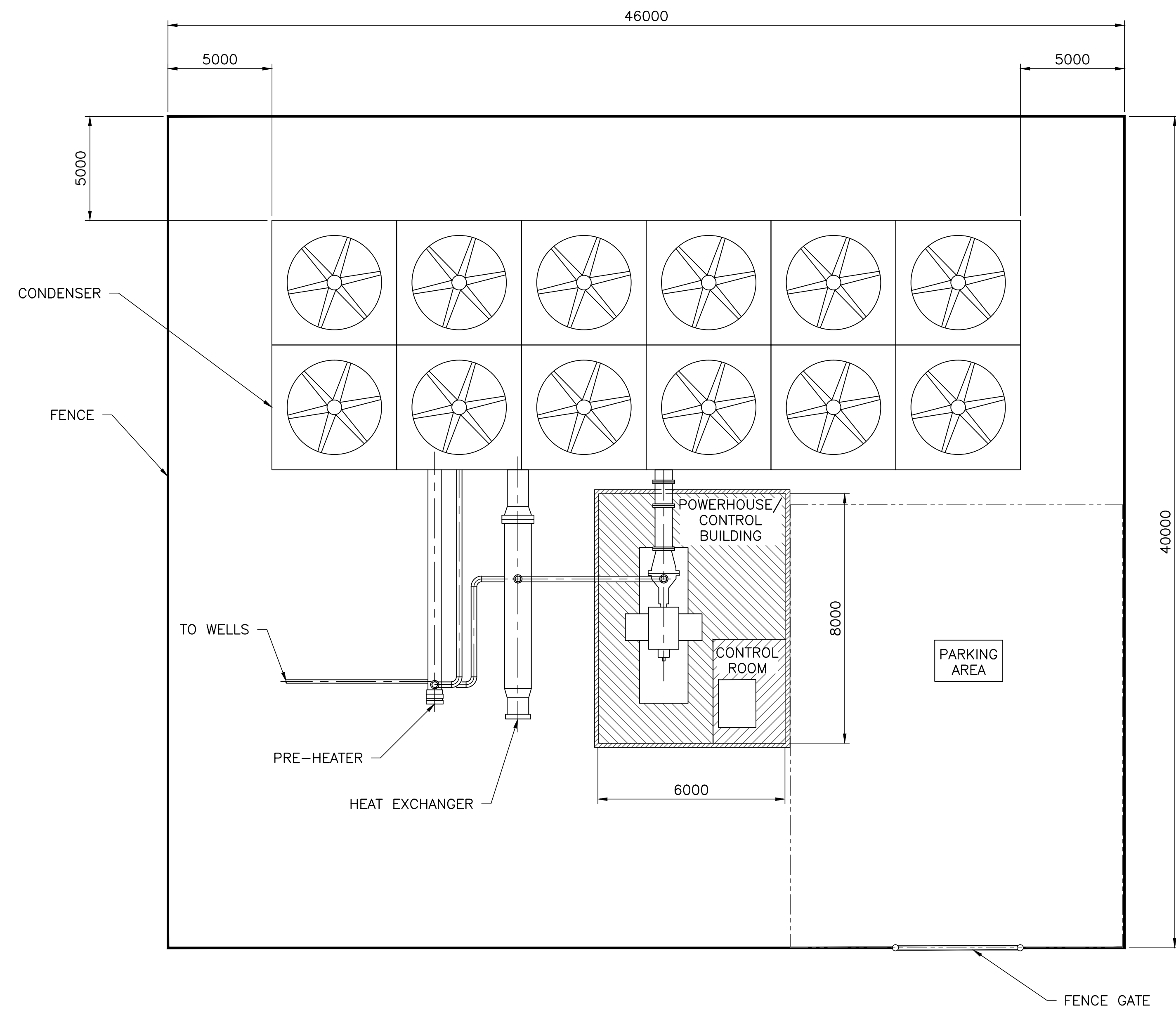
VISTA MOUNTAIN GEOTHERMAL ORC PLANT (1.2 MW)
