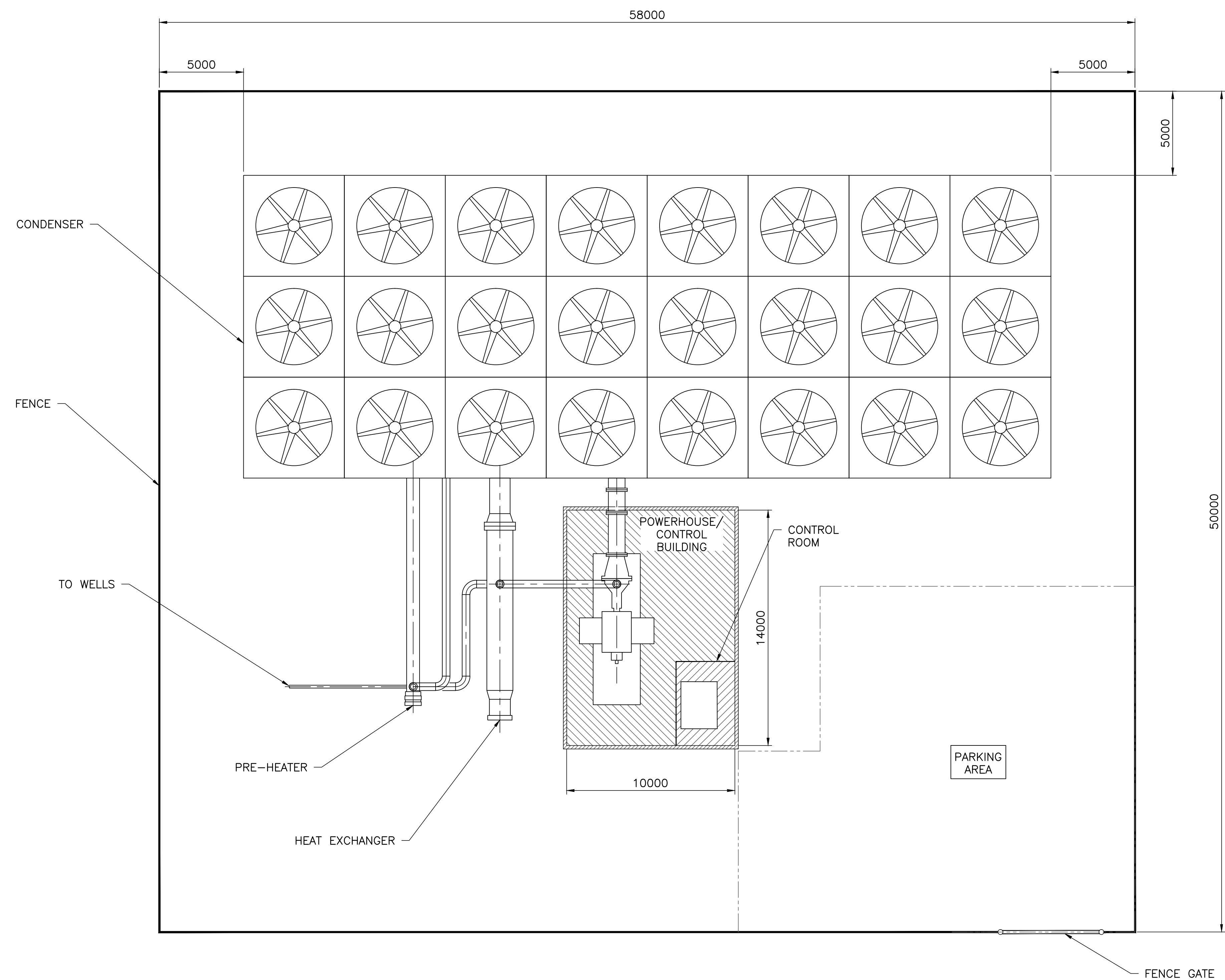
McARTHUR SPRINGS GEOTHERMAL ORC PLANT (2.8 MW)
