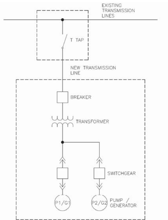
Figure 4.7 Indicative T-tap Interconnection Arrangement
