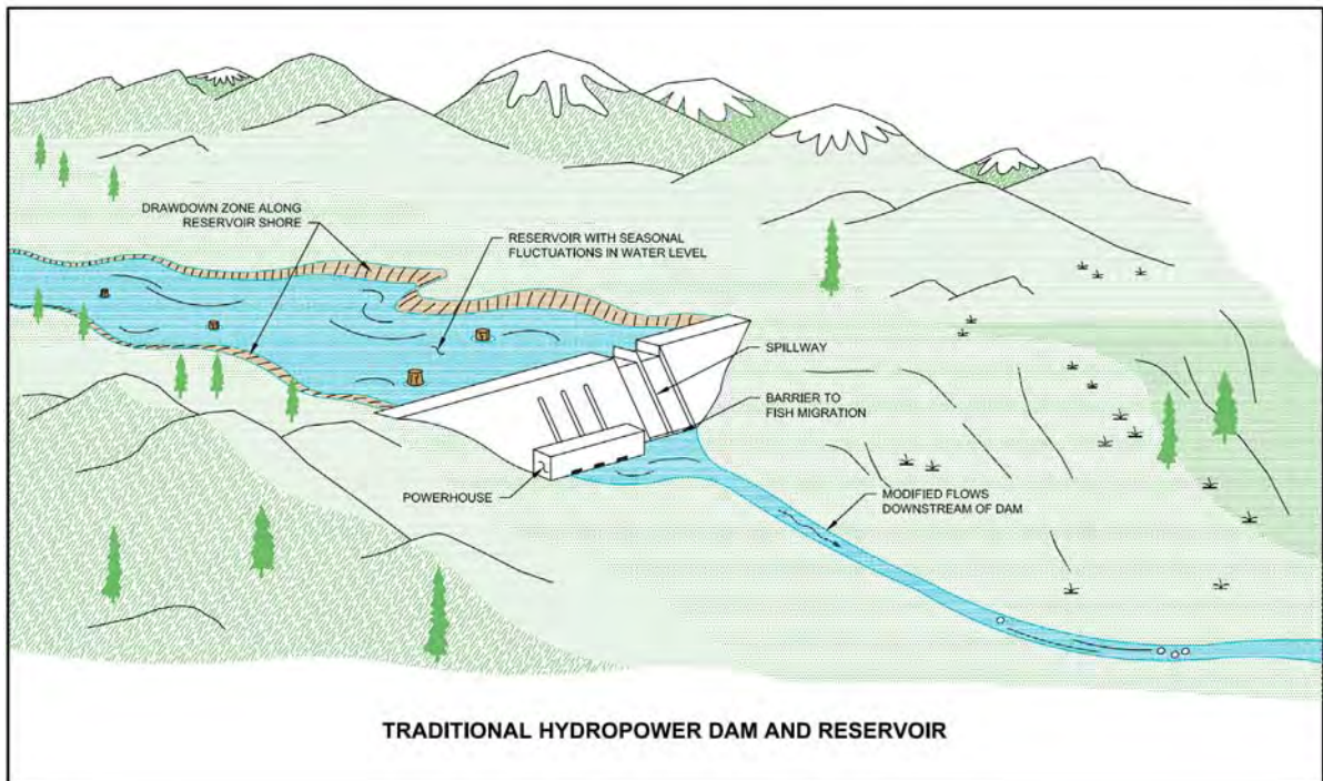
Figure 1.1 Conceptual Hydropower Project Layouts
