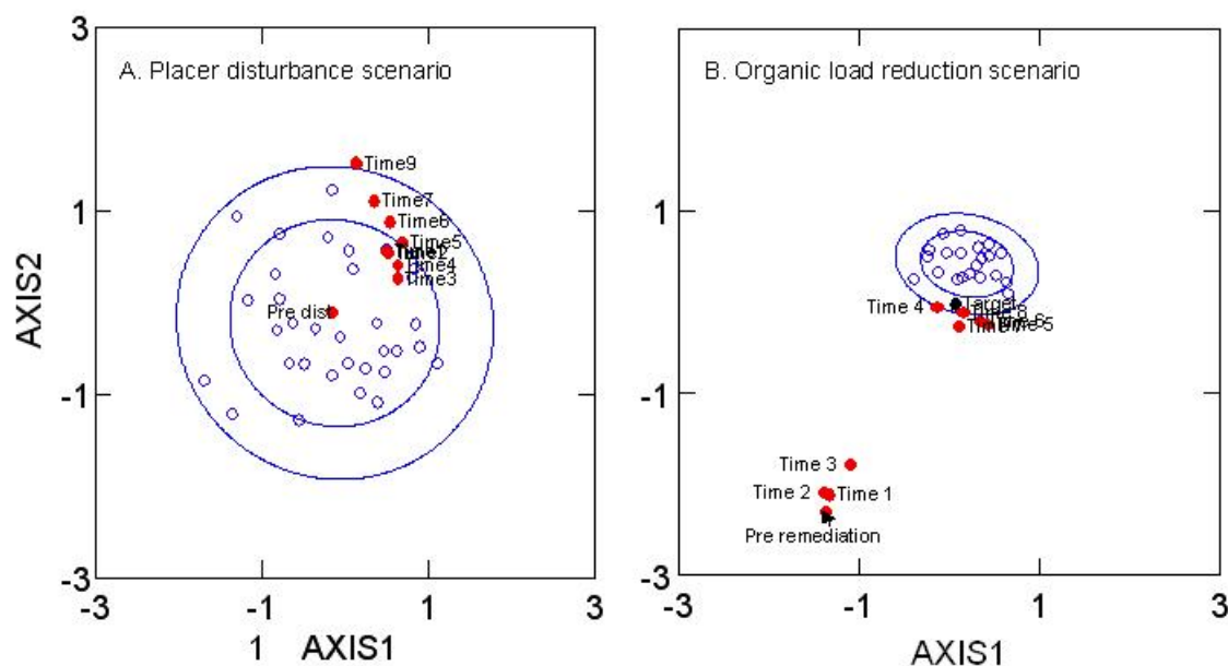
Figure 7. Assessment of temporal response to sites exposed to (A) sediment stress from placer activity and (B) recovery after reduction in organic load (simulated data show response through time) where time 1 is first response and time 9 is full manifestation of effect) probability ellipses are 75 and 95%.
