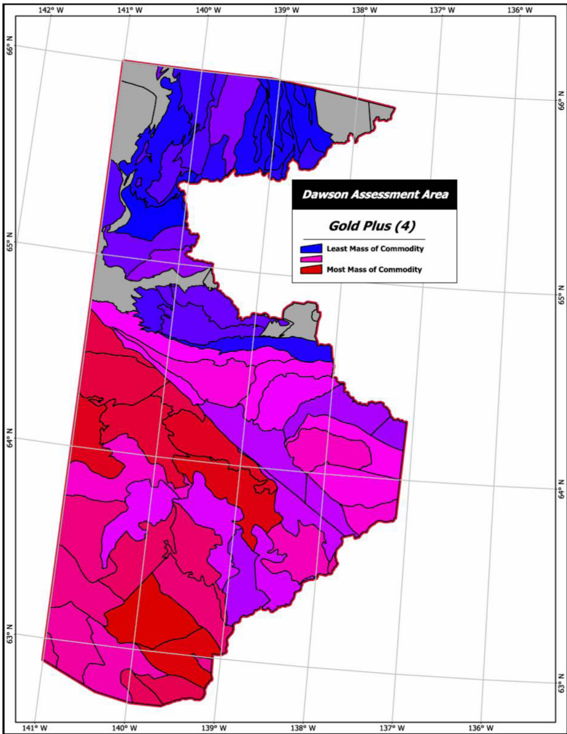
Figure 17. Relative distribution of Gold within the assessment area. The Plus designation indicates that this map includes the estimated plus known commodity amounts. Grey tracts contain no estimates.
