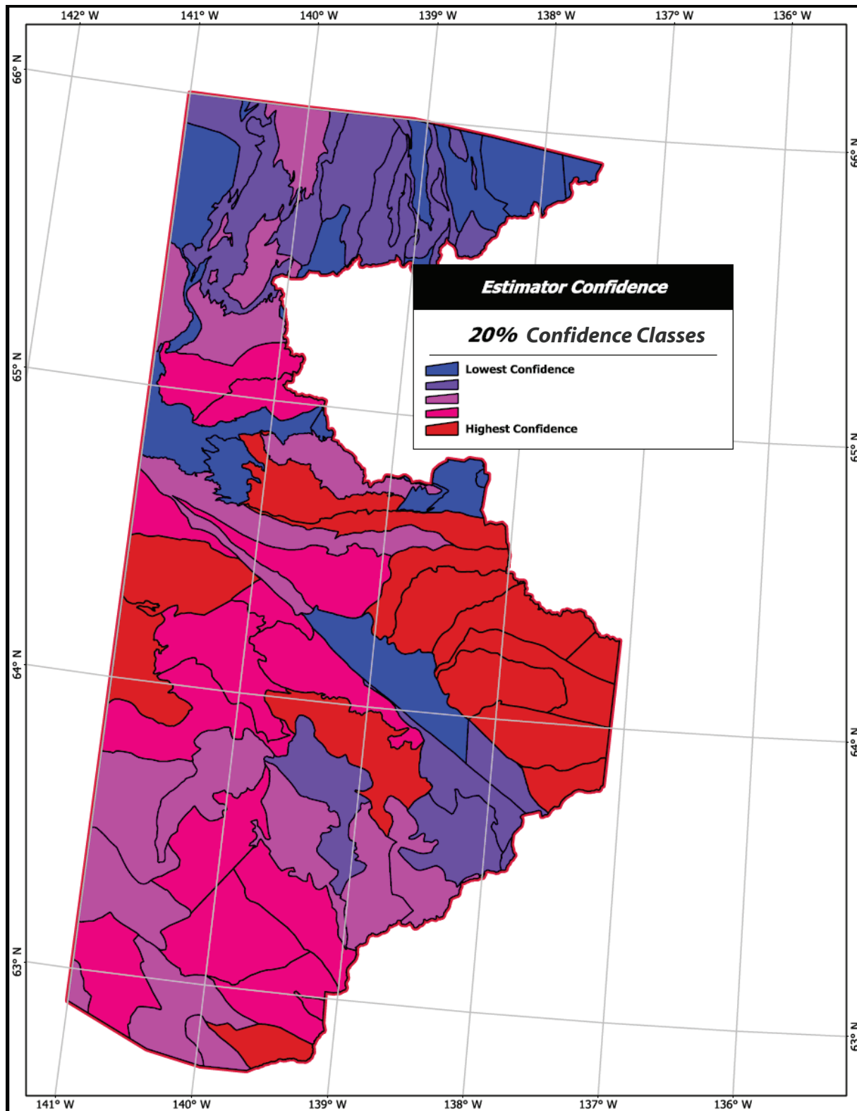
Figure 42. Distribution of normalized mean estimator confidence values grouped into five equal area classes.
