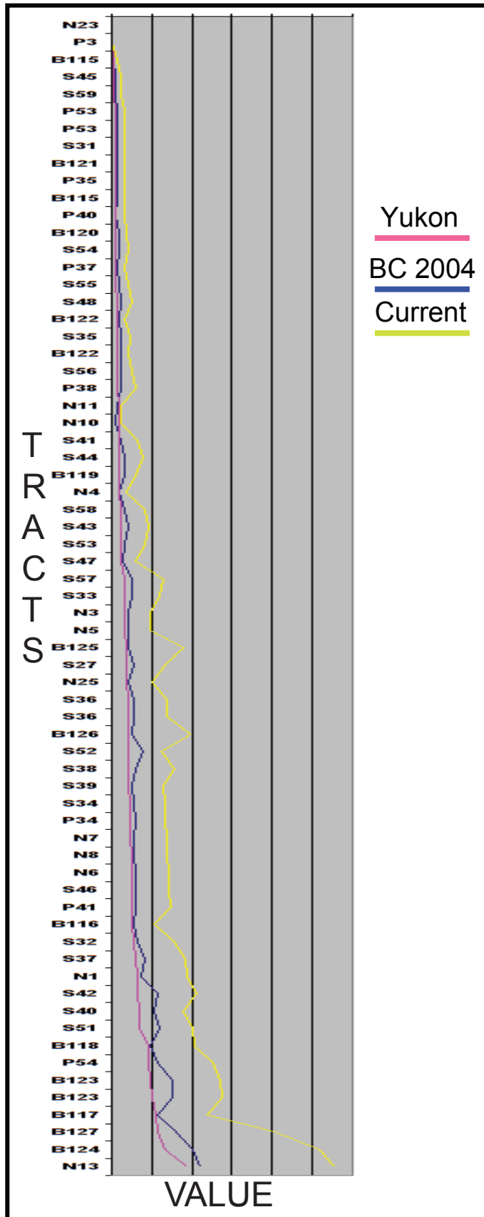
Figure 20. Graph showing the relative values of all commodities in each tract using the three different price lists. Each increment along the VALUE scale is $10,000,000.
