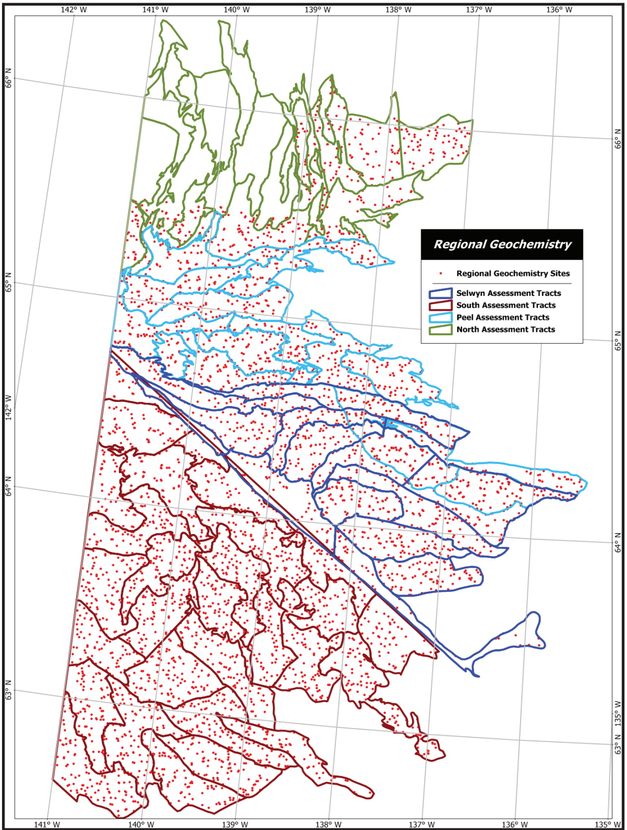
Figure 30. Distribution of regional geochemistry sample sites relative to the original workshop tract shapes.
