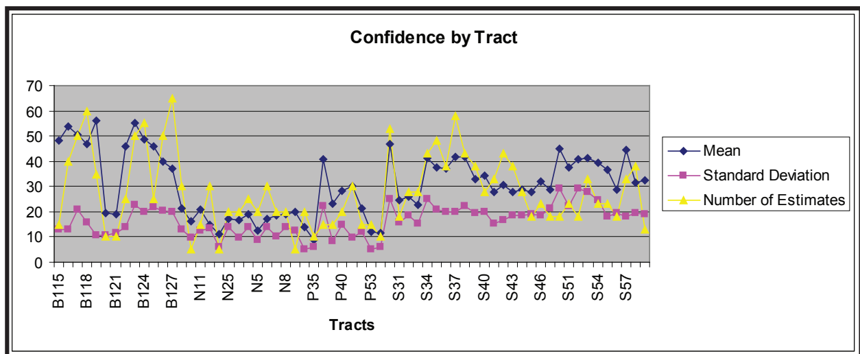
Figure 36. Graphical display of the combined raw estimator confidences for all of the tracts.
