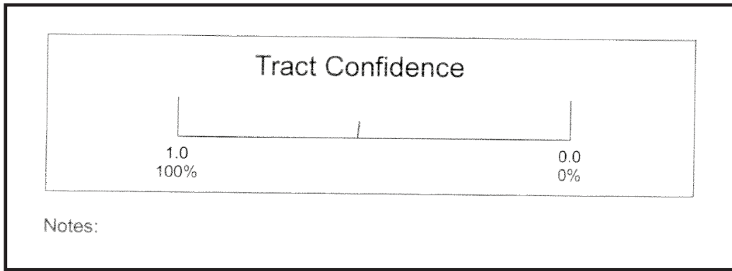
Figure 33. The section of the workshop coding sheet used by the estimator to indicate the level of confidence relative to the estimate recorded.
