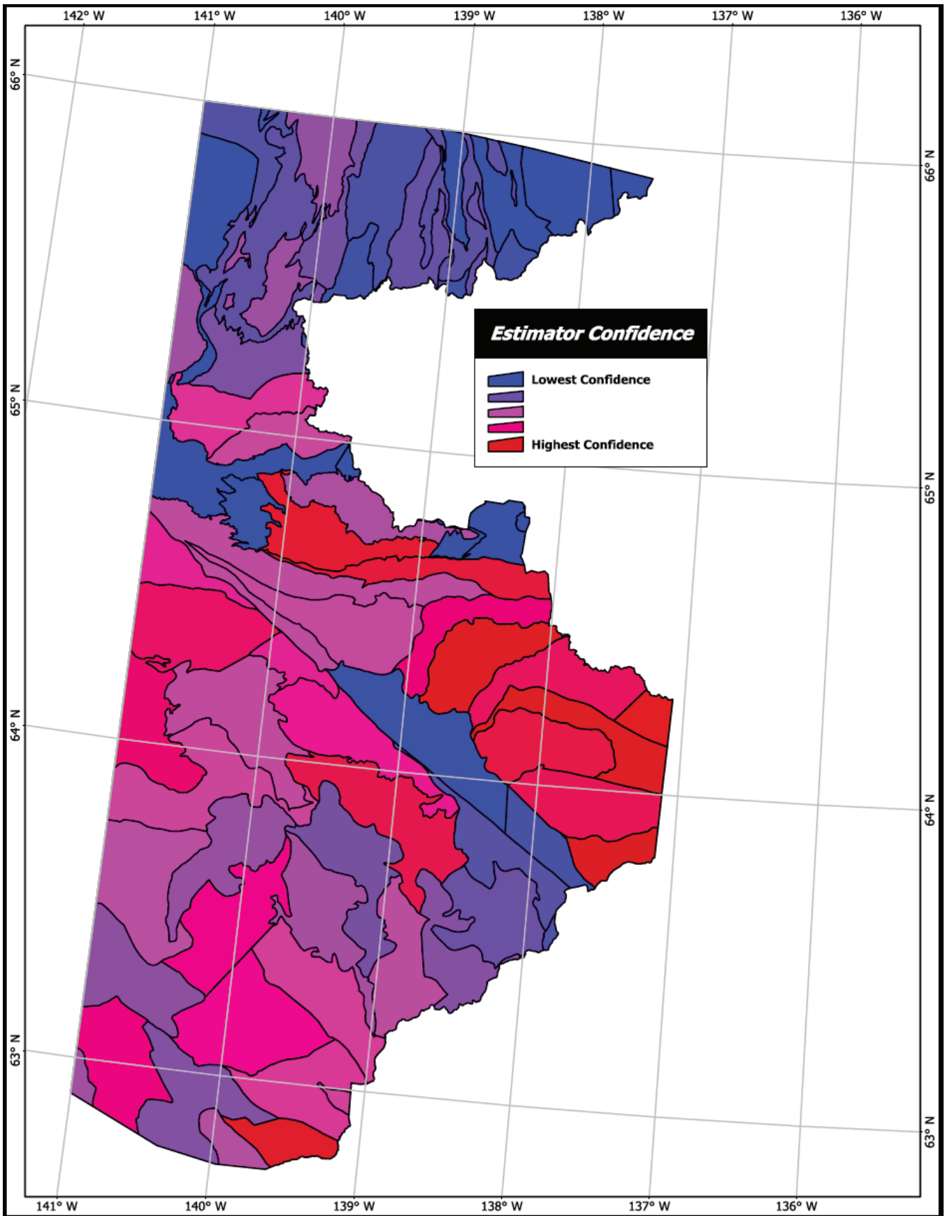
Figure 43. Distribution of normalized mean estimator confidence values with each tract shown as a unique colour.
