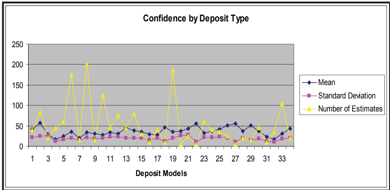
Figure 38. Display of raw estimator confidence statistics relative to the deposit types examined in the Dawson area.
