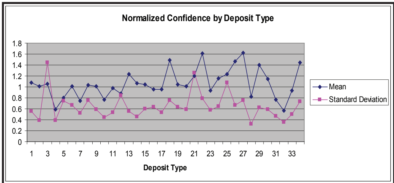
Figure 39. Normalized estimator confidence statistics relative to the different deposit types.
