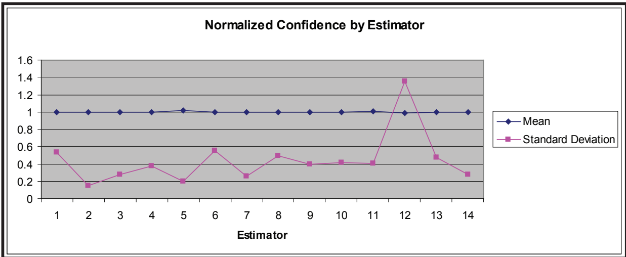
Figure 35. Display of the relative differences in estimator confidence standard deviation after the raw values have been normalized by dividing by the mean value for each estimator.
