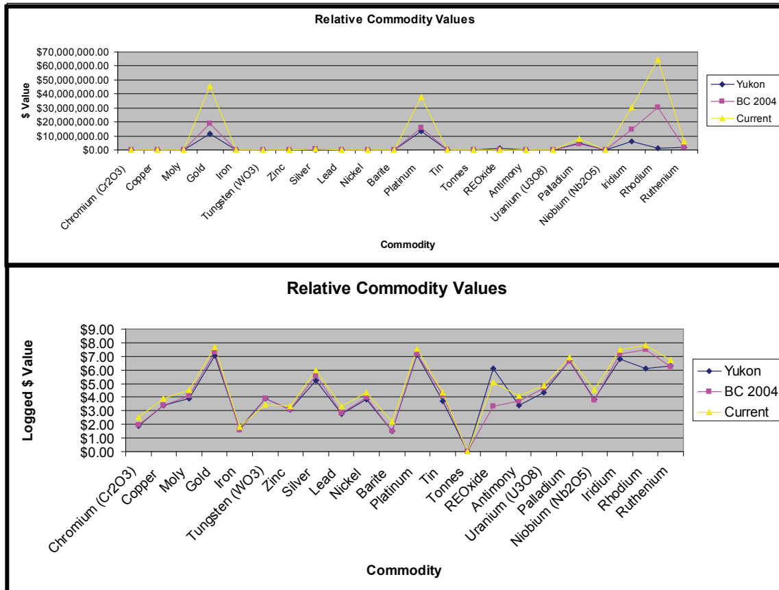
Figure 19. Graphs showing the relationships between the relative value of the commodities based on the three price lists. The lower graph is in logged dollar values.
