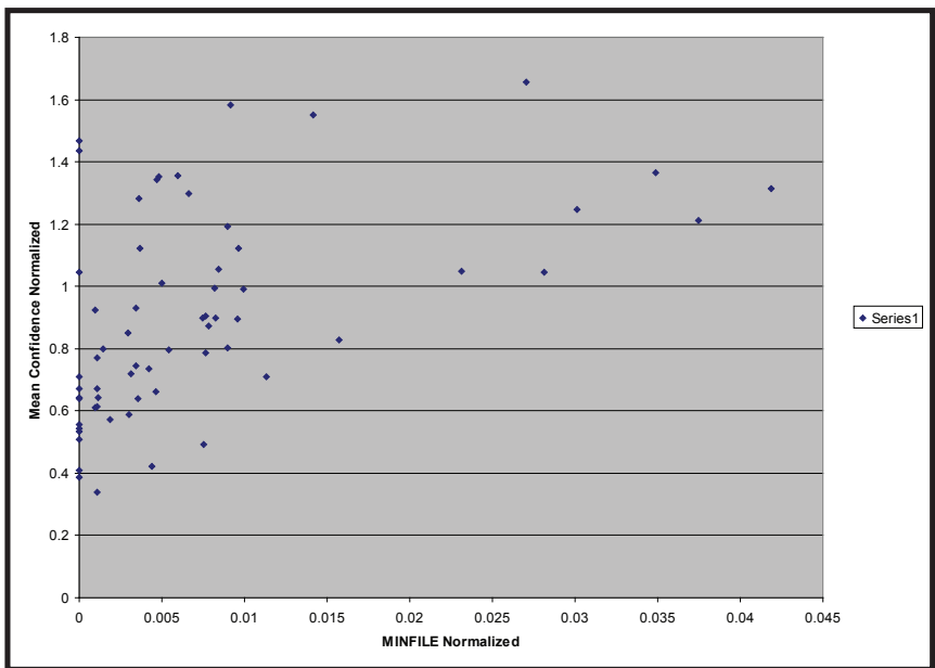
Figure 41. Cross plot showing the relationship between number of MINFILE occurrences in a tract and the normalized mean estimator confidence for the tract.
