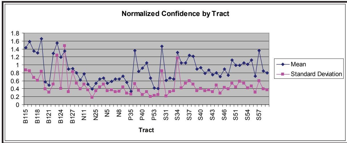
Figure 37. The mean and standard deviations of all estimator confidences in each tract. These values have been normalized to make comparing between estimators possible.
