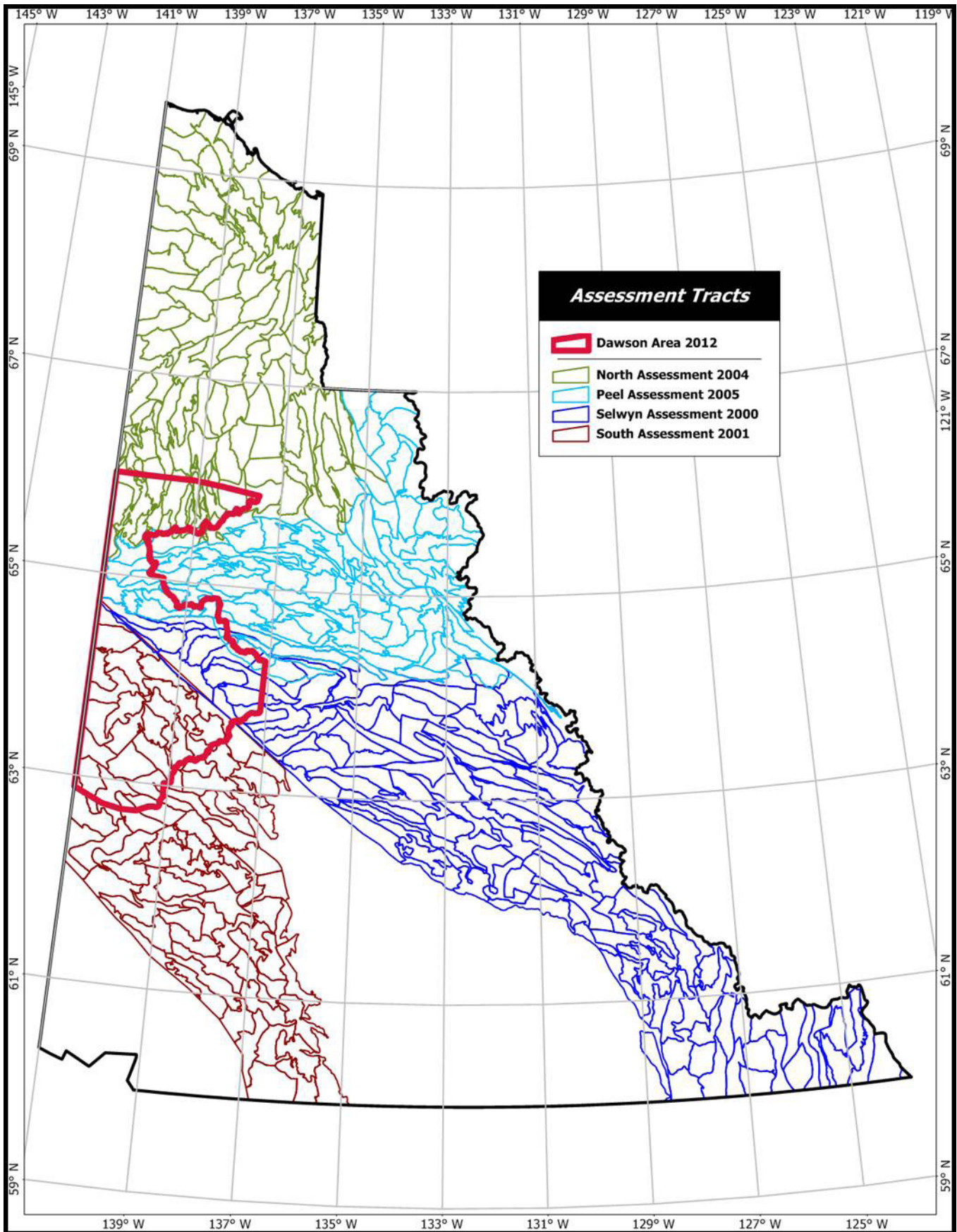
Figure 1. Tracts from the four original mineral potential assessments used in this compilation. Bold red outline is the Dawson assessment area.
