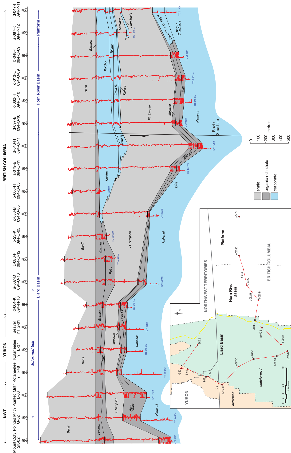
Figure A.1. Cross-section across study area with Exshaw top as datum
