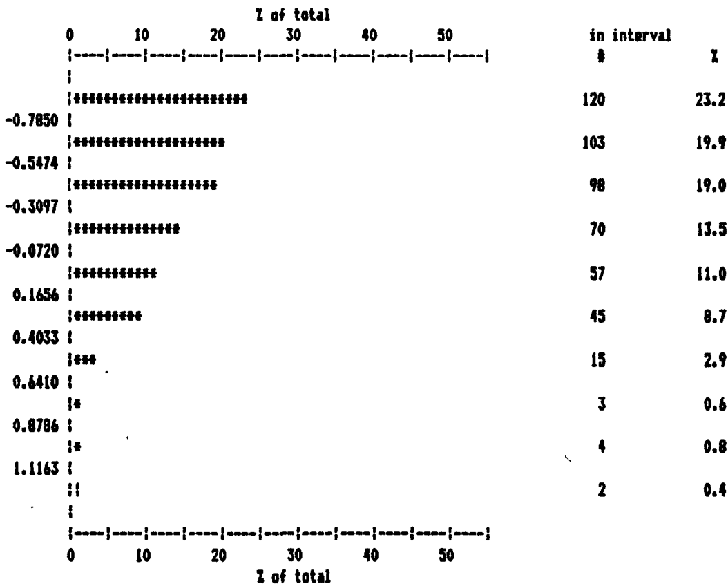
Histogram for Log10 Ag ( LOGAG )
