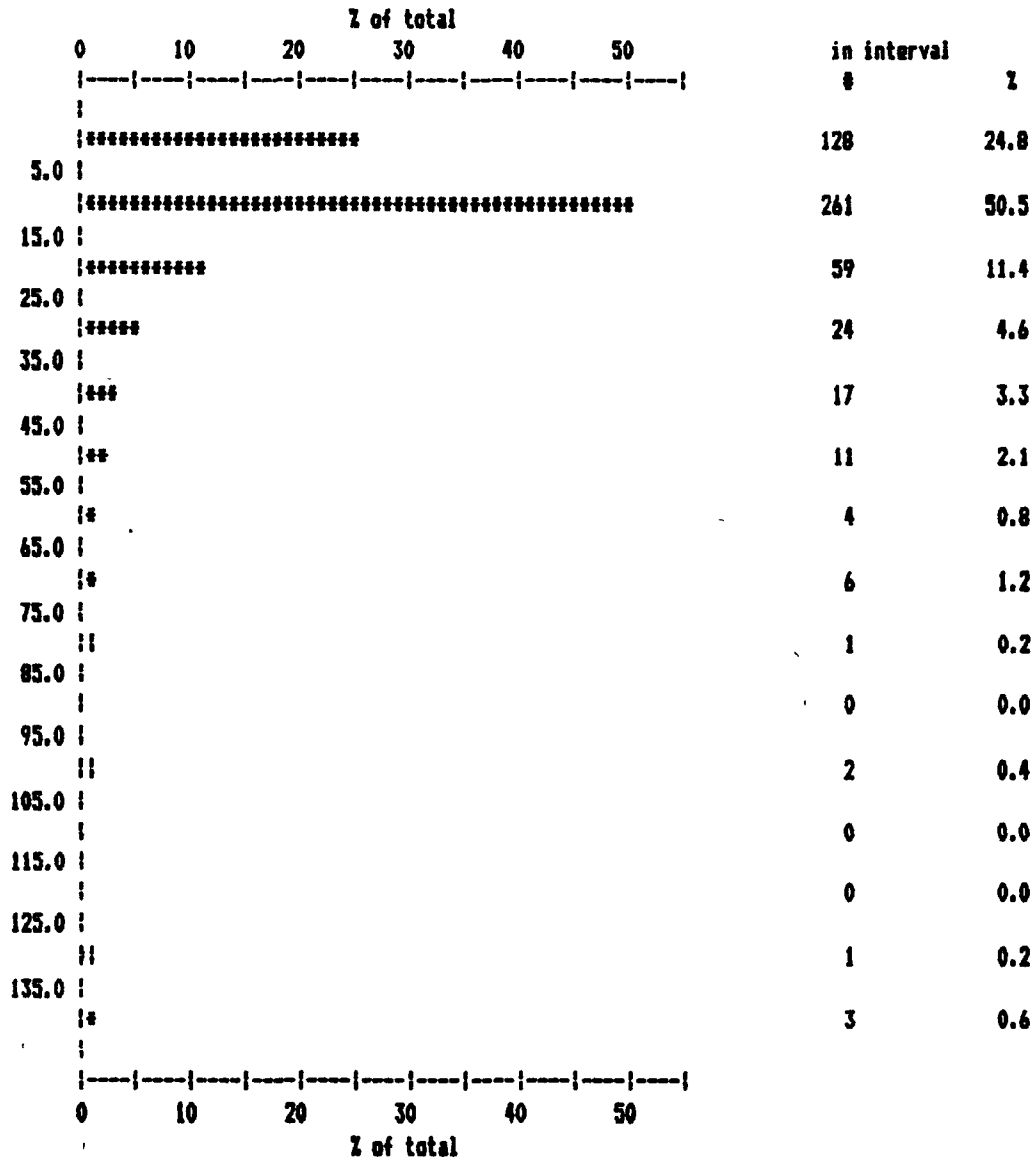
Histogram for Gold ( AU ) Values in PPD
